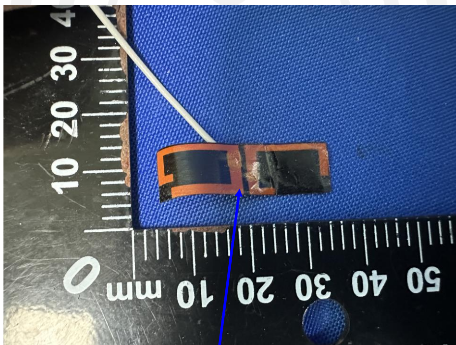
WiFi ANT
