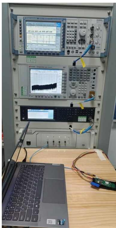
Test Setup Photo(s) of RF Conducted Measurement
