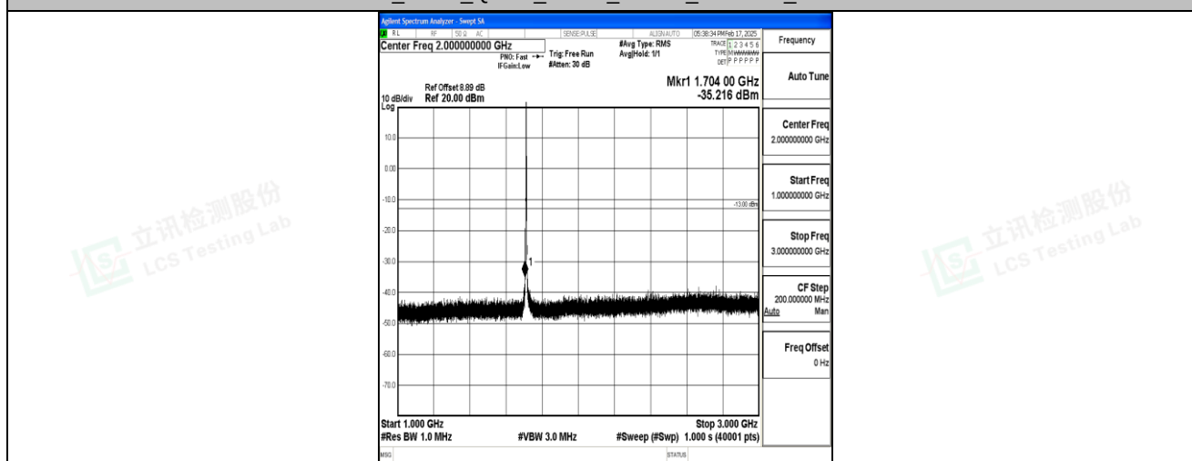
Band4_3MHz_QPSK_19965_1RB#0_1000~3000_1000~3000
