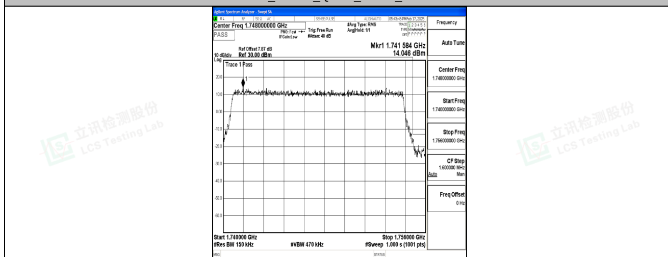
Band4_15MHz_16QAM_20325_75RB#0
