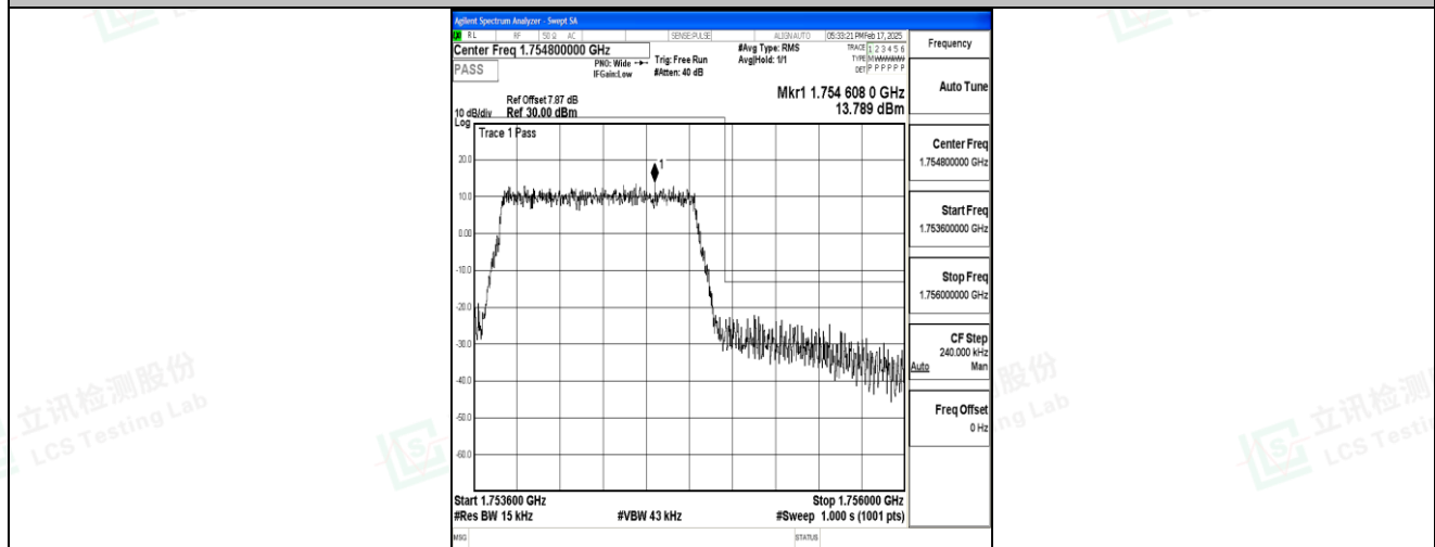
Band4_1.4MHz_16QAM_20393_6RB#0
