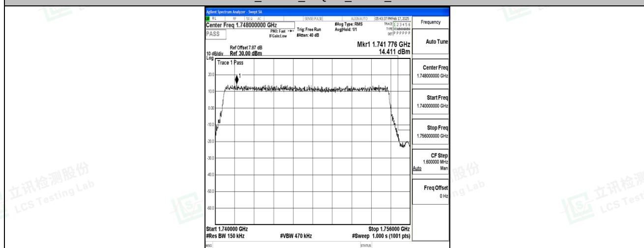
Band4_15MHz_QPSK_20325_75RB#0
