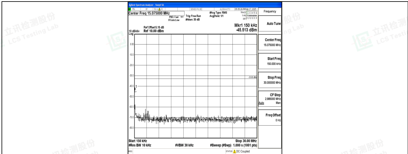
Band4_1.4MHz_16QAM_20175_1RB#0_0.15~30_0.15~30
