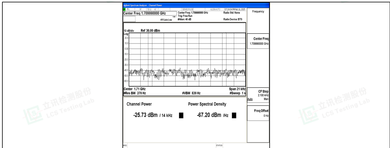
Band4_1.4MHz_16QAM_19957_6RB#0_Final1
