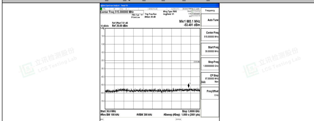
Band4_3MHz_QPSK_20175_1RB#0_30~1000_30~1000
