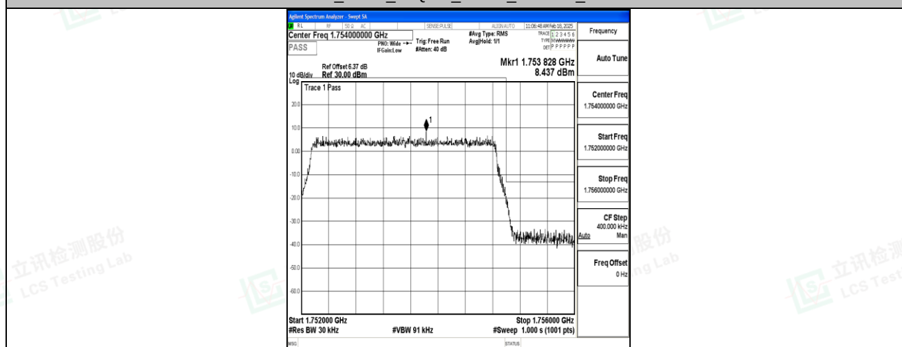
Band4_3MHz_QPSK_20385_15RB#0
