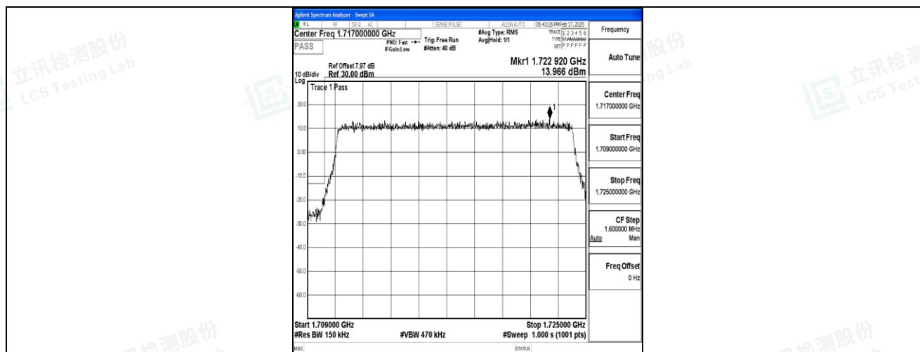
Band4_15MHz_16QAM_20025_75RB#0
