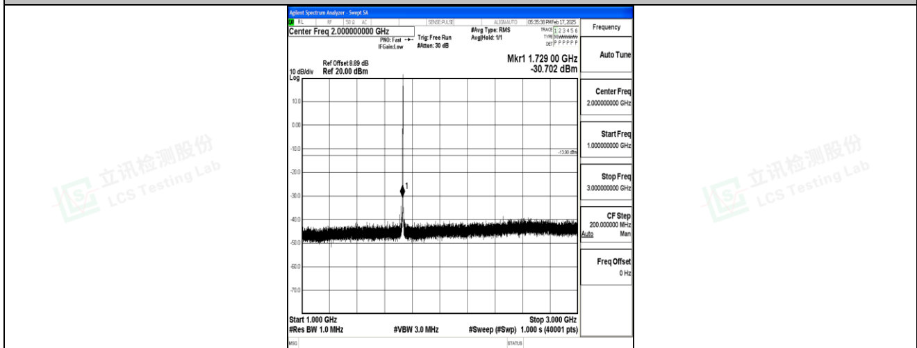
Band4_1.4MHz_16QAM_20175_1RB#0_1000~3000_1000~3000
