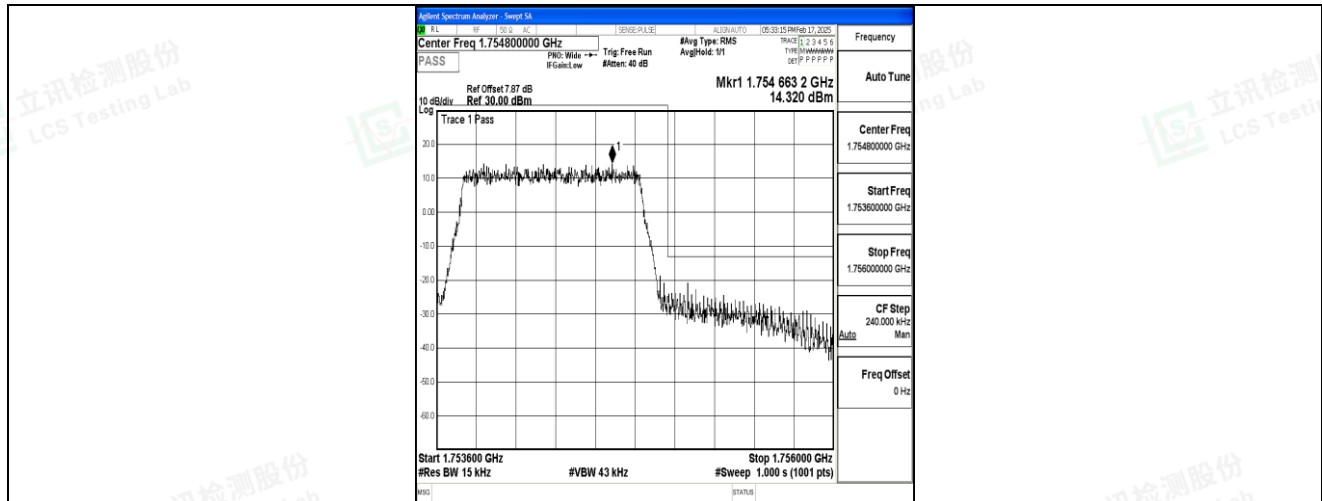
Band4_1.4MHz_QPSK_20393_6RB#0
