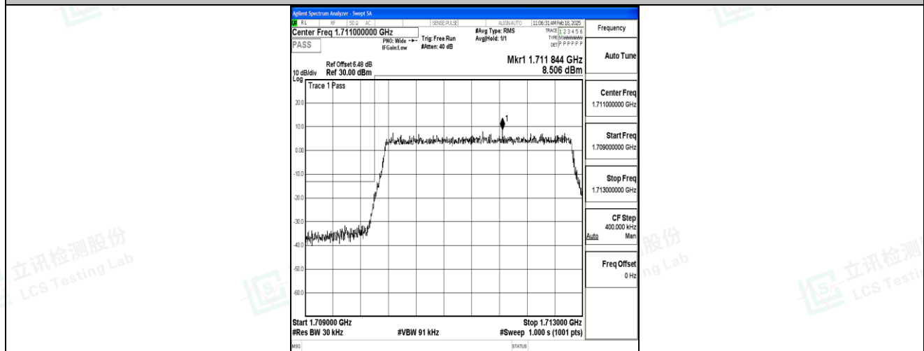
Band4_3MHz_QPSK_19965_15RB#0
