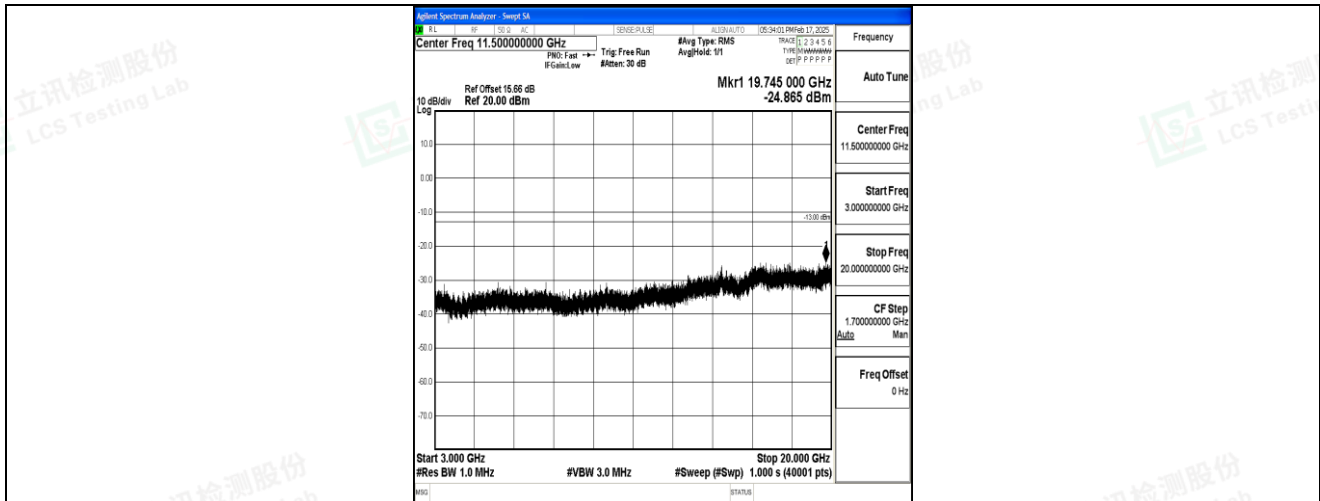
Band4_1.4MHz_QPSK_19957_1RB#0_3000~20000_3000~20000
