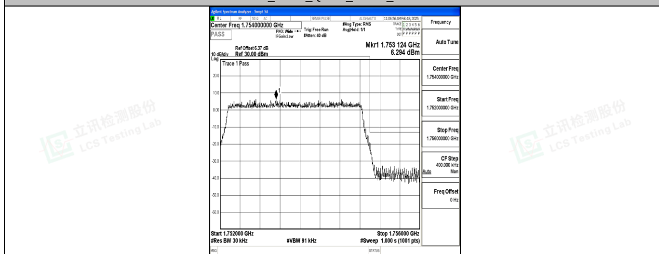
Band4_3MHz_16QAM_20385_15RB#0
