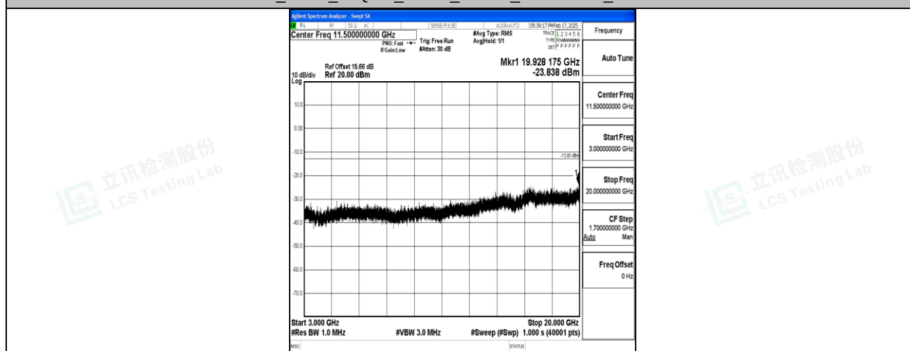
Band4_3MHz_16QAM_19965_1RB#0_3000~20000_3000~20000
