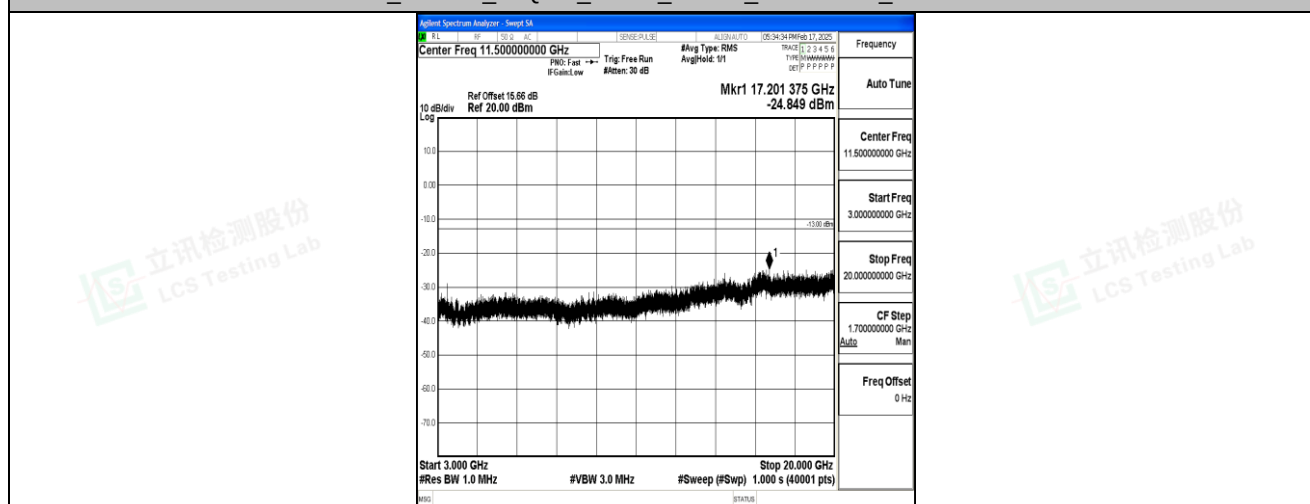
Band4_1.4MHz_16QAM_19957_1RB#0_3000~20000_3000~20000
