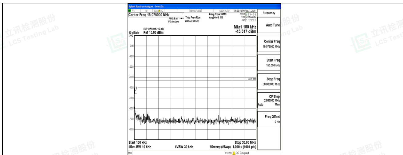
Band4_1.4MHz_QPSK_19957_1RB#0_0.15~30_0.15~30
