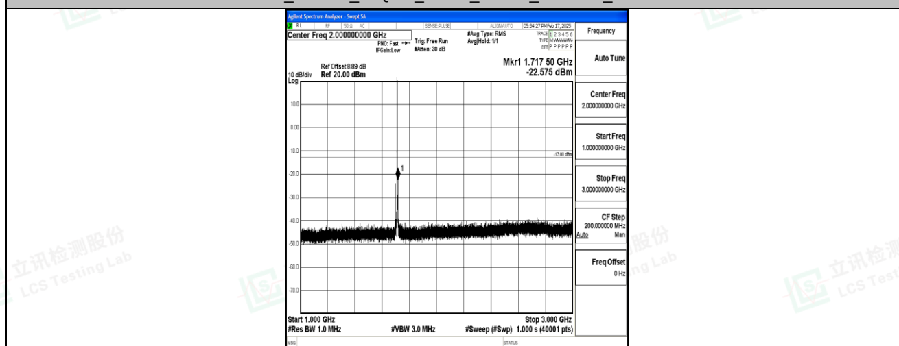
Band4_1.4MHz_16QAM_19957_1RB#0_1000~3000_1000~3000
