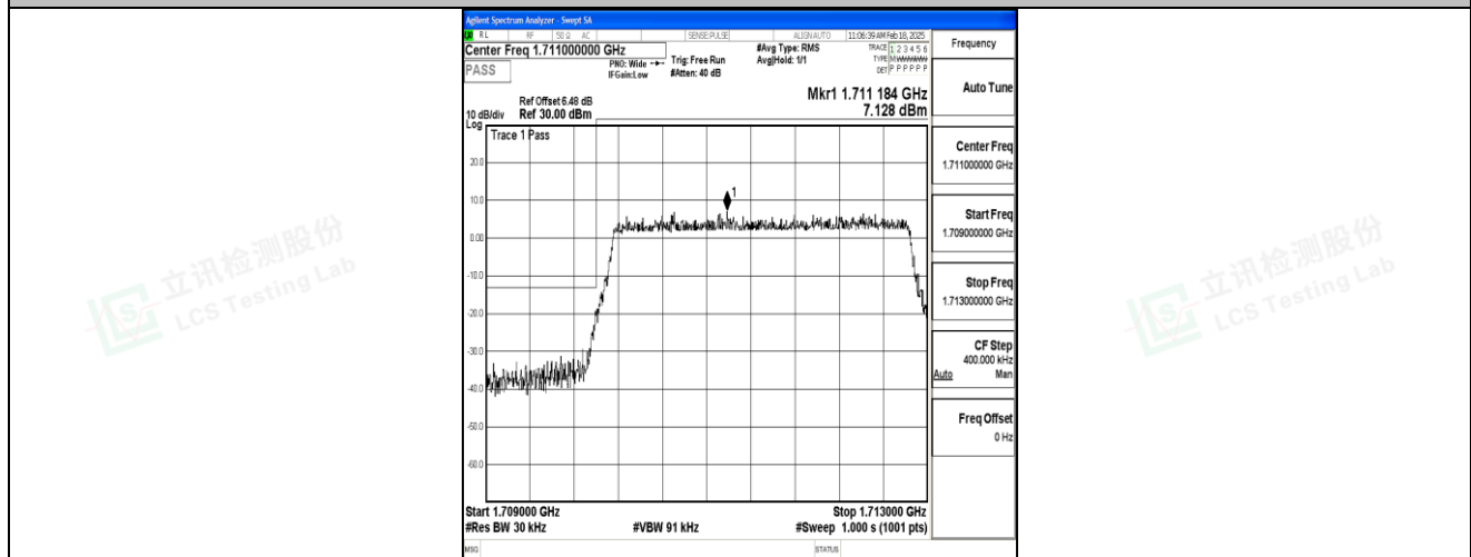
Band4_3MHz_16QAM_19965_15RB#0
