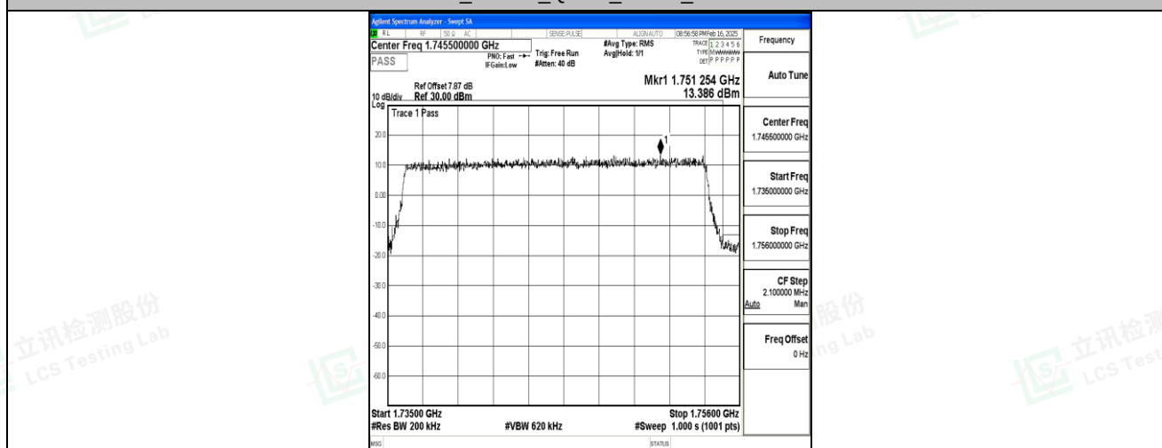
Band4_20MHz_16QAM_20300_100RB#0
