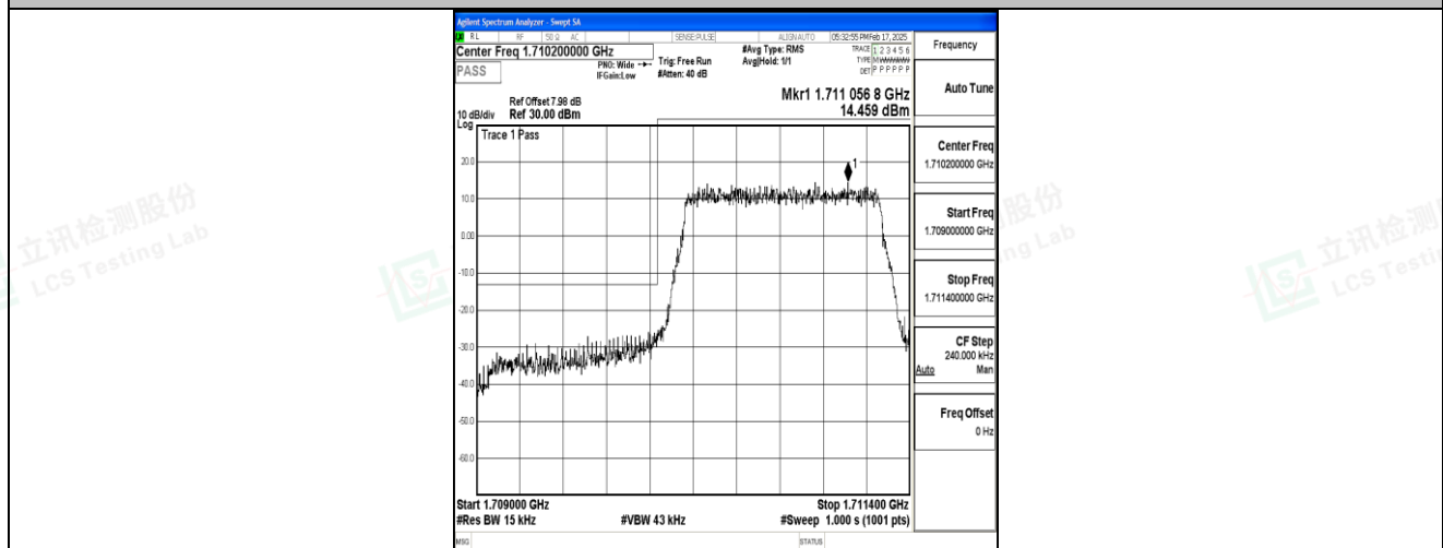
Band4_1.4MHz_QPSK_19957_6RB#0
