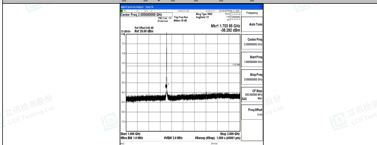
Band4_3MHz_16QAM_19965_1RB#0_1000~3000_1000~3000
