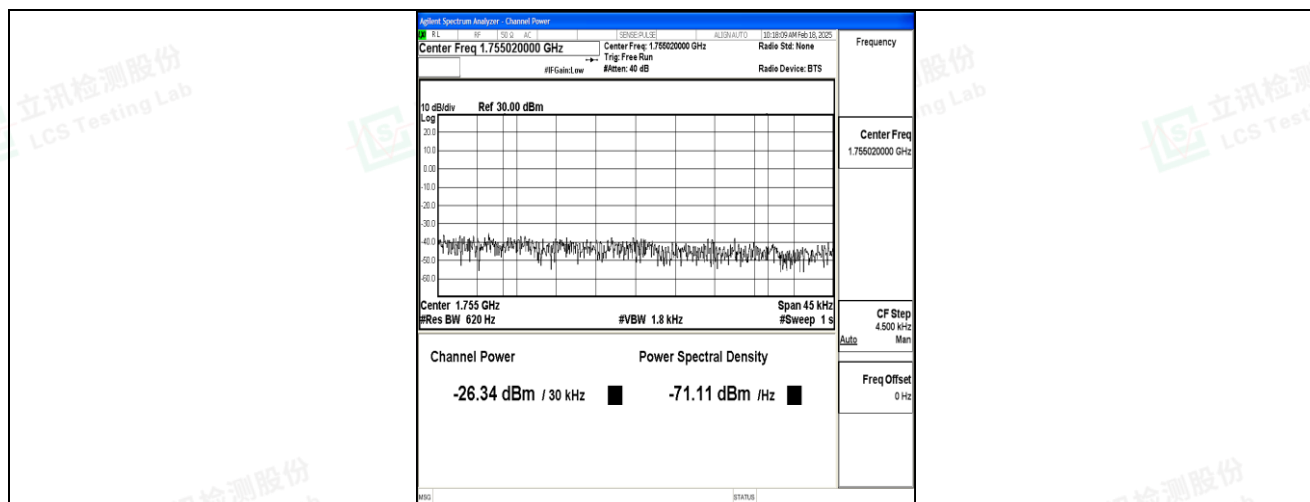
Band4_3MHz_16QAM_20385_15RB#0_Final1
