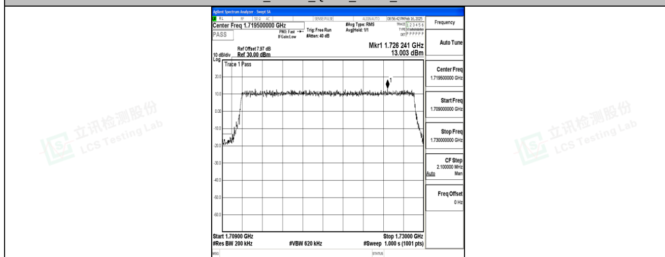
Band4_20MHz_16QAM_20050_100RB#0
