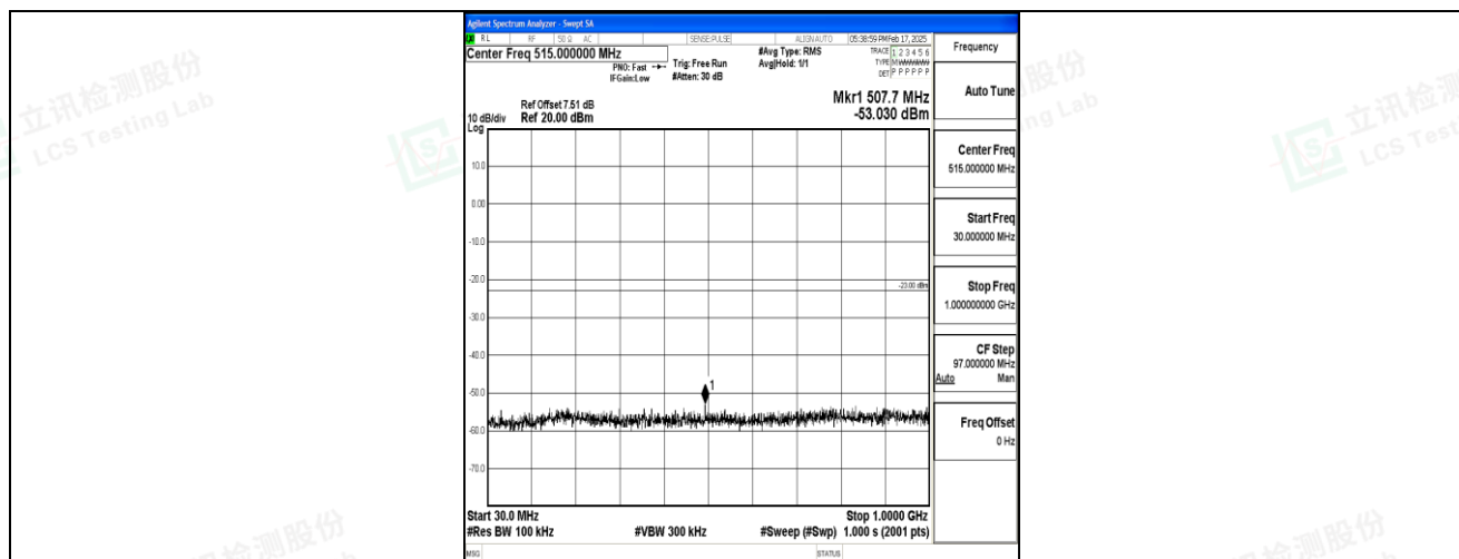
Band4_3MHz_16QAM_19965_1RB#0_30~1000_30~1000
