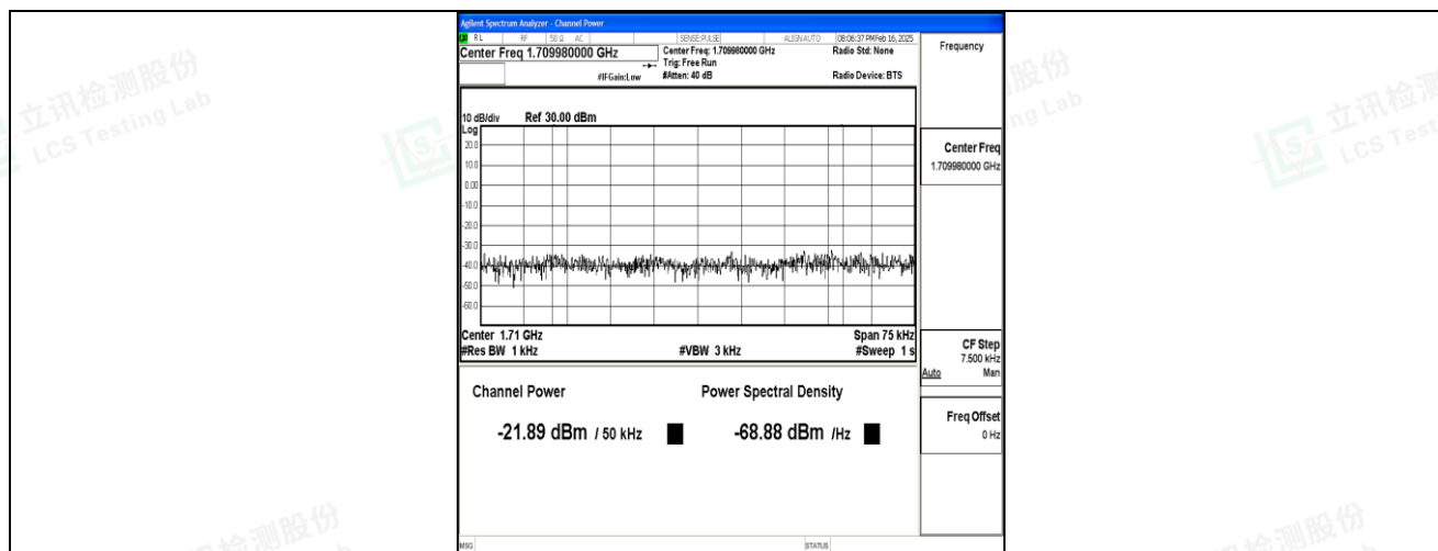
Band4_5MHz_QPSK_19975_25RB#0_Final1
