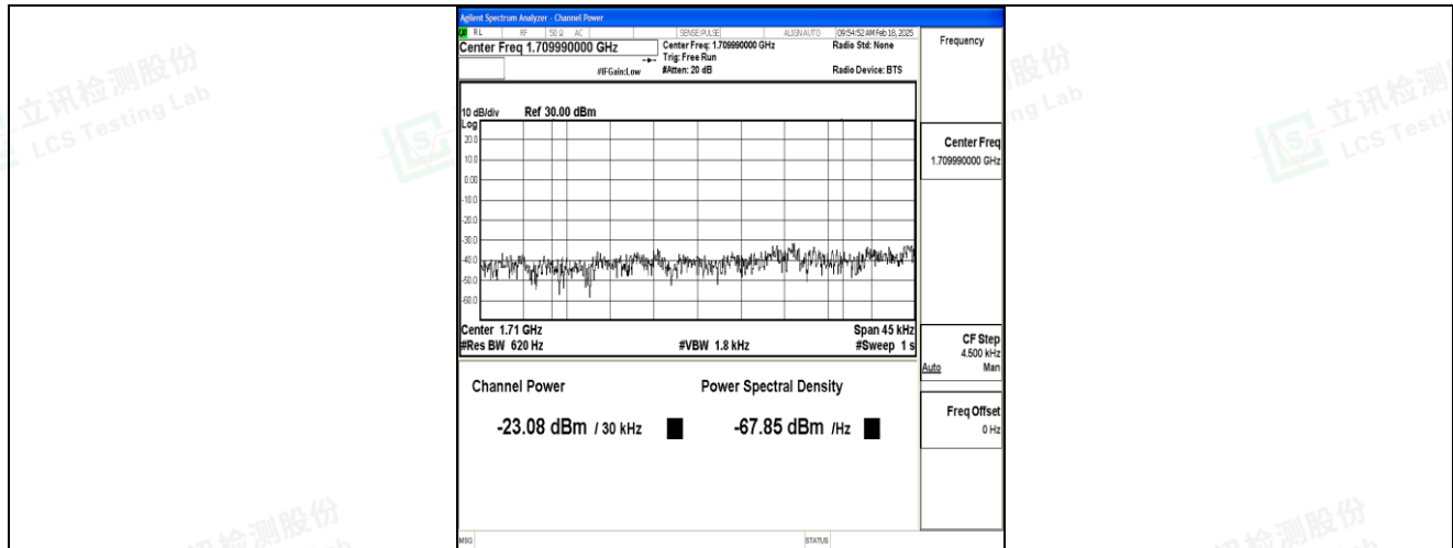
Band4_3MHz_QPSK_19965_15RB#0_Final1
