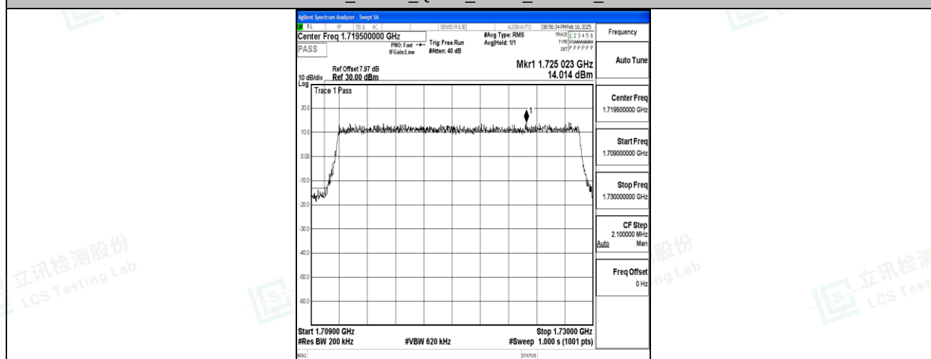
Band4_20MHz_QPSK_20050_100RB#0
