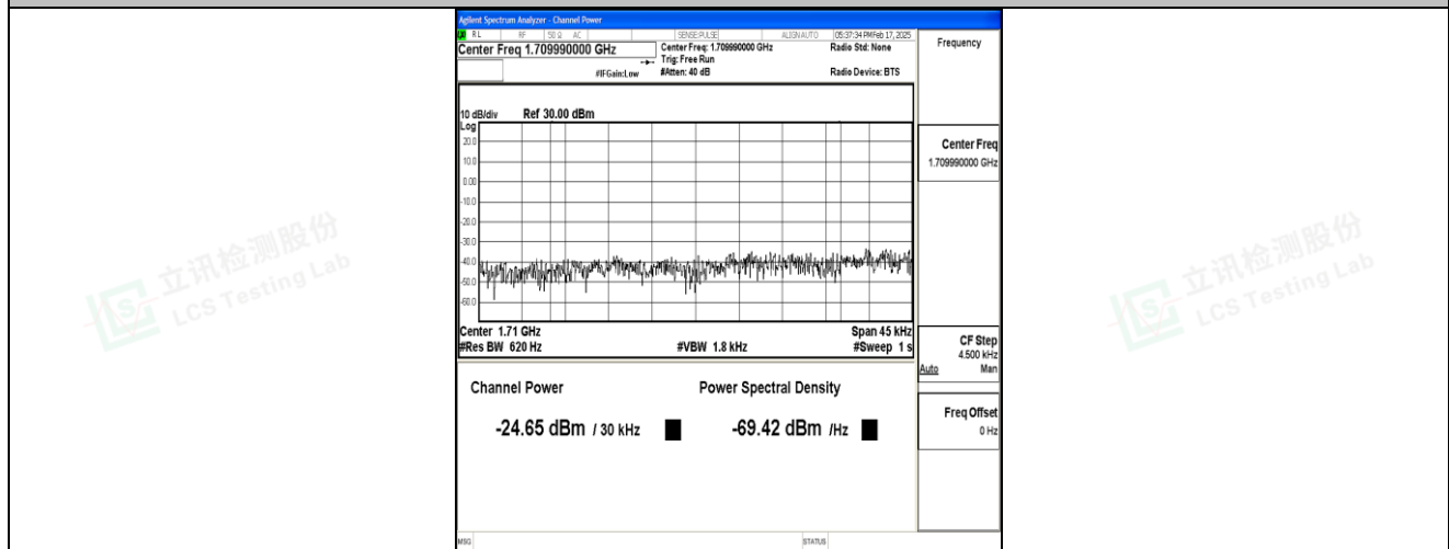
Band4_3MHz_16QAM_19965_15RB#0_Final1
