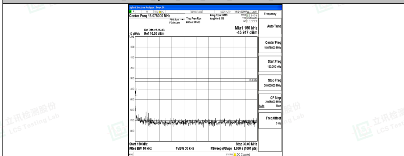
Band4_1.4MHz_QPSK_20175_1RB#0_0.15~30_0.15~30
