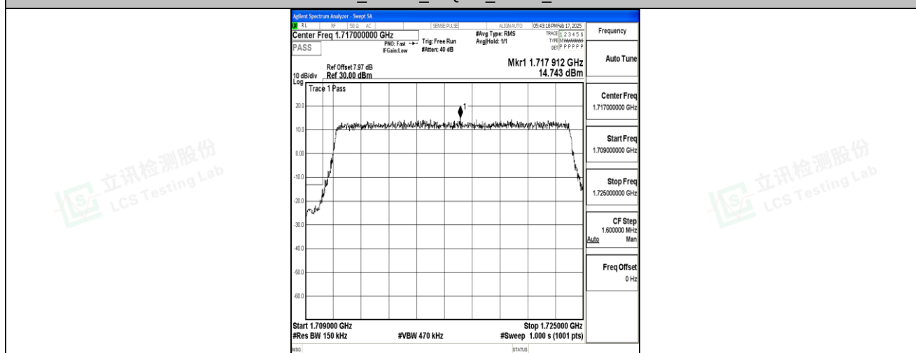
Band4_15MHz_QPSK_20025_75RB#0
