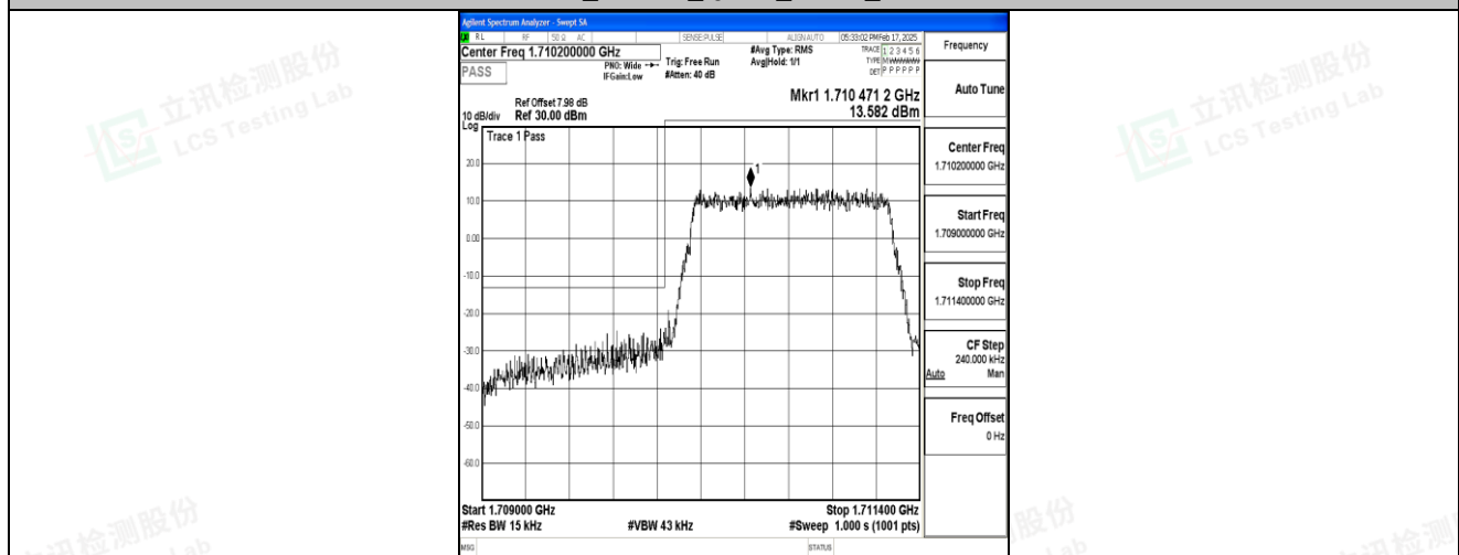
Band4_1.4MHz_16QAM_19957_6RB#0
