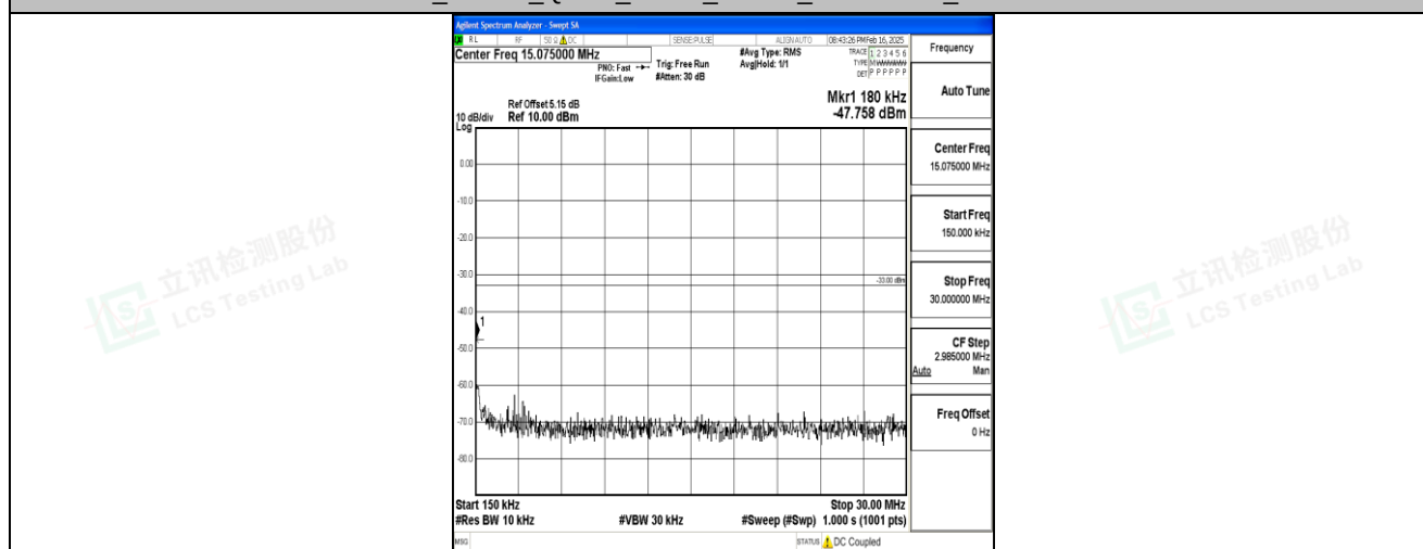
Band4_15MHz_QPSK_20325_1RB#0_0.15~30_0.15~30
