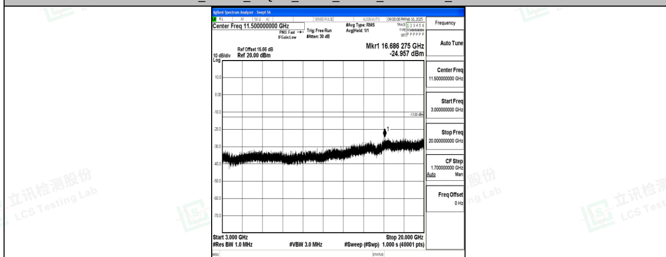
Band4_20MHz_16QAM_20300_1RB#0_3000~20000_3000~20000
