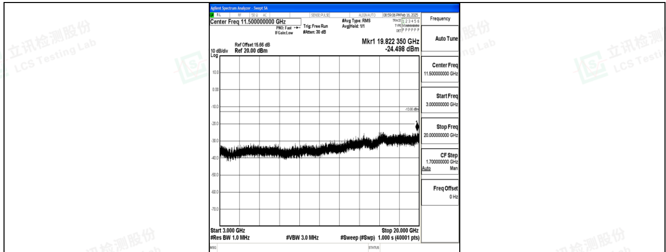
Band4_20MHz_16QAM_20175_1RB#0_3000~20000_3000~20000
