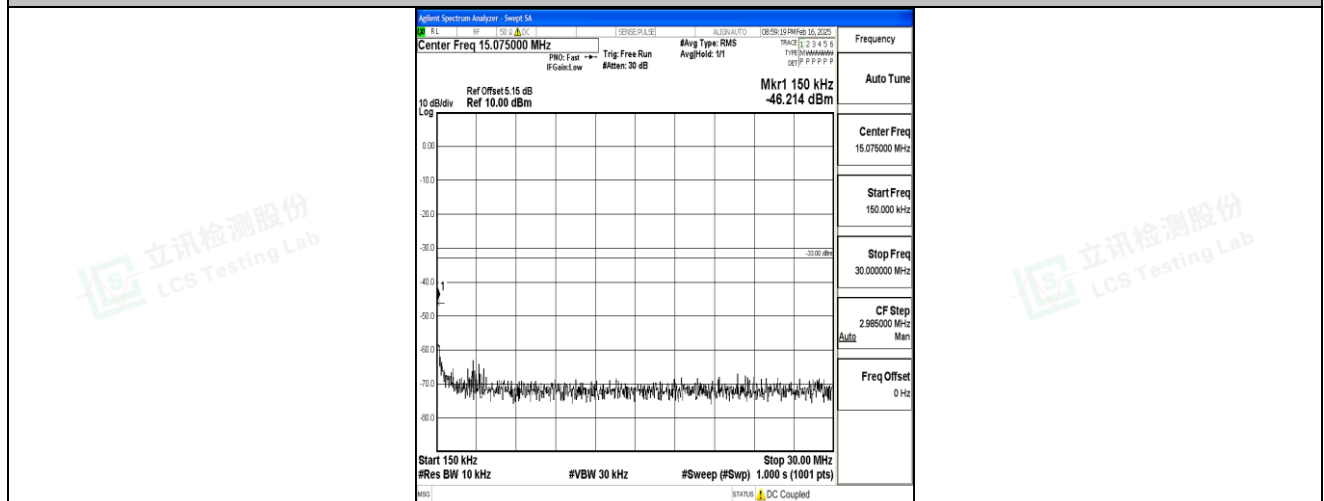
Band4_20MHz_QPSK_20300_1RB#0_0.15~30_0.15~30
