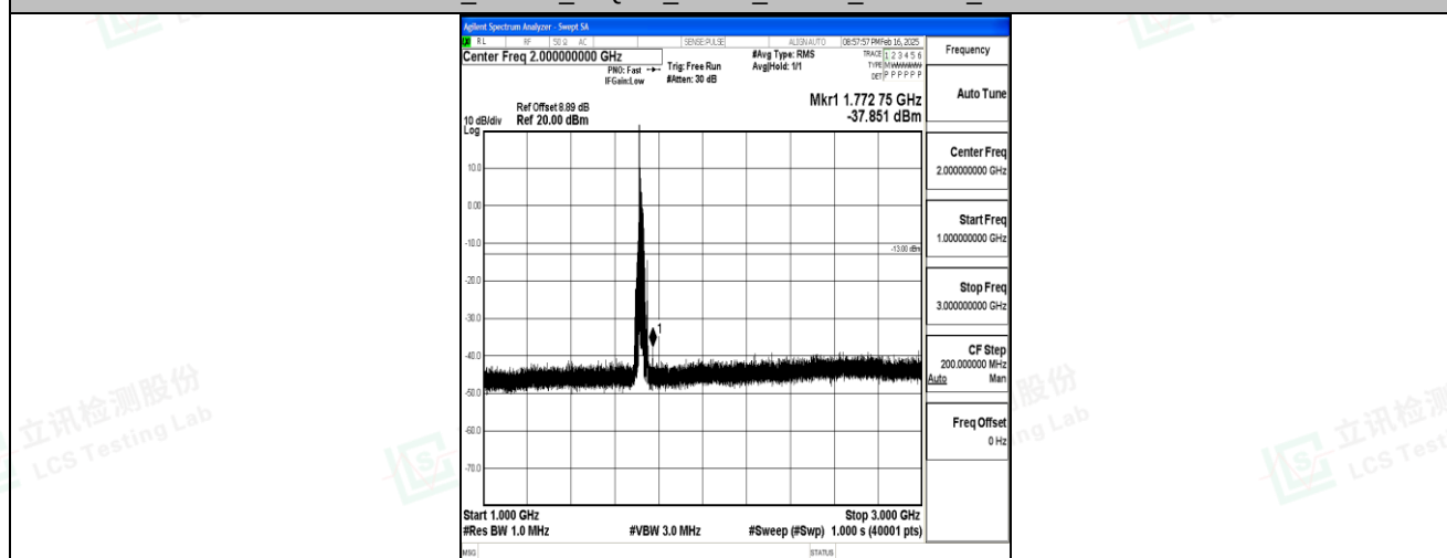
Band4_20MHz_16QAM_20050_1RB#0_1000~3000_1000~3000
