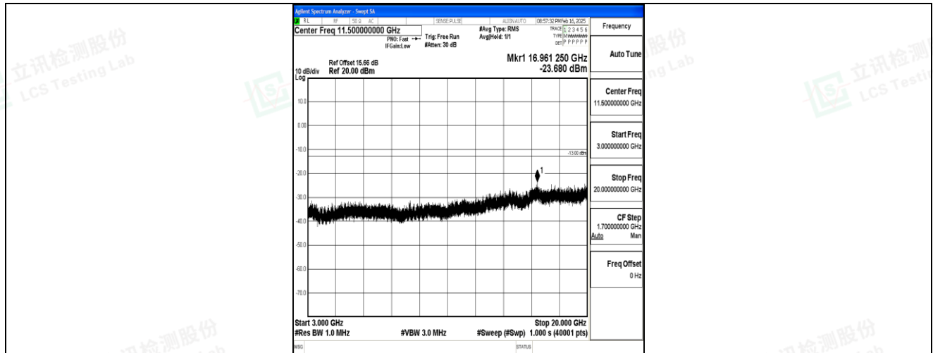
Band4_20MHz_QPSK_20050_1RB#0_3000~20000_3000~20000
