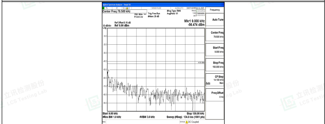
Band4_20MHz_16QAM_20050_1RB#0_0.009~0.15_0.009~0.15
