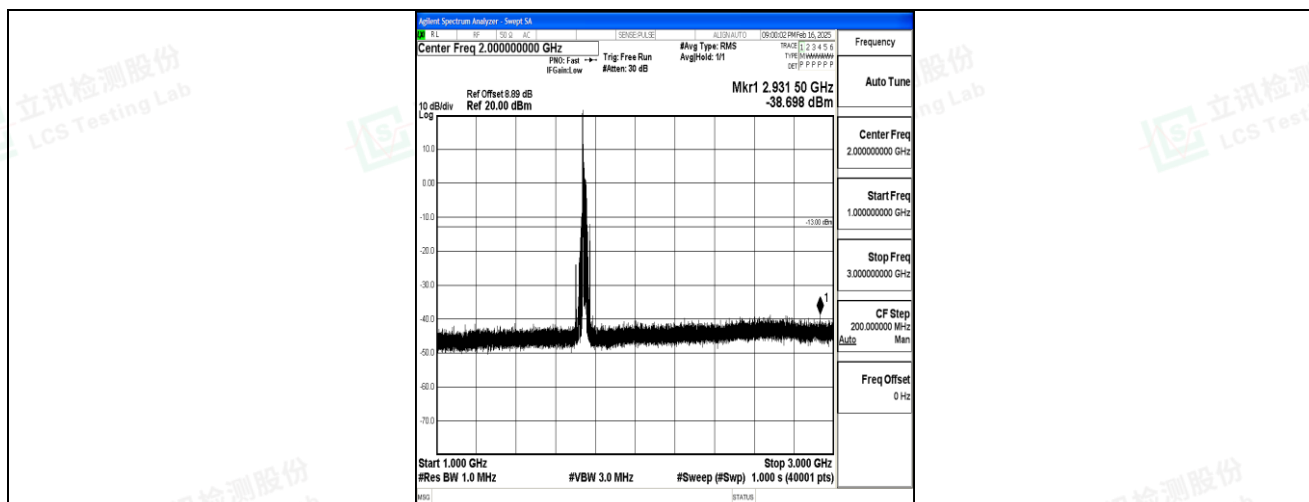
Band4_20MHz_16QAM_20300_1RB#0_1000~3000_1000~3000
