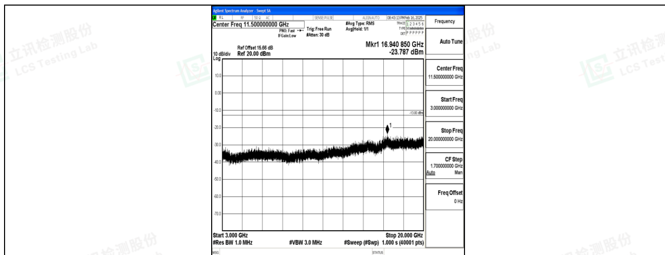
Band4_15MHz_16QAM_20175_1RB#0_3000~20000_3000~20000
