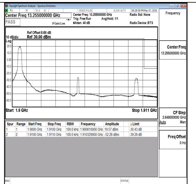
Band2-10MHz-16QAM-19150-1RB#0-PASS
