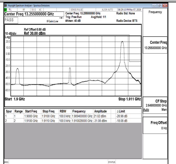
Band2-10MHz-QPSK-19150-1RB#49-PASS
