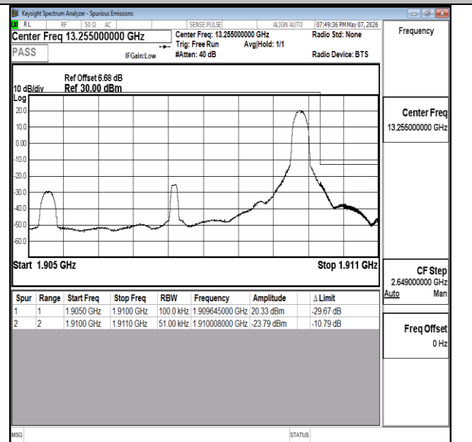
Band2-5MHz-QPSK-19175-1RB#24-PASS
