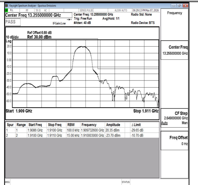
Band2-1.4MHz-QPSK-19193-1RB#5-PASS
