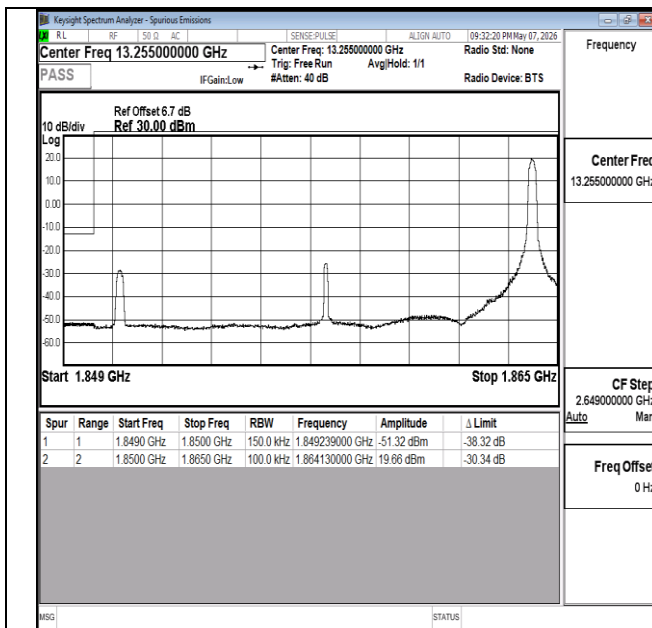
Band2-15MHz-16QAM-18675-1RB#74-PASS
