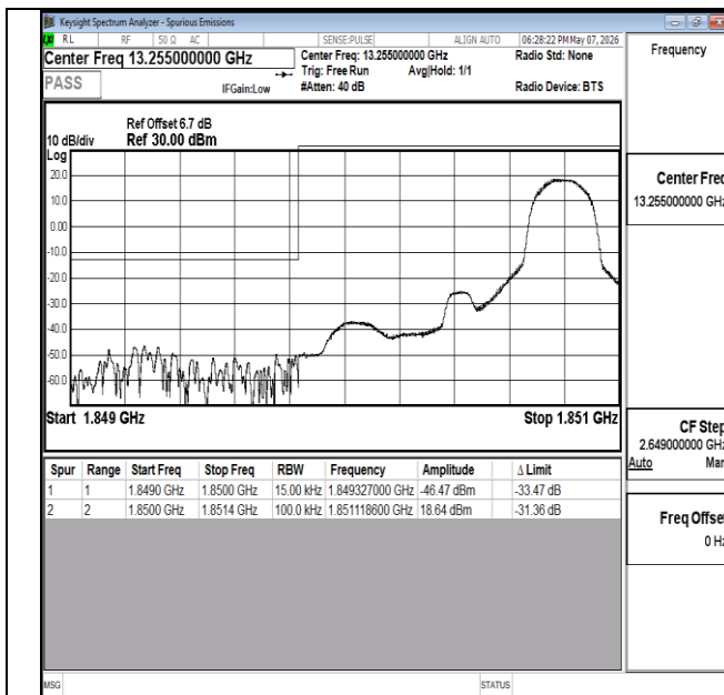
Band2-1.4MHz-16QAM-18607-1RB#5-PASS
