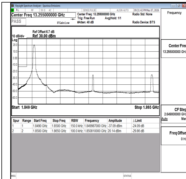
Band2-15MHz-QPSK-18675-1RB#0-PASS
