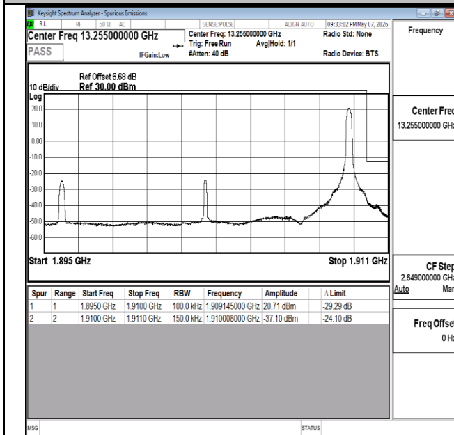
Band2-15MHz-QPSK-19125-1RB#74-PASS
