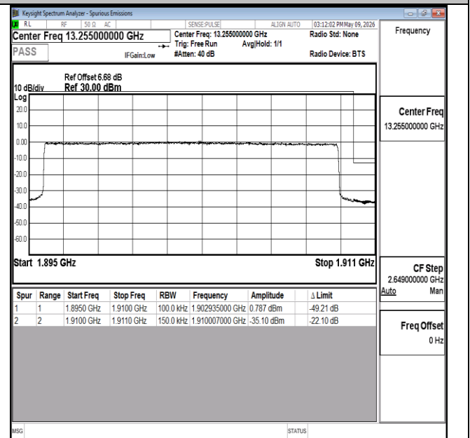
Band2-15MHz-QPSK-19125-75RB#0-PASS
