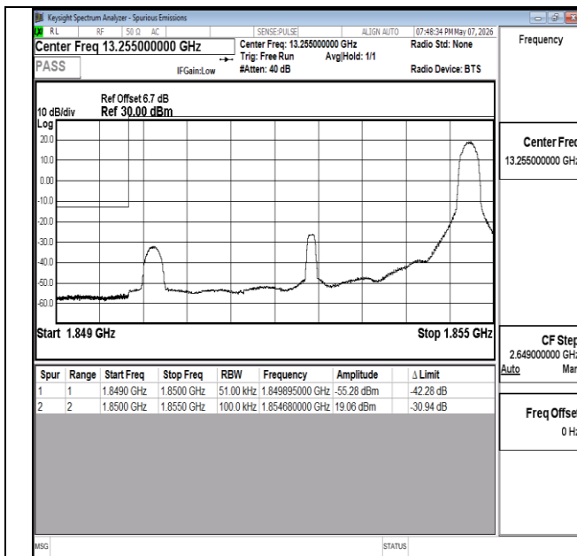
Band2-5MHz-16QAM-18625-1RB#24-PASS
