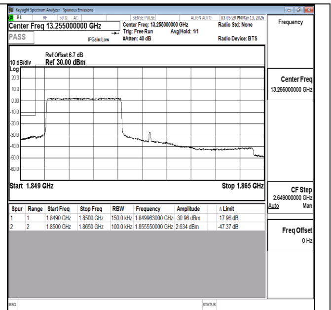
Band2-15MHz-16QAM-18675-27RB#0-PASS
