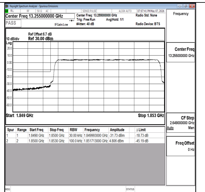
Band2-3MHz-16QAM-18615-15RB#0-PASS
