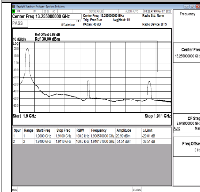
Band2-10MHz-QPSK-19150-1RB#0-PASS
