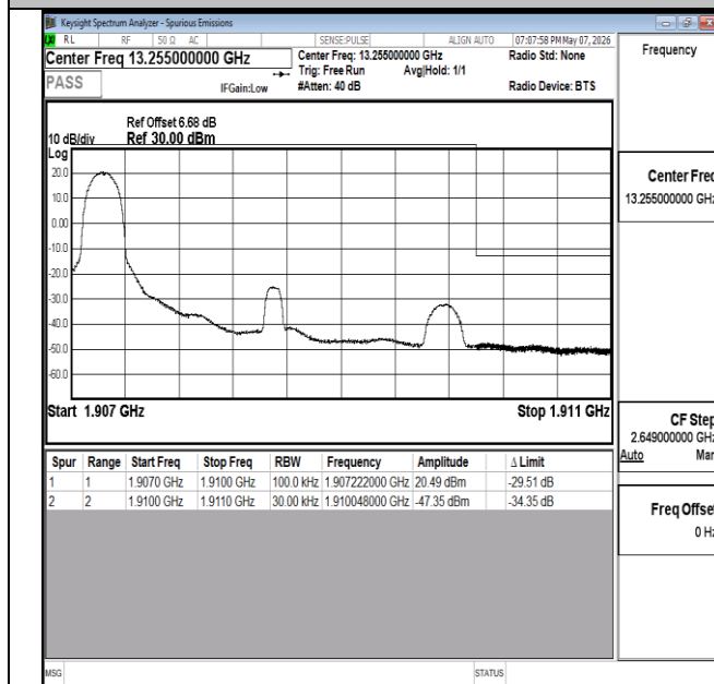
Band2-3MHz-QPSK-19185-1RB#0-PASS
