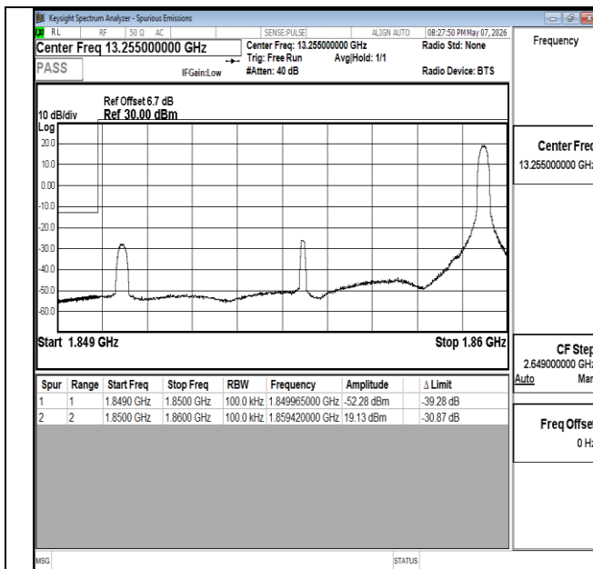
Band2-10MHz-16QAM-18650-1RB#49-PASS
