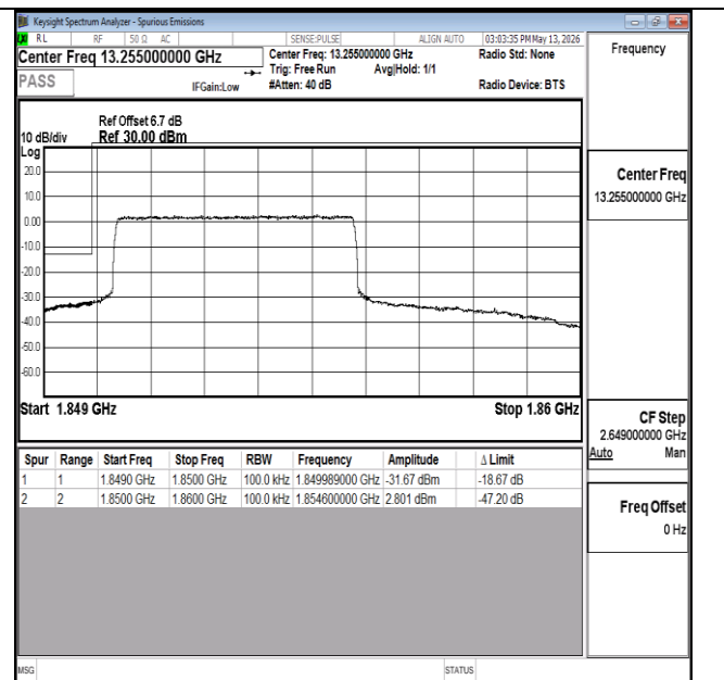
Band2-10MHz-16QAM-18650-27RB#0-PASS
