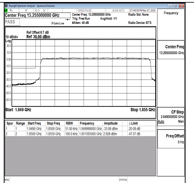
Band2-5MHz-16QAM-18625-25RB#0-PASS
