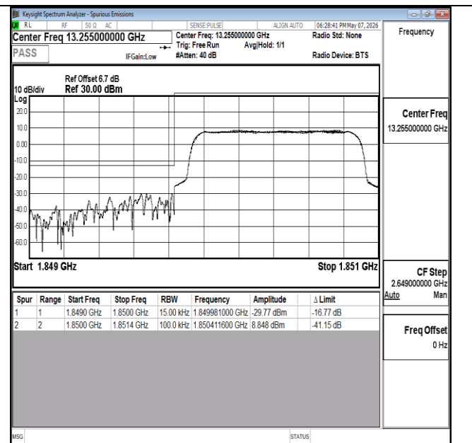
Band2-1.4MHz-16QAM-18607-6RB#0-PASS
