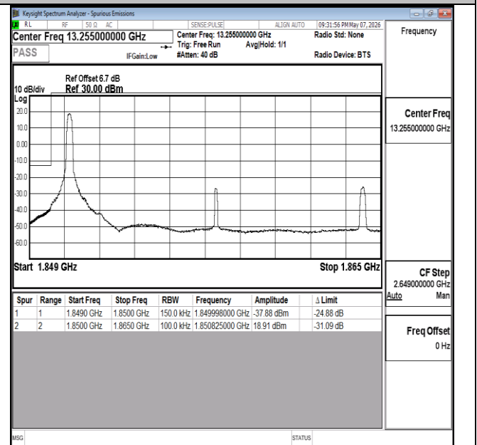
Band2-15MHz-16QAM-18675-1RB#0-PASS
