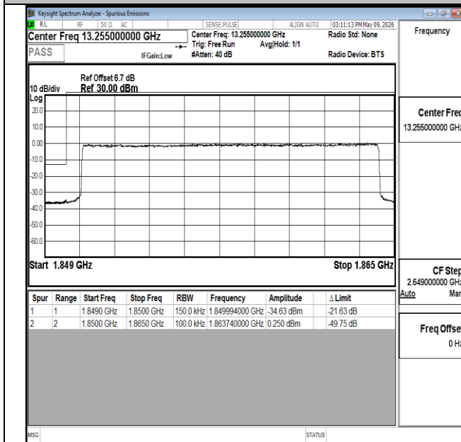
Band2-15MHz-QPSK-18675-75RB#0-PASS
