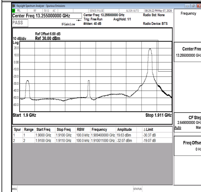
Band2-10MHz-16QAM-19150-1RB#49-PASS
