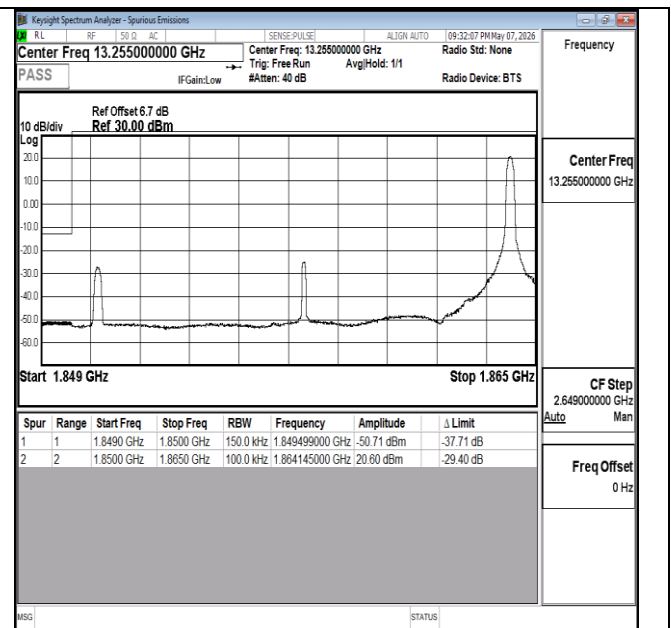
Band2-15MHz-QPSK-18675-1RB#74-PASS
