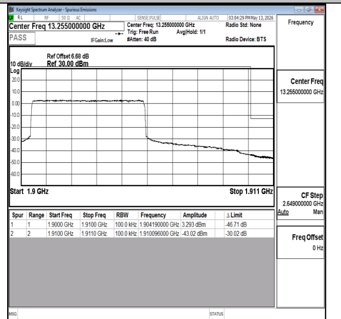
Band2-10MHz-16QAM-19150-27RB#0-PASS
