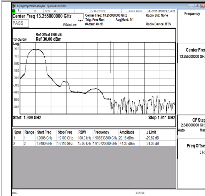
Band2-1.4MHz-QPSK-19193-1RB#0-PASS
