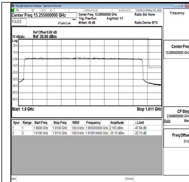
Band2-10MHz-QPSK-19150-50RB#0-PASS
