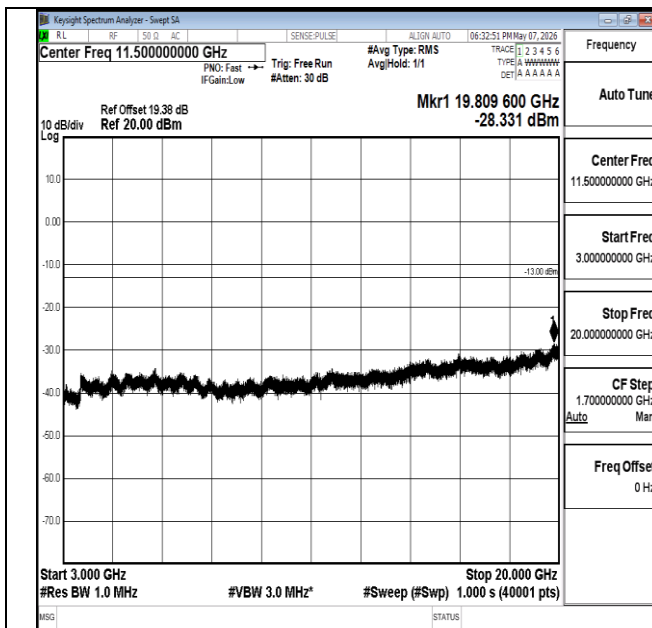
Band2-1.4MHz-16QAM-18607-1RB#5-3000~20000-PASS
