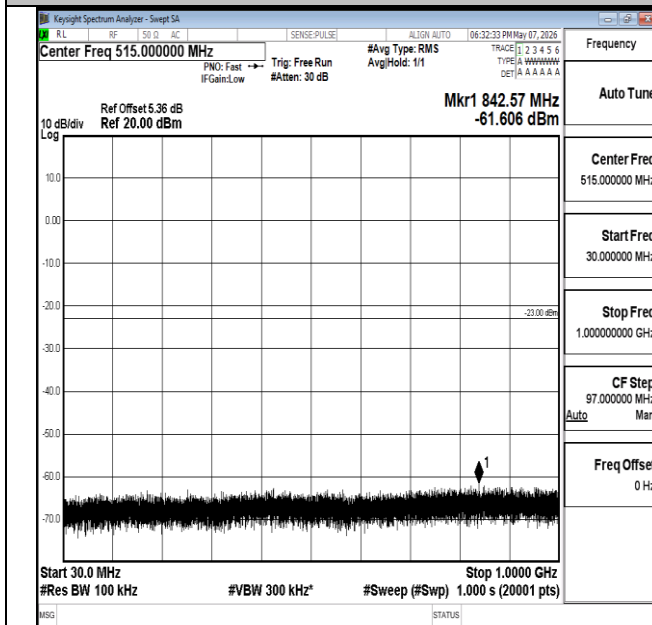
Band2-1.4MHz-16QAM-18607-1RB#5-30~1000-PASS
