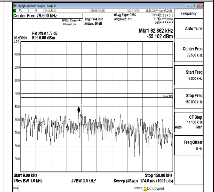
Band2-1.4MHz-16QAM-18900-6RB#0-0.009~0.15-PASS
