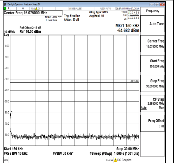
Band2-1.4MHz-16QAM-18900-1RB#5-0.15~30-PASS
