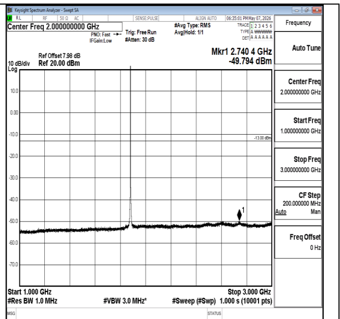
Band2-1.4MHz-QPSK-18900-1RB#0-1000~3000-PASS
