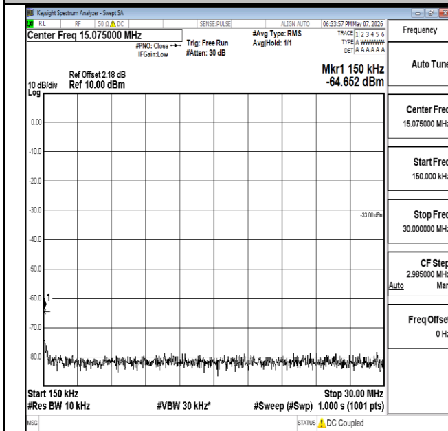
Band2-1.4MHz-16QAM-18607-6RB#0-0.15~30-PASS
