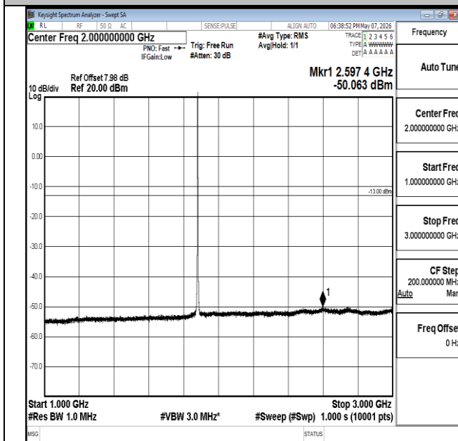
Band2-1.4MHz-16QAM-18900-6RB#0-1000~3000-PASS
