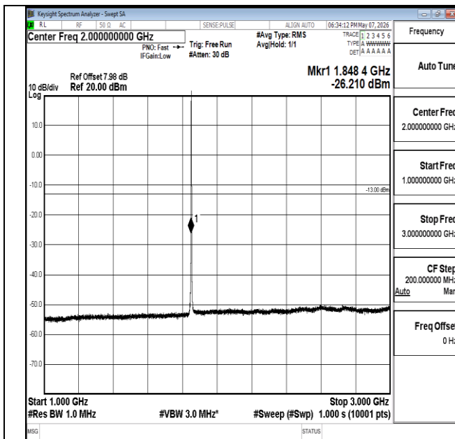
Band2-1.4MHz-16QAM-18607-6RB#0-1000~3000-PASS
