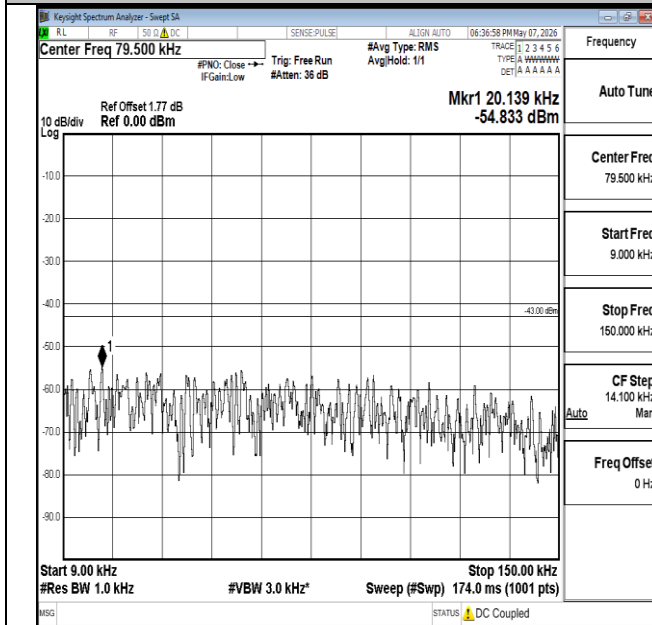
Band2-1.4MHz-16QAM-18900-1RB#5-0.009~0.15-PASS
