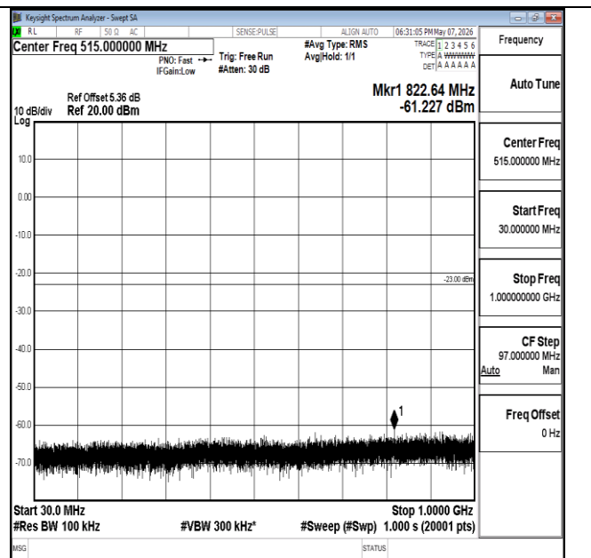
Band2-1.4MHz-16QAM-18607-1RB#0-30~1000-PASS
