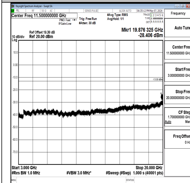
Band2-1.4MHz-QPSK-18900-1RB#0-3000~20000-PASS
