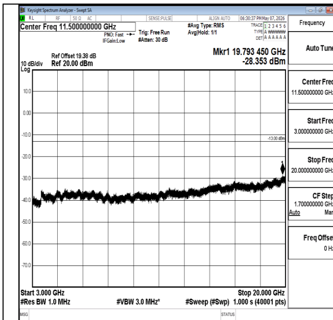
Band2-1.4MHz-QPSK-18607-1RB#0-3000~20000-PASS
