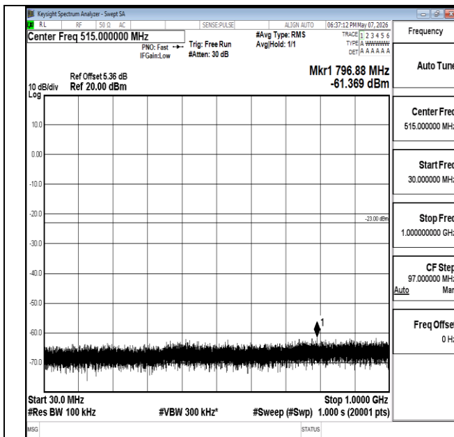
Band2-1.4MHz-16QAM-18900-1RB#5-30~1000-PASS
