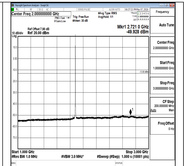
Band2-1.4MHz-16QAM-18900-1RB#5-1000~3000-PASS
