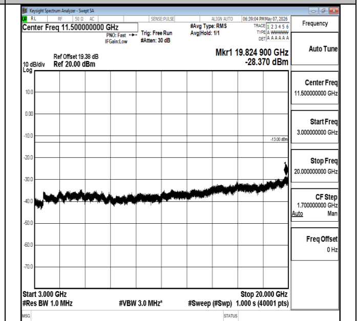
Band2-1.4MHz-16QAM-18900-6RB#0-3000~20000-PASS
