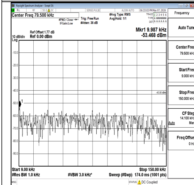
Band2-1.4MHz-QPSK-18607-6RB#0-0.009~0.15-PASS
