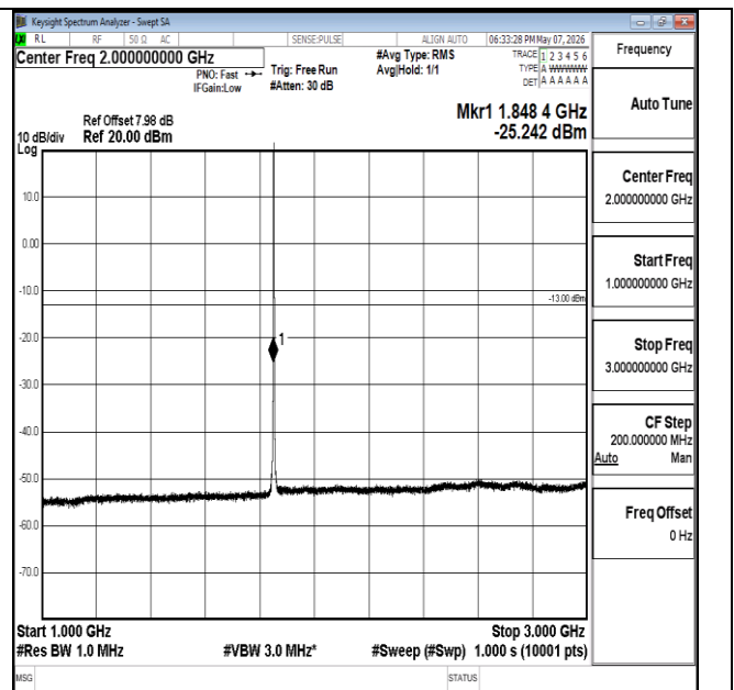
Band2-1.4MHz-QPSK-18607-6RB#0-1000~3000-PASS
