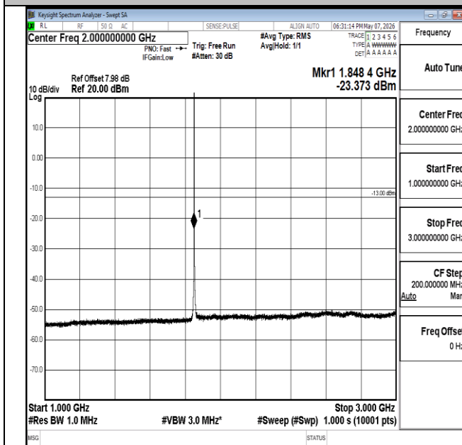
Band2-1.4MHz-16QAM-18607-1RB#0-1000~3000-PASS
