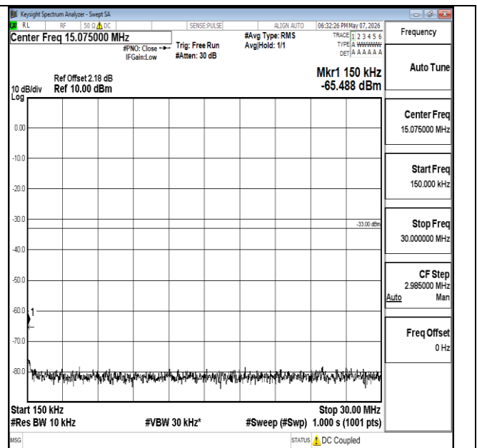
Band2-1.4MHz-16QAM-18607-1RB#5-0.15~30-PASS
