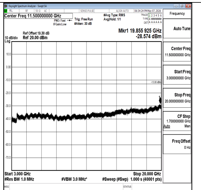
Band2-1.4MHz-16QAM-18607-6RB#0-3000~20000-PASS
