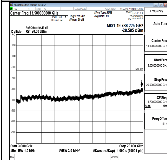
Band2-1.4MHz-QPSK-18607-6RB#0-3000~20000-PASS
