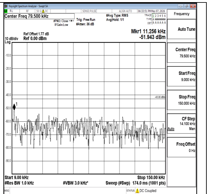
Band2-1.4MHz-16QAM-18607-6RB#0-0.009~0.15-PASS
