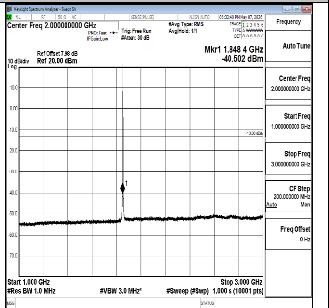
Band2-1.4MHz-16QAM-18607-1RB#5-1000~3000-PASS
