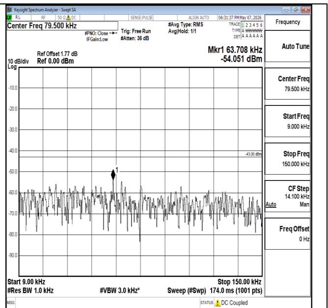
Band2-1.4MHz-QPSK-18607-1RB#5-0.009~0.15-PASS
