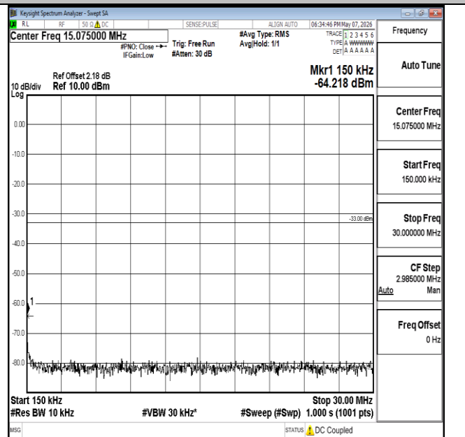
Band2-1.4MHz-QPSK-18900-1RB#0-0.15~30-PASS
