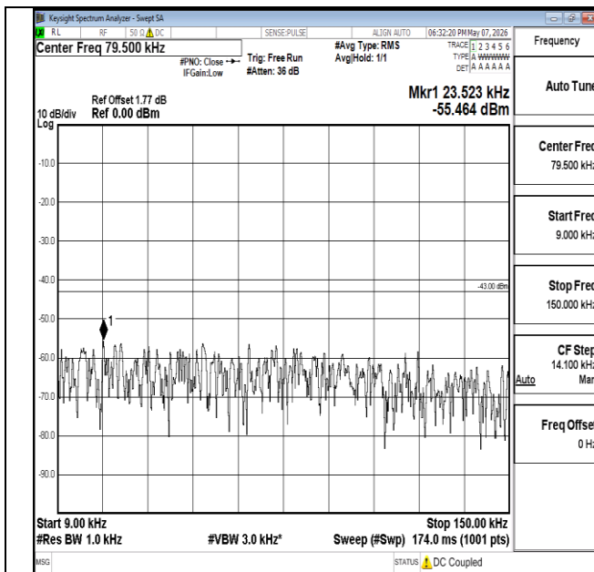
Band2-1.4MHz-16QAM-18607-1RB#5-0.009~0.15-PASS
