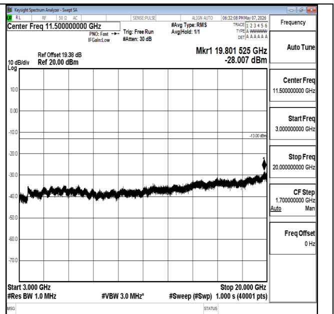
Band2-1.4MHz-QPSK-18607-1RB#5-3000~20000-PASS
