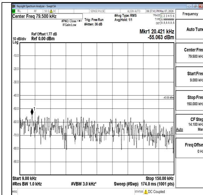
Band2-1.4MHz-QPSK-18900-6RB#0-0.009~0.15-PASS
