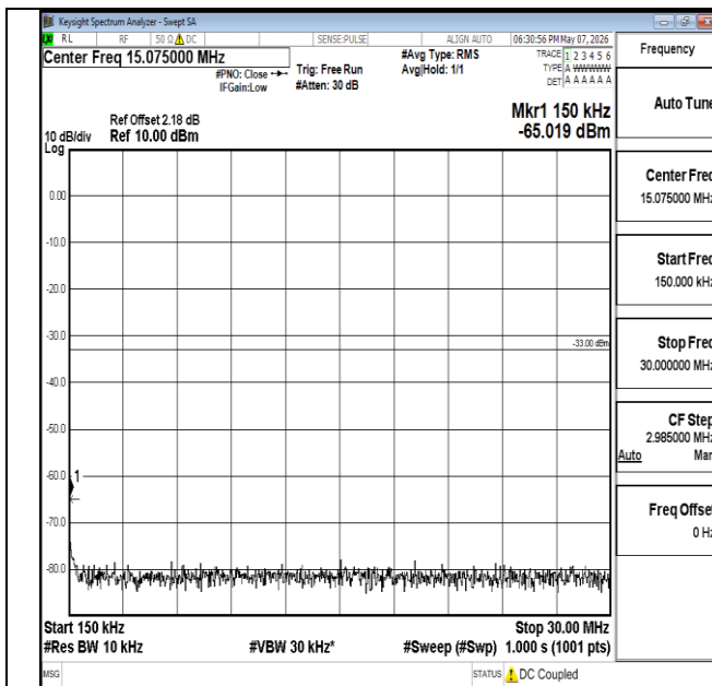
Band2-1.4MHz-16QAM-18607-1RB#0-0.15~30-PASS
