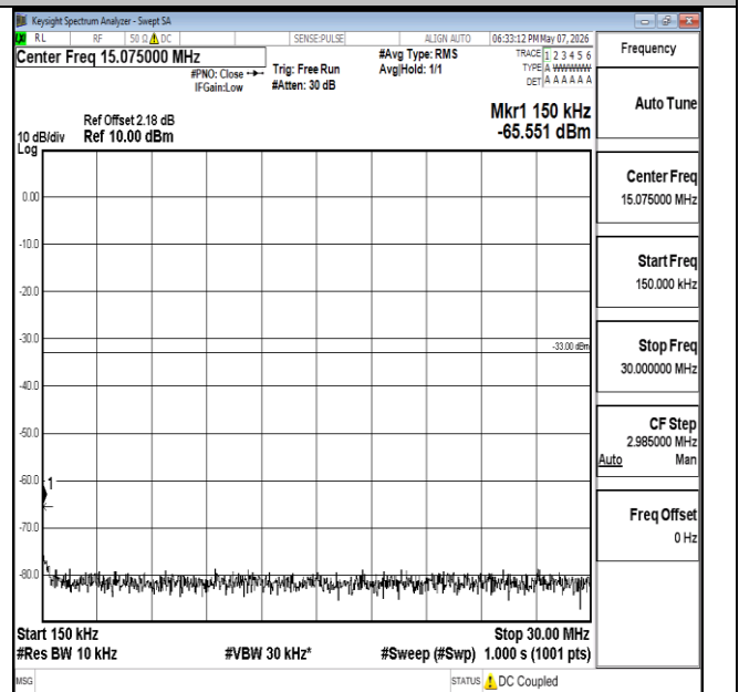
Band2-1.4MHz-QPSK-18607-6RB#0-0.15~30-PASS
