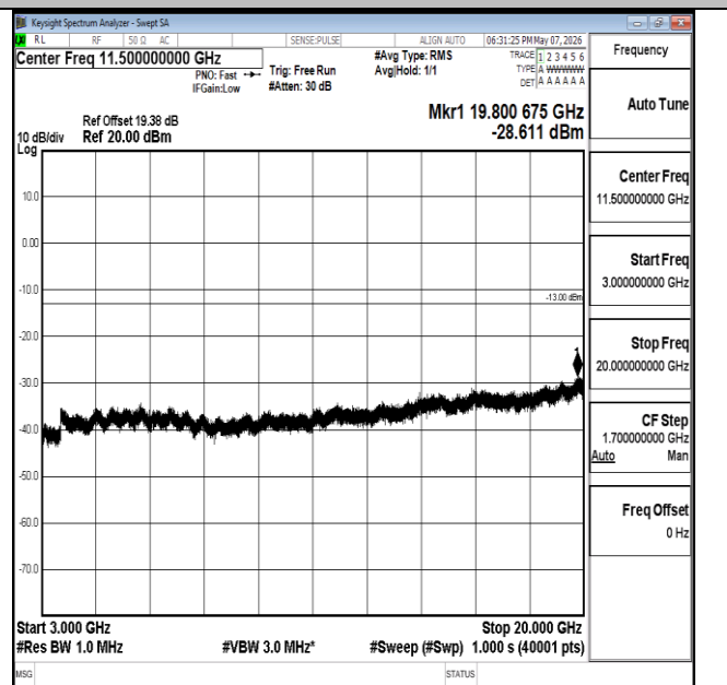
Band2-1.4MHz-16QAM-18607-1RB#0-3000~20000-PASS
