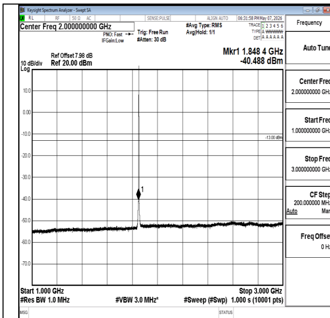
Band2-1.4MHz-QPSK-18607-1RB#5-1000~3000-PASS
