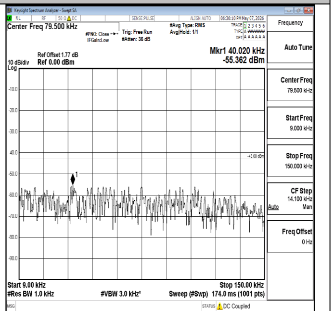
Band2-1.4MHz-QPSK-18900-1RB#5-0.009~0.15-PASS
