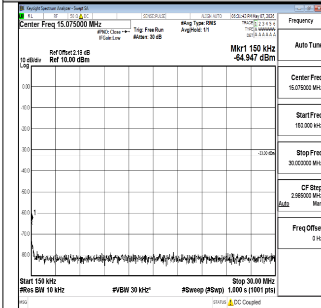
Band2-1.4MHz-QPSK-18607-1RB#5-0.15~30-PASS
