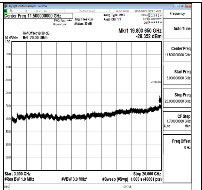
Band2-1.4MHz-16QAM-18900-1RB#0-3000~20000-PASS
