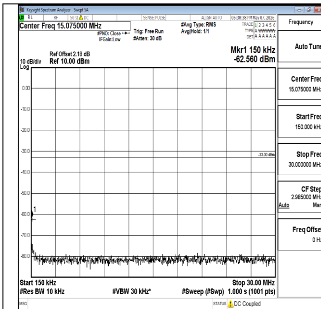
Band2-1.4MHz-16QAM-18900-6RB#0-0.15~30-PASS
