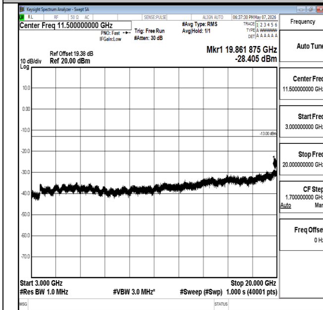
Band2-1.4MHz-16QAM-18900-1RB#5-3000~20000-PASS
