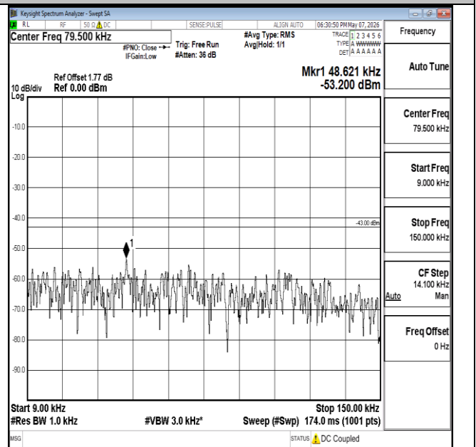
Band2-1.4MHz-16QAM-18607-1RB#0-0.009~0.15-PASS
