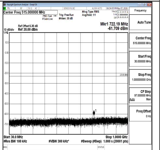
Band2-1.4MHz-16QAM-18607-6RB#0-30~1000-PASS
