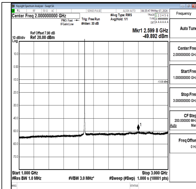
Band2-1.4MHz-16QAM-18900-1RB#0-1000~3000-PASS
