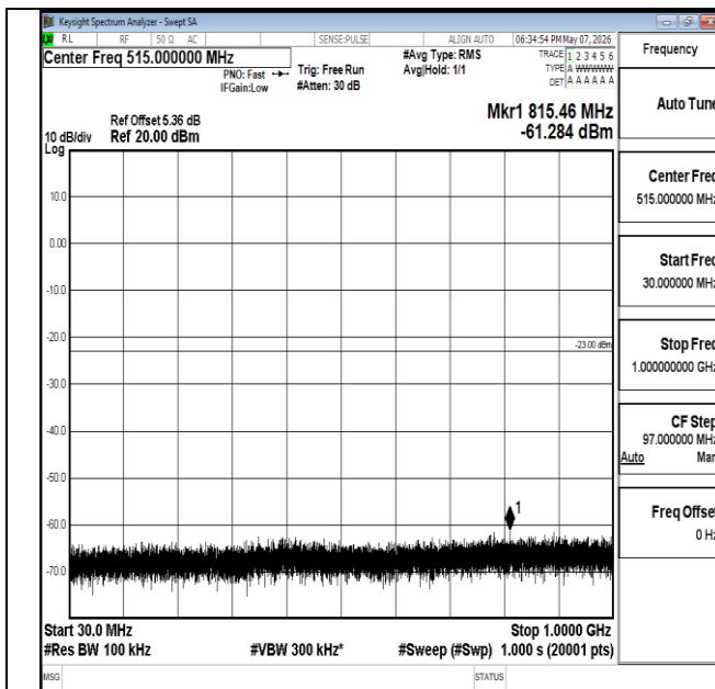
Band2-1.4MHz-QPSK-18900-1RB#0-30~1000-PASS
