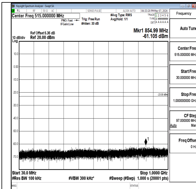
Band2-1.4MHz-QPSK-18607-6RB#0-30~1000-PASS
