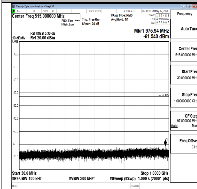
Band2-1.4MHz-QPSK-18900-6RB#0-30~1000-PASS
