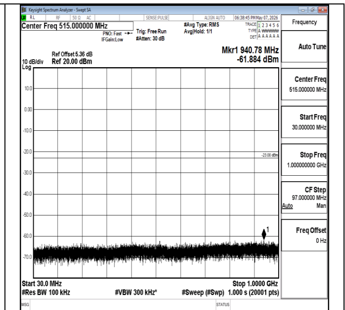
Band2-1.4MHz-16QAM-18900-6RB#0-30~1000-PASS
