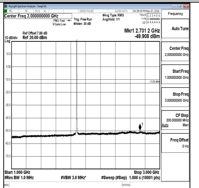
Band2-1.4MHz-QPSK-18900-6RB#0-1000~3000-PASS
