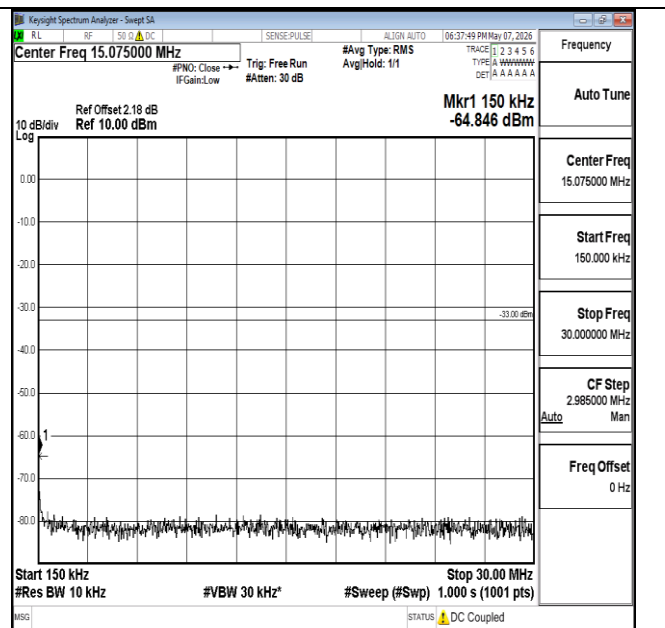
Band2-1.4MHz-QPSK-18900-6RB#0-0.15~30-PASS
