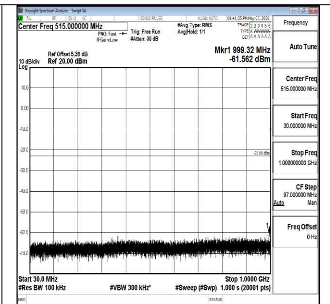
Band2-15MHz-QPSK-19125-1RB#0-30~1000-PASS
