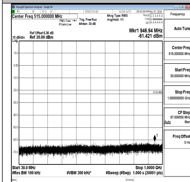
Band2-15MHz-QPSK-19125-1RB#74-30~1000-PASS
