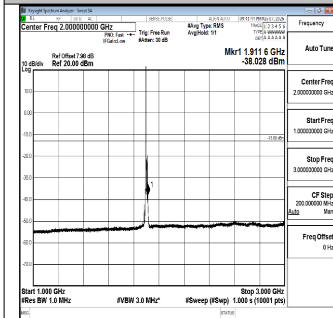
Band2-15MHz-QPSK-19125-1RB#0-1000~3000-PASS
