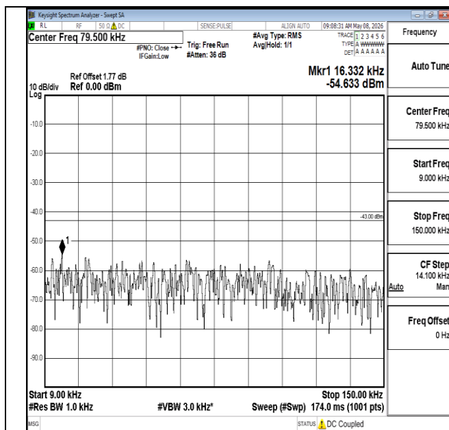
Band2-20MHz-16QAM-18900-1RB#0-0.009~0.15-PASS
