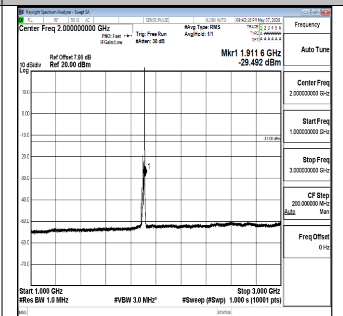
Band2-15MHz-QPSK-19125-1RB#74-1000~3000-PASS
