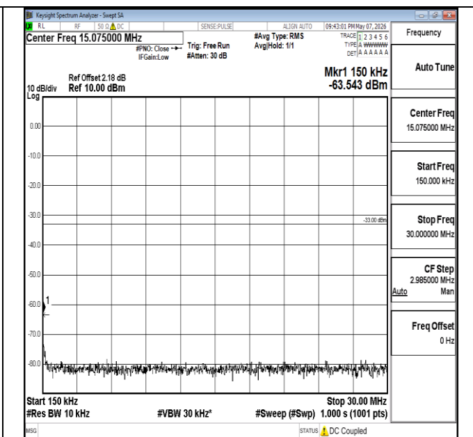
Band2-15MHz-QPSK-19125-1RB#74-0.15~30-PASS
