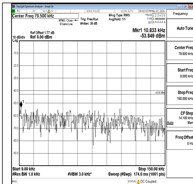
Band2-15MHz-QPSK-19125-1RB#74-0.009~0.15-PASS
