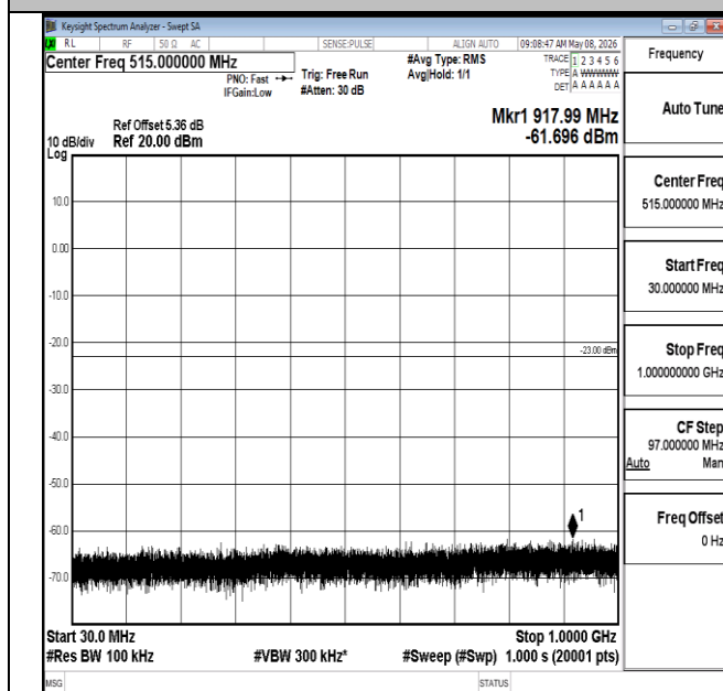
Band2-20MHz-16QAM-18900-1RB#0-30~1000-PASS
