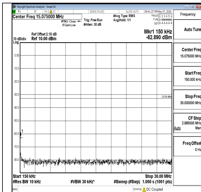
Band2-15MHz-QPSK-19125-1RB#0-0.15~30-PASS
