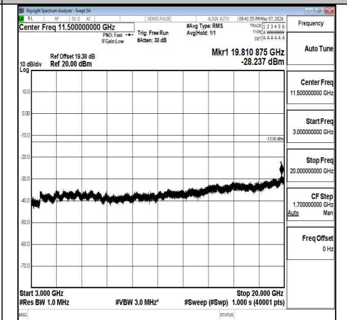
Band2-15MHz-QPSK-19125-1RB#0-3000~20000-PASS
