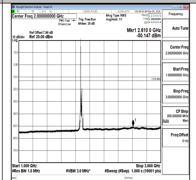
Band2-20MHz-16QAM-18900-1RB#0-1000~3000-PASS
