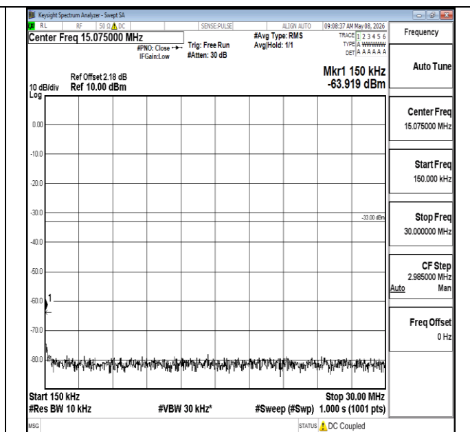
Band2-20MHz-16QAM-18900-1RB#0-0.15~30-PASS
