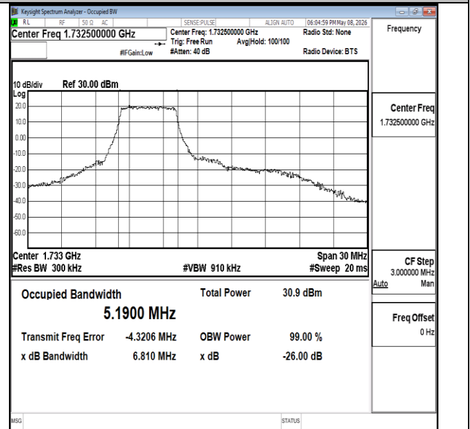
Band4-15MHz-16QAM-20175-27RB#0-PASS
