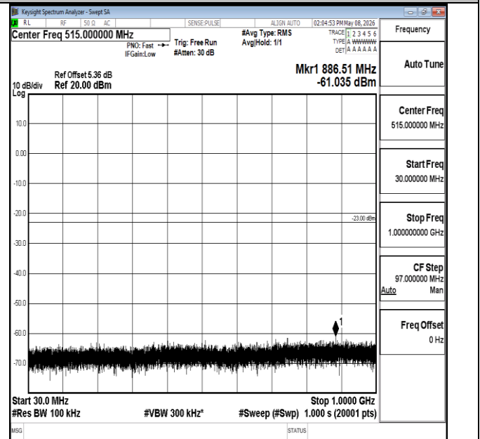
Band4-1.4MHz-QPSK-19957-1RB#5-30~1000-PASS
