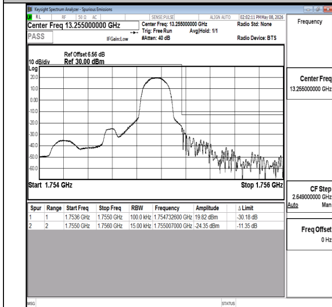
Band4-1.4MHz-16QAM-20393-1RB#5-PASS
