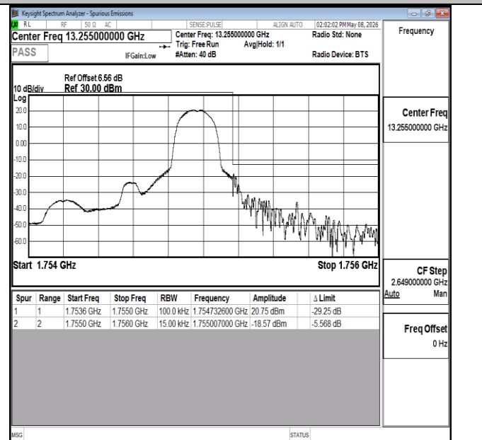
Band4-1.4MHz-QPSK-20393-1RB#5-PASS
