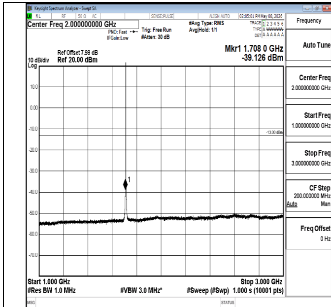
Band4-1.4MHz-QPSK-19957-1RB#5-1000~3000-PASS
