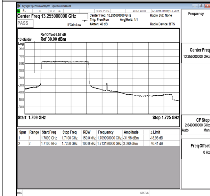
Band4-15MHz-16QAM-20025-27RB#0-PASS
