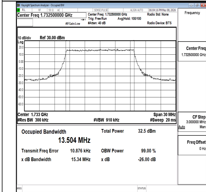
Band4-15MHz-QPSK-20175-75RB#0-PASS
