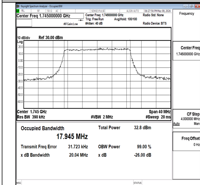
Band4-20MHz-QPSK-20300-100RB#0-PASS
