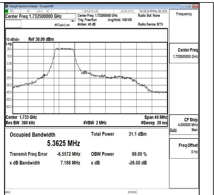
Band4-20MHz-16QAM-20175-27RB#0-PASS
