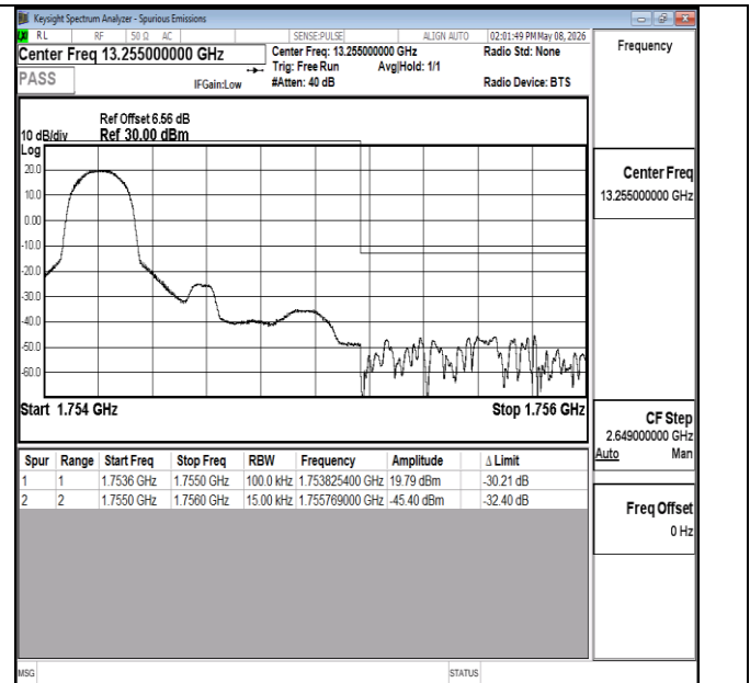
Band4-1.4MHz-16QAM-20393-1RB#0-PASS
