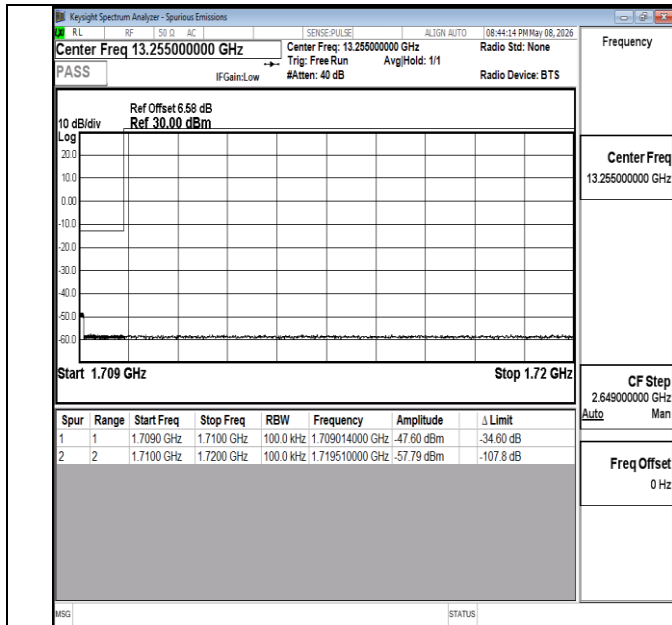
Band4-10MHz-QPSK-20000-1RB#50-PASS
