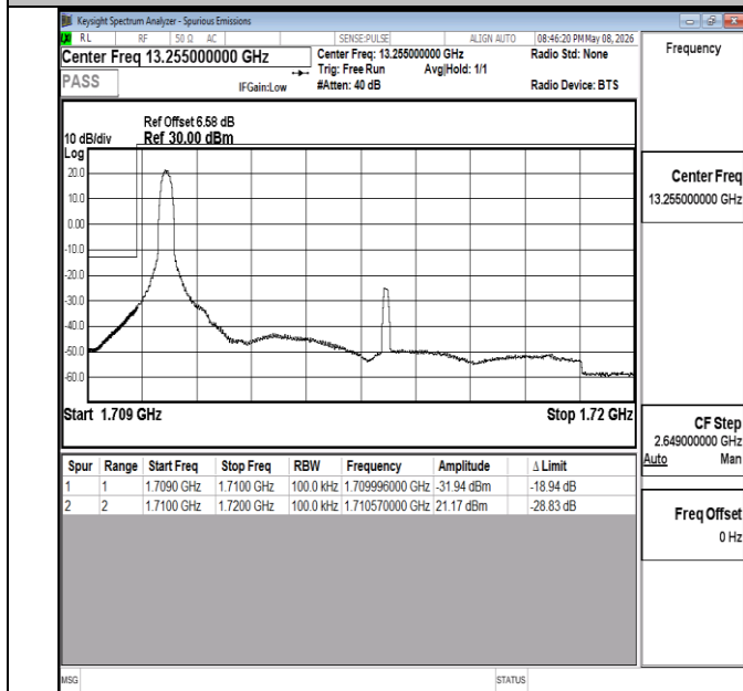
Band4-10MHz-16QAM-20000-1RB#50-PASS
