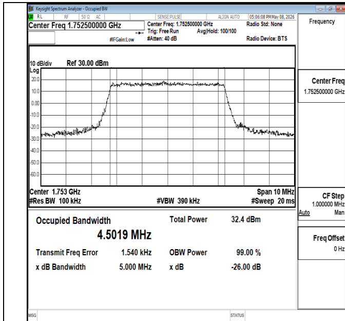
Band4-5MHz-QPSK-20375-25RB#0-PASS
