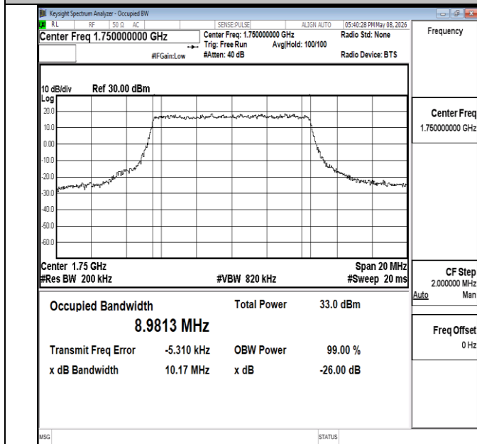
Band4-10MHz-QPSK-20350-50RB#0-PASS
