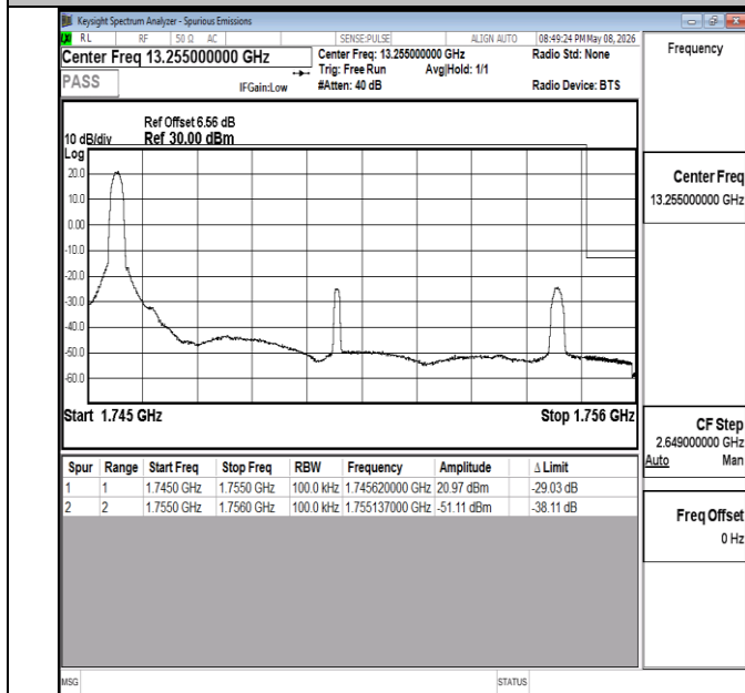
Band4-10MHz-16QAM-20350-1RB#50-PASS
