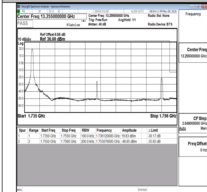
Band4-20MHz-16QAM-20300-1RB#100-PASS
