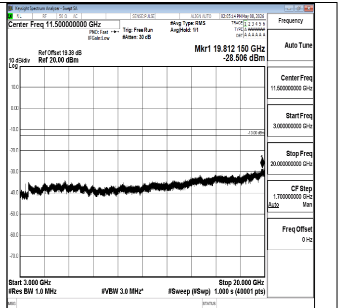
Band4-1.4MHz-QPSK-19957-1RB#5-3000~20000-PASS
