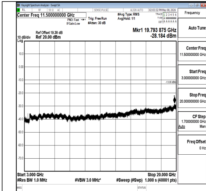
Band4-1.4MHz-QPSK-19957-1RB#0-3000~20000-PASS
