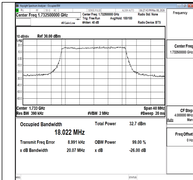
Band4-20MHz-QPSK-20175-100RB#0-PASS
