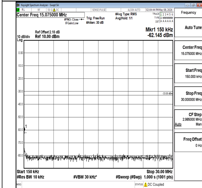
Band4-1.4MHz-QPSK-19957-1RB#5-0.15~30-PASS
