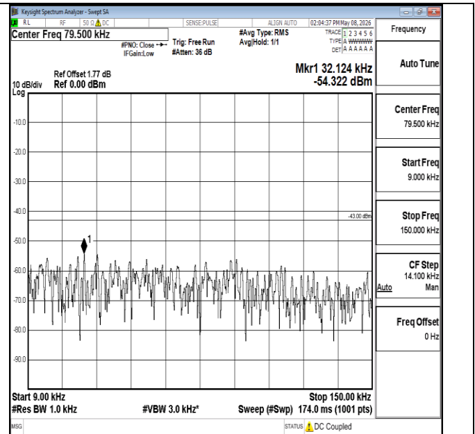
Band4-1.4MHz-QPSK-19957-1RB#5-0.009~0.15-PASS
