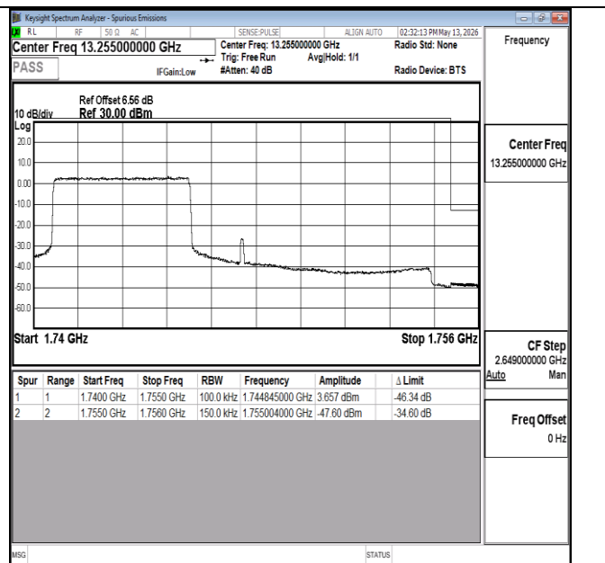
Band4-15MHz-16QAM-20325-27RB#0-PASS
