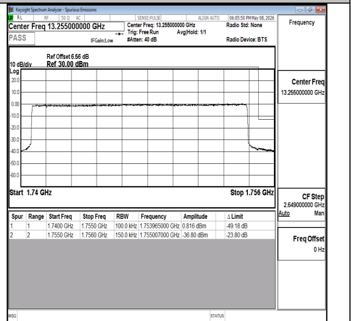
Band4-15MHz-QPSK-20325-75RB#0-PASS
