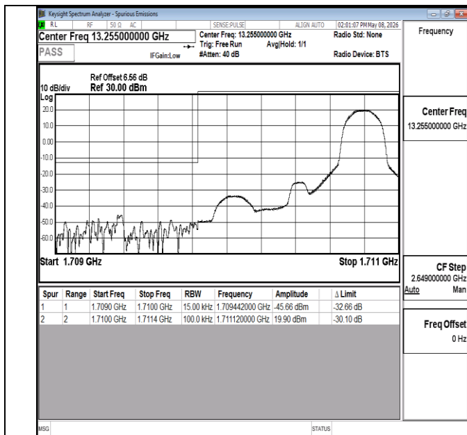
Band4-1.4MHz-16QAM-19957-1RB#5-PASS
