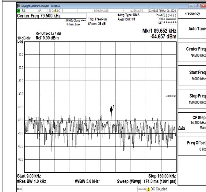
Band4-1.4MHz-QPSK-19957-6RB#0-0.009~0.15-PASS
