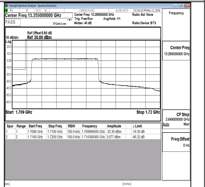
Band4-10MHz-16QAM-20000-27RB#0-PASS
