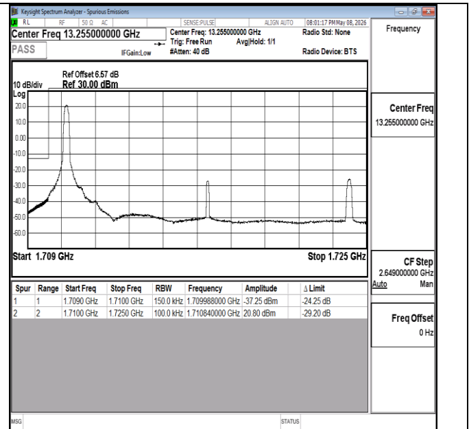
Band4-15MHz-16QAM-20025-1RB#75-PASS
