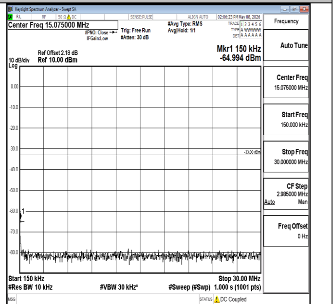
Band4-1.4MHz-QPSK-19957-6RB#0-0.15~30-PASS
