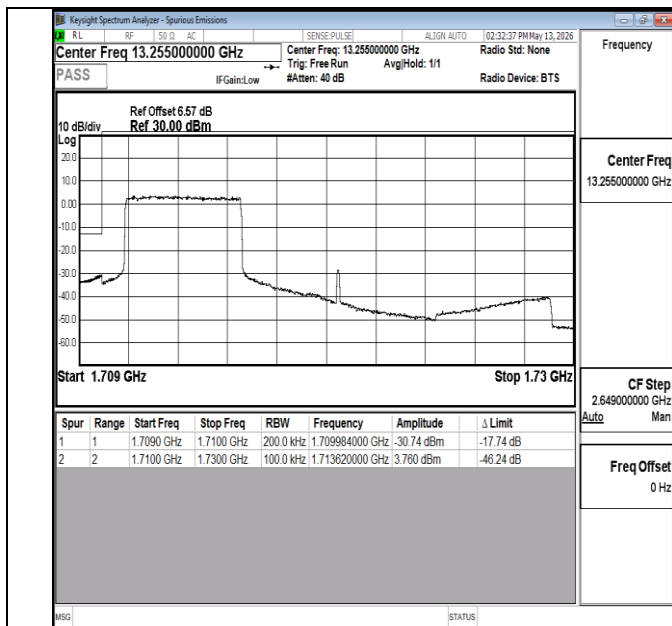
Band4-20MHz-16QAM-20050-27RB#0-PASS
