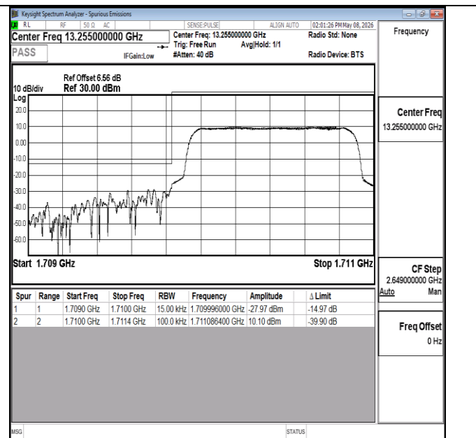
Band4-1.4MHz-16QAM-19957-6RB#0-PASS
