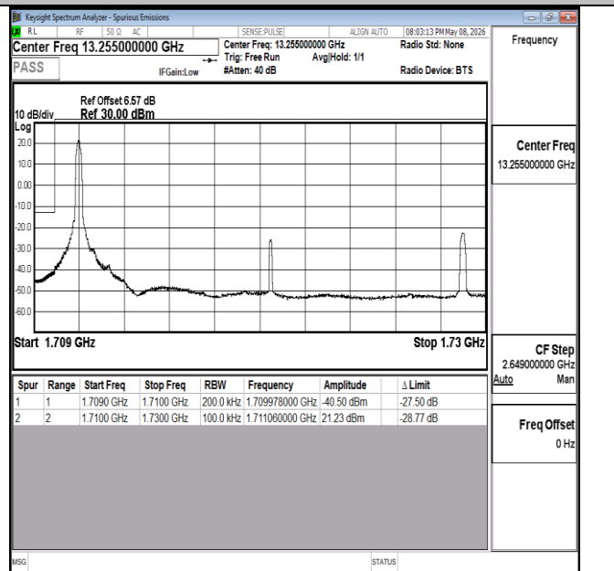
Band4-20MHz-16QAM-20050-1RB#100-PASS
