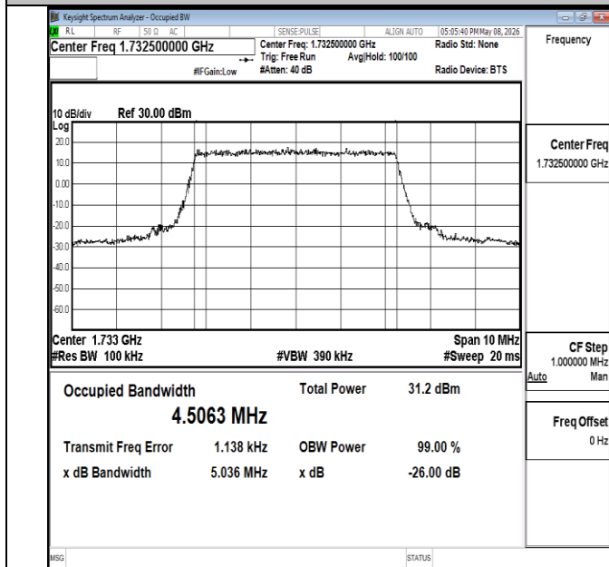
Band4-5MHz-QPSK-20175-25RB#0-PASS
