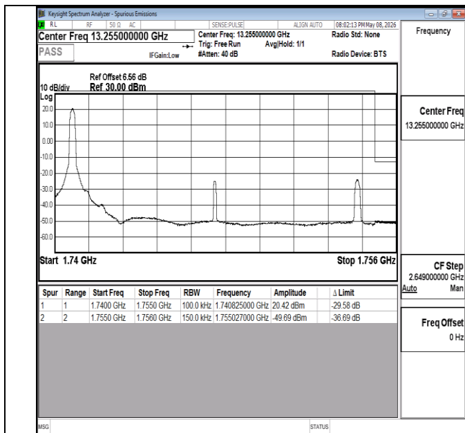
Band4-15MHz-16QAM-20325-1RB#75-PASS
