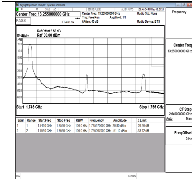
Band4-10MHz-QPSK-20350-1RB#50-PASS
