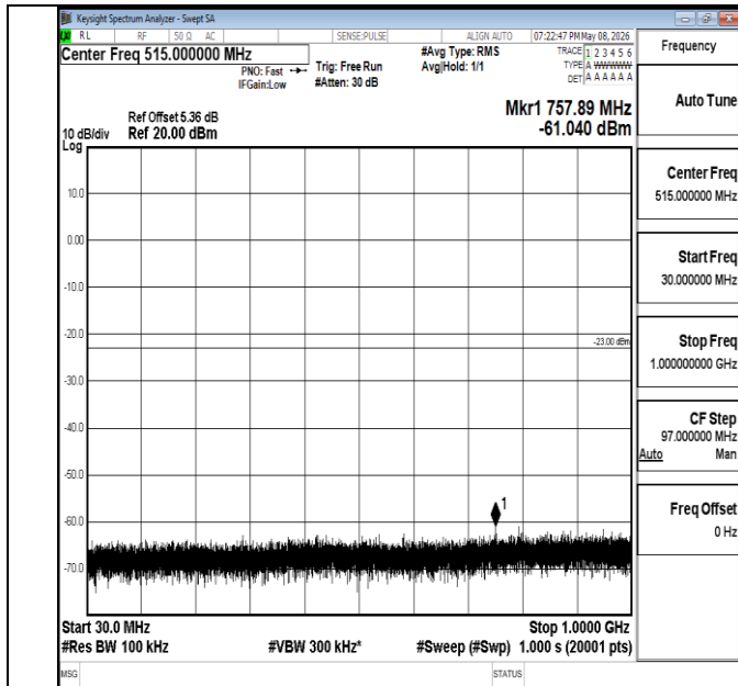
Band4-20MHz-QPSK-20300-1RB#0-30~1000-PASS
