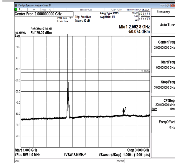
Band4-15MHz-16QAM-20175-1RB#0-1000~3000-PASS
