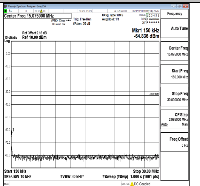
Band4-20MHz-QPSK-20050-1RB#0-0.15~30-PASS
