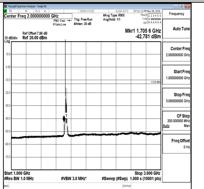
Band4-20MHz-QPSK-20175-1RB#0-1000~3000-PASS
