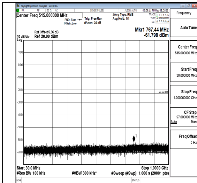
Band4-15MHz-QPSK-20175-1RB#0-30~1000-PASS
