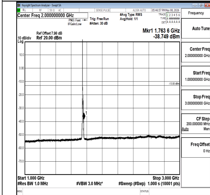
Band4-10MHz-16QAM-20350-1RB#0-1000~3000-PASS
