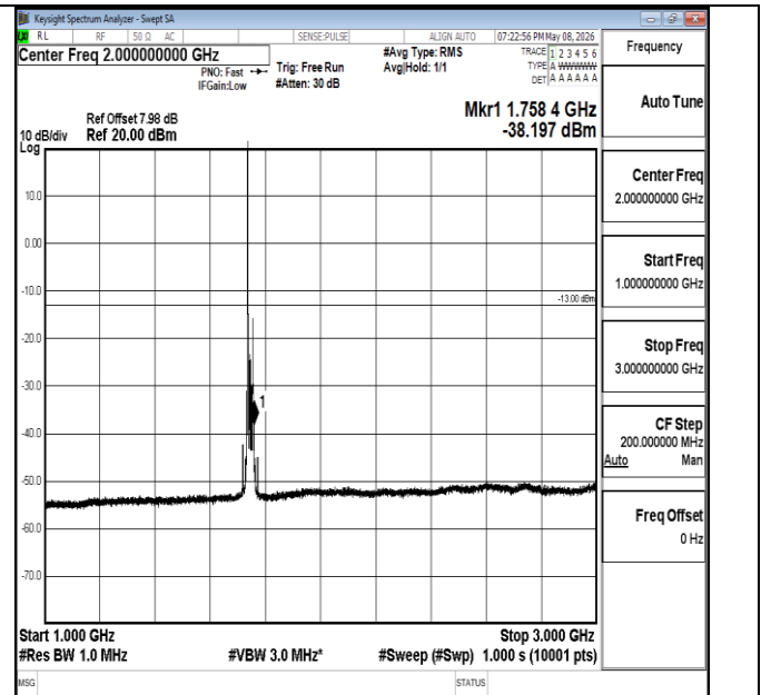
Band4-20MHz-QPSK-20300-1RB#0-1000~3000-PASS
