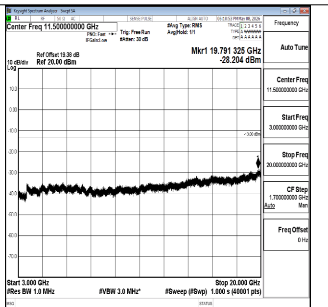
Band4-15MHz-16QAM-20325-1RB#0-3000~20000-PASS
