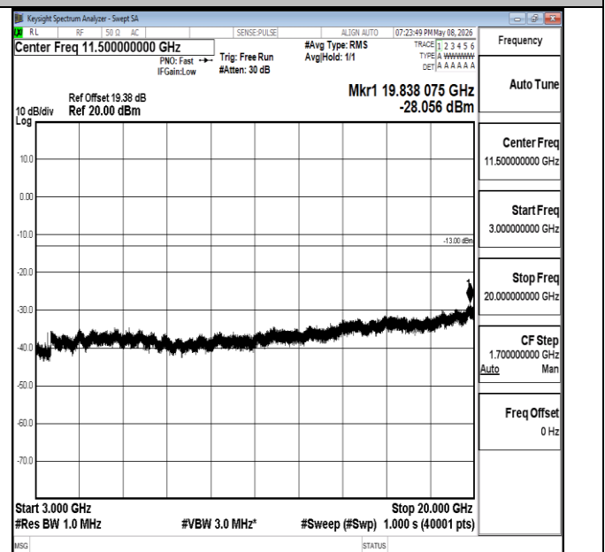
Band4-20MHz-16QAM-20300-1RB#0-3000~20000-PASS
