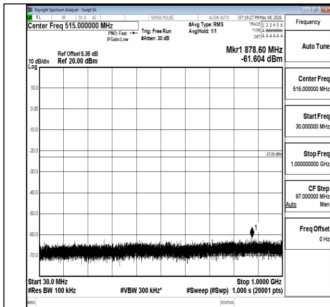
Band4-20MHz-QPSK-20050-1RB#0-30~1000-PASS
