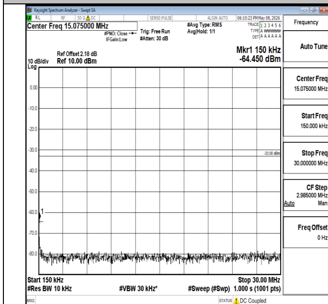
Band4-15MHz-16QAM-20325-1RB#0-0.15~30-PASS
