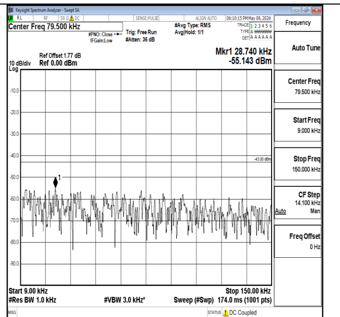
Band4-15MHz-16QAM-20325-1RB#0-0.009~0.15-PASS
