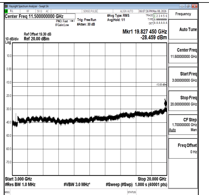
Band4-15MHz-16QAM-20025-1RB#0-3000~20000-PASS
