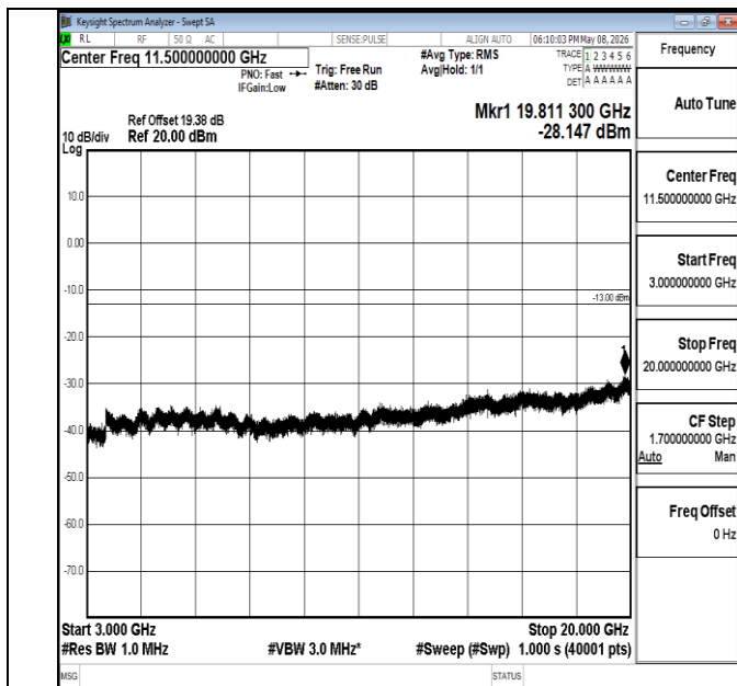
Band4-15MHz-QPSK-20325-1RB#0-3000~20000-PASS
