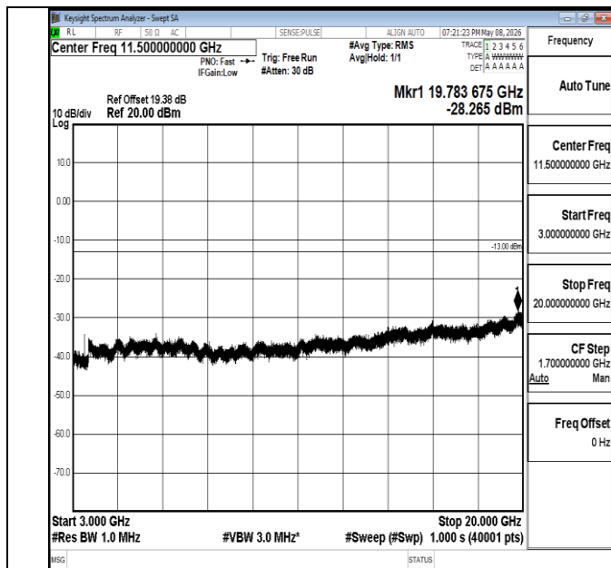
Band4-20MHz-QPSK-20175-1RB#0-3000~20000-PASS
