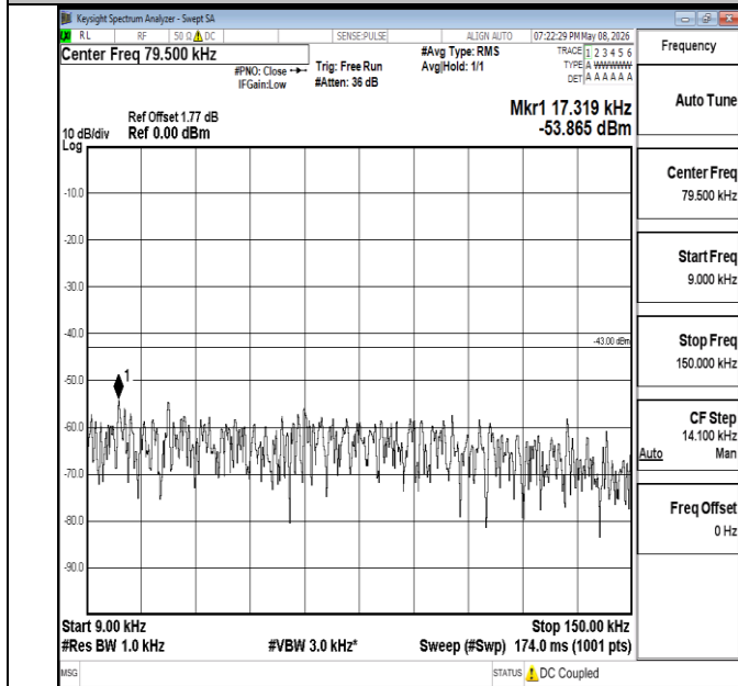
Band4-20MHz-QPSK-20300-1RB#0-0.009~0.15-PASS
