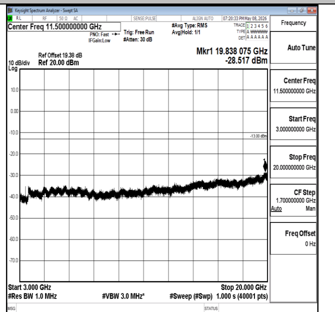
Band4-20MHz-16QAM-20050-1RB#0-3000~20000-PASS
