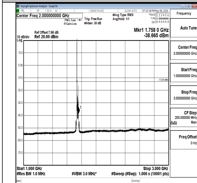
Band4-20MHz-16QAM-20300-1RB#0-1000~3000-PASS
