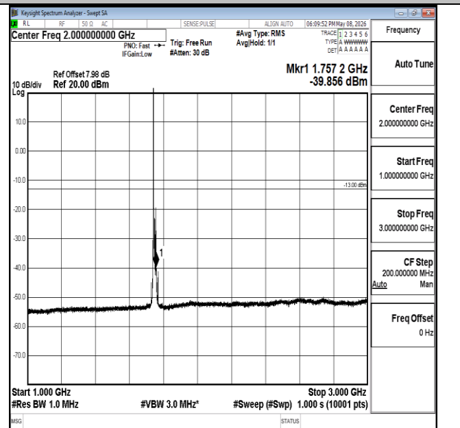
Band4-15MHz-QPSK-20325-1RB#0-1000~3000-PASS
