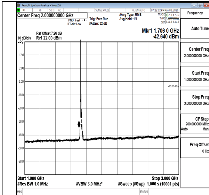
Band4-20MHz-16QAM-20175-1RB#0-1000~3000-PASS
