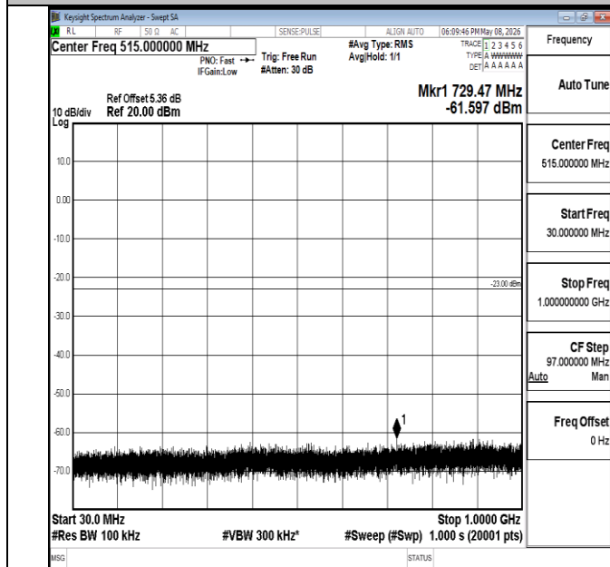
Band4-15MHz-QPSK-20325-1RB#0-30~1000-PASS
