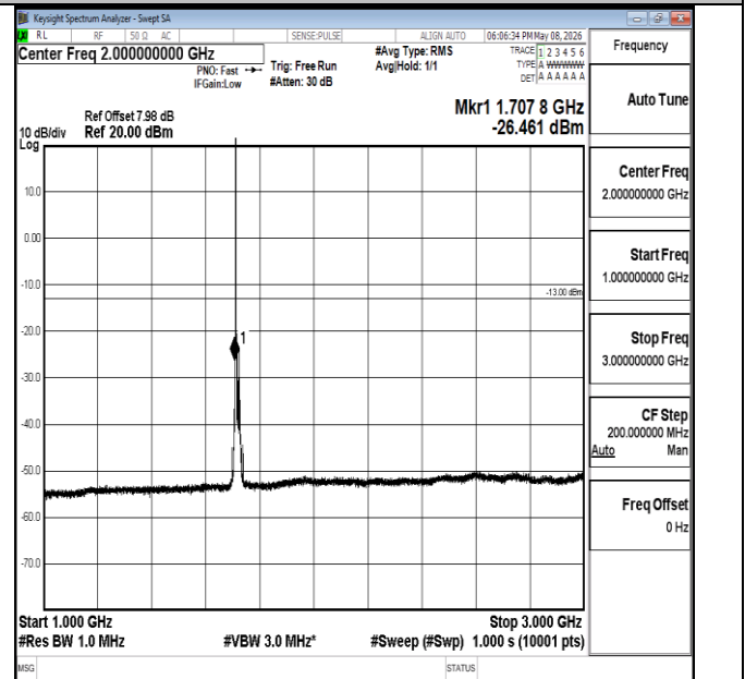
Band4-15MHz-QPSK-20025-1RB#0-1000~3000-PASS
