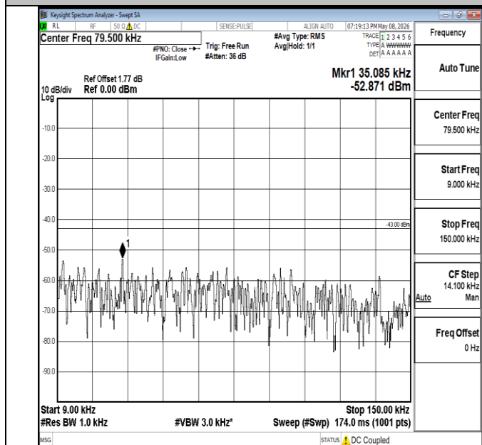
Band4-20MHz-QPSK-20050-1RB#0-0.009~0.15-PASS
