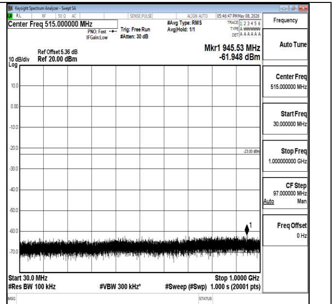
Band4-10MHz-16QAM-20350-1RB#0-30~1000-PASS
