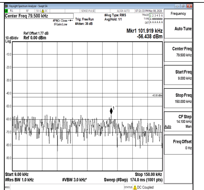
Band4-20MHz-16QAM-20175-1RB#0-0.009~0.15-PASS
