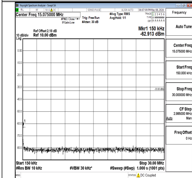
Band4-15MHz-16QAM-20025-1RB#0-0.15~30-PASS
