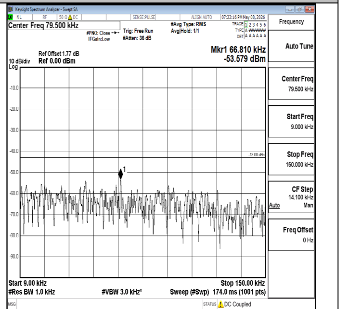
Band4-20MHz-16QAM-20300-1RB#0-0.009~0.15-PASS
