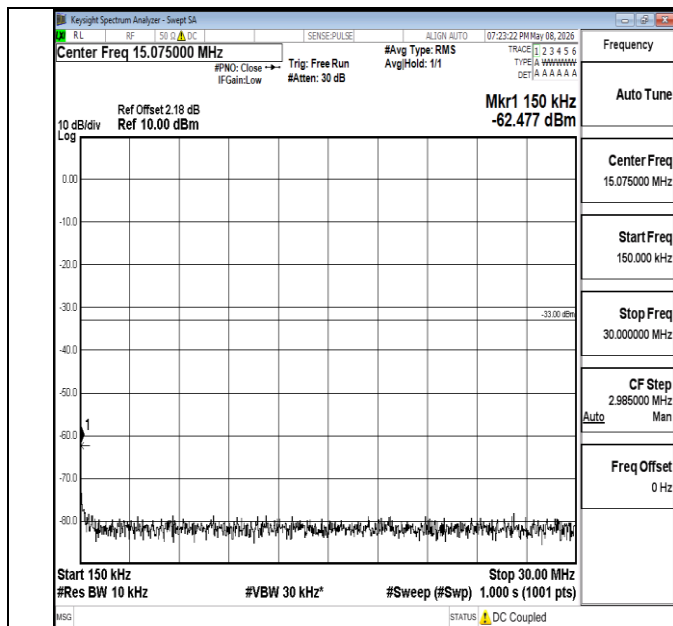
Band4-20MHz-16QAM-20300-1RB#0-0.15~30-PASS
