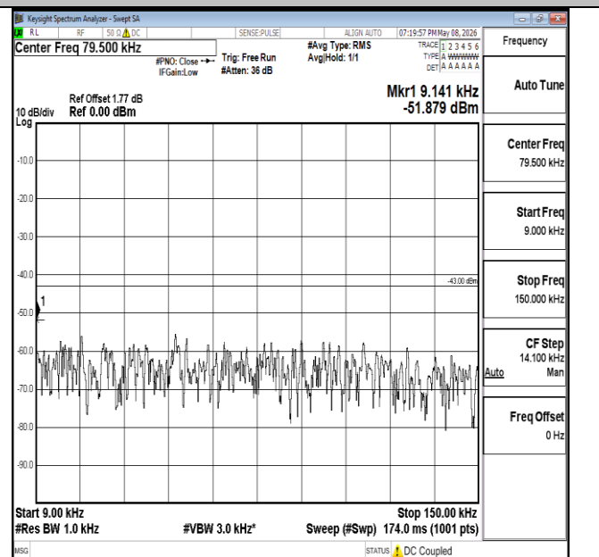
Band4-20MHz-16QAM-20050-1RB#0-0.009~0.15-PASS
