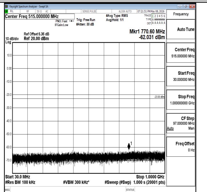
Band4-20MHz-16QAM-20175-1RB#0-30~1000-PASS
