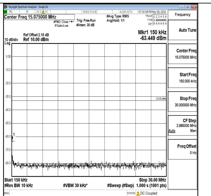
Band4-20MHz-QPSK-20175-1RB#0-0.15~30-PASS
