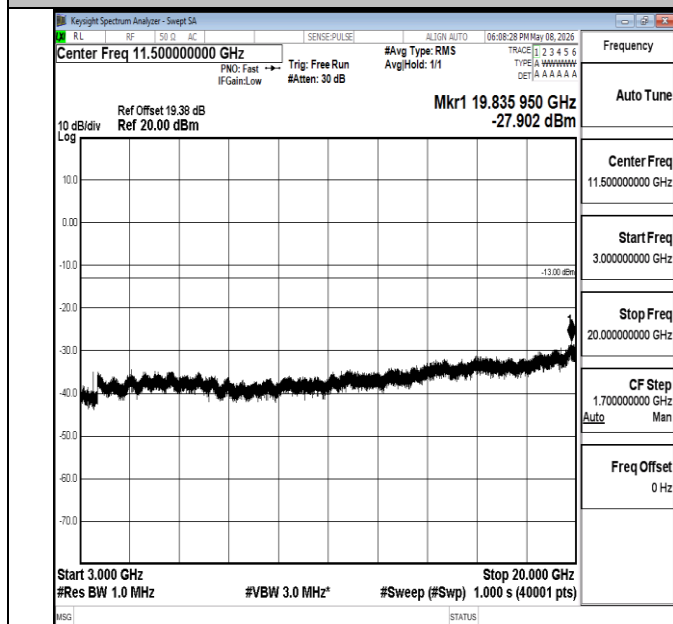
Band4-15MHz-QPSK-20175-1RB#0-3000~20000-PASS
