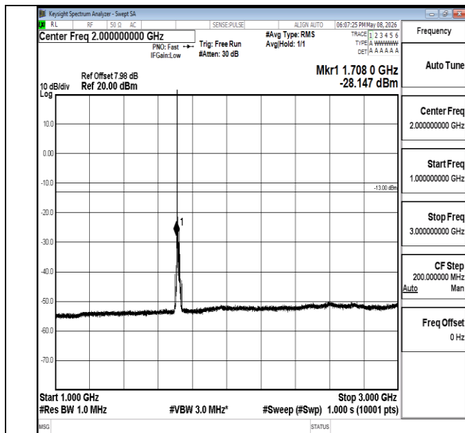
Band4-15MHz-16QAM-20025-1RB#0-1000~3000-PASS
