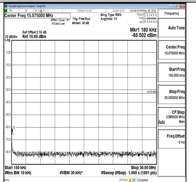
Band4-15MHz-QPSK-20175-1RB#0-0.15~30-PASS
