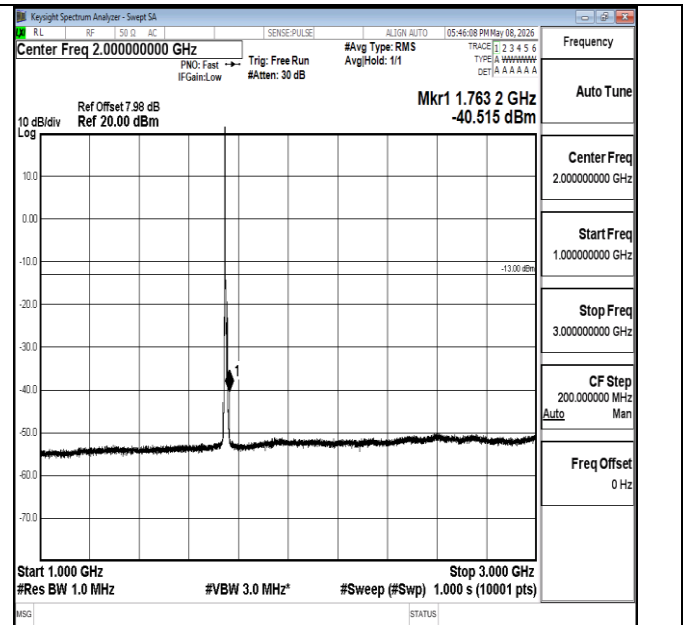
Band4-10MHz-QPSK-20350-1RB#0-1000~3000-PASS
