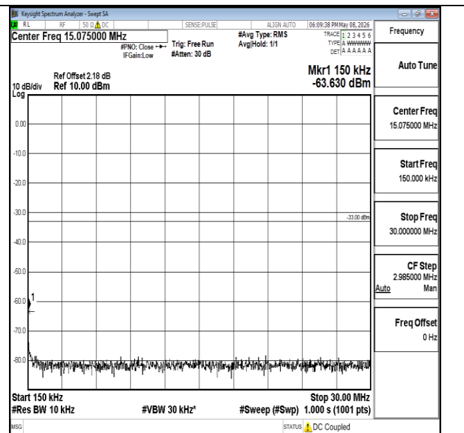
Band4-15MHz-QPSK-20325-1RB#0-0.15~30-PASS
