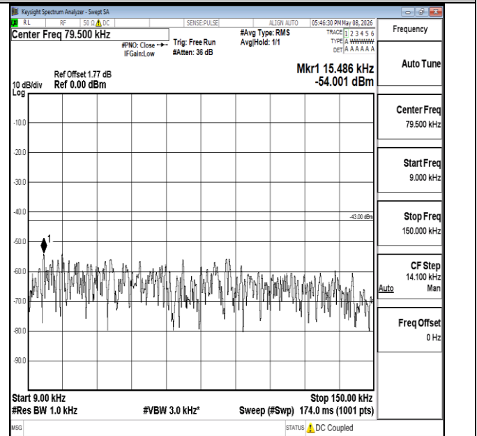
Band4-10MHz-16QAM-20350-1RB#0-0.009~0.15-PASS
