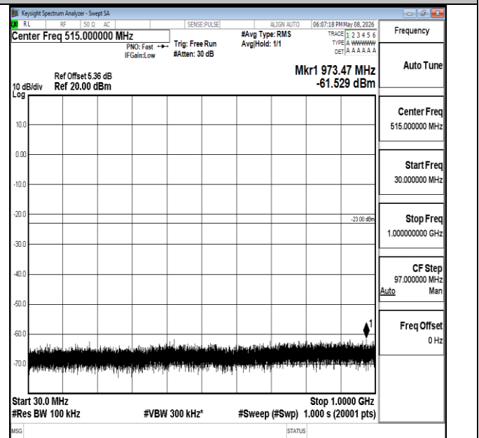
Band4-15MHz-16QAM-20025-1RB#0-30~1000-PASS
