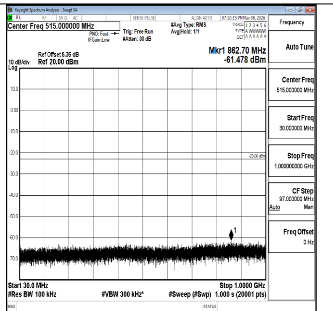
Band4-20MHz-16QAM-20050-1RB#0-0.30~1000-PASS
