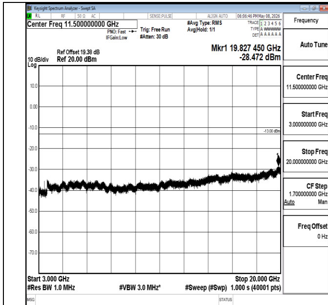
Band4-15MHz-QPSK-20025-1RB#0-3000~20000-PASS
