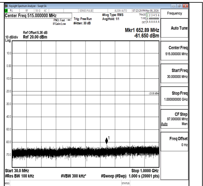
Band4-20MHz-16QAM-20300-1RB#0-30~1000-PASS
