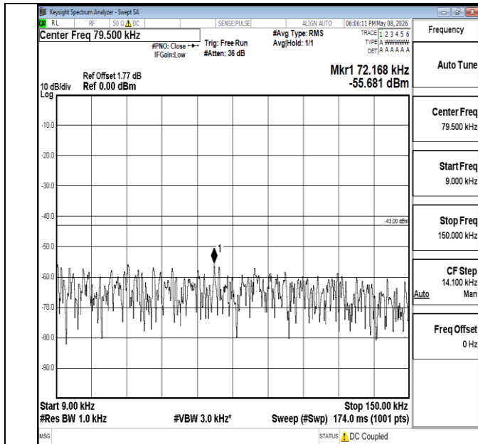
Band4-15MHz-QPSK-20025-1RB#0-0.009~0.15-PASS
