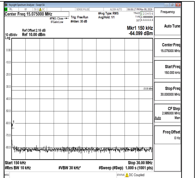
Band4-15MHz-QPSK-20025-1RB#0-0.15~30-PASS
