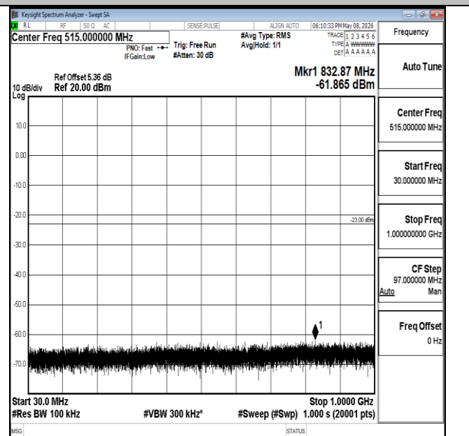
Band4-15MHz-16QAM-20325-1RB#0-30~1000-PASS
