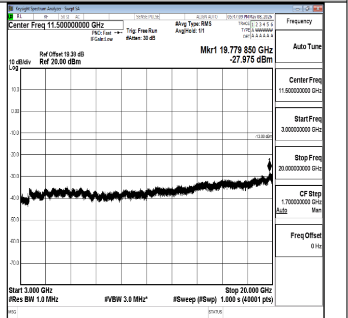
Band4-10MHz-16QAM-20350-1RB#0-3000~20000-PASS
