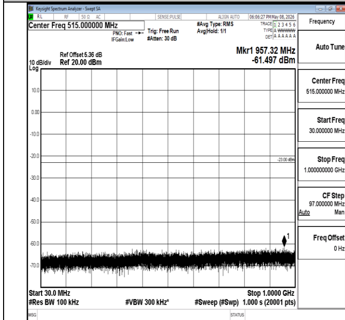
Band4-15MHz-QPSK-20025-1RB#0-30~1000-PASS
