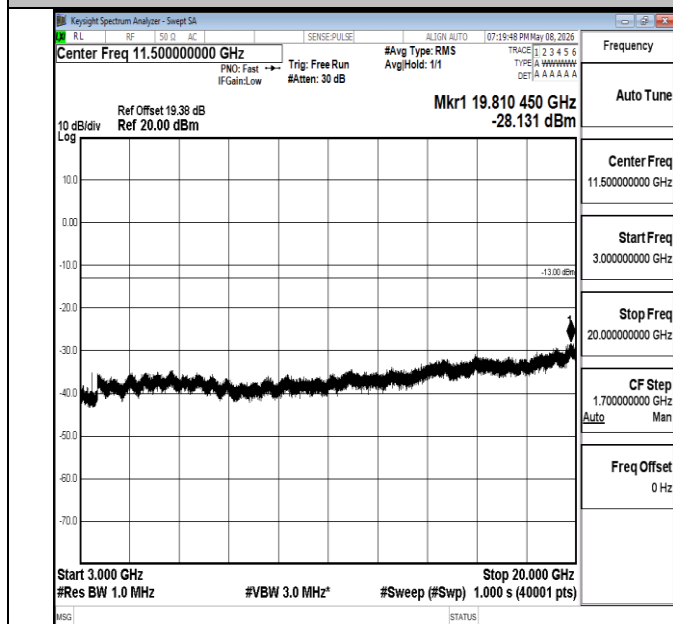
Band4-20MHz-QPSK-20050-1RB#0-3000~20000-PASS
