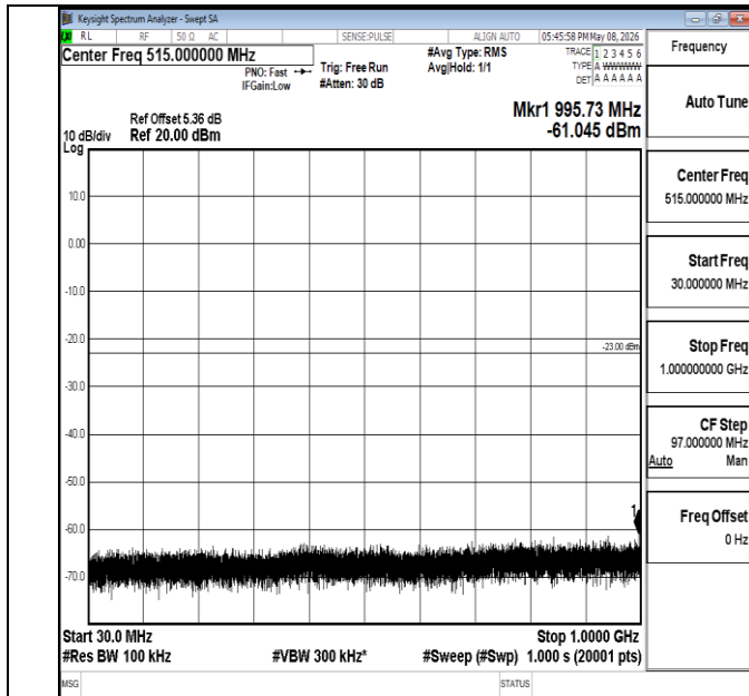
Band4-10MHz-QPSK-20350-1RB#0-30~1000-PASS
