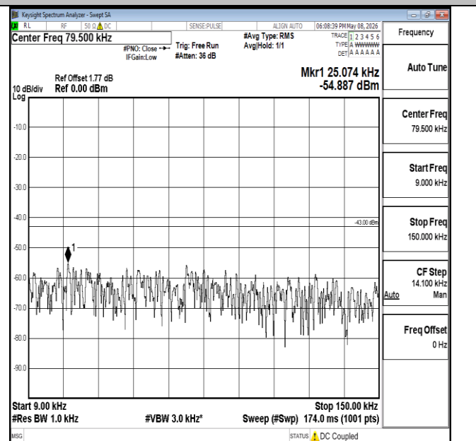
Band4-15MHz-16QAM-20175-1RB#0-0.009~0.15-PASS
