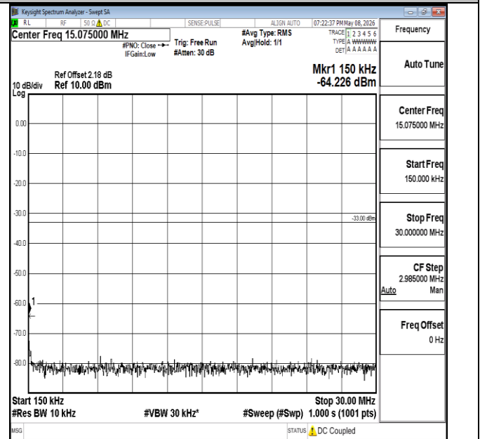
Band4-20MHz-QPSK-20300-1RB#0-0.15~30-PASS
