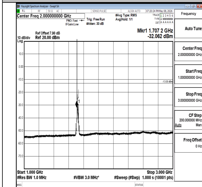
Band4-20MHz-16QAM-20050-1RB#0-1000~3000-PASS
