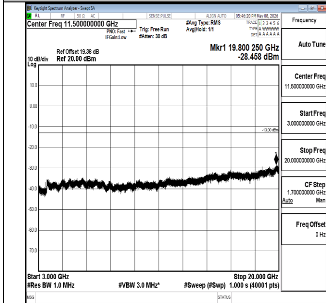
Band4-10MHz-QPSK-20350-1RB#0-3000~20000-PASS
