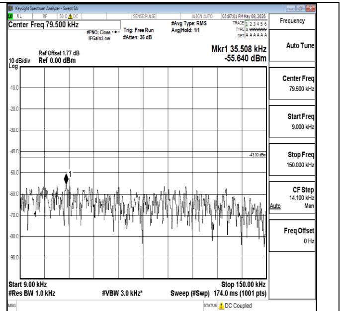
Band4-15MHz-16QAM-20025-1RB#0-0.009~0.15-PASS
