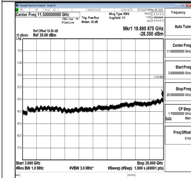
Band4-20MHz-QPSK-20300-1RB#0-3000~20000-PASS
