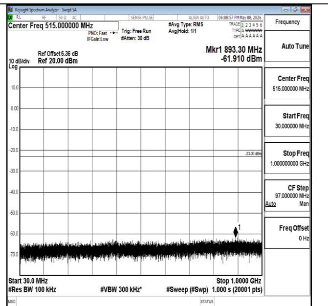
Band4-15MHz-16QAM-20175-1RB#0-30~1000-PASS
