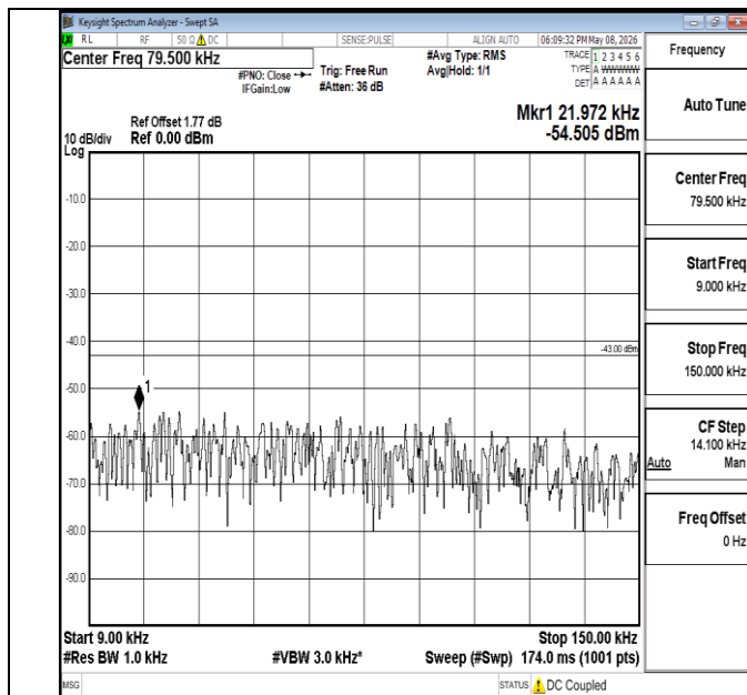
Band4-15MHz-QPSK-20325-1RB#0-0.009~0.15-PASS
