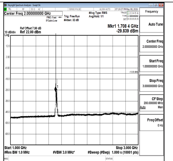
Band4-20MHz-QPSK-20050-1RB#0-1000~3000-PASS
