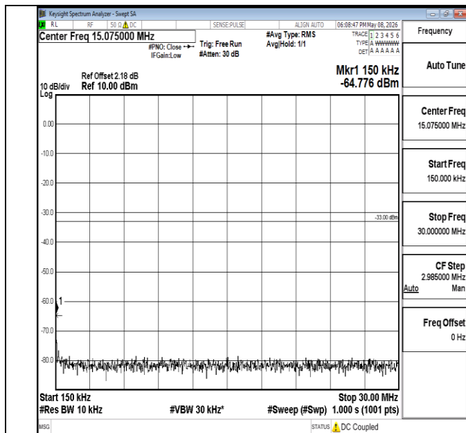
Band4-15MHz-16QAM-20175-1RB#0-0.15~30-PASS
