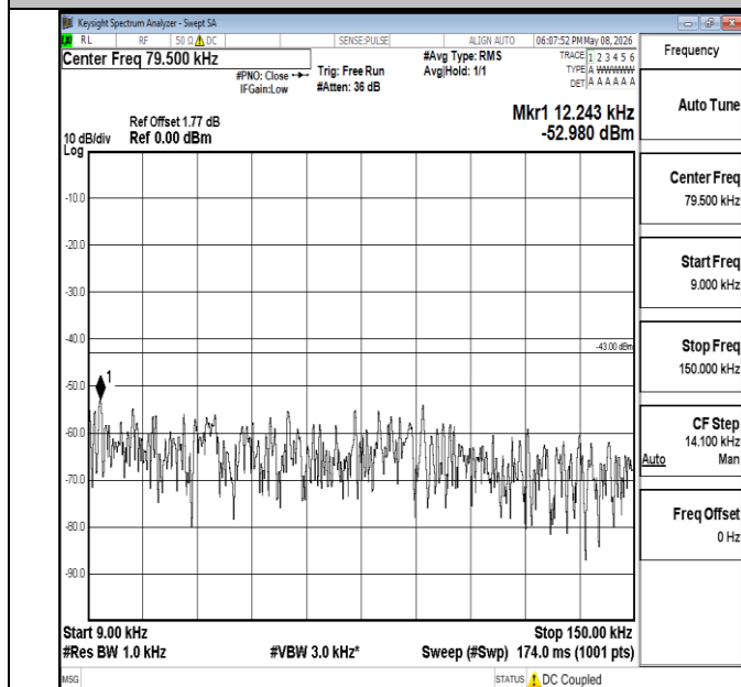
Band4-15MHz-QPSK-20175-1RB#0-0.009~0.15-PASS
