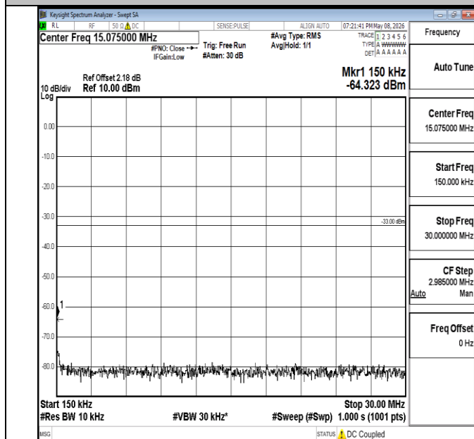
Band4-20MHz-16QAM-20175-1RB#0-0.15~30-PASS
