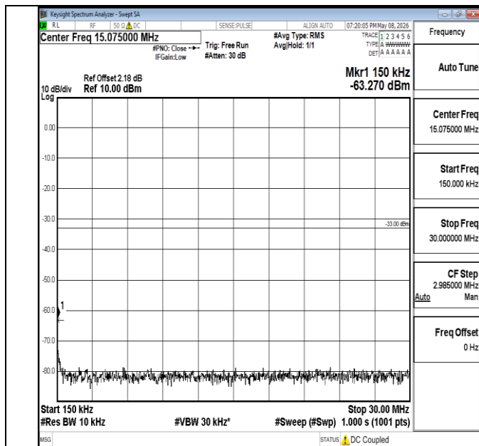
Band4-20MHz-16QAM-20050-1RB#0-0.15~30-PASS
