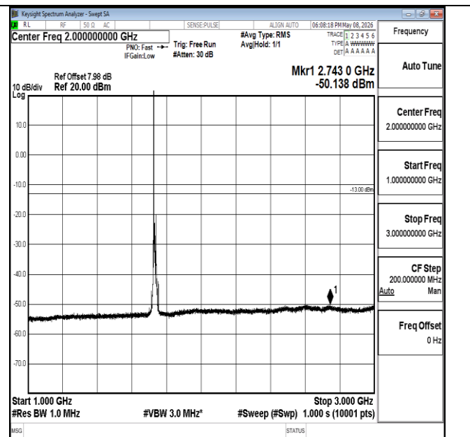
Band4-15MHz-QPSK-20175-1RB#0-1000~3000-PASS
