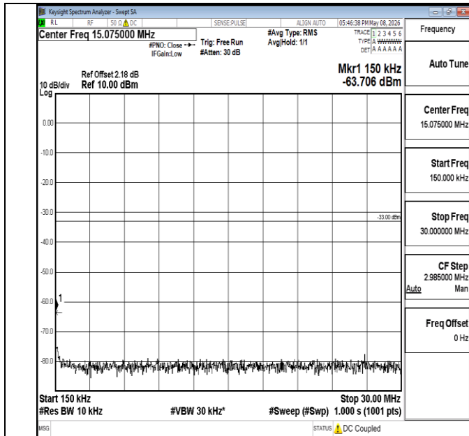
Band4-10MHz-16QAM-20350-1RB#0-0.15~30-PASS
