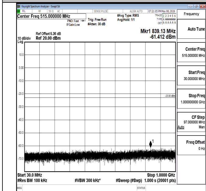
Band4-20MHz-QPSK-20175-1RB#0-30~1000-PASS
