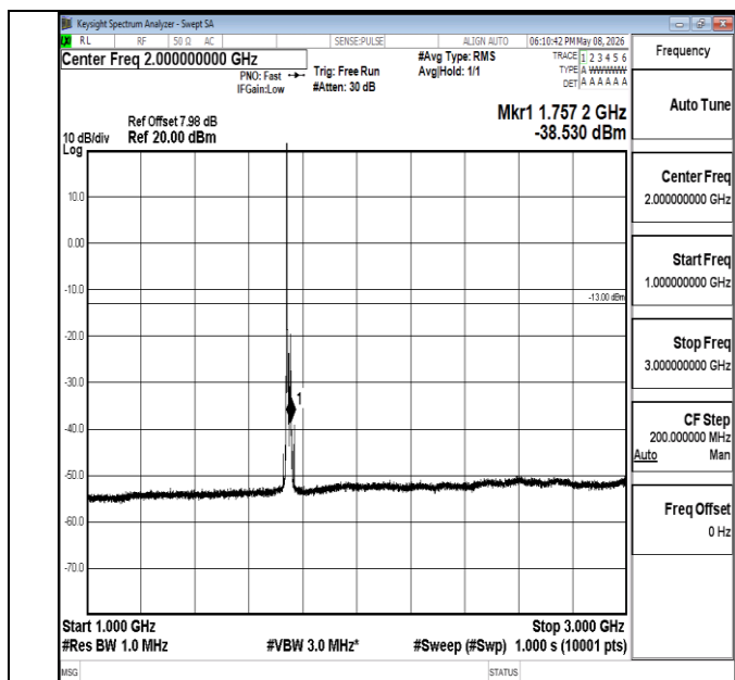
Band4-15MHz-16QAM-20325-1RB#0-1000~3000-PASS
