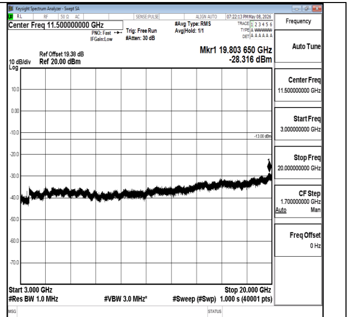
Band4-20MHz-16QAM-20175-1RB#0-3000~20000-PASS
