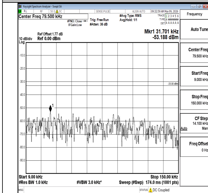
Band5-3MHz-QPSK-20415-1RB#0-0.009~0.15-PASS
