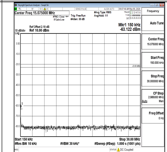
Band5-1.4MHz-QPSK-20525-1RB#0-0.15~30-PASS
