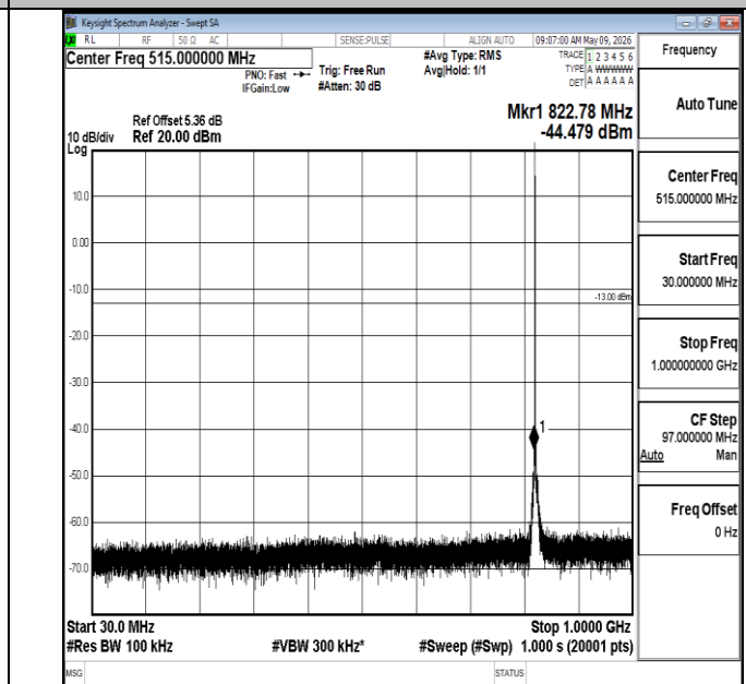
Band5-1.4MHz-16QAM-20407-1RB#0-30~1000-PASS
