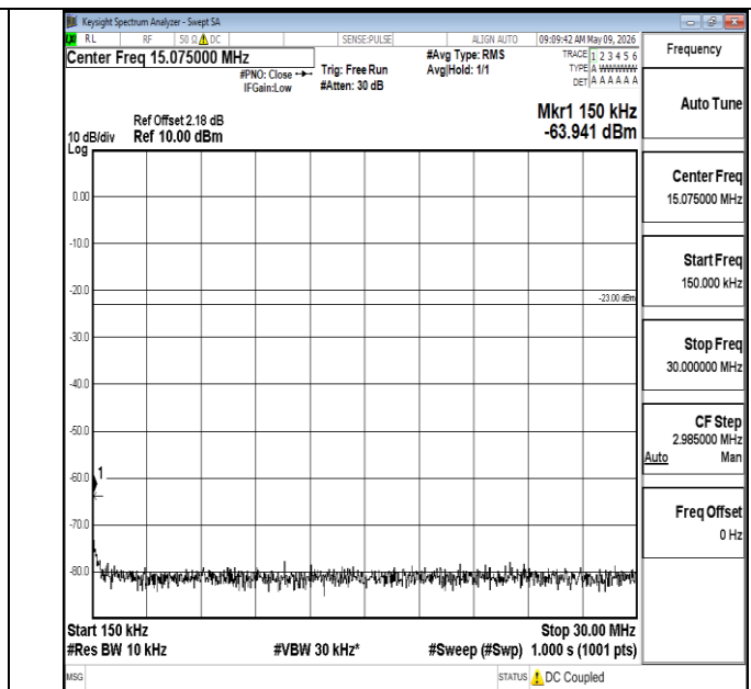
Band5-1.4MHz-QPSK-20643-1RB#0-0.15~30-PASS
