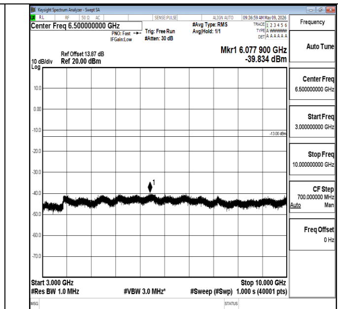
Band5-3MHz-16QAM-20525-1RB#0-3000~10000-PASS
