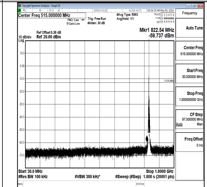
Band5-3MHz-16QAM-20525-1RB#0-30~1000-PASS
