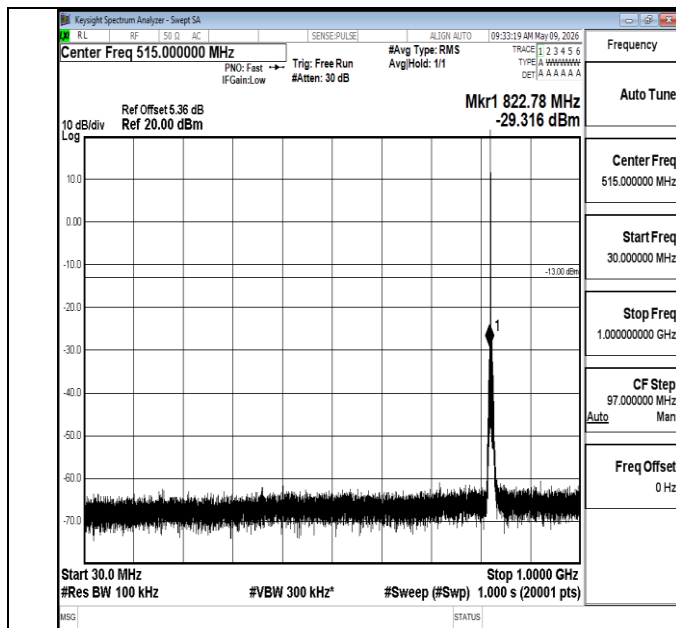
Band5-3MHz-QPSK-20415-1RB#0-30~1000-PASS
