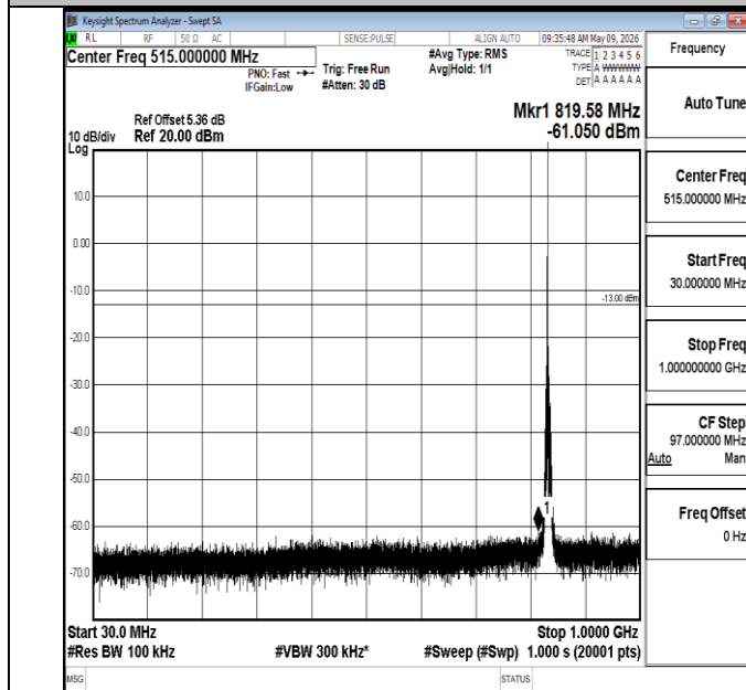
Band5-3MHz-QPSK-20525-1RB#0-30~1000-PASS
