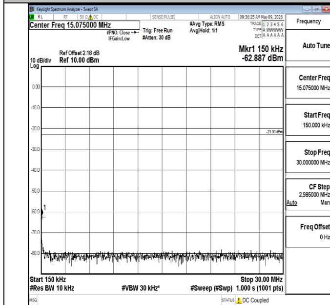
Band5-3MHz-16QAM-20525-1RB#0-0.15~30-PASS
