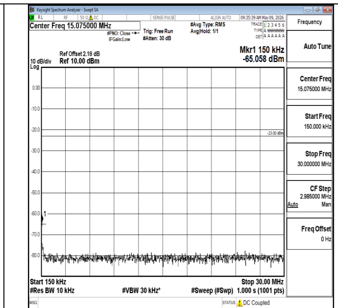
Band5-3MHz-QPSK-20525-1RB#0-0.15~30-PASS
