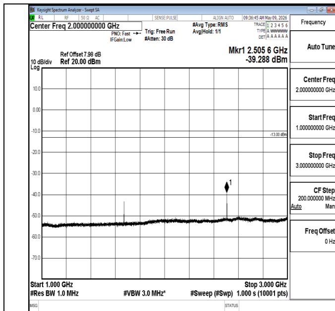
Band5-3MHz-16QAM-20525-1RB#0-1000~3000-PASS
