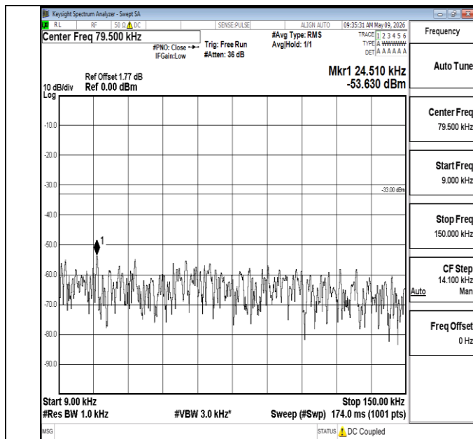
Band5-3MHz-QPSK-20525-1RB#0-0.009~0.15-PASS
