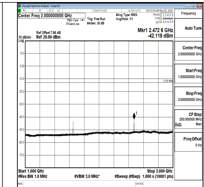
Band5-3MHz-QPSK-20415-1RB#0-1000~3000-PASS
