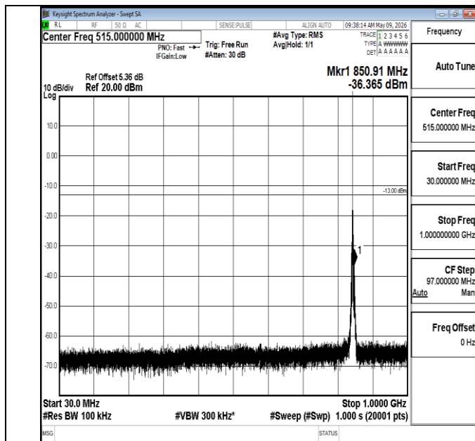
Band5-3MHz-QPSK-20635-1RB#0-30~1000-PASS
