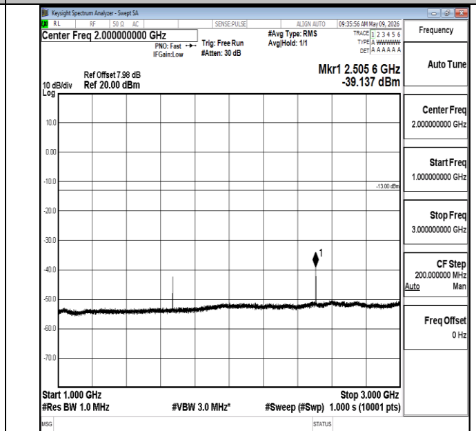
Band5-3MHz-QPSK-20525-1RB#0-1000~3000-PASS
