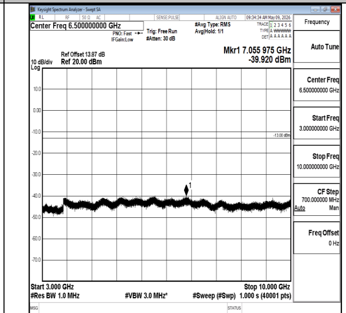
Band5-3MHz-16QAM-20415-1RB#0-3000~10000-PASS
