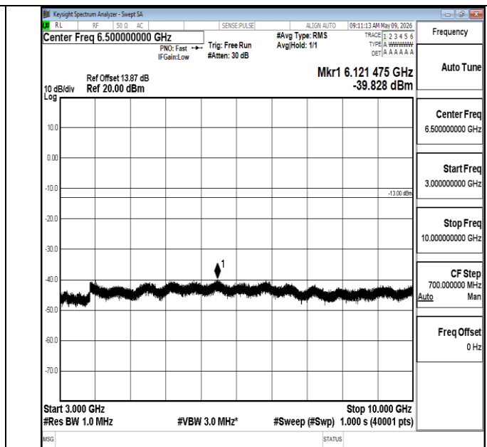
Band5-1.4MHz-16QAM-20643-1RB#0-3000~10000-PASS
