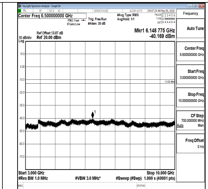
Band5-1.4MHz-16QAM-20407-1RB#0-3000~10000-PASS
