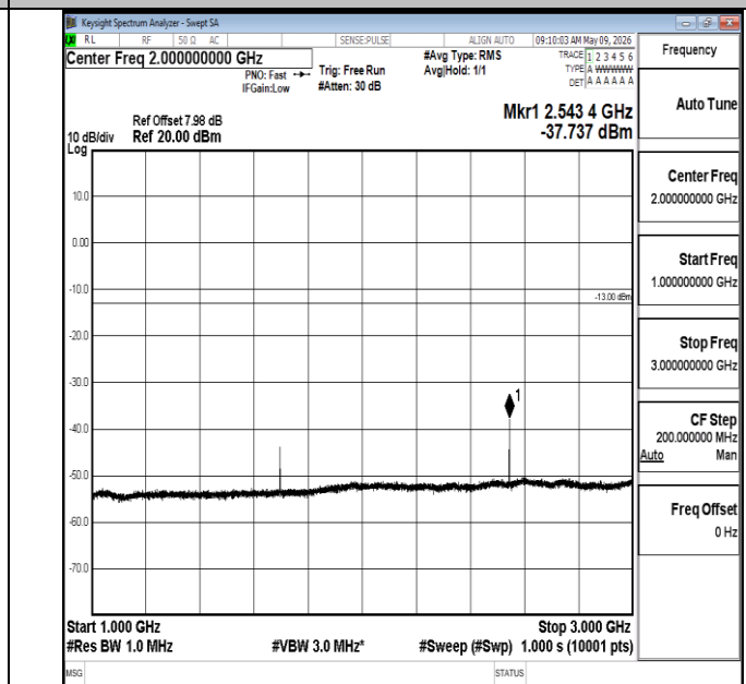
Band5-1.4MHz-QPSK-20643-1RB#0-1000~3000-PASS
