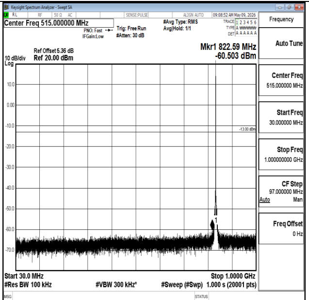
Band5-1.4MHz-16QAM-20525-1RB#0-30~1000-PASS
