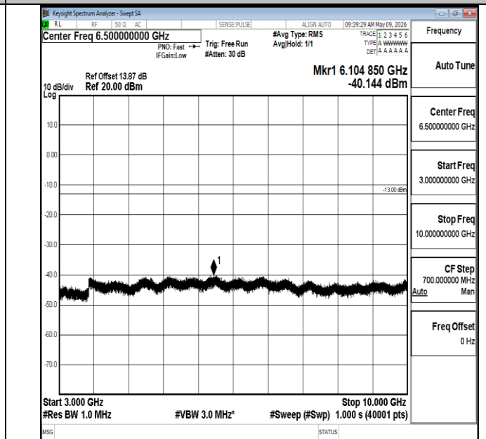
Band5-3MHz-16QAM-20635-1RB#0-3000~10000-PASS
