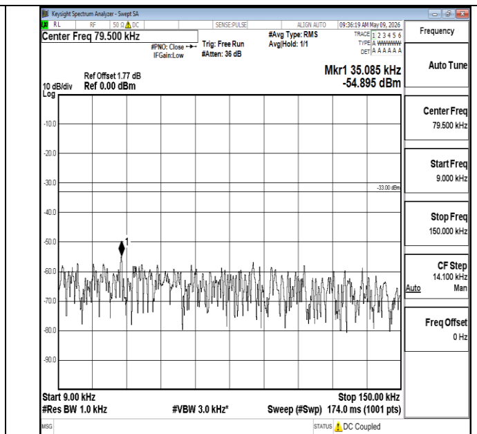
Band5-3MHz-16QAM-20525-1RB#0-0.009~0.15-PASS
