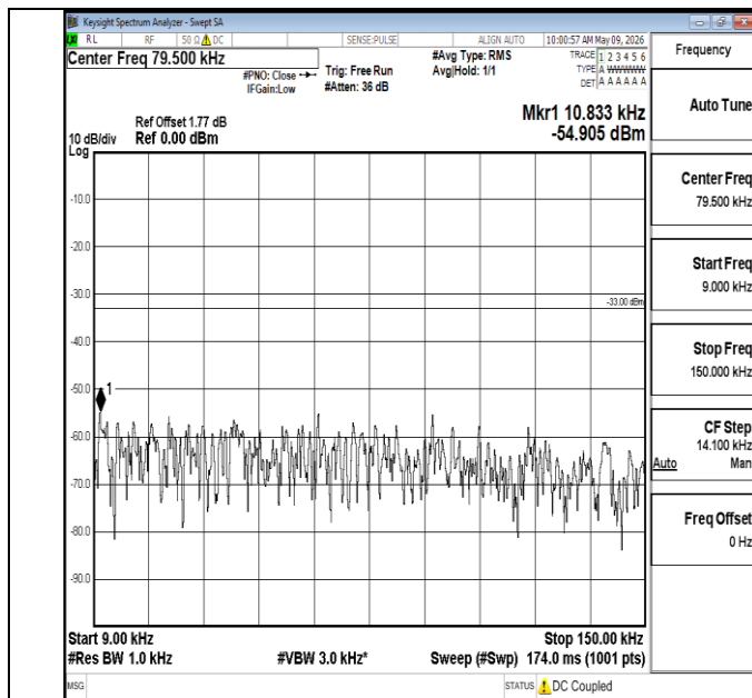
Band5-5MHz-QPSK-20425-1RB#0-0.009~0.15-PASS
