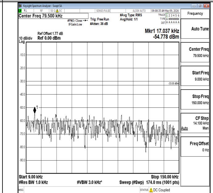
Band5-1.4MHz-16QAM-20525-1RB#0-0.009~0.15-PASS
