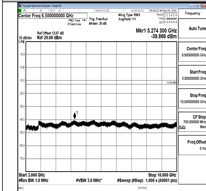
Band5-1.4MHz-QPSK-20525-1RB#0-3000~10000-PASS
