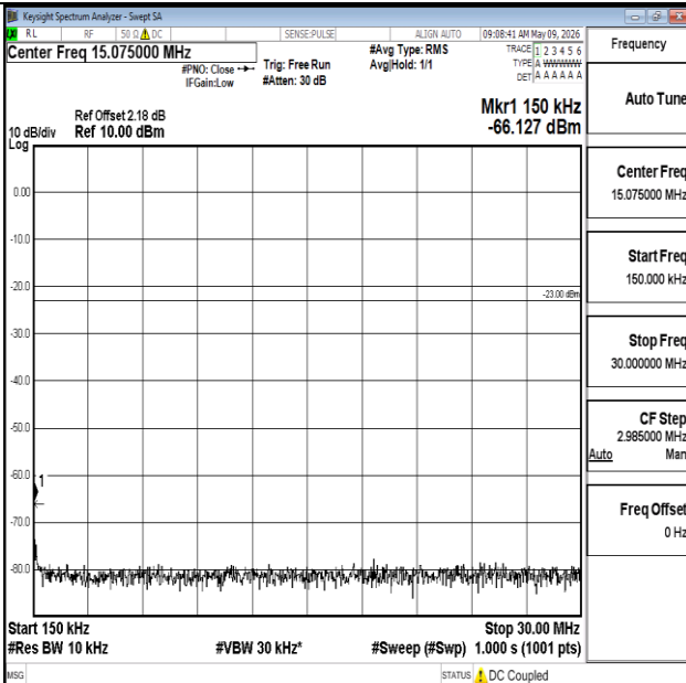
Band5-1.4MHz-16QAM-20525-1RB#0-0.15~30-PASS
