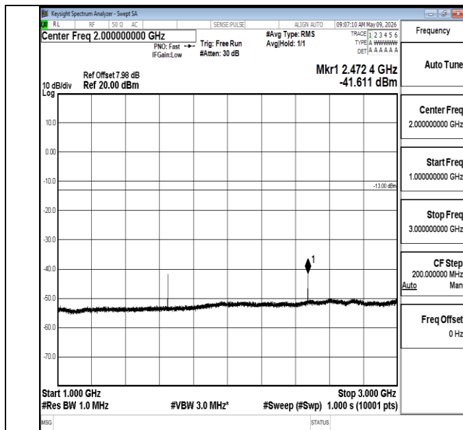
Band5-1.4MHz-16QAM-20407-1RB#0-1000~3000-PASS
