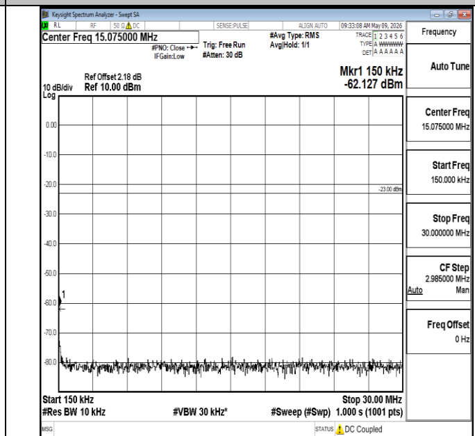
Band5-3MHz-QPSK-20415-1RB#0-0.15~30-PASS
