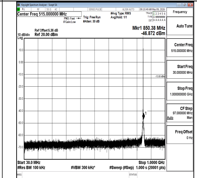
Band5-1.4MHz-16QAM-20643-1RB#0-30~1000-PASS
