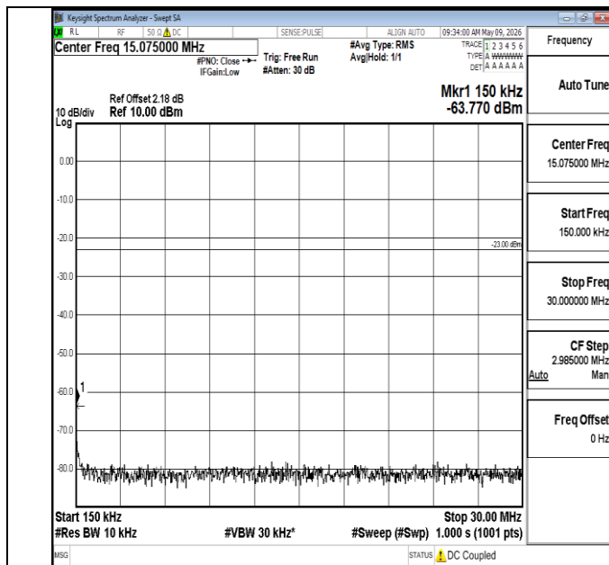
Band5-3MHz-16QAM-20415-1RB#0-0.15~30-PASS
