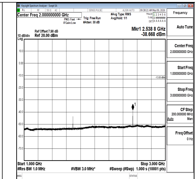
Band5-3MHz-QPSK-20635-1RB#0-1000~3000-PASS
