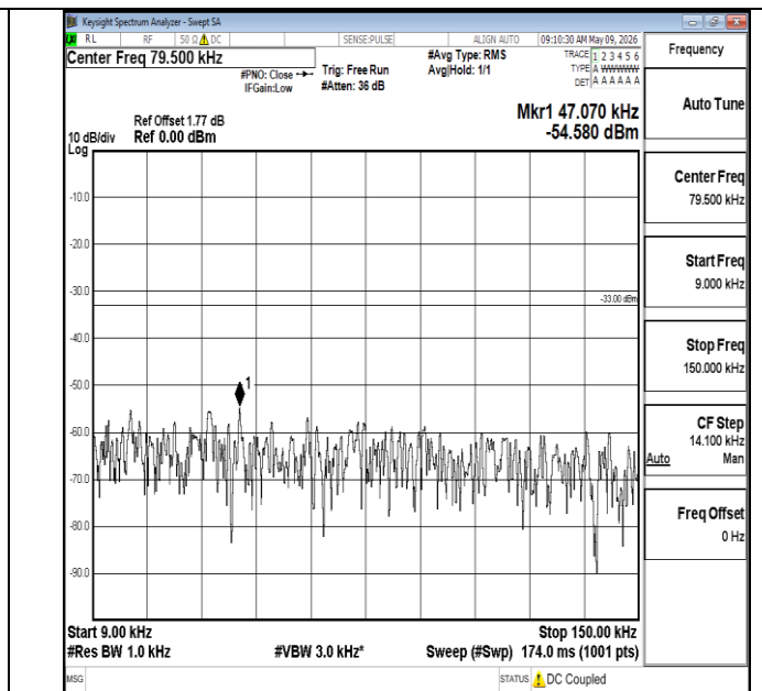
Band5-1.4MHz-16QAM-20643-1RB#0-0.009~0.15-PASS
