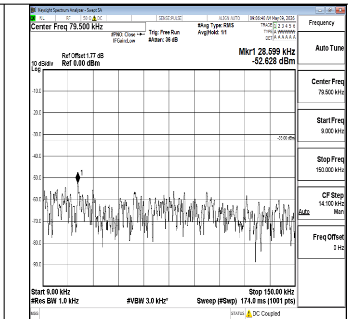
Band5-1.4MHz-16QAM-20407-1RB#0-0.009~0.15-PASS
