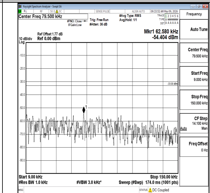
Band5-3MHz-16QAM-20415-1RB#0-0.009~0.15-PASS
