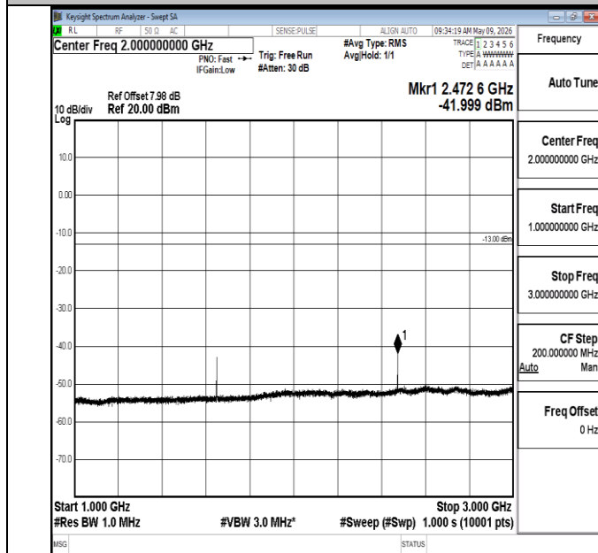
Band5-3MHz-16QAM-20415-1RB#0-1000~3000-PASS
