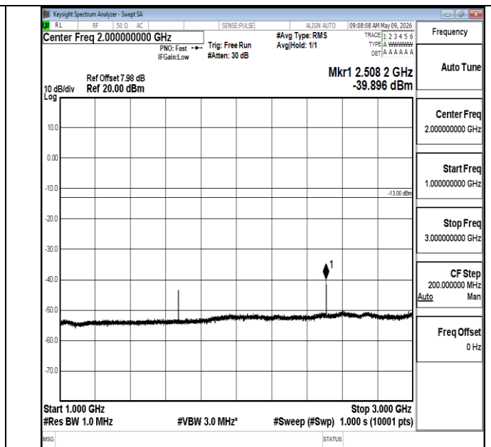
Band5-1.4MHz-QPSK-20525-1RB#0-1000~3000-PASS
