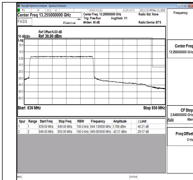
Band5-10MHz-16QAM-20600-27RB#0-PASS
