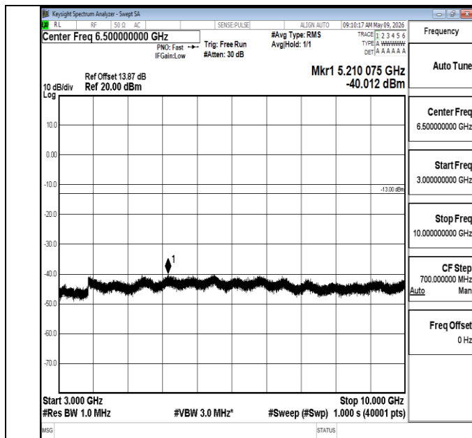
Band5-1.4MHz-QPSK-20643-1RB#0-3000~10000-PASS
