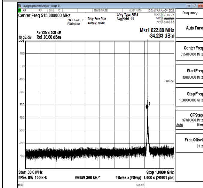
Band5-5MHz-QPSK-20425-1RB#0-30~1000-PASS
