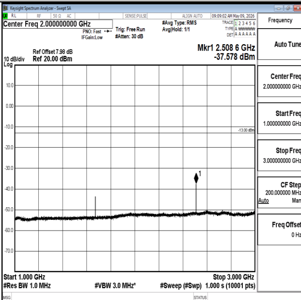
Band5-1.4MHz-16QAM-20525-1RB#0-1000~3000-PASS
