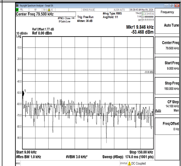
Band5-3MHz-16QAM-20635-1RB#0-0.009~0.15-PASS
