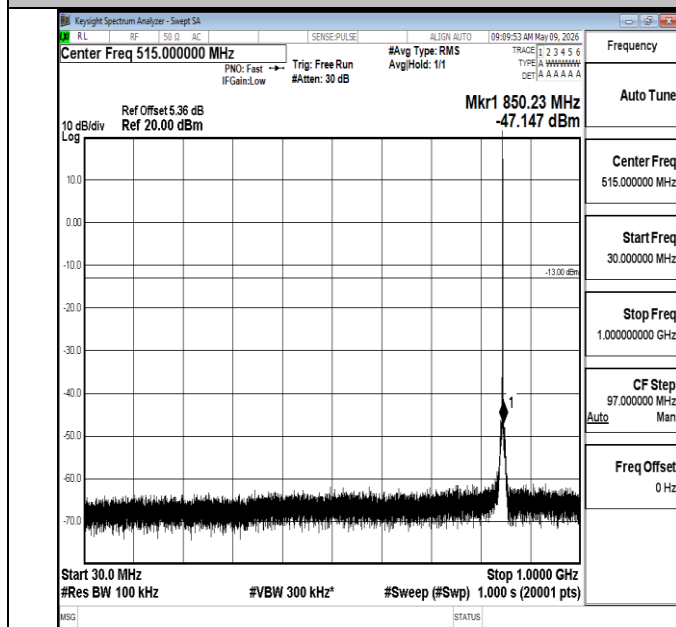
Band5-1.4MHz-QPSK-20643-1RB#0-30~1000-PASS
