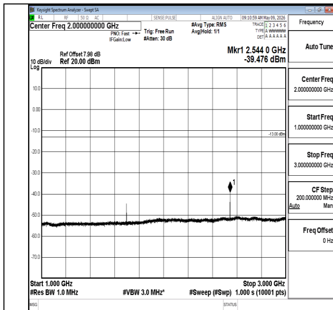
Band5-1.4MHz-16QAM-20643-1RB#0-1000~3000-PASS
