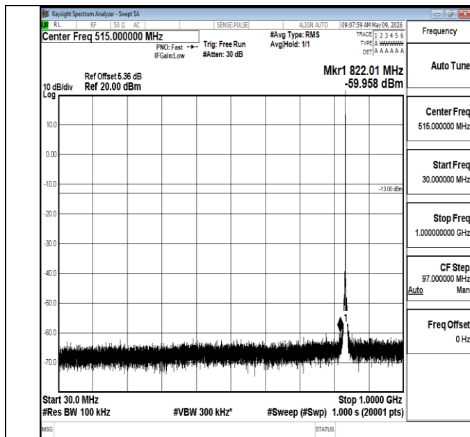
Band5-1.4MHz-QPSK-20525-1RB#0-30~1000-PASS
