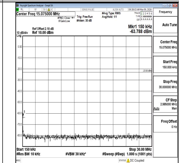
Band5-3MHz-QPSK-20635-1RB#0-0.15~30-PASS
