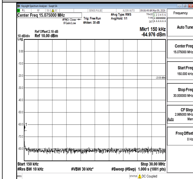
Band5-1.4MHz-16QAM-20407-1RB#0-0.15~30-PASS
