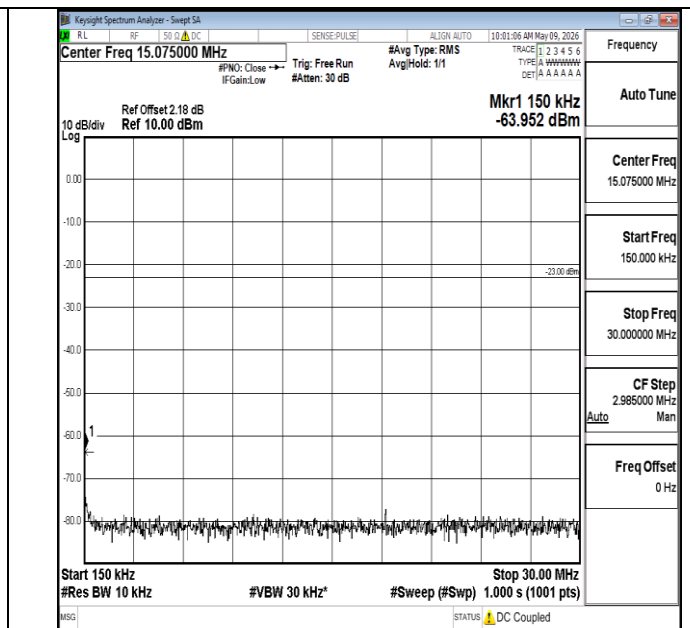
Band5-5MHz-QPSK-20425-1RB#0-0.15~30-PASS
