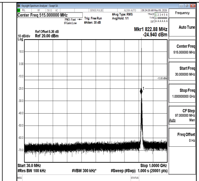
Band5-3MHz-16QAM-20415-1RB#0-30~1000-PASS
