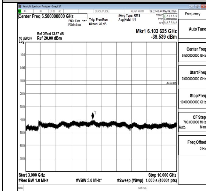
Band5-3MHz-QPSK-20415-1RB#0-3000~10000-PASS
