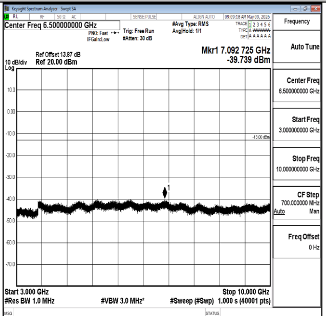
Band5-1.4MHz-16QAM-20525-1RB#0-3000~10000-PASS
