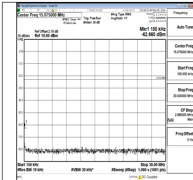
Band5-3MHz-16QAM-20635-1RB#0-0.15~30-PASS
