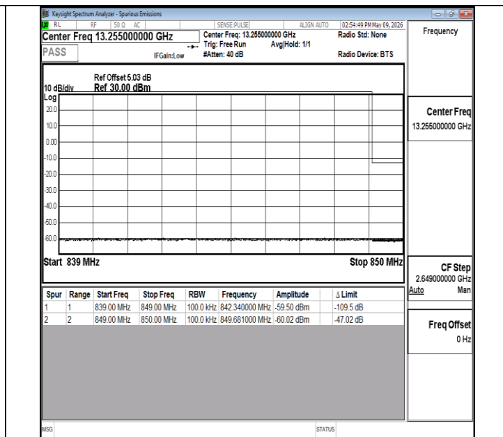
Band5-10MHz-16QAM-20600-50RB#0-PASS
