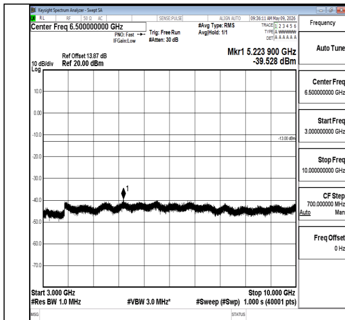
Band5-3MHz-QPSK-20525-1RB#0-3000~10000-PASS
