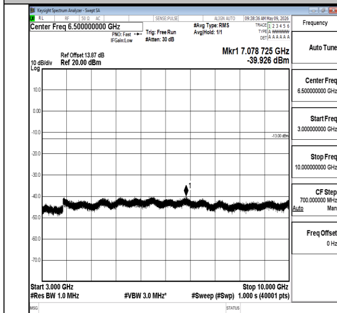
Band5-3MHz-QPSK-20635-1RB#0-3000~10000-PASS
