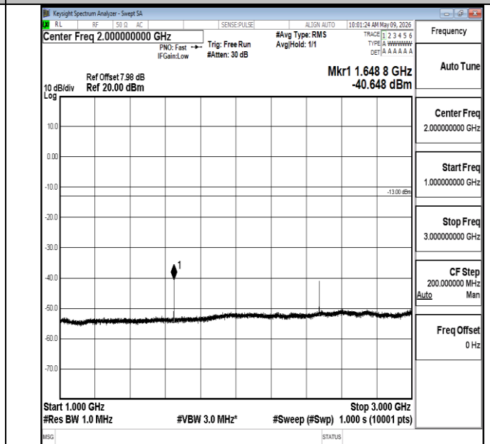
Band5-5MHz-QPSK-20425-1RB#0-1000~3000-PASS
