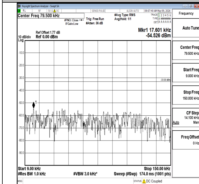
Band5-1.4MHz-QPSK-20525-1RB#0-0.009~0.15-PASS
