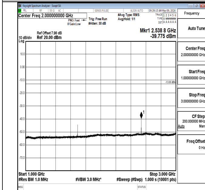
Band5-3MHz-16QAM-20635-1RB#0-1000~3000-PASS
