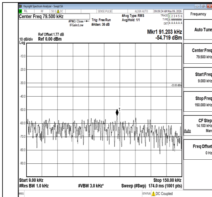
Band5-1.4MHz-QPSK-20643-1RB#0-0.009~0.15-PASS
