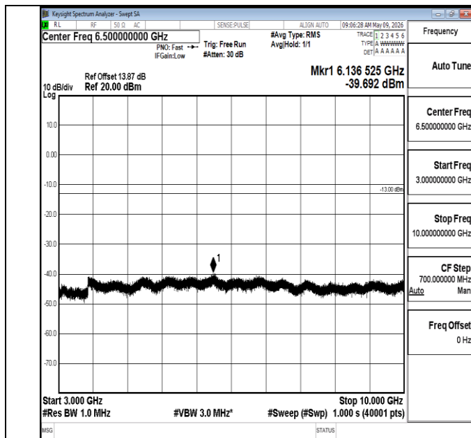
Band5-1.4MHz-QPSK-20407-1RB#0-3000~10000-PASS
