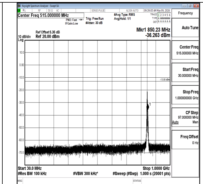
Band5-3MHz-16QAM-20635-1RB#0-30~1000-PASS
