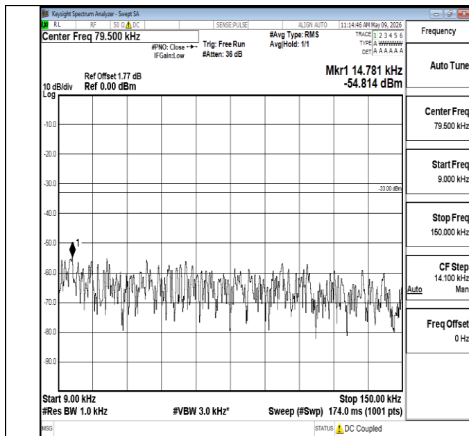
Band5-10MHz-QPSK-20525-1RB#0-0.009~0.15-PASS
