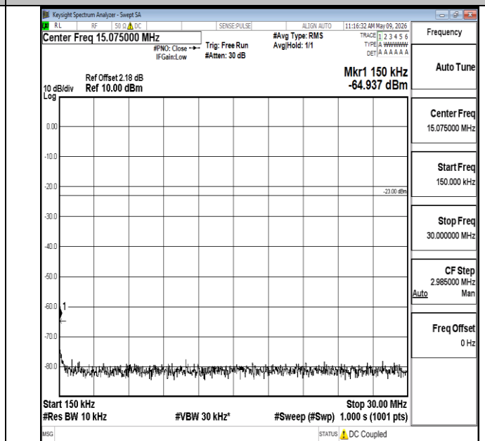
Band5-10MHz-QPSK-20600-1RB#0-0.15~30-PASS
