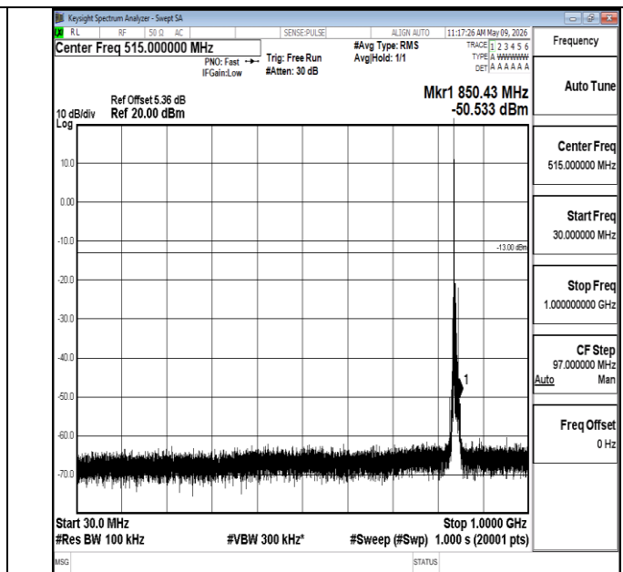
Band5-10MHz-16QAM-20600-1RB#0-30~1000-PASS
