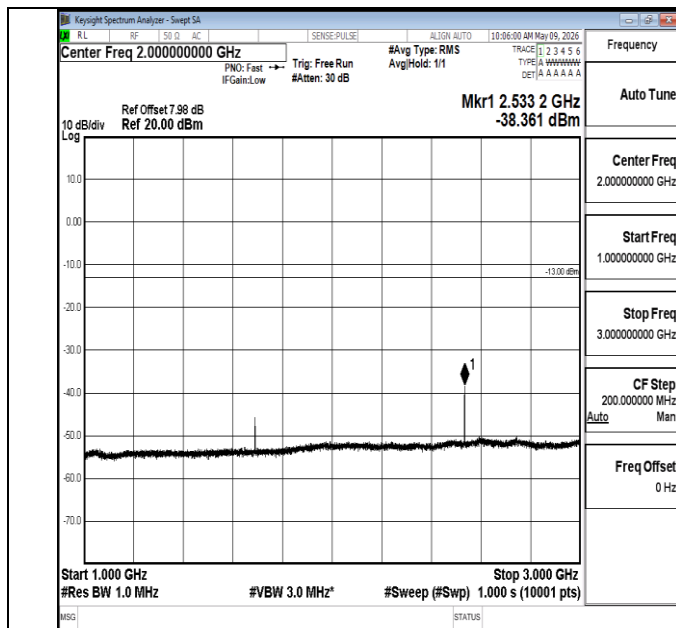
Band5-5MHz-16QAM-20625-1RB#0-1000~3000-PASS
