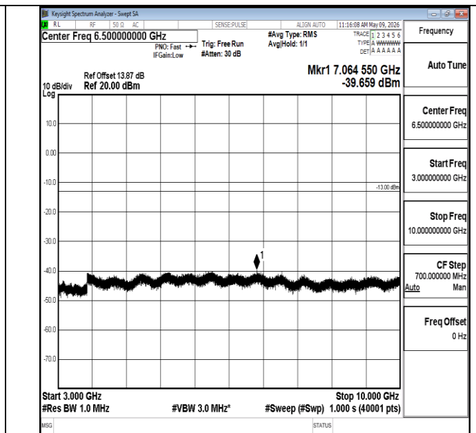
Band5-10MHz-16QAM-20525-1RB#0-3000~10000-PASS
