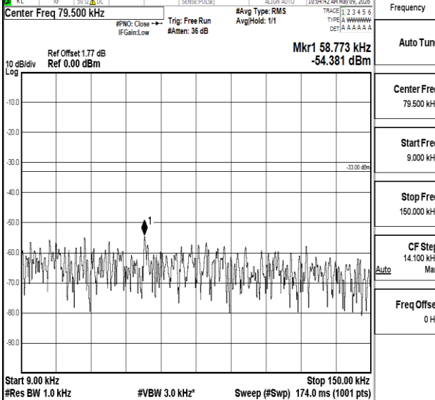
Band5-5MHz-QPSK-20625-1RB#0-0.009~0.15-PASS
