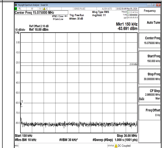
Band5-5MHz-QPSK-20525-1RB#0-0.15~30-PASS
