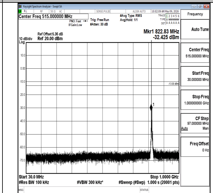
Band5-5MHz-16QAM-20425-1RB#0-30~1000-PASS
