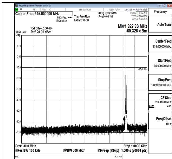
Band5-5MHz-QPSK-20525-1RB#0-30~1000-PASS
