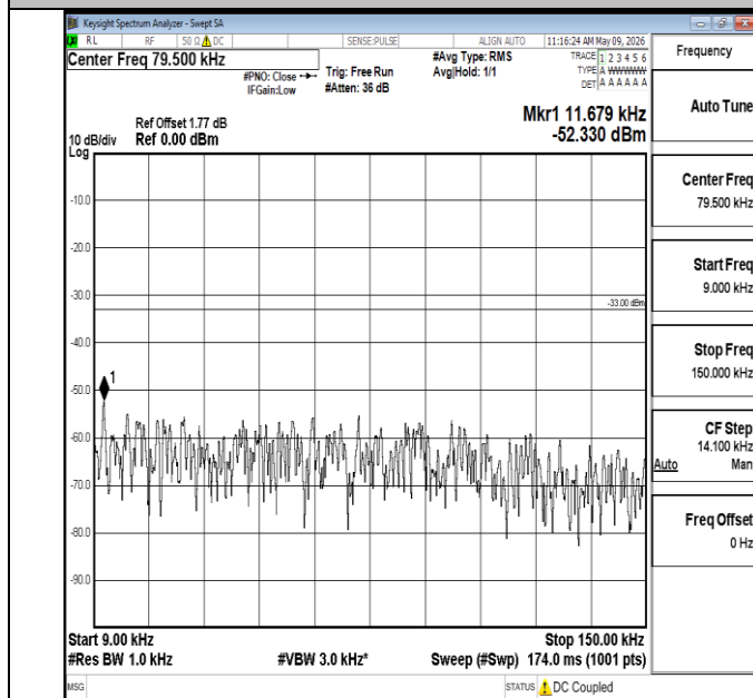
Band5-10MHz-QPSK-20600-1RB#0-0.009~0.15-PASS
