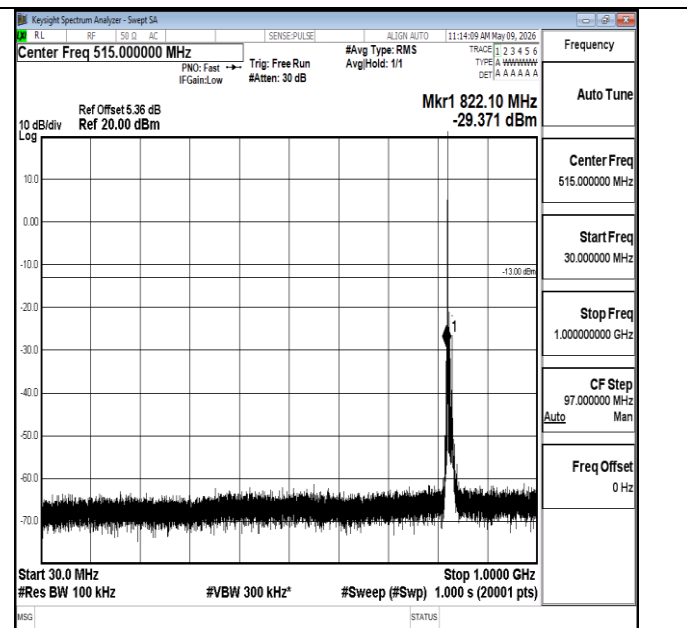
Band5-10MHz-16QAM-20450-1RB#0-0-30~1000-PASS
