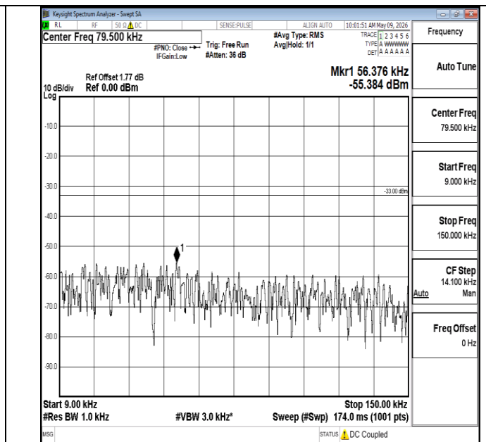
Band5-5MHz-16QAM-20425-1RB#0-0.009~0.15-PASS
