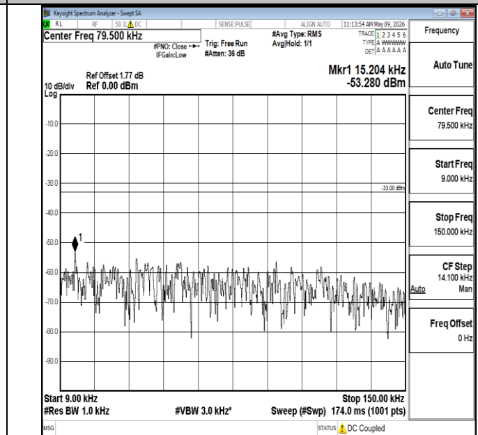
Band5-10MHz-16QAM-20450-1RB#0-0.009~0.15-PASS
