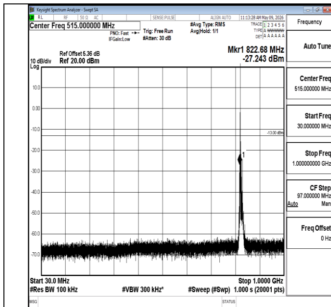
Band5-10MHz-QPSK-20450-1RB#0-30~1000-PASS
