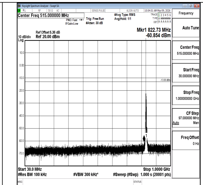
Band5-5MHz-16QAM-20525-1RB#0-30~1000-PASS
