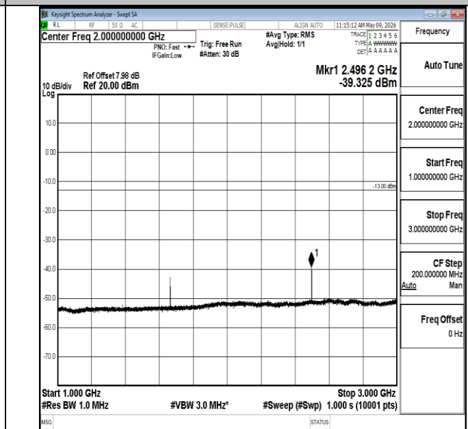
Band5-10MHz-QPSK-20525-1RB#0-1000~3000-PASS
