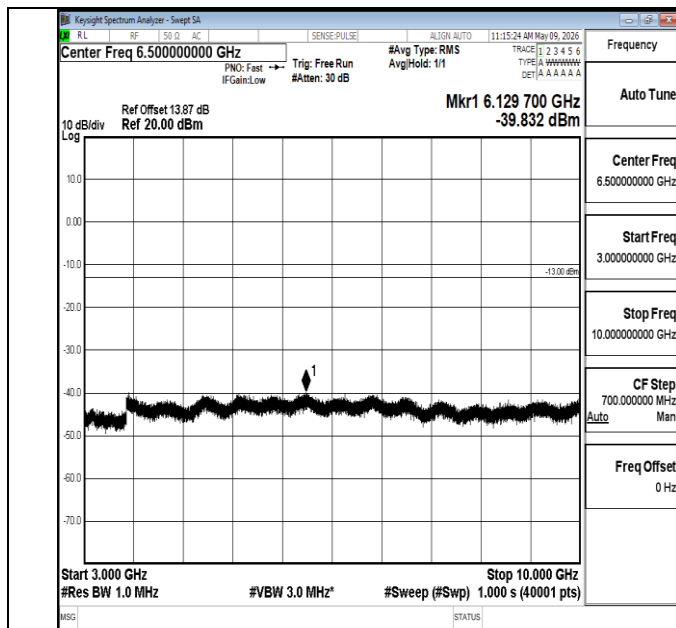
Band5-10MHz-QPSK-20525-1RB#0-3000~10000-PASS
