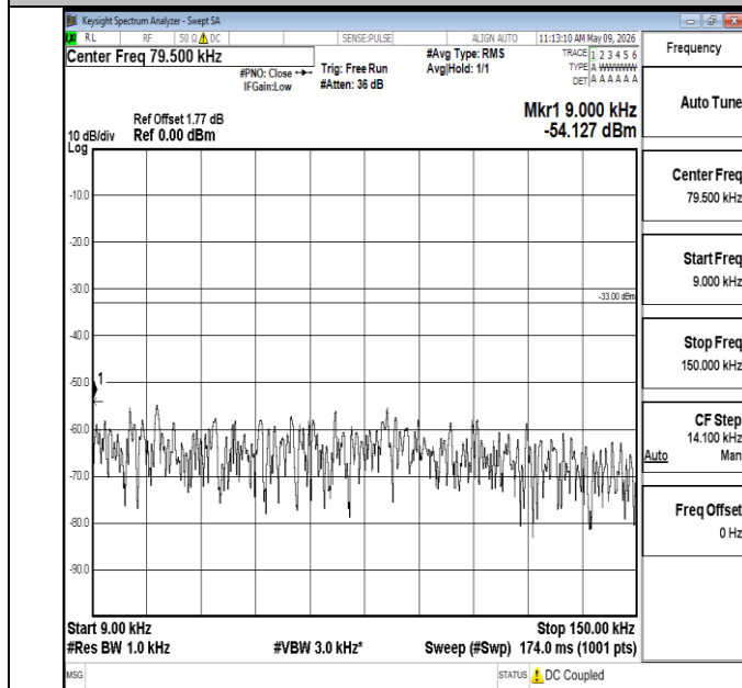
Band5-10MHz-QPSK-20450-1RB#0-0.009~0.15-PASS
