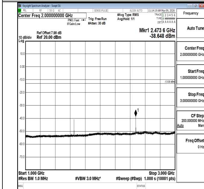
Band5-10MHz-16QAM-20450-1RB#0-1000~3000-PASS
