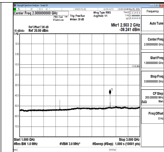
Band5-5MHz-QPSK-20525-1RB#0-1000~3000-PASS
