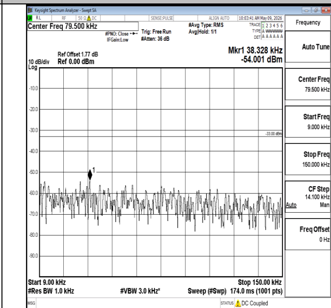
Band5-5MHz-16QAM-20525-1RB#0-0.009~0.15-PASS
