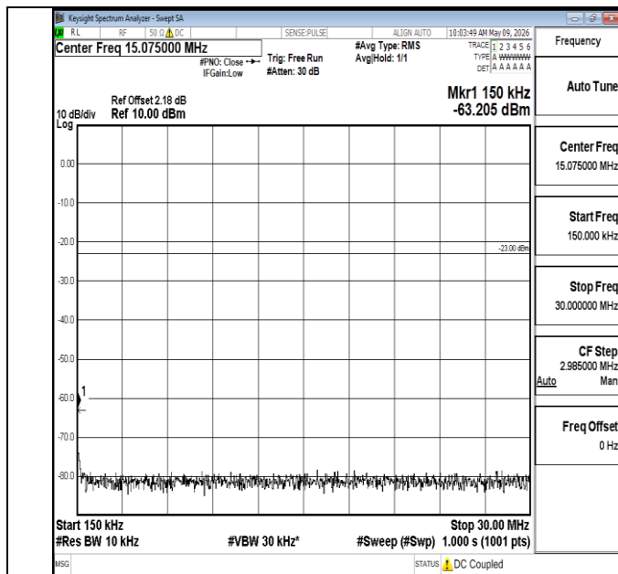
Band5-5MHz-16QAM-20525-1RB#0-0.15~30-PASS
