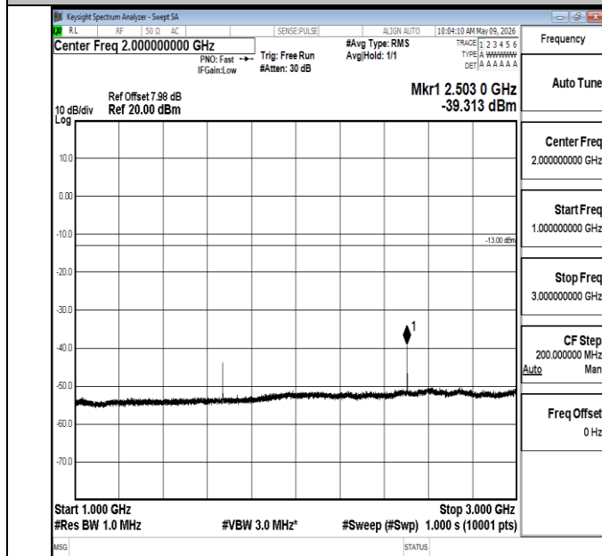
Band5-5MHz-16QAM-20525-1RB#0-1000~3000-PASS
