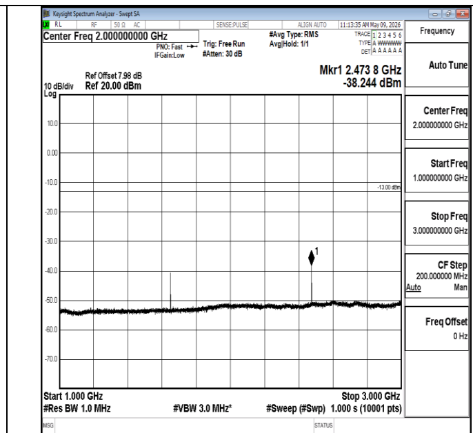
Band5-10MHz-QPSK-20450-1RB#0-1000~3000-PASS
