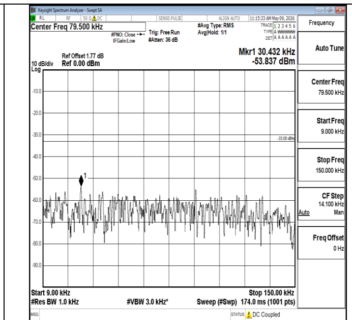
Band5-10MHz-16QAM-20525-1RB#0-0.009~0.15-PASS
