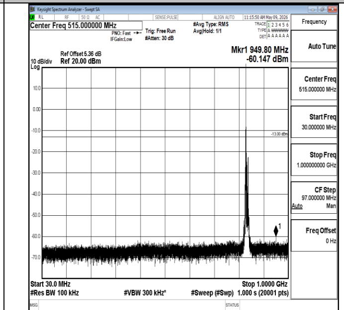
Band5-10MHz-16QAM-20525-1RB#0-30~1000-PASS
