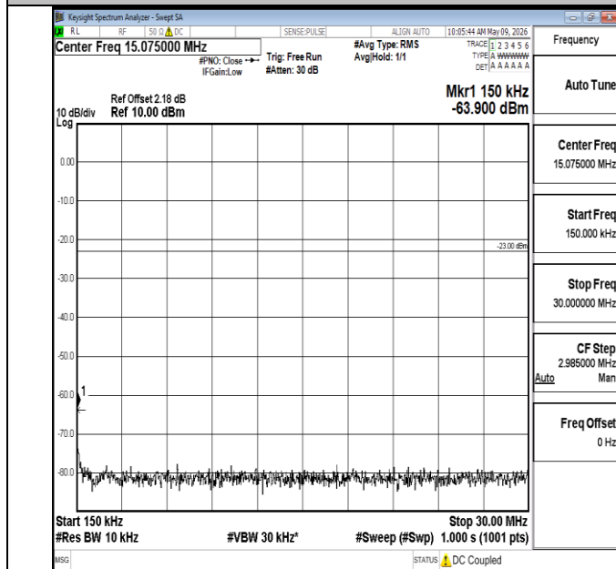
Band5-5MHz-16QAM-20625-1RB#0-0.15~30-PASS
