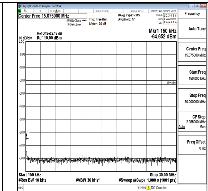
Band5-10MHz-QPSK-20525-1RB#0-0.15~30-PASS
