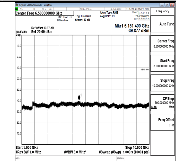
Band5-10MHz-16QAM-20600-1RB#0-3000~10000-PASS
