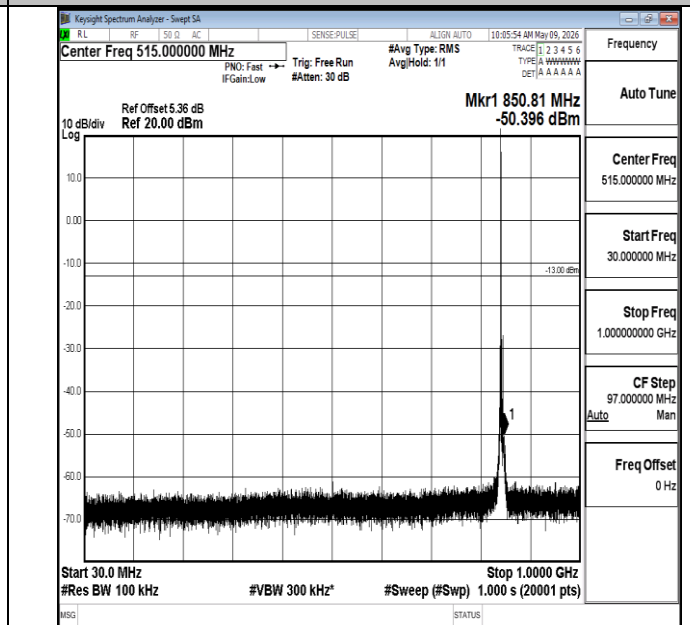
Band5-5MHz-16QAM-20625-1RB#0-30~1000-PASS
