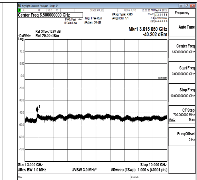
Band5-5MHz-16QAM-20625-1RB#0-3000~10000-PASS
