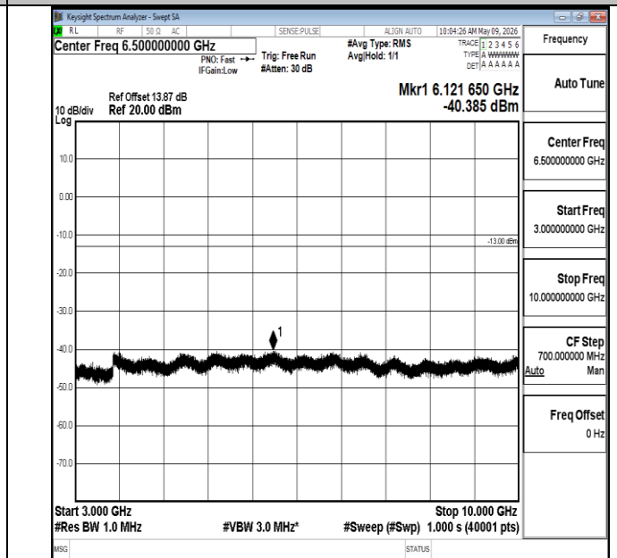
Band5-5MHz-16QAM-20525-1RB#0-3000~10000-PASS
