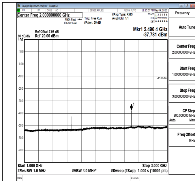
Band5-10MHz-16QAM-20525-1RB#0-1000~3000-PASS
