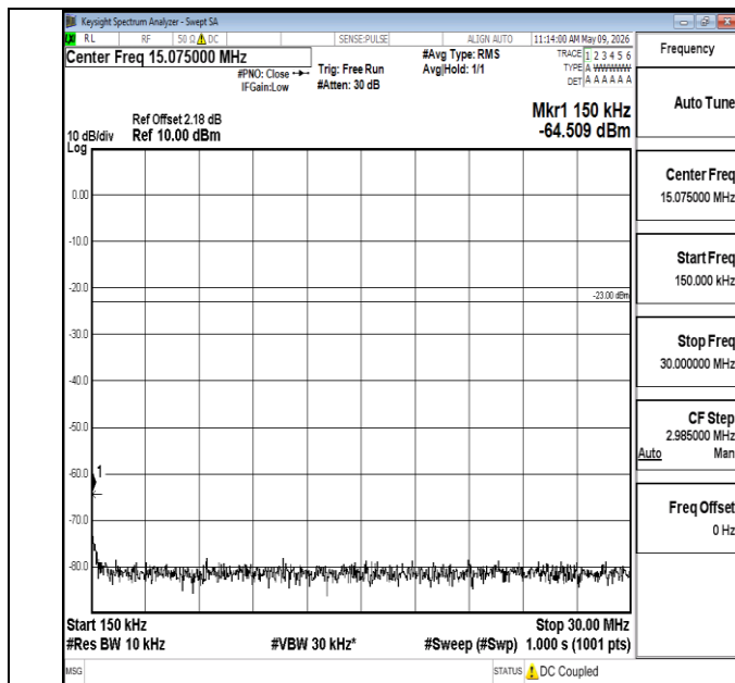
Band5-10MHz-16QAM-20450-1RB#0-0.15~30-PASS
