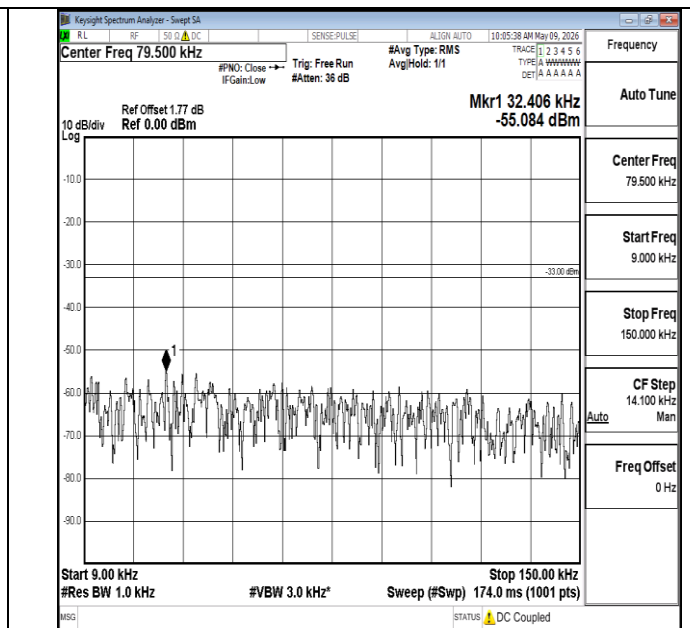
Band5-5MHz-16QAM-20625-1RB#0-0.009~0.15-PASS
