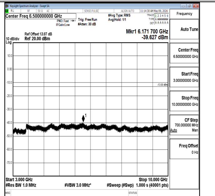
Band5-10MHz-16QAM-20450-1RB#0-3000~10000-PASS
