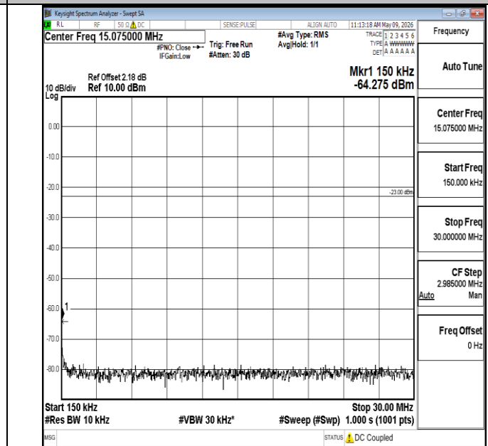
Band5-10MHz-QPSK-20450-1RB#0-0.15~30-PASS
