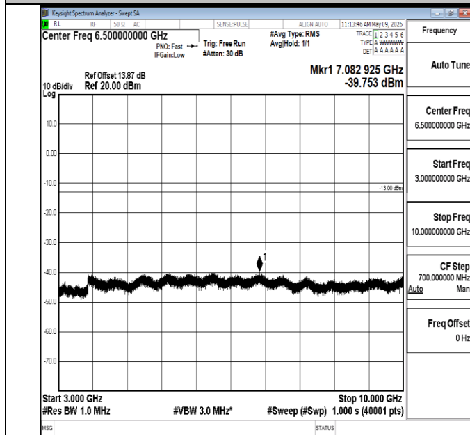
Band5-10MHz-QPSK-20450-1RB#0-3000~10000-PASS
