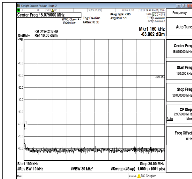
Band5-10MHz-16QAM-20600-1RB#0-0.15~30-PASS
