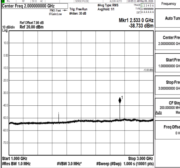
Band5-5MHz-QPSK-20625-1RB#0-1000~3000-PASS
