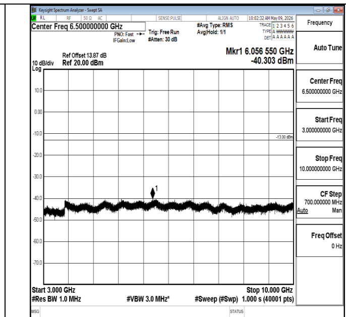
Band5-5MHz-16QAM-20425-1RB#0-3000~10000-PASS
