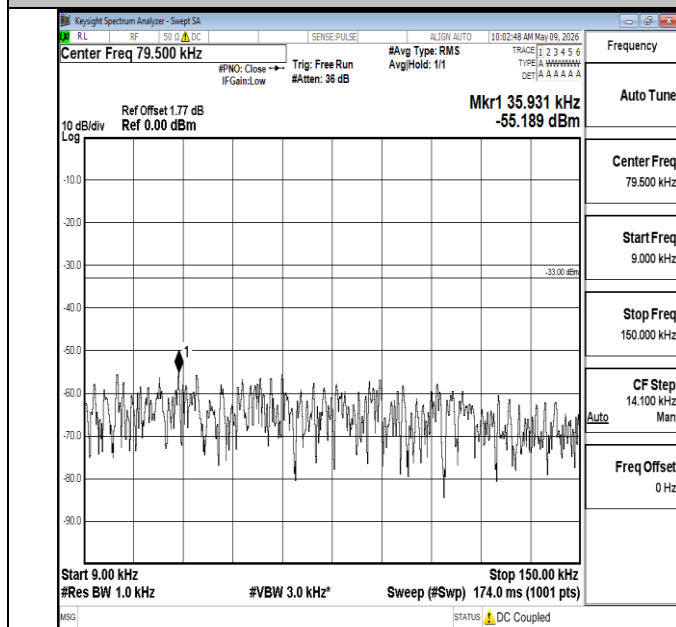
Band5-5MHz-QPSK-20525-1RB#0-0.009~0.15-PASS
