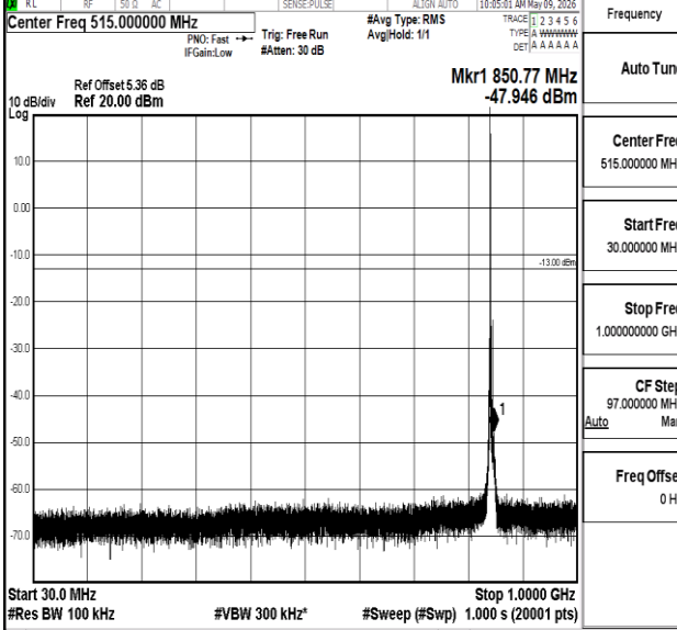
Band5-5MHz-QPSK-20625-1RB#0-30~1000-PASS
