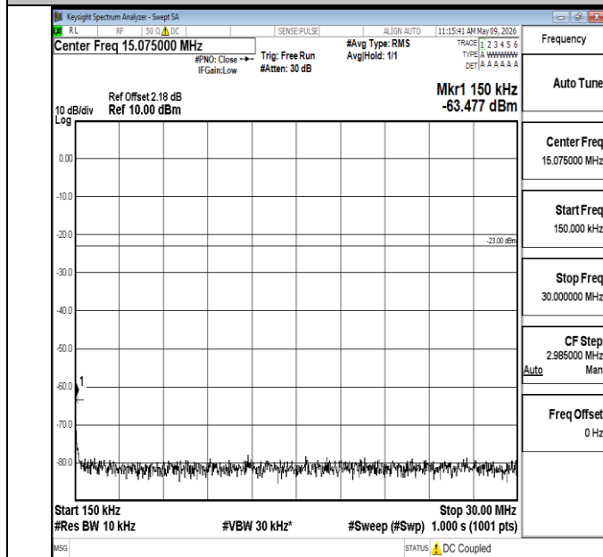
Band5-10MHz-16QAM-20525-1RB#0-0.15~30-PASS
