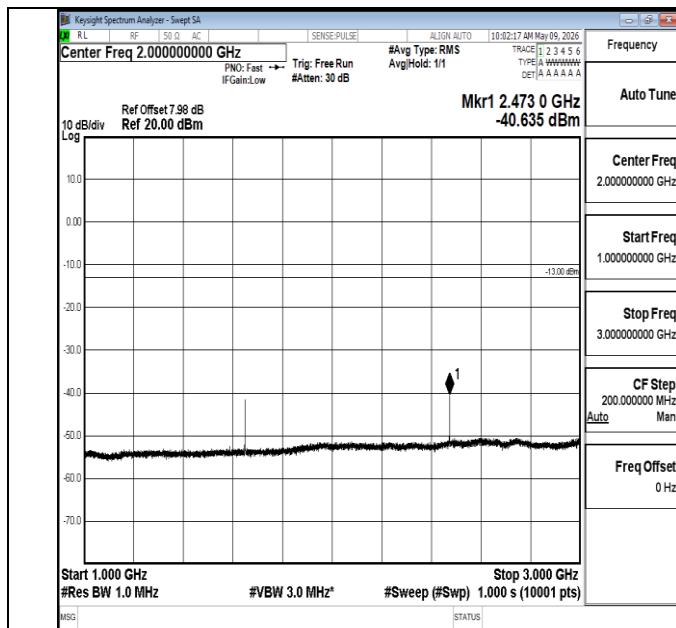
Band5-5MHz-16QAM-20425-1RB#0-1000~3000-PASS
