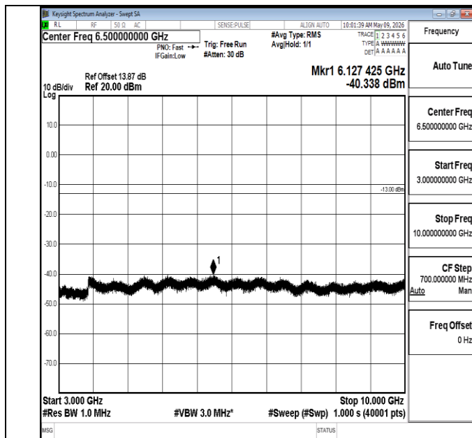
Band5-5MHz-QPSK-20425-1RB#0-3000~10000-PASS
