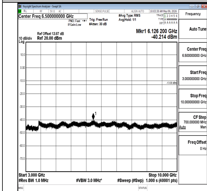
Band5-5MHz-QPSK-20525-1RB#0-3000~10000-PASS
