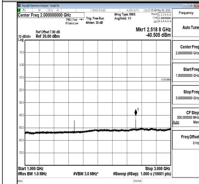
Band5-10MHz-16QAM-20600-1RB#0-1000~3000-PASS
