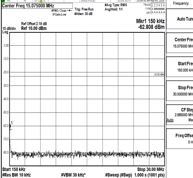
Band5-5MHz-QPSK-20625-1RB#0-0.15~30-PASS
