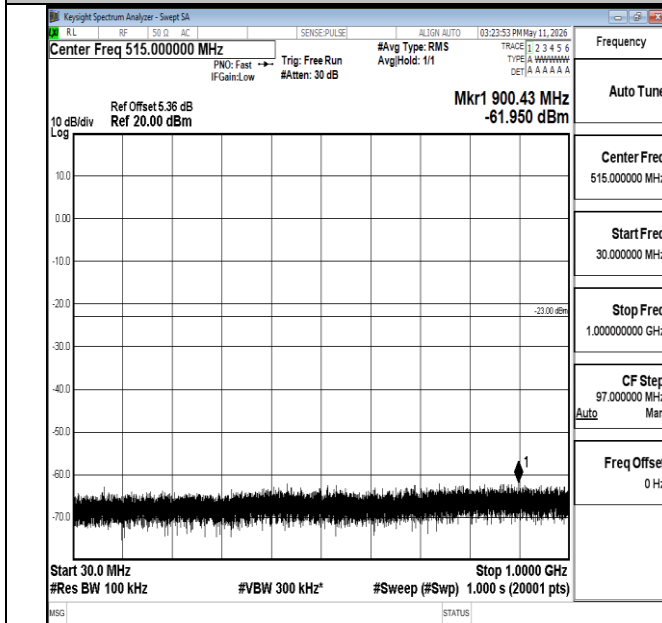
Band66-1.4MHz-QPSK-132665-1RB#0-30~1000-PASS
