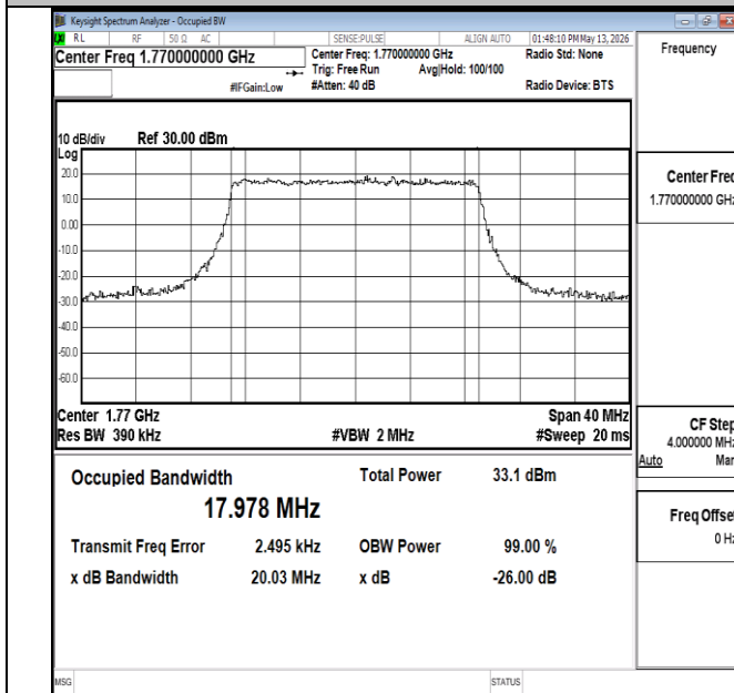
Band66-20MHz-QPSK-132572-100RB#0-PASS
