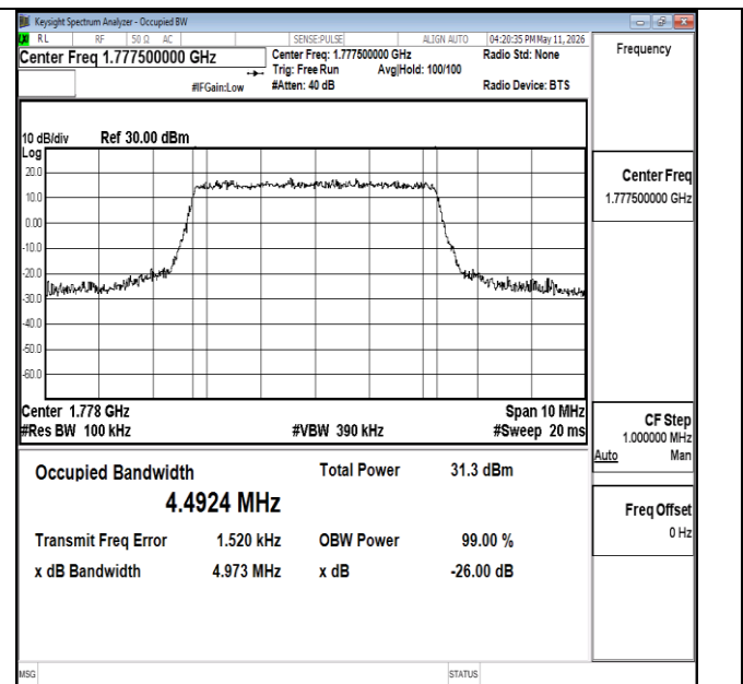
Band66-5MHz-16QAM-132647-25RB#0-PASS
