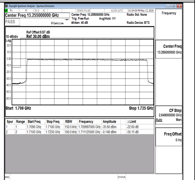
Band66-15MHz-QPSK-132047-75RB#0-PASS
