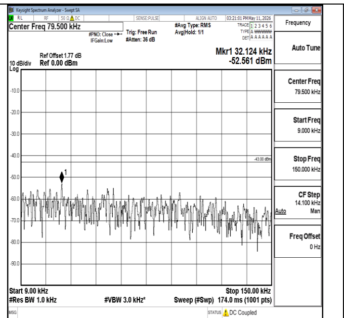
Band66-1.4MHz-16QAM-131979-1RB#0-0.009~0.15-PASS
