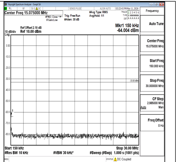
Band66-1.4MHz-QPSK-132665-1RB#0-0.15~30-PASS
