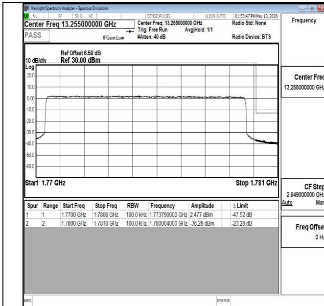
Band66-10MHz-QPSK-132622-50RB#0-PASS
