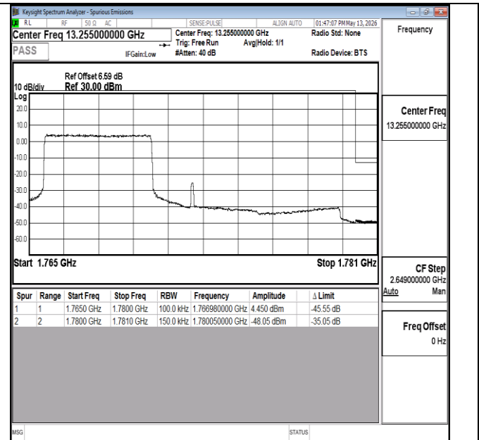
Band66-15MHz-QPSK-132597-27RB#0-PASS
