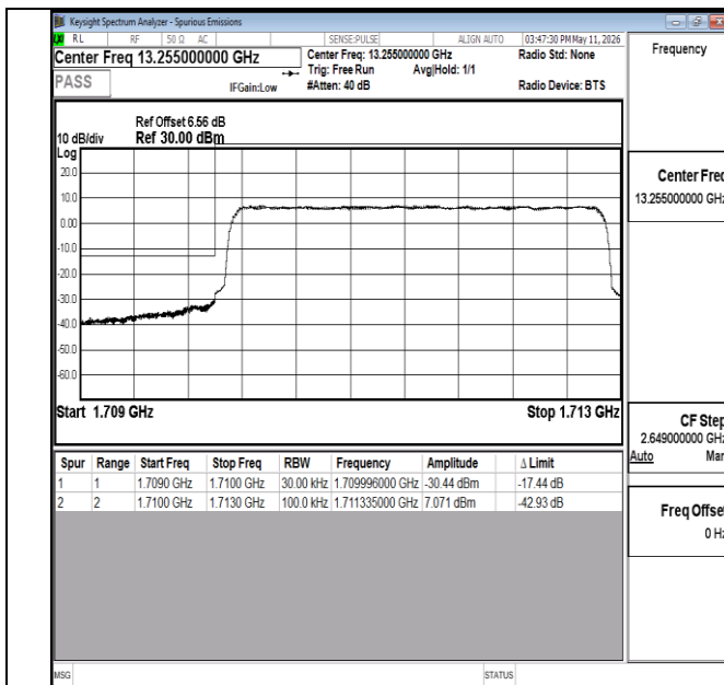
Band66-3MHz-QPSK-131987-15RB#0-PASS
