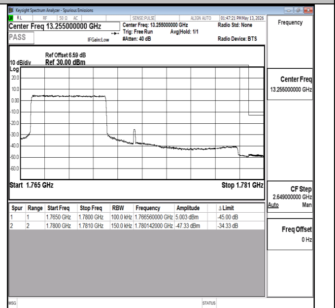
Band66-15MHz-16QAM-132597-27RB#0-PASS
