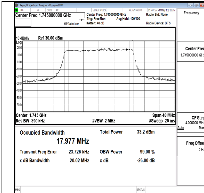
Band66-20MHz-QPSK-132322-100RB#0-PASS
