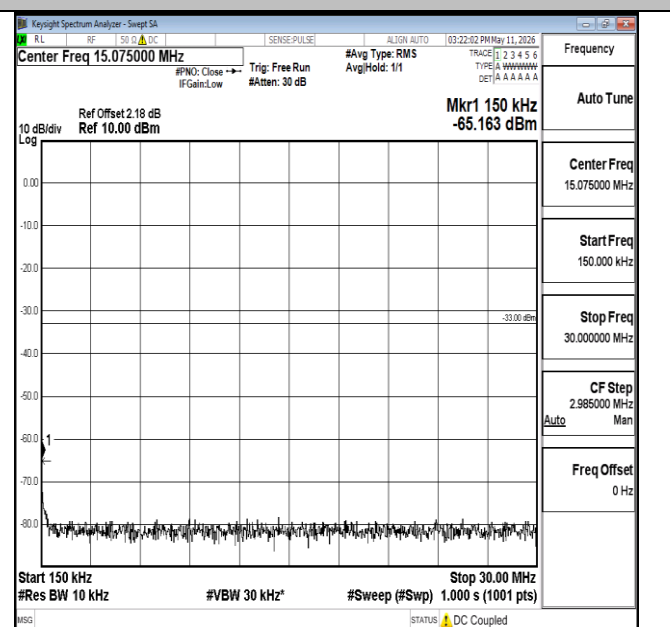
Band66-1.4MHz-QPSK-132322-1RB#0-0.15~30-PASS
