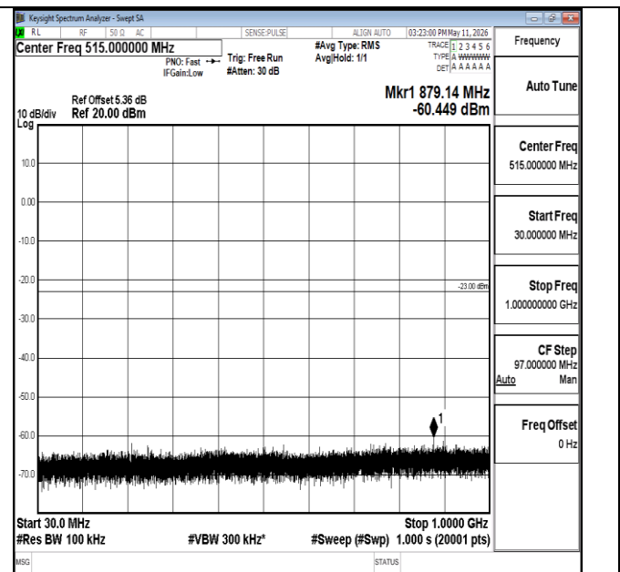
Band66-1.4MHz-16QAM-132322-1RB#0-30~1000-PASS
