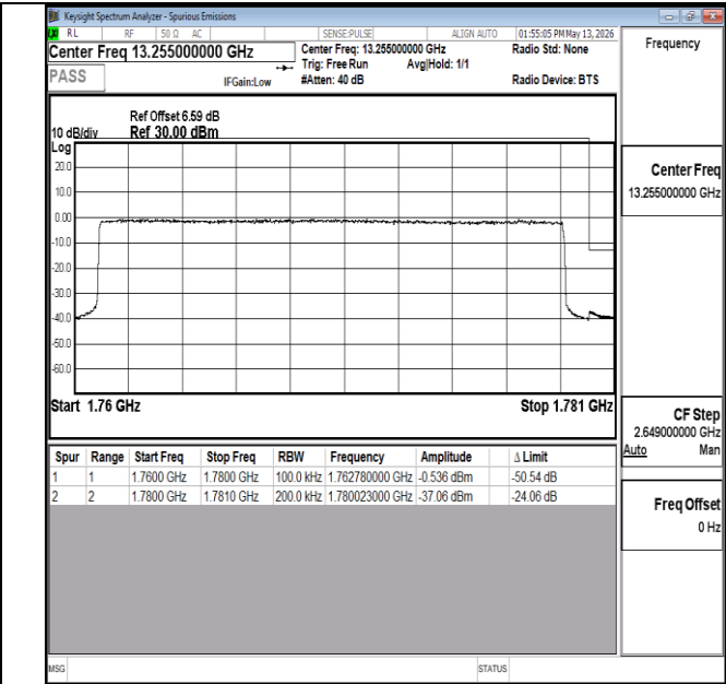
Band66-20MHz-QPSK-132572-100RB#0-PASS
