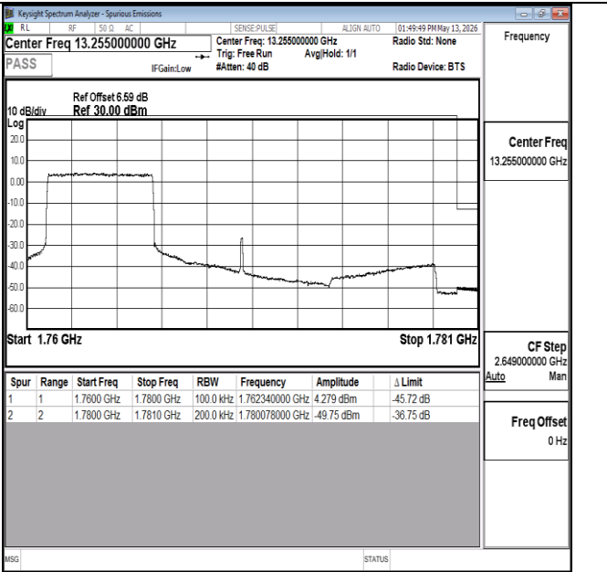
Band66-20MHz-16QAM-132572-27RB#0-PASS
