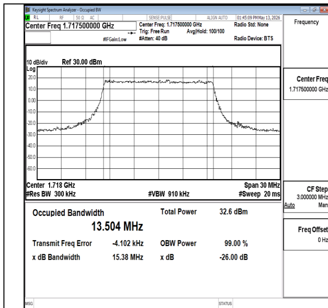
Band66-15MHz-QPSK-132047-75RB#0-PASS
