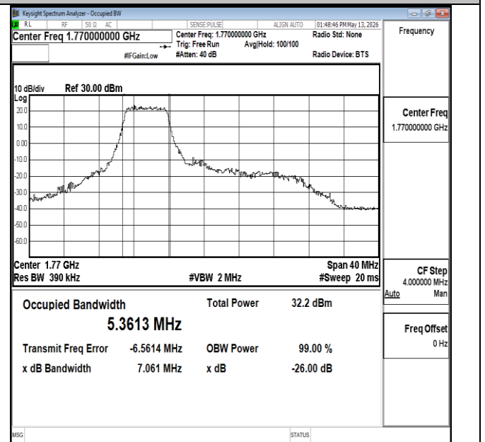
Band66-20MHz-16QAM-132572-27RB#0-PASS
