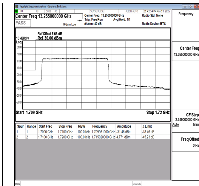
Band66-10MHz-QPSK-132022-27RB#0-PASS
