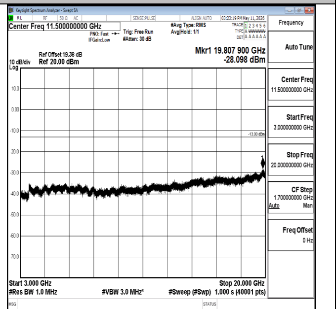
Band66-1.4MHz-16QAM-132322-1RB#0-3000~20000-PASS
