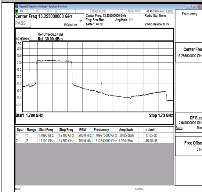
Band66-20MHz-16QAM-132072-27RB#0-PASS
