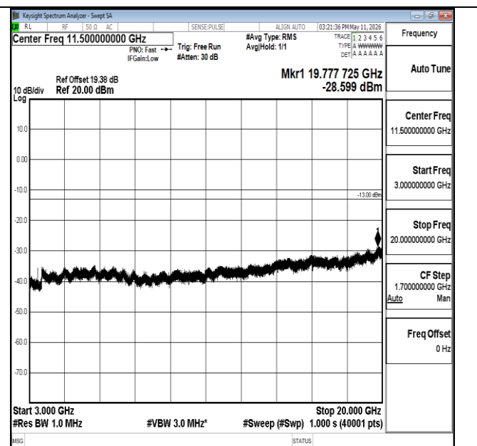
Band66-1.4MHz-16QAM-131979-1RB#0-3000~20000-PASS
