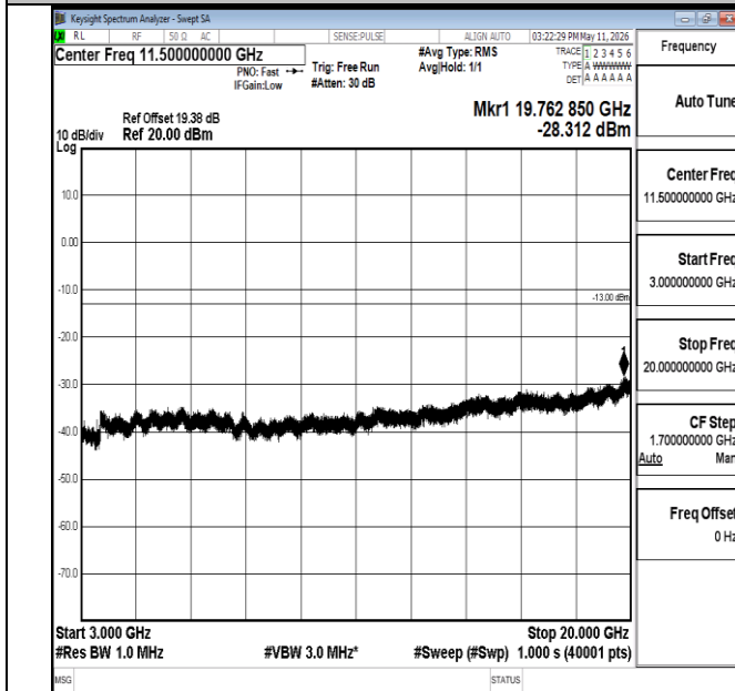
Band66-1.4MHz-QPSK-132322-1RB#0-3000~20000-PASS
