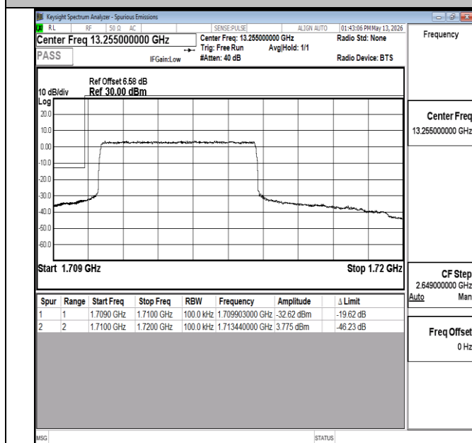
Band66-10MHz-16QAM-132022-27RB#0-PASS
