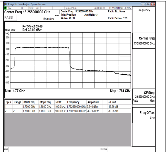
Band66-10MHz-16QAM-132622-27RB#0-PASS
