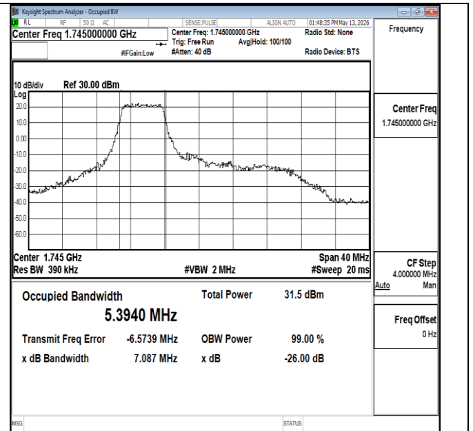
Band66-20MHz-16QAM-132322-27RB#0-PASS
