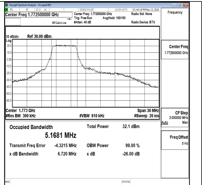
Band66-15MHz-16QAM-132597-27RB#0-PASS
