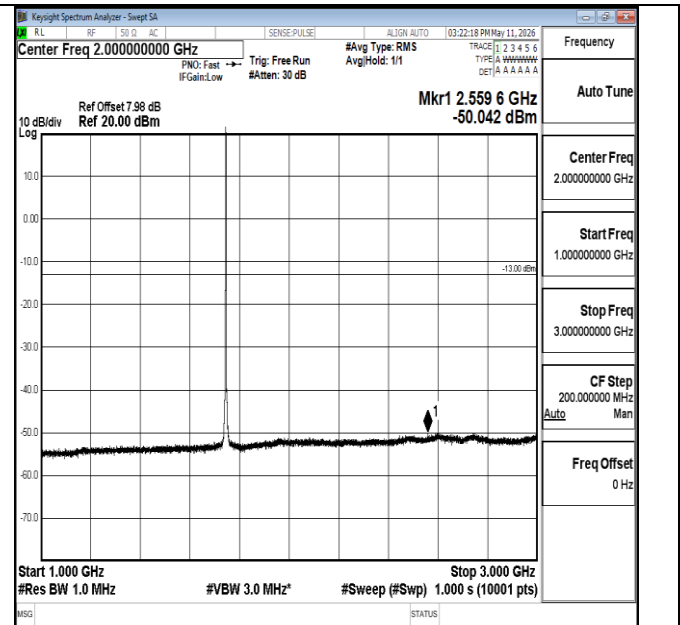
Band66-1.4MHz-QPSK-132322-1RB#0-1000~3000-PASS
