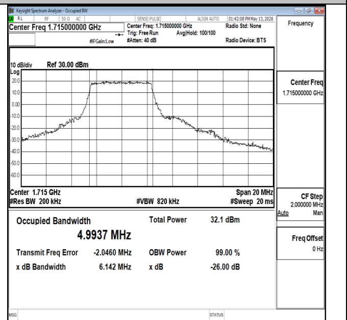
Band66-10MHz-16QAM-132022-27RB#0-PASS
