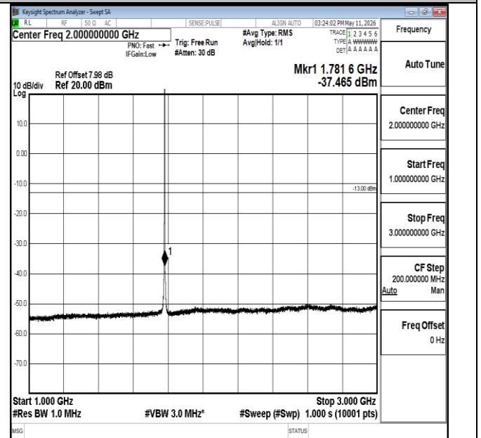
Band66-1.4MHz-QPSK-132665-1RB#0-1000~3000-PASS
