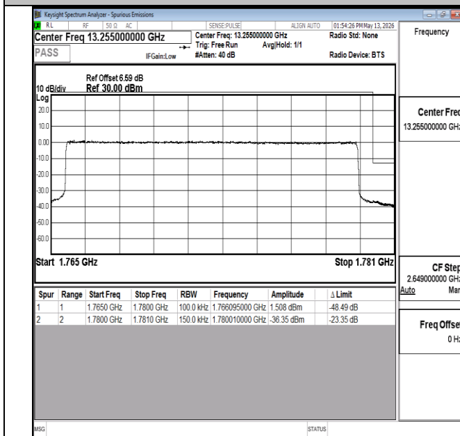
Band66-15MHz-QPSK-132597-75RB#0-PASS
