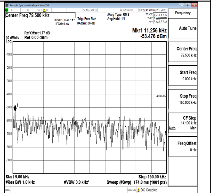
Band66-1.4MHz-16QAM-132322-1RB#0-0.009~0.15-PASS
