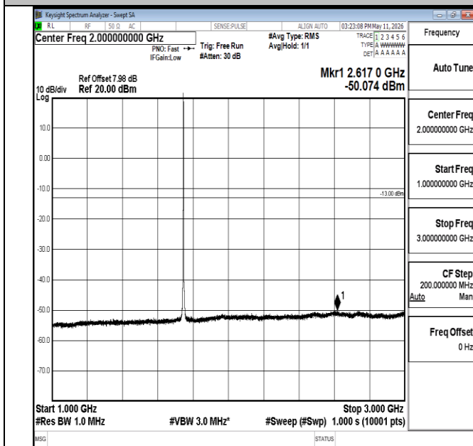
Band66-1.4MHz-16QAM-132322-1RB#0-1000~3000-PASS
