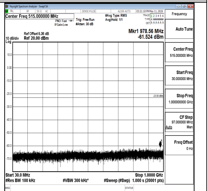
Band66-1.4MHz-16QAM-131979-1RB#0-30~1000-PASS
