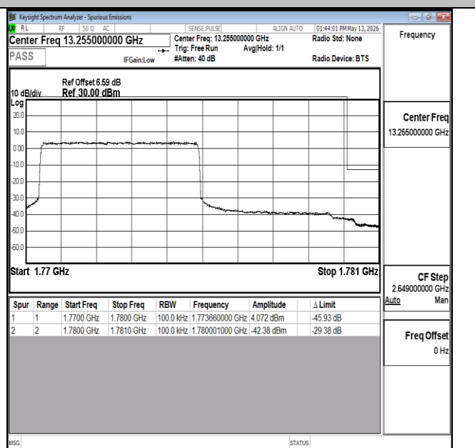
Band66-10MHz-QPSK-132622-27RB#0-PASS
