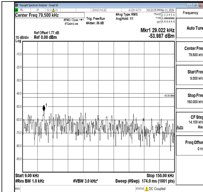
Band66-1.4MHz-QPSK-132665-1RB#0-0.009~0.15-PASS
