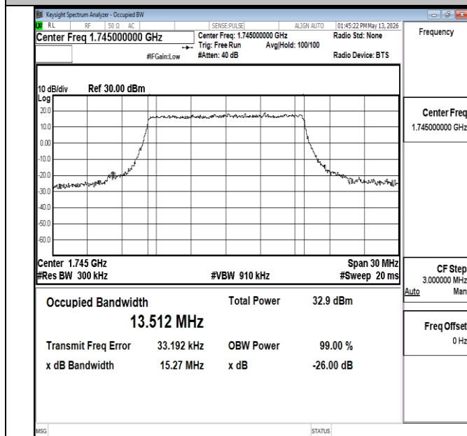
Band66-15MHz-QPSK-132322-75RB#0-PASS
