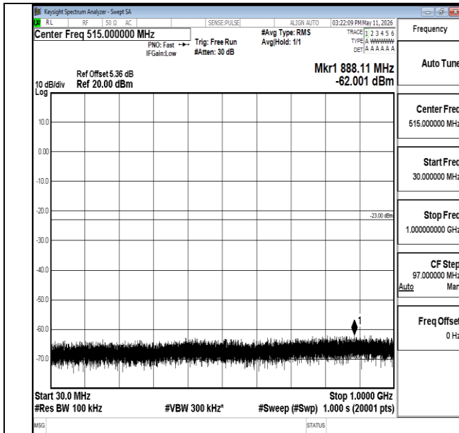
Band66-1.4MHz-QPSK-132322-1RB#0-30~1000-PASS
