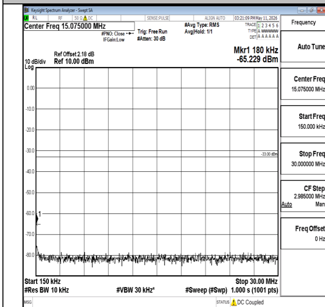
Band66-1.4MHz-16QAM-131979-1RB#0-0.15~30-PASS
