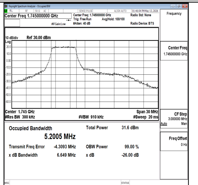
Band66-15MHz-16QAM-132322-27RB#0-PASS
