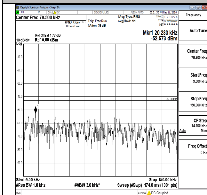
Band66-1.4MHz-QPSK-132322-1RB#0-0.009~0.15-PASS
