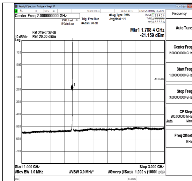
Band66-1.4MHz-16QAM-131979-1RB#0-1000~3000-PASS
