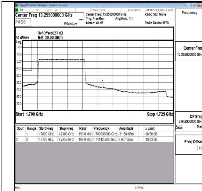
Band66-15MHz-16QAM-132047-27RB#0-PASS
