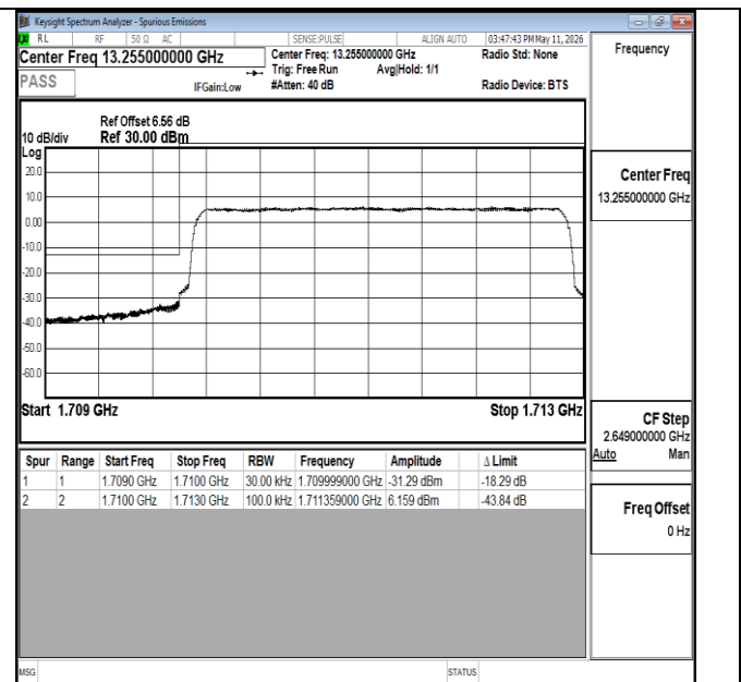
Band66-3MHz-16QAM-131987-15RB#0-PASS
