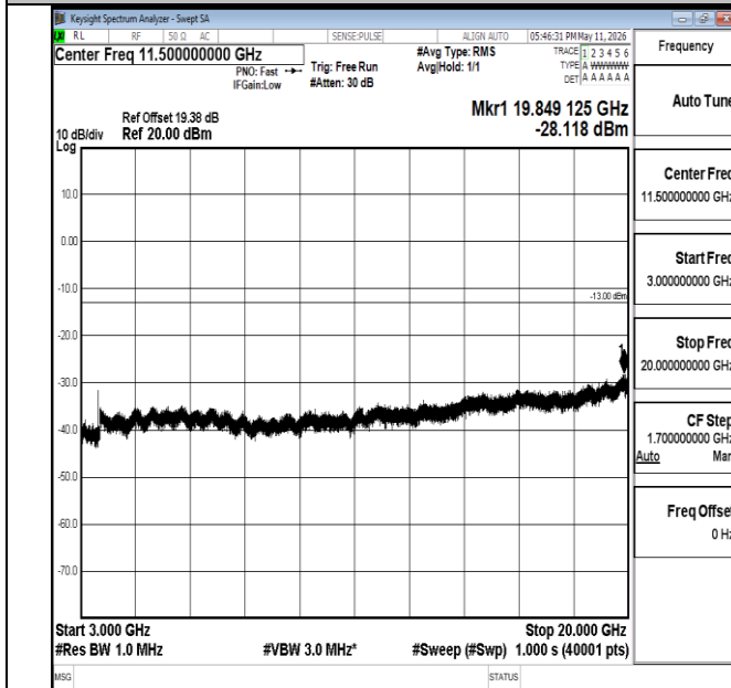
Band66-10MHz-QPSK-132622-1RB#0-3000~20000-PASS
