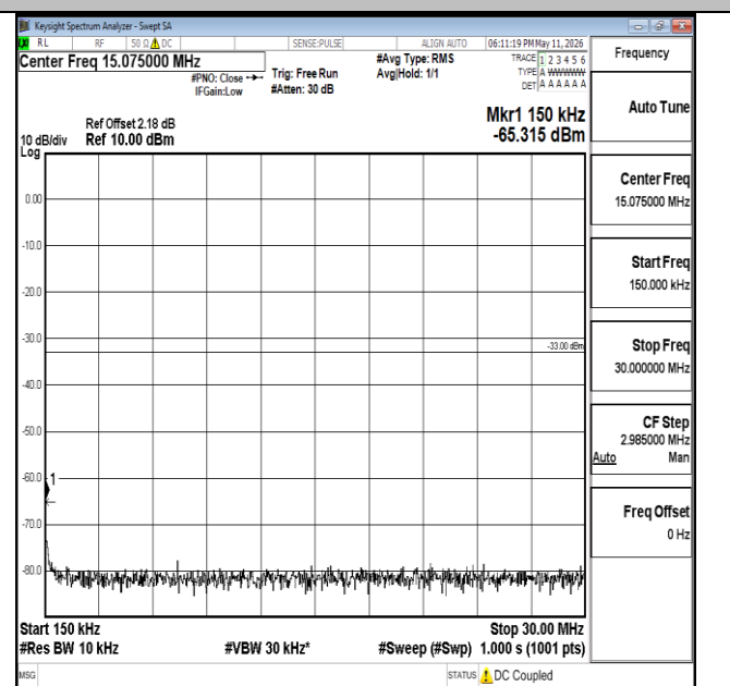
Band66-15MHz-QPSK-132322-1RB#0-0.15~30-PASS
