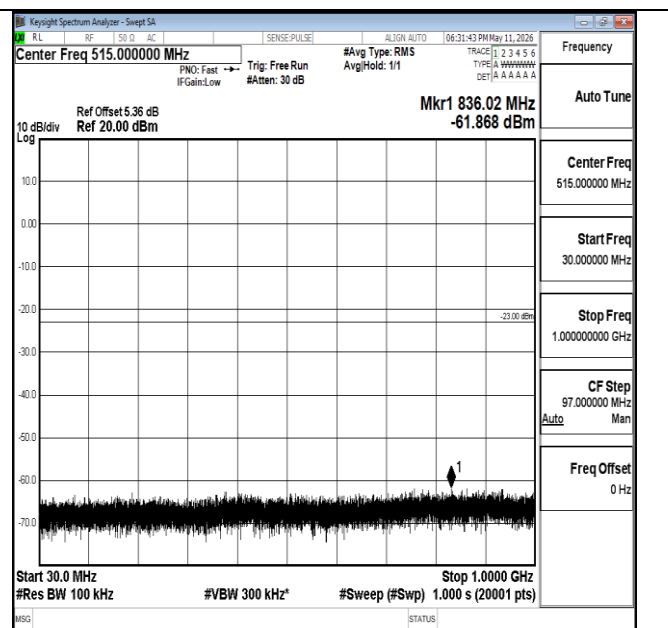
Band66-20MHz-16QAM-132572-1RB#0-30~1000-PASS
