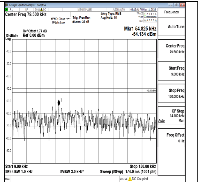
Band66-15MHz-16QAM-132597-1RB#0-0.009~0.15-PASS
