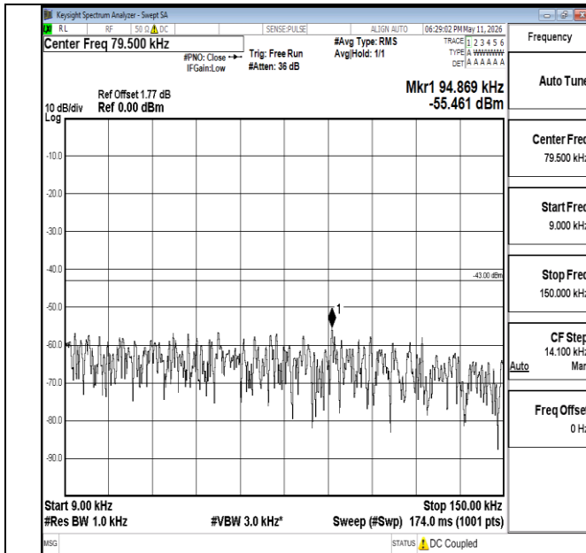
Band66-20MHz-QPSK-132322-1RB#0-0.009~0.15-PASS
