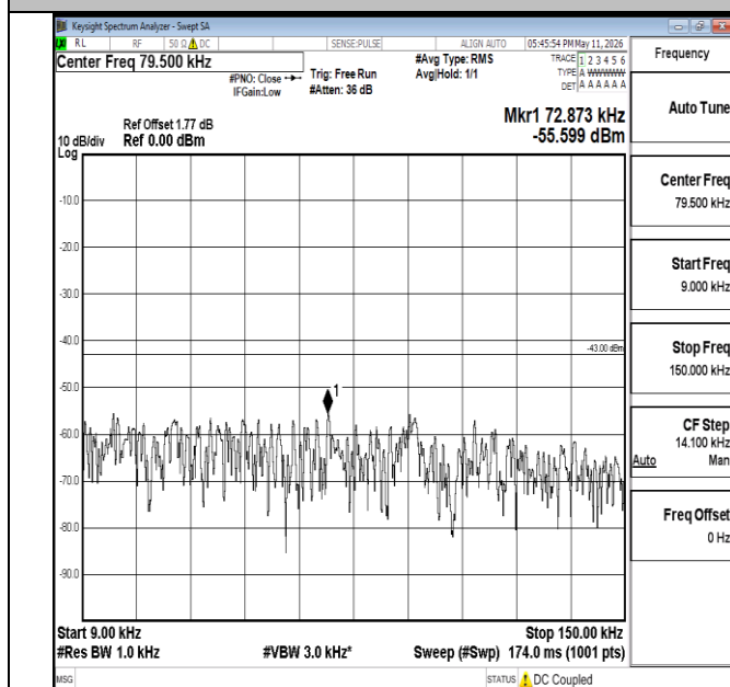
Band66-10MHz-QPSK-132622-1RB#0-0.009~0.15-PASS
