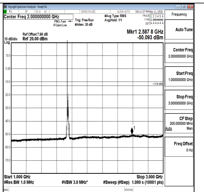
Band66-15MHz-QPSK-132322-1RB#0-1000~3000-PASS
