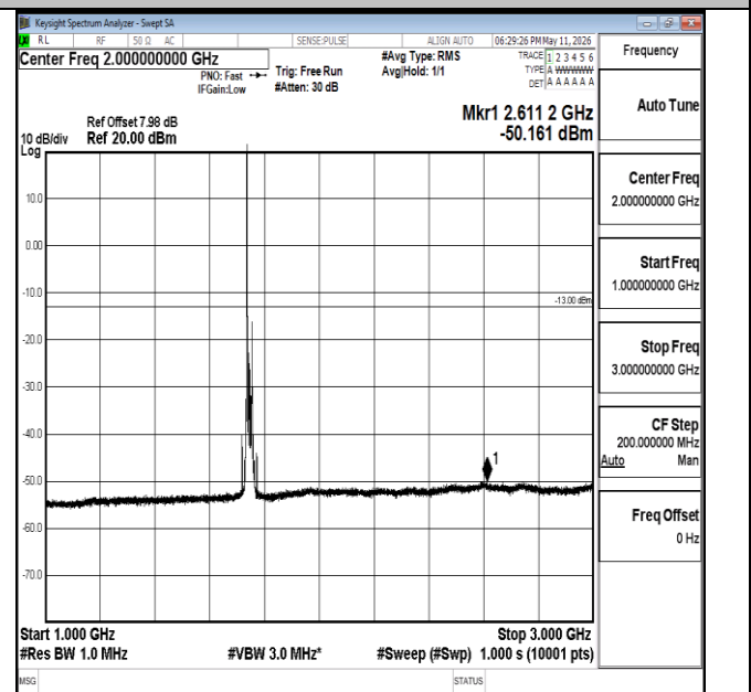
Band66-20MHz-QPSK-132322-1RB#0-1000~3000-PASS
