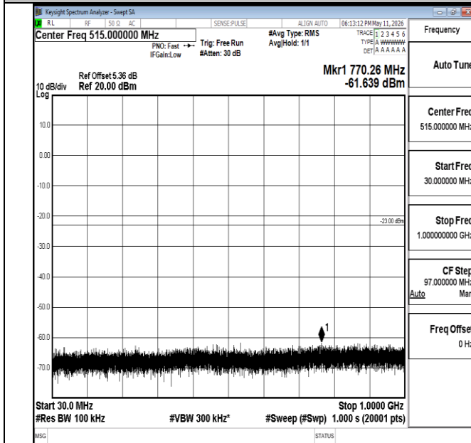
Band66-15MHz-QPSK-132597-1RB#0-30~1000-PASS
