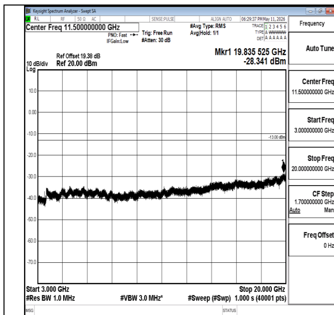
Band66-20MHz-QPSK-132322-1RB#0-3000~20000-PASS
