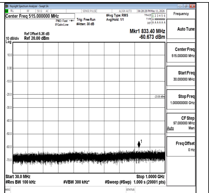
Band66-20MHz-16QAM-132072-1RB#0-30~1000-PASS
