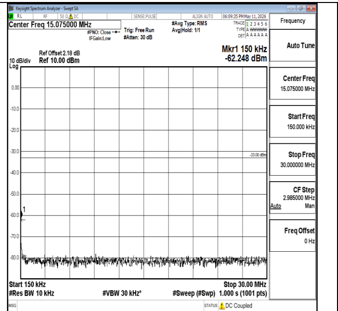
Band66-15MHz-QPSK-132047-1RB#0-0.15~30-PASS
