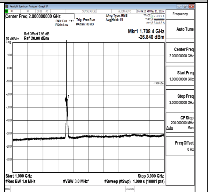
Band66-15MHz-QPSK-132047-1RB#0-1000~3000-PASS
