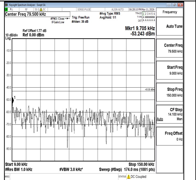
Band66-20MHz-16QAM-132072-1RB#0-0.009~0.15-PASS
