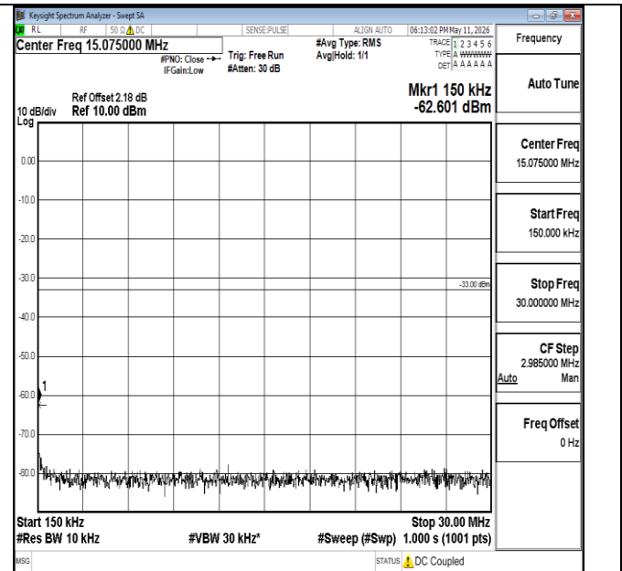
Band66-15MHz-QPSK-132597-1RB#0-0.15~30-PASS
