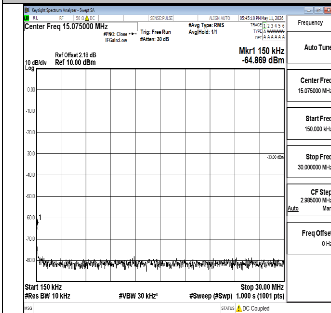
Band66-10MHz-16QAM-132322-1RB#0-0.15~30-PASS
