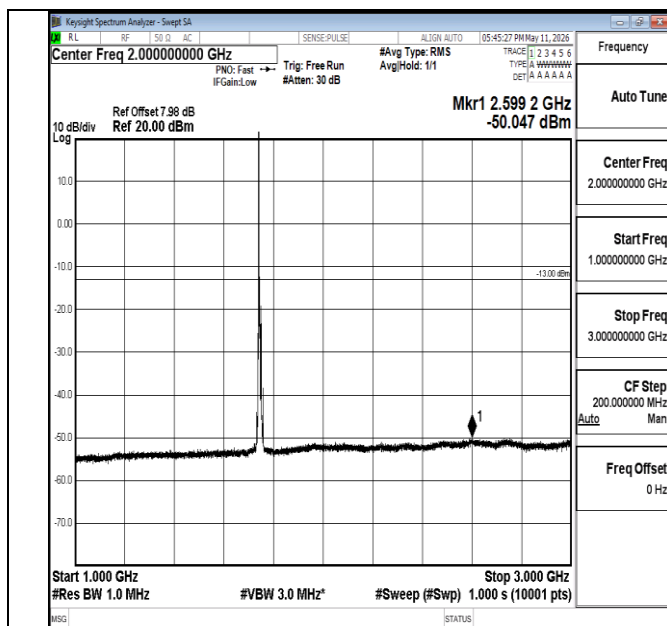
Band66-10MHz-16QAM-132322-1RB#0-1000~3000-PASS
