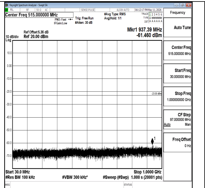
Band66-15MHz-16QAM-132322-1RB#0-30~1000-PASS
