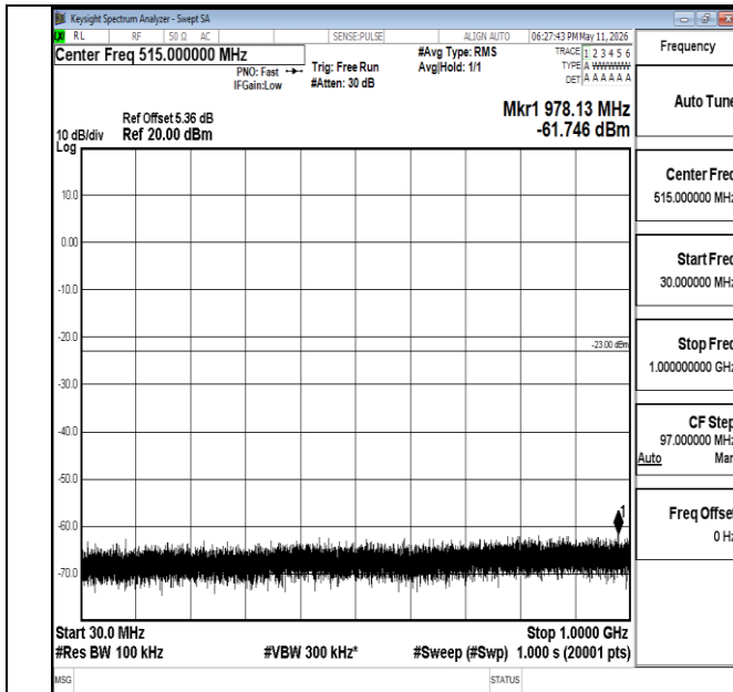
Band66-20MHz-QPSK-132072-1RB#0-30~1000-PASS
