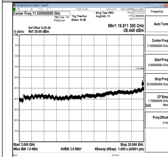
Band66-15MHz-QPSK-132322-1RB#0-3000~20000-PASS
