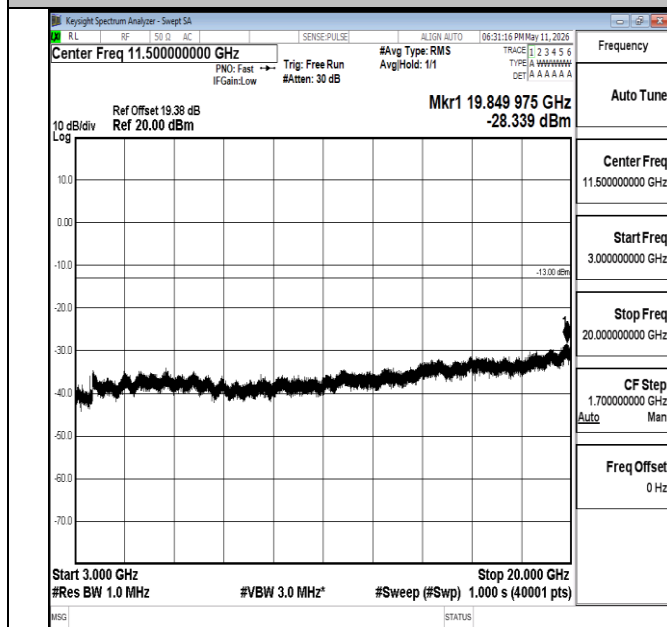
Band66-20MHz-QPSK-132572-1RB#0-3000~20000-PASS
