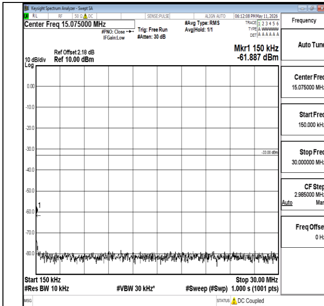
Band66-15MHz-16QAM-132322-1RB#0-0.15~30-PASS
