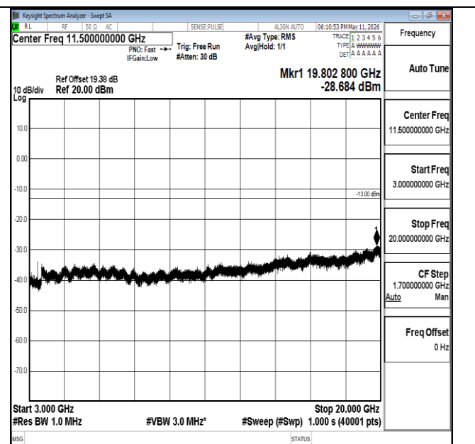
Band66-15MHz-16QAM-132047-1RB#0-3000~20000-PASS
