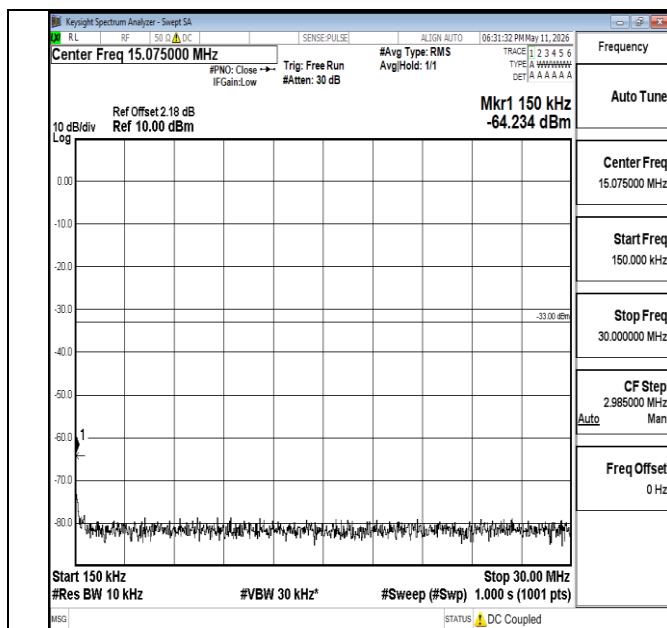
Band66-20MHz-16QAM-132572-1RB#0-0.15~30-PASS
