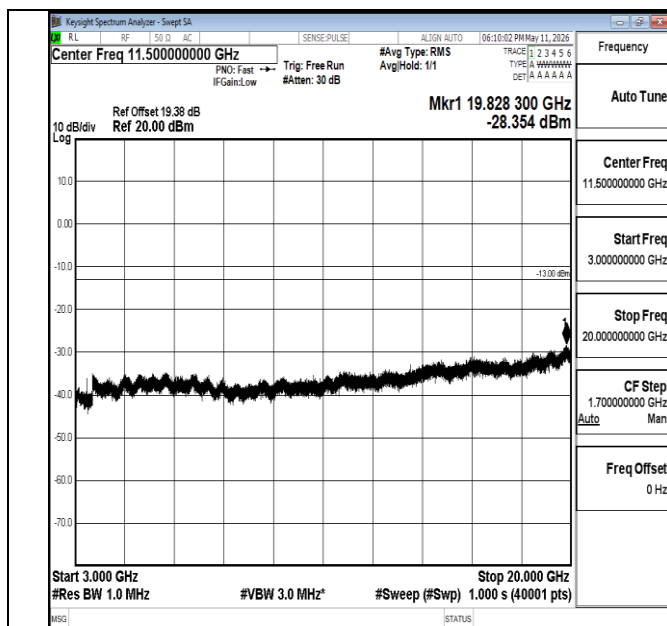
Band66-15MHz-QPSK-132047-1RB#0-3000~20000-PASS
