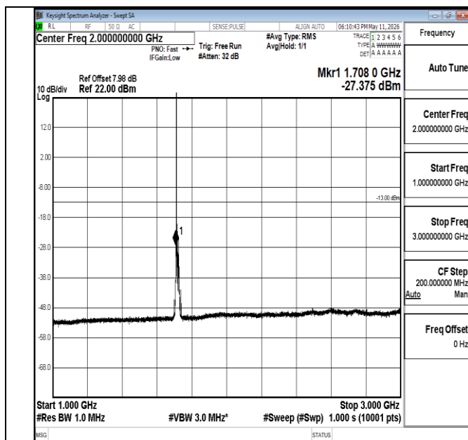
Band66-15MHz-16QAM-132047-1RB#0-1000~3000-PASS
