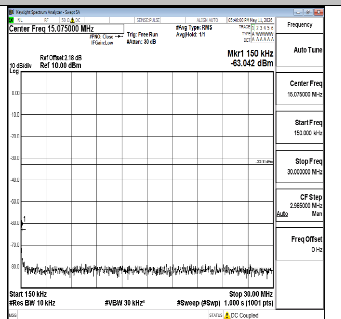
Band66-10MHz-QPSK-132622-1RB#0-0.15~30-PASS
