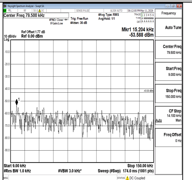
Band66-15MHz-16QAM-132322-1RB#0-0.009~0.15-PASS
