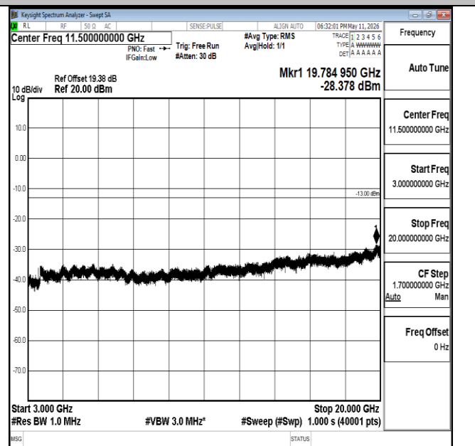
Band66-20MHz-16QAM-132572-1RB#0-3000~20000-PASS
