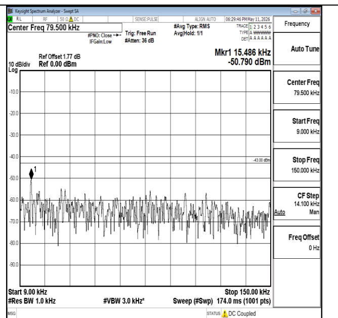
Band66-20MHz-16QAM-132322-1RB#0-0.009~0.15-PASS
