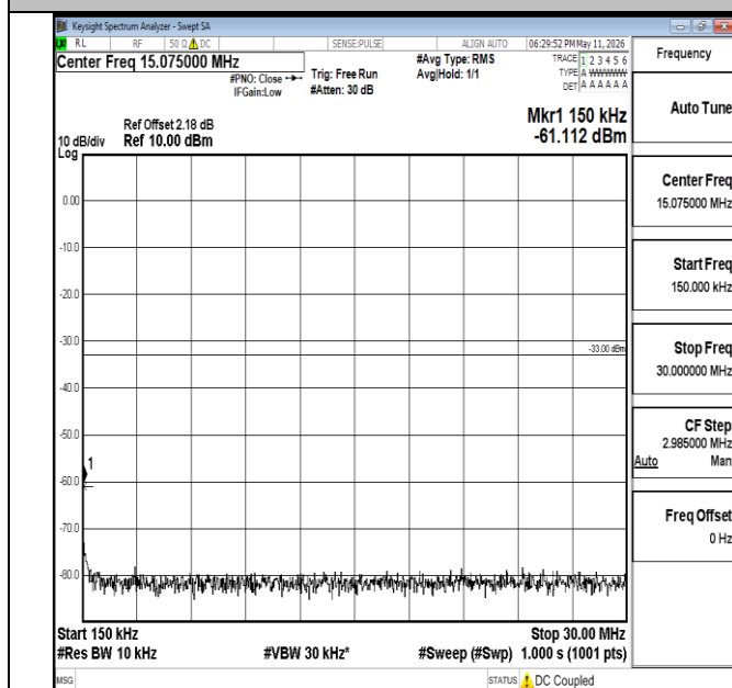
Band66-20MHz-16QAM-132322-1RB#0-0.15~30-PASS
