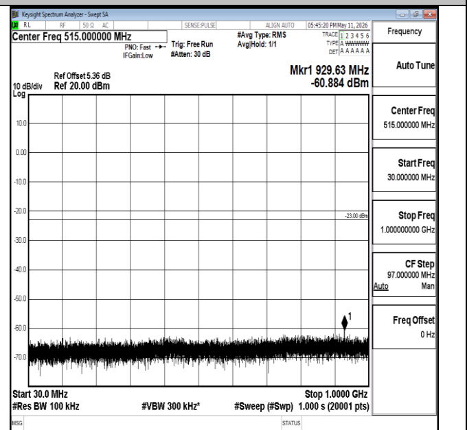
Band66-10MHz-16QAM-132322-1RB#0-30~1000-PASS
