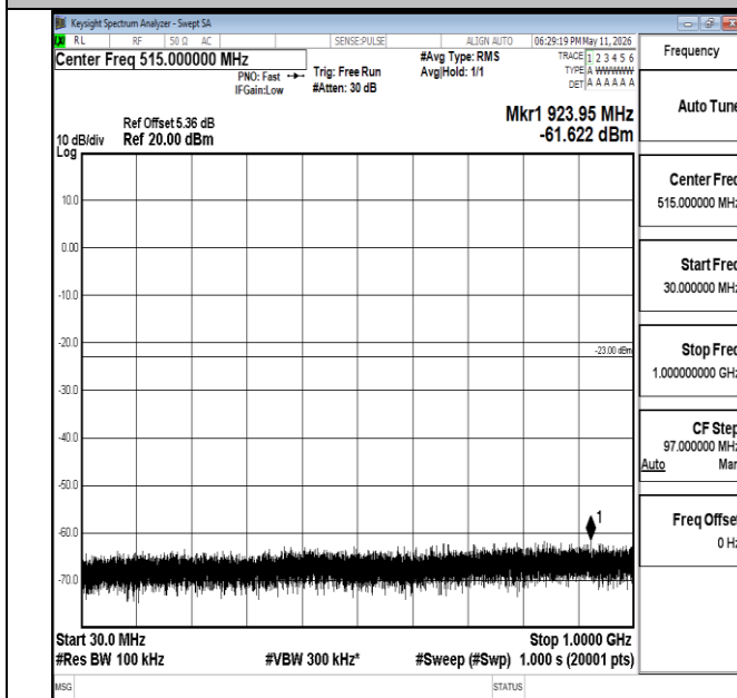
Band66-20MHz-QPSK-132322-1RB#0-30~1000-PASS
