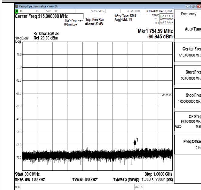
Band66-15MHz-QPSK-132047-1RB#0-30~1000-PASS
