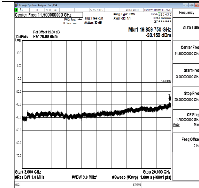
Band66-10MHz-QPSK-132322-1RB#0-3000~20000-PASS
