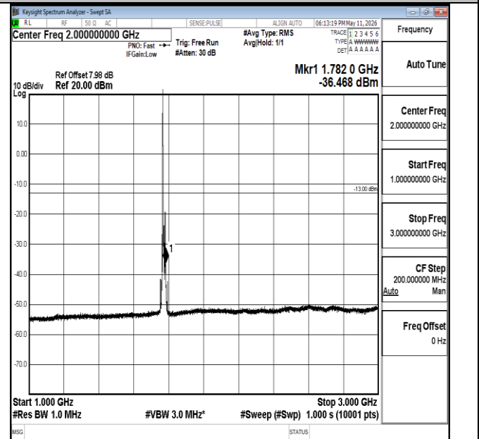
Band66-15MHz-QPSK-132597-1RB#0-1000~3000-PASS
