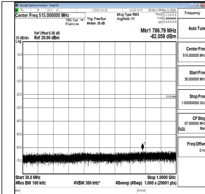
Band66-10MHz-QPSK-132622-1RB#0-30~1000-PASS
