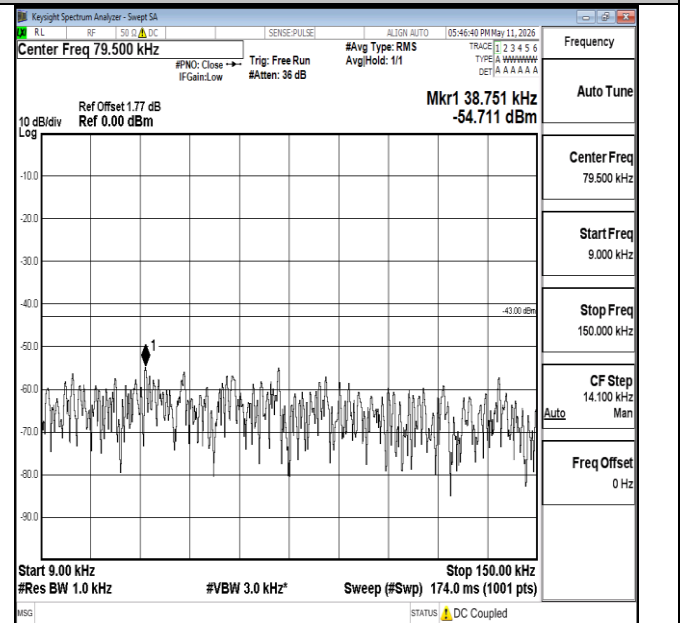
Band66-10MHz-16QAM-132622-1RB#0-0.009~0.15-PASS
