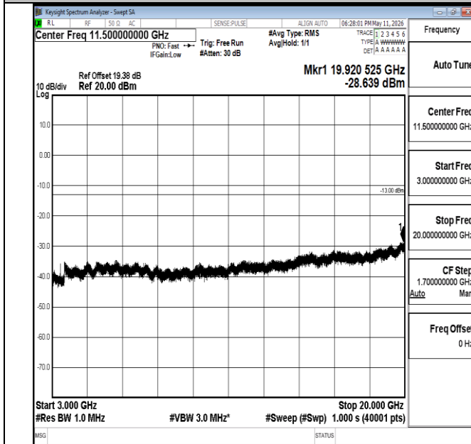
Band66-20MHz-QPSK-132072-1RB#0-3000~20000-PASS
