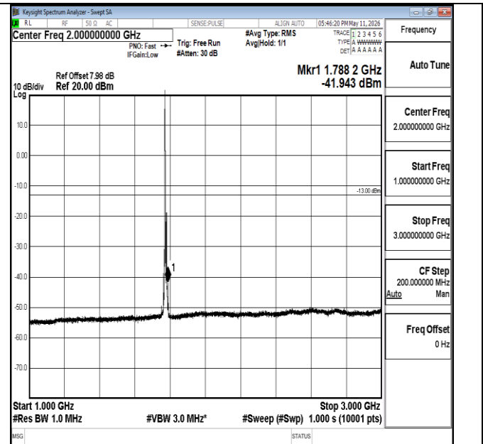
Band66-10MHz-QPSK-132622-1RB#0-1000~3000-PASS
