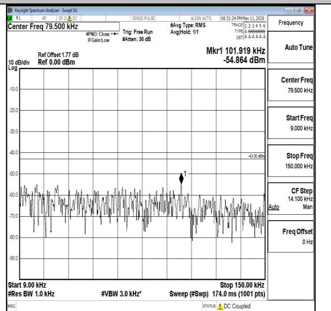
Band66-20MHz-16QAM-132572-1RB#0-0.009~0.15-PASS
