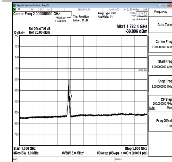
Band66-20MHz-16QAM-132572-1RB#0-1000~3000-PASS
