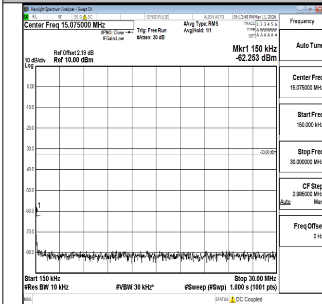
Band66-15MHz-16QAM-132597-1RB#0-0.15~30-PASS
