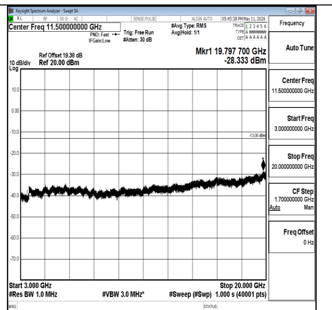
Band66-10MHz-16QAM-132322-1RB#0-3000~20000-PASS
