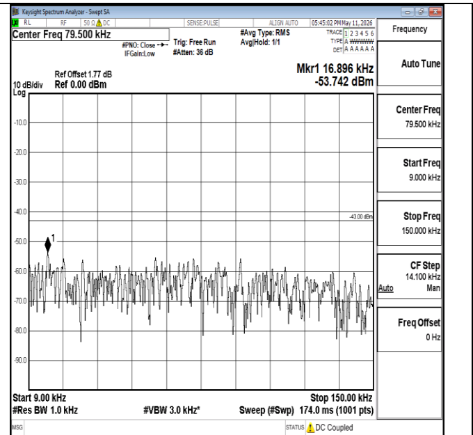
Band66-10MHz-16QAM-132322-1RB#0-0.009~0.15-PASS
