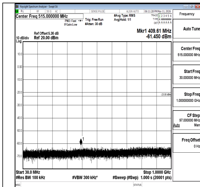
Band66-15MHz-QPSK-132322-1RB#0-30~1000-PASS
