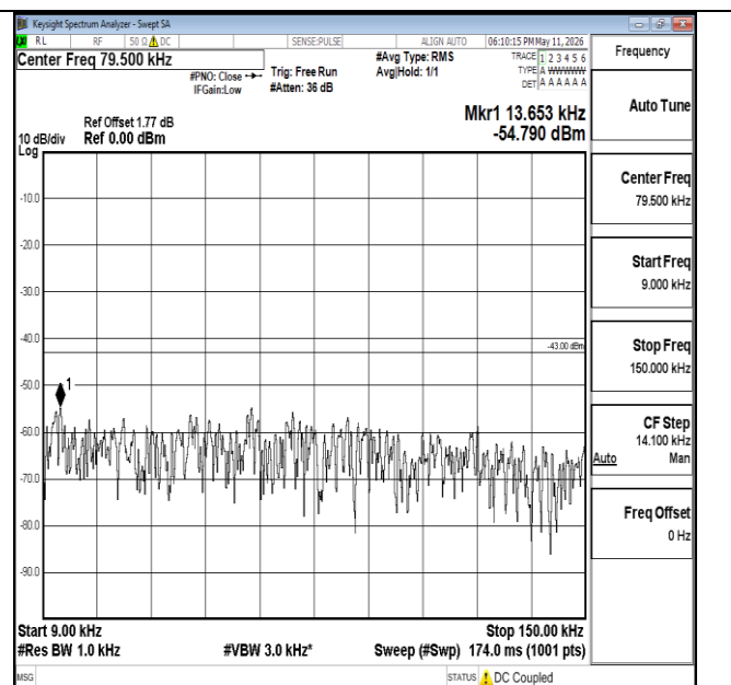
Band66-15MHz-16QAM-132047-1RB#0-0.009~0.15-PASS
