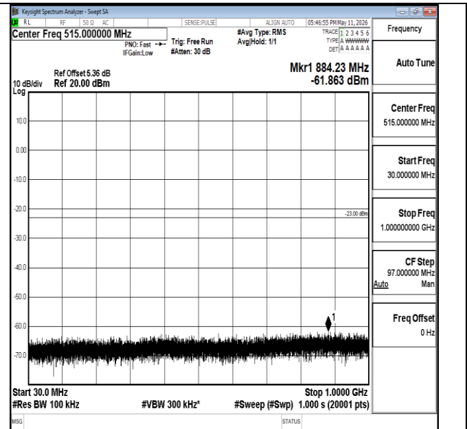
Band66-10MHz-16QAM-132622-1RB#0-30~1000-PASS
