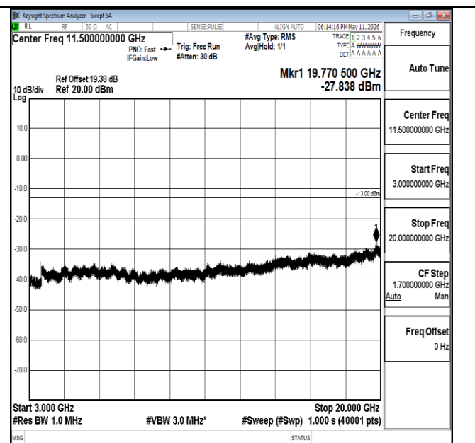
Band66-15MHz-16QAM-132597-1RB#0-3000~20000-PASS
