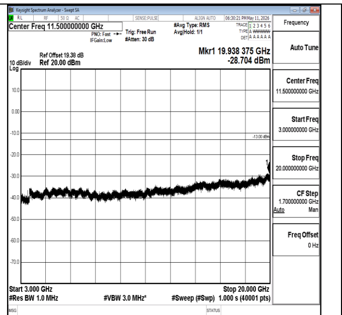
Band66-20MHz-16QAM-132322-1RB#0-3000~20000-PASS
