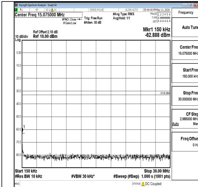
Band66-10MHz-16QAM-132622-1RB#0-0.15~30-PASS
