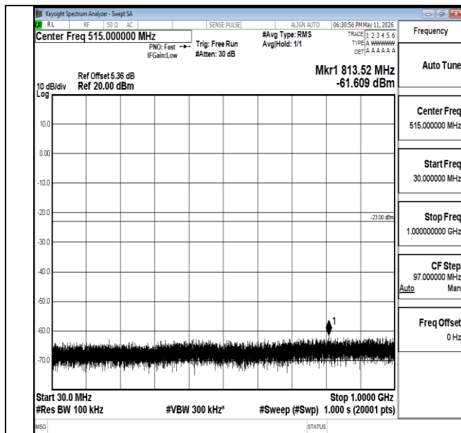
Band66-20MHz-QPSK-132572-1RB#0-30~1000-PASS
