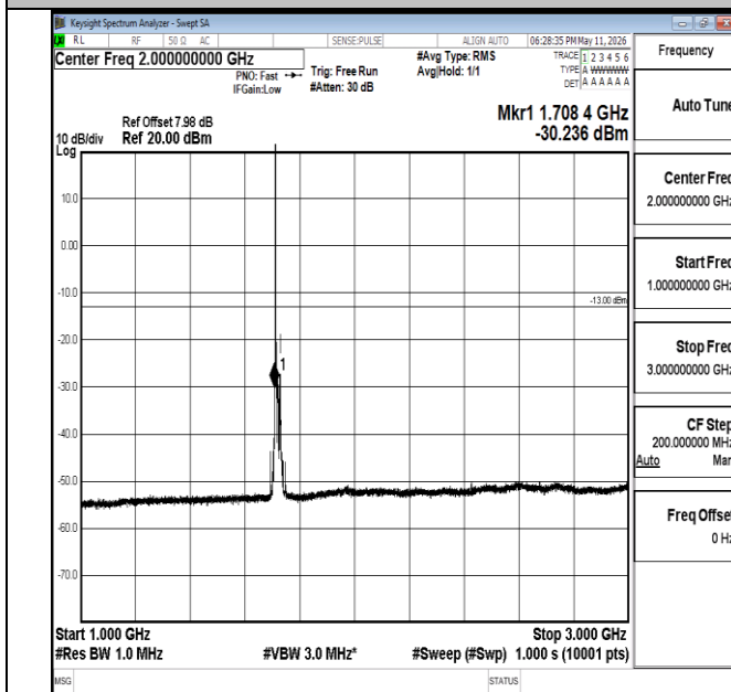
Band66-20MHz-16QAM-132072-1RB#0-1000~3000-PASS
