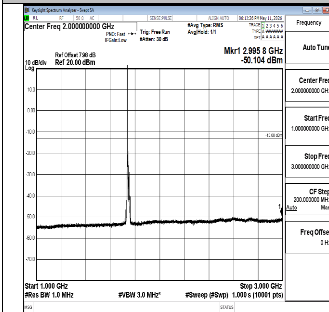
Band66-15MHz-16QAM-132322-1RB#0-1000~3000-PASS
