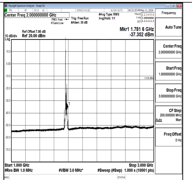
Band66-20MHz-QPSK-132572-1RB#0-1000~3000-PASS
