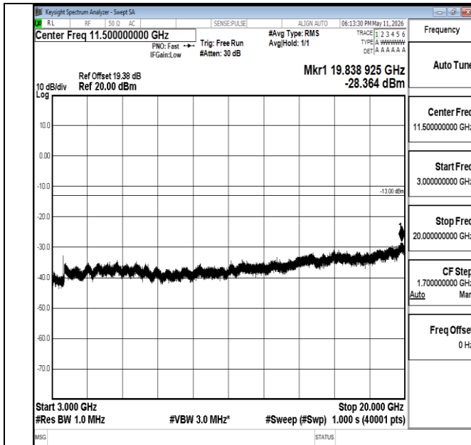
Band66-15MHz-QPSK-132597-1RB#0-3000~20000-PASS
