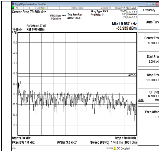
Band66-15MHz-QPSK-132047-1RB#0-0.009~0.15-PASS
