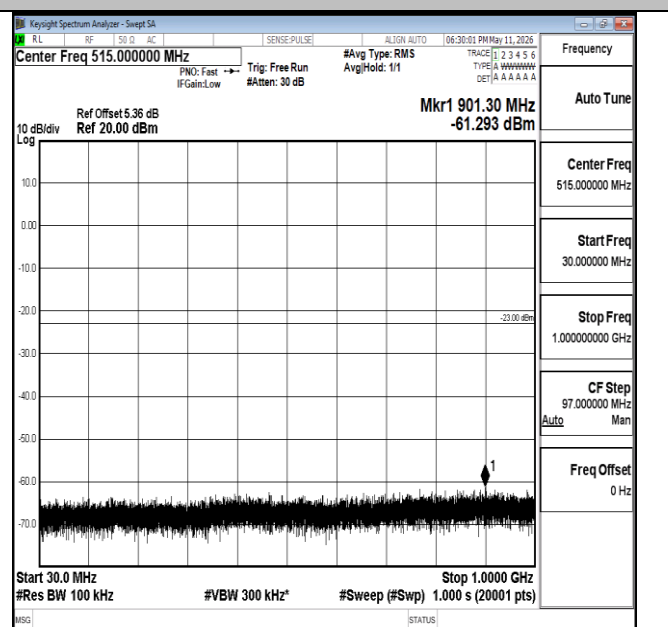
Band66-20MHz-16QAM-132322-1RB#0-30~1000-PASS
