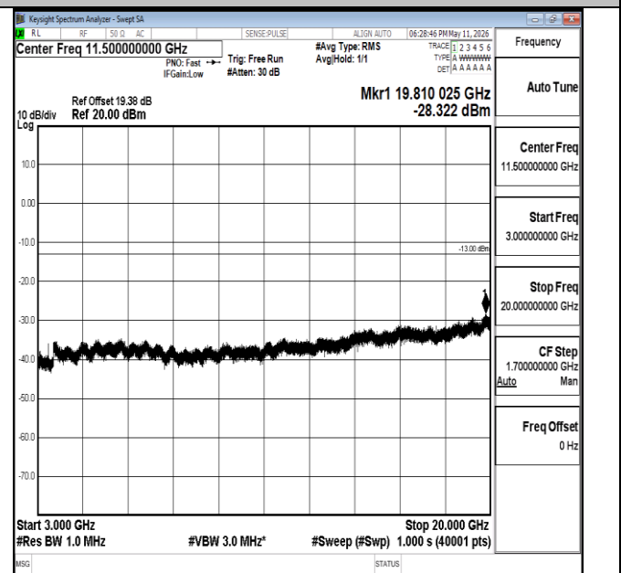
Band66-20MHz-16QAM-132072-1RB#0-3000~20000-PASS
