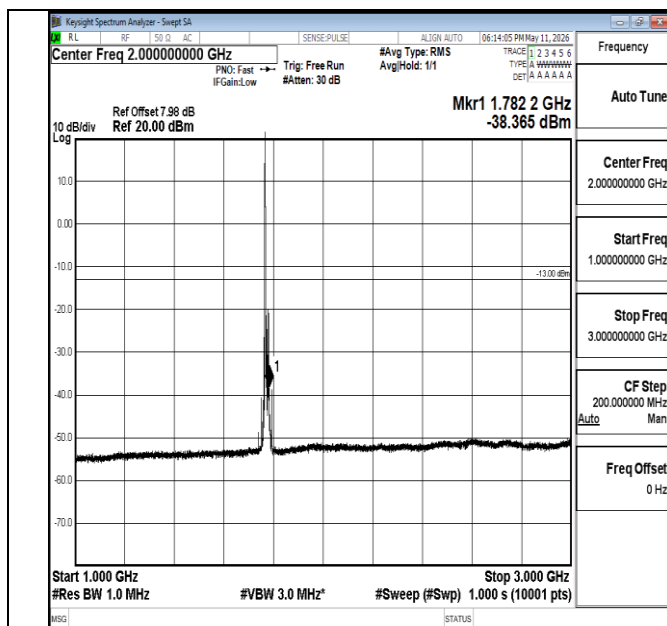
Band66-15MHz-16QAM-132597-1RB#0-1000~3000-PASS
