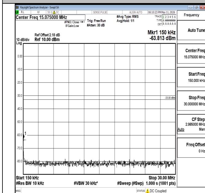
Band66-15MHz-16QAM-132047-1RB#0-0.15~30-PASS
