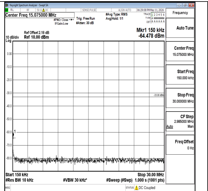
Band66-20MHz-QPSK-132322-1RB#0-0.15~30-PASS
