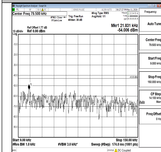
Band66-20MHz-QPSK-132072-1RB#0-0.009~0.15-PASS
