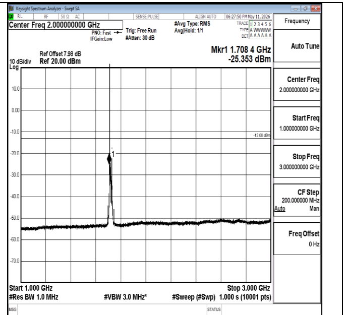
Band66-20MHz-QPSK-132072-1RB#0-1000~3000-PASS
