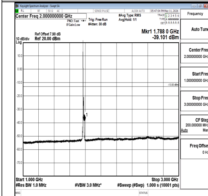
Band66-10MHz-16QAM-132622-1RB#0-1000~3000-PASS
