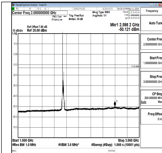
Band66-20MHz-16QAM-132322-1RB#0-1000~3000-PASS
