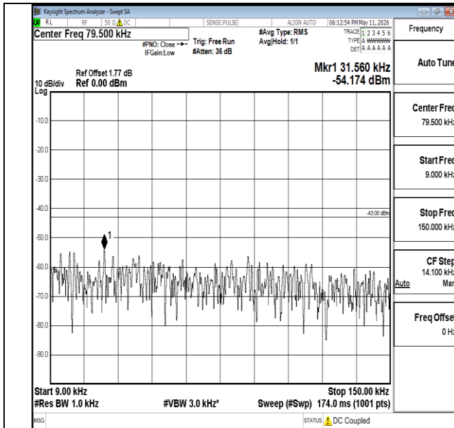
Band66-15MHz-QPSK-132597-1RB#0-0.009~0.15-PASS
