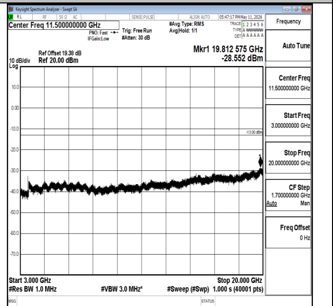
Band66-10MHz-16QAM-132622-1RB#0-3000~20000-PASS
