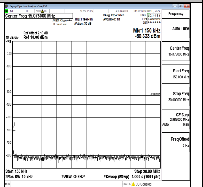
Band66-20MHz-QPSK-132572-1RB#0-0.15~30-PASS
