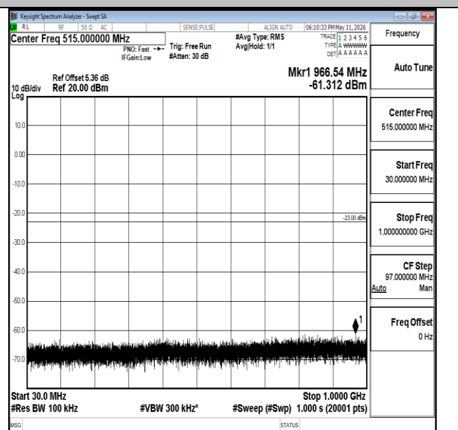
Band66-15MHz-16QAM-132047-1RB#0-30~1000-PASS
