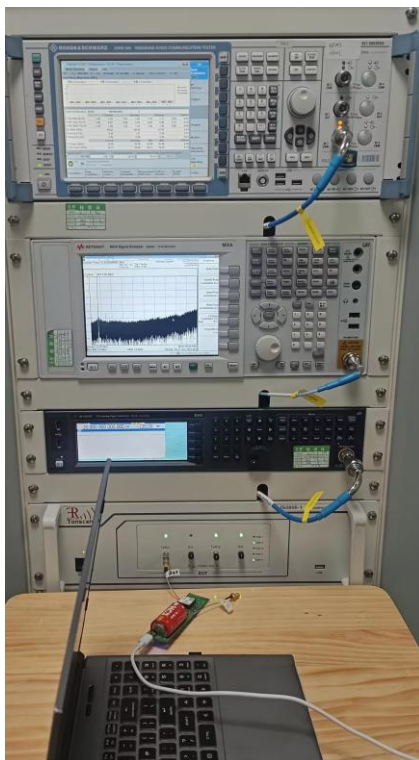
Test Setup Photo(s) of RF Conducted Measurement
