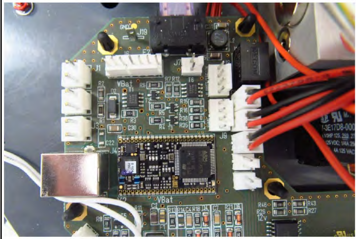
PCB top view D
