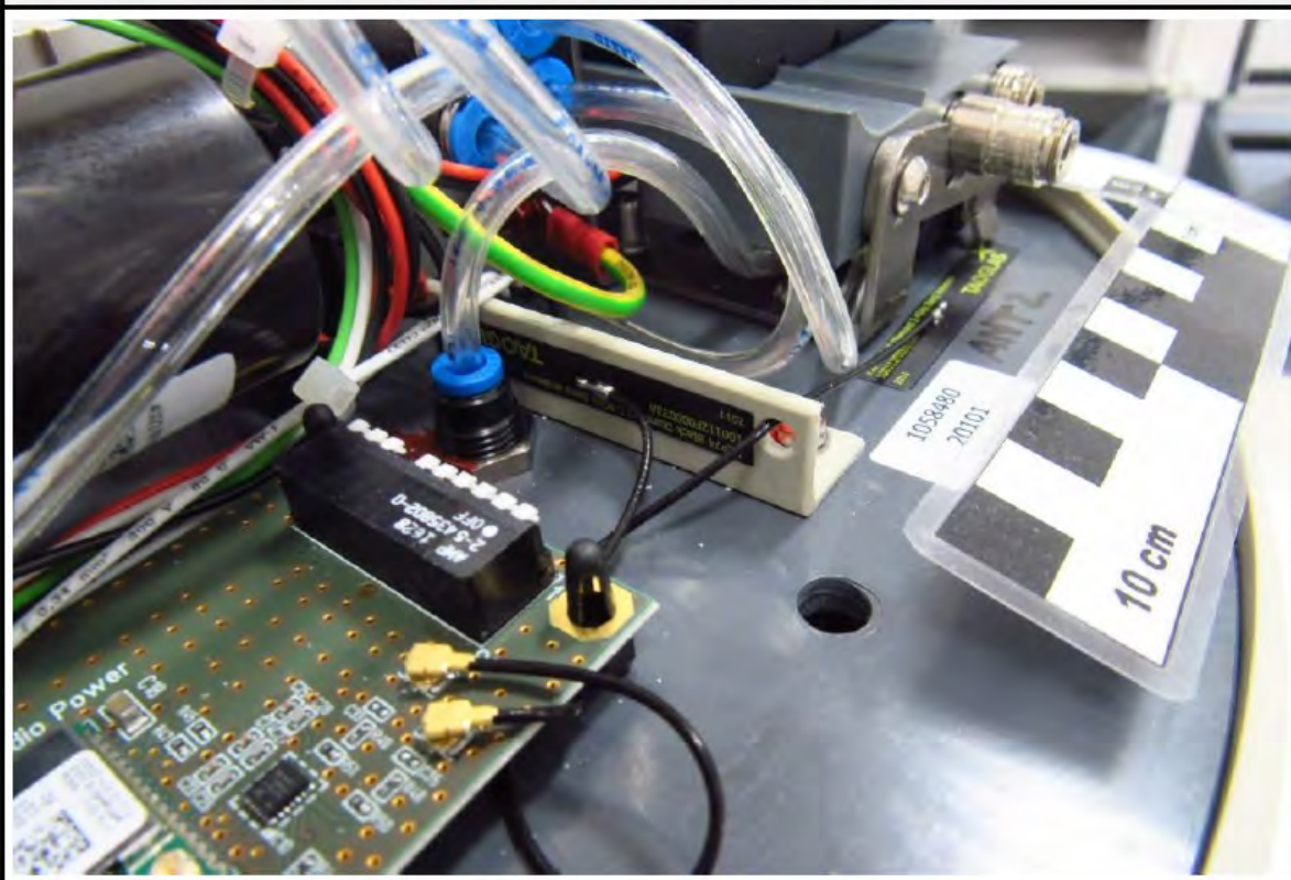
ZB Antenna view B
