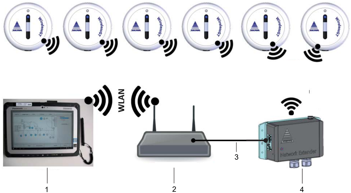
Figure 5: WirelessGT network
