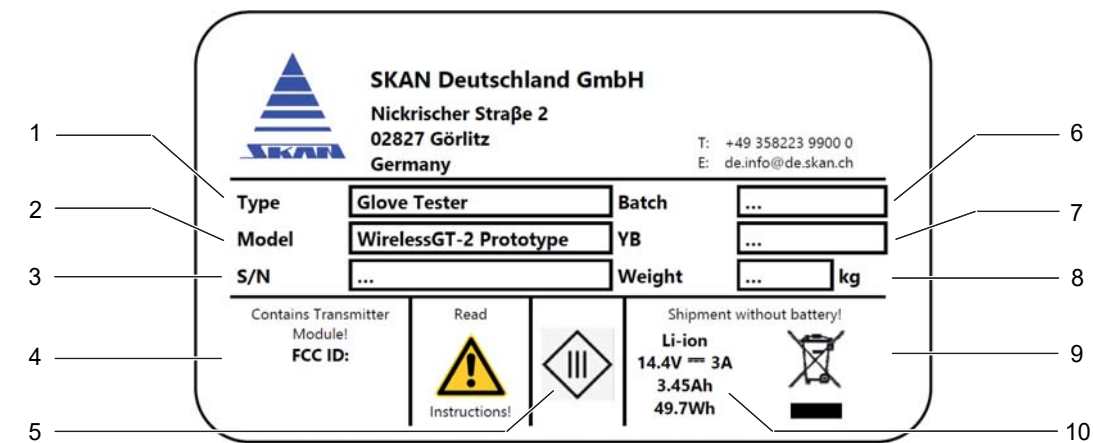
Figure 1: Nameplate
