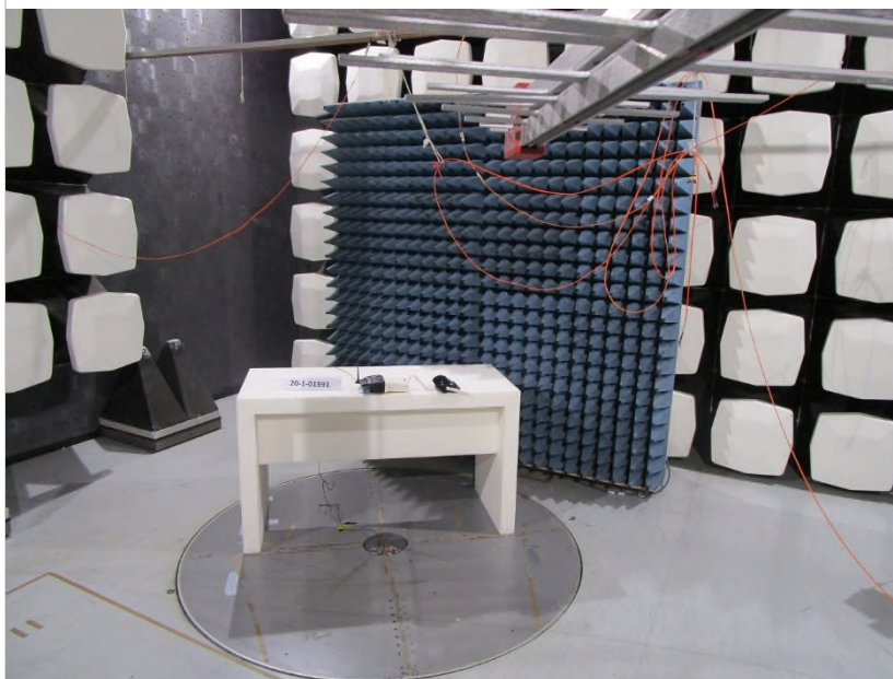
Photograph 2: EUT test setup in the semi anechoic chamber, overview
