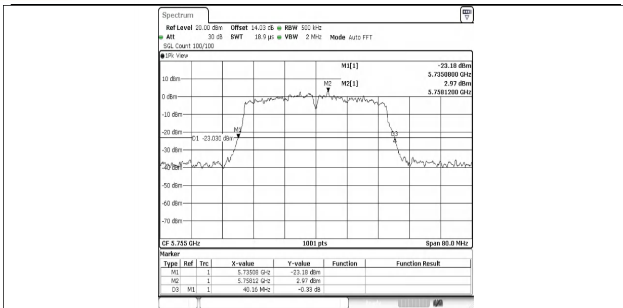
11N40SISO-Ant1-5755
