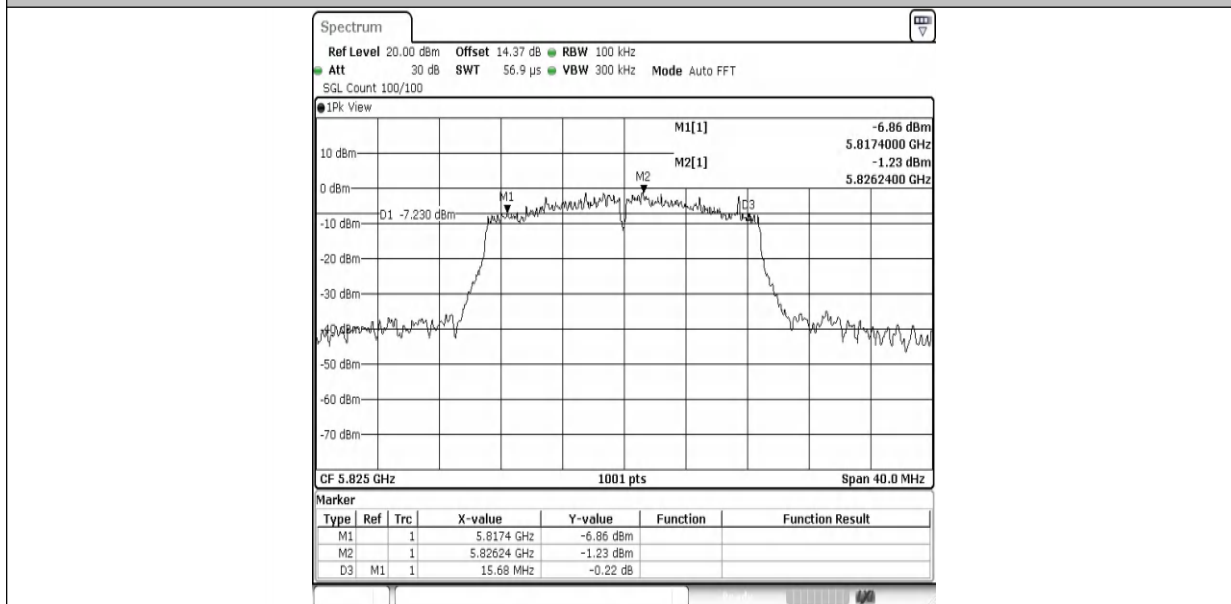
11N20SISO-Ant1-5825-PASS
