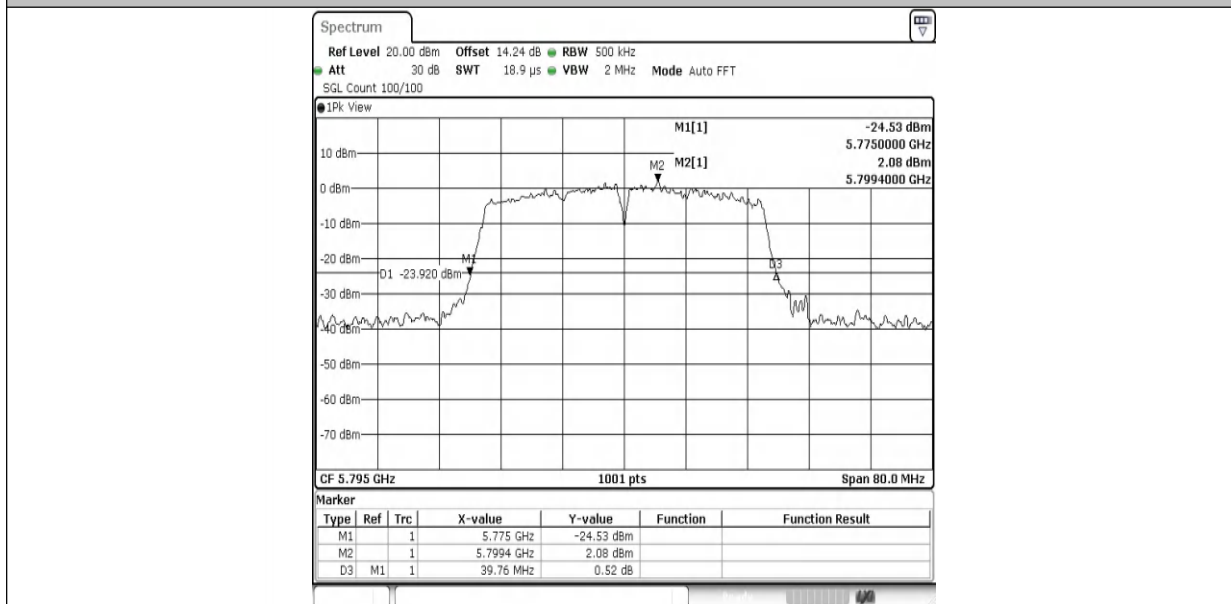
11N40SISO-Ant1-5795
