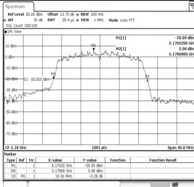
11AC20SISO-Ant1-5180
