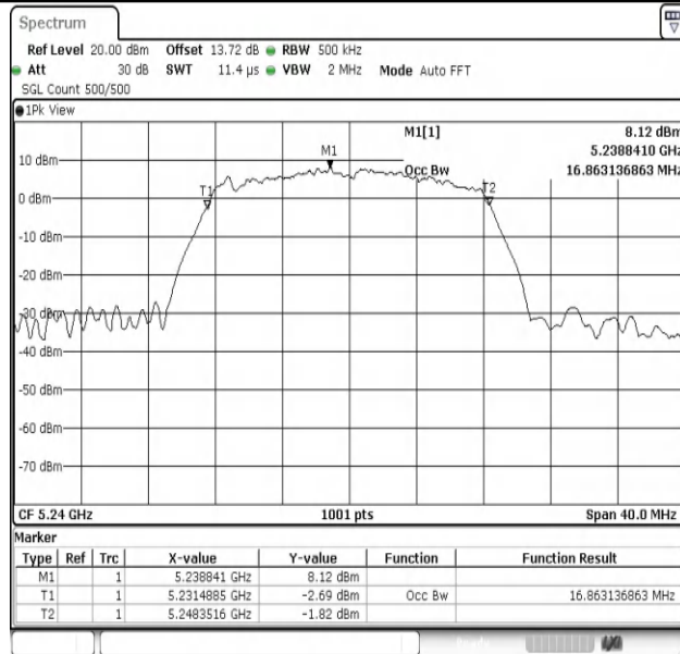
11A-Ant1-5240
