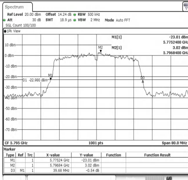
11AC40SISO-Ant1-5795
