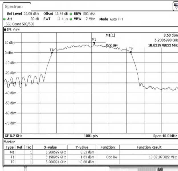
11AC20SISO-Ant1-5200
