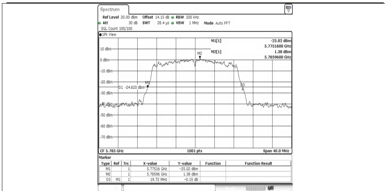
11AC20SISO-Ant1-5785
