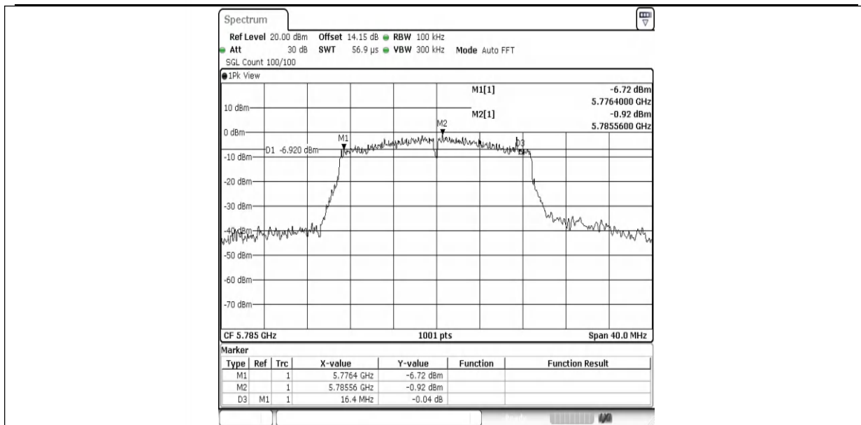
11N20SISO-Ant1-5785-PASS
