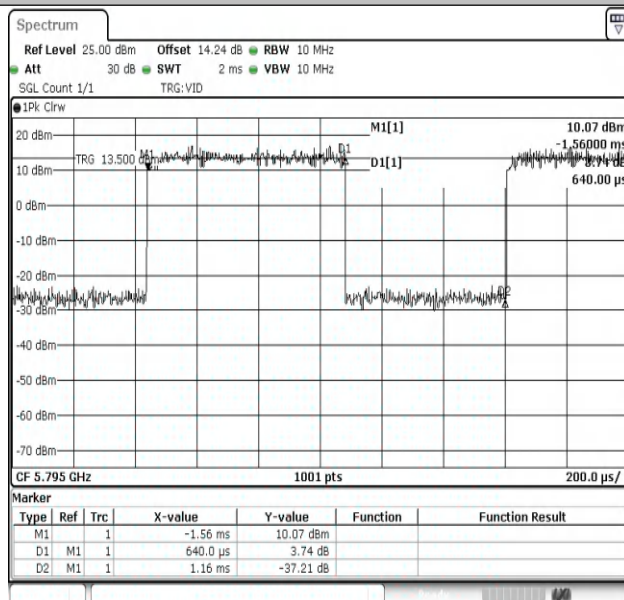
NTNV-11N40SISO-Ant1-5795
