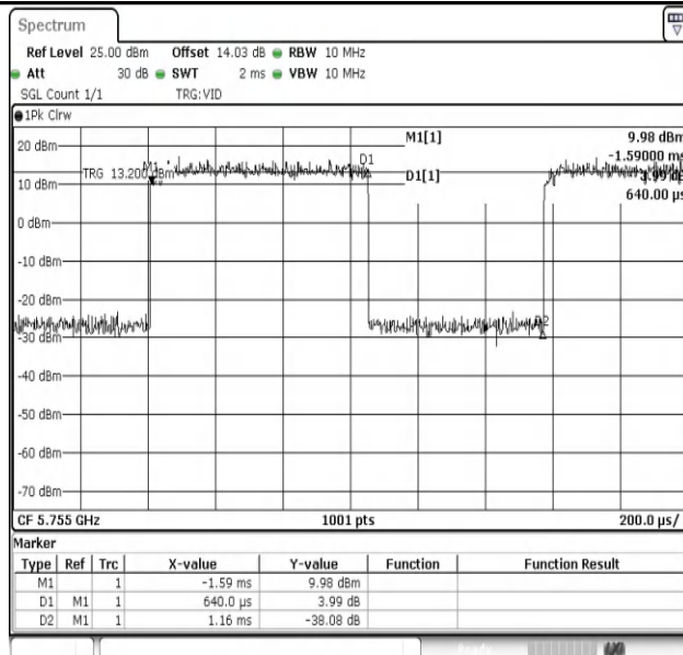
NTNV-11N40SISO-Ant1-5755
