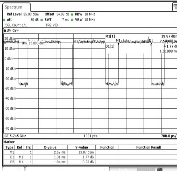
NTNV-11AC20SISO-Ant1-5745
