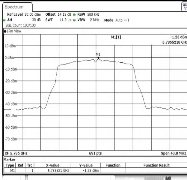
11A-Ant1-5785-PASS
