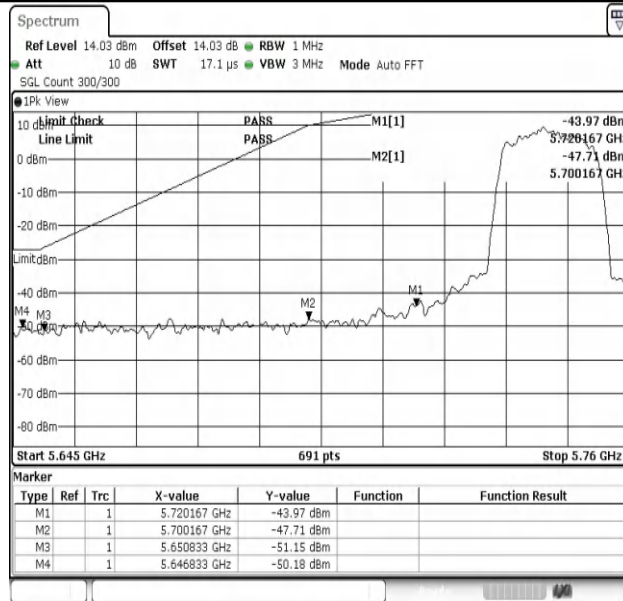
11N20SISO-Ant1-5745-PASS
