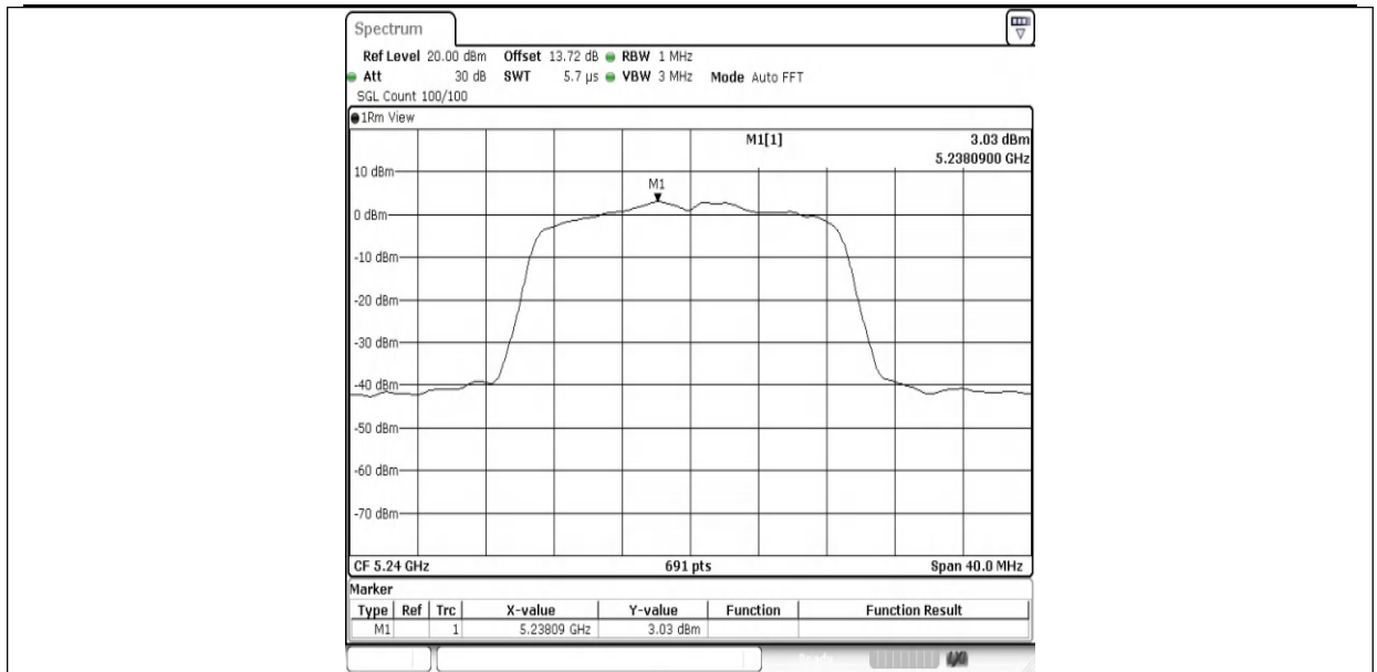
11N20SISO-Ant1-5240-PASS
