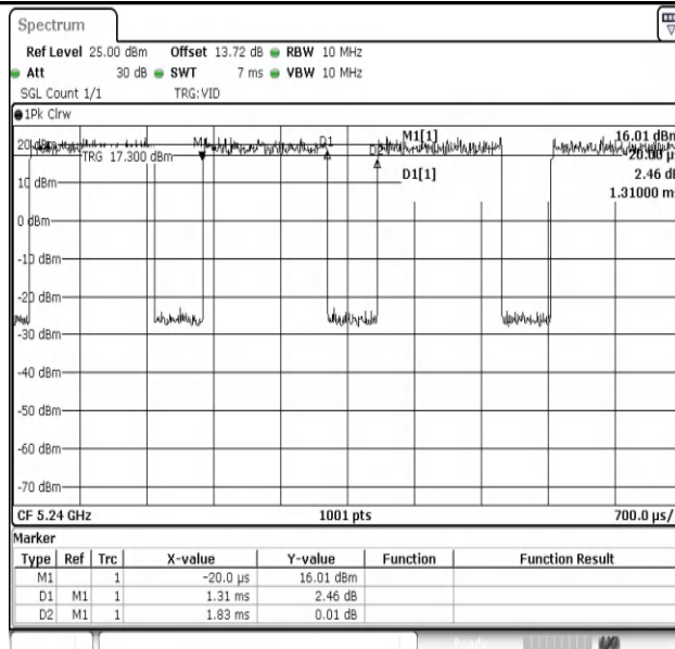
NTNV-11AC20SISO-Ant1-5240
