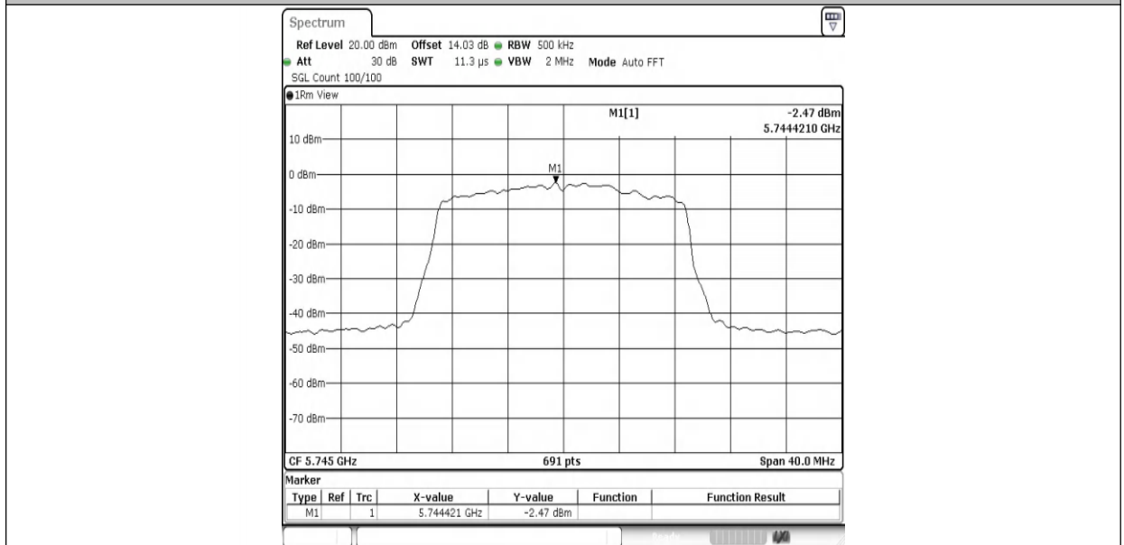
11N20SISO-Ant1-5745-PASS
