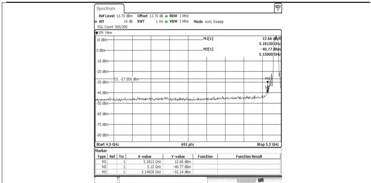
11AC20SISO-Ant1-5180-PASS
