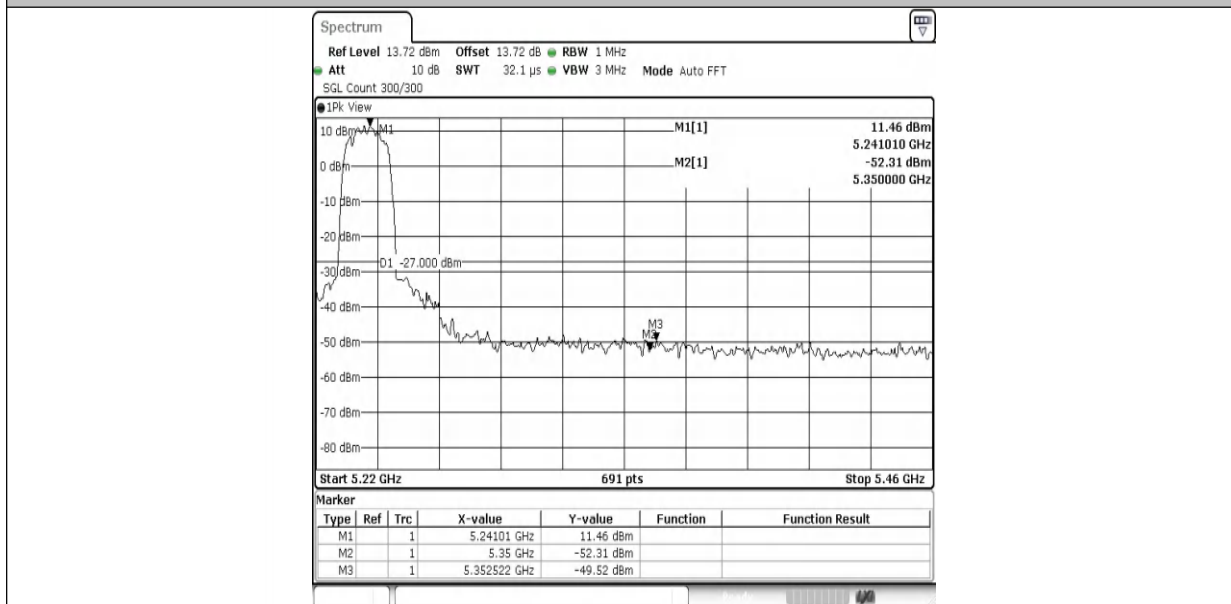
11AC20SISO-Ant1-5240-PASS
