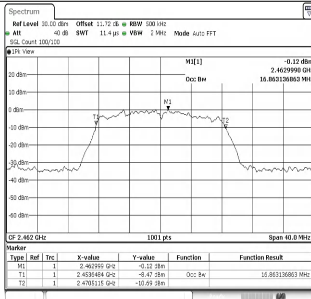
11G-Ant2-2462
