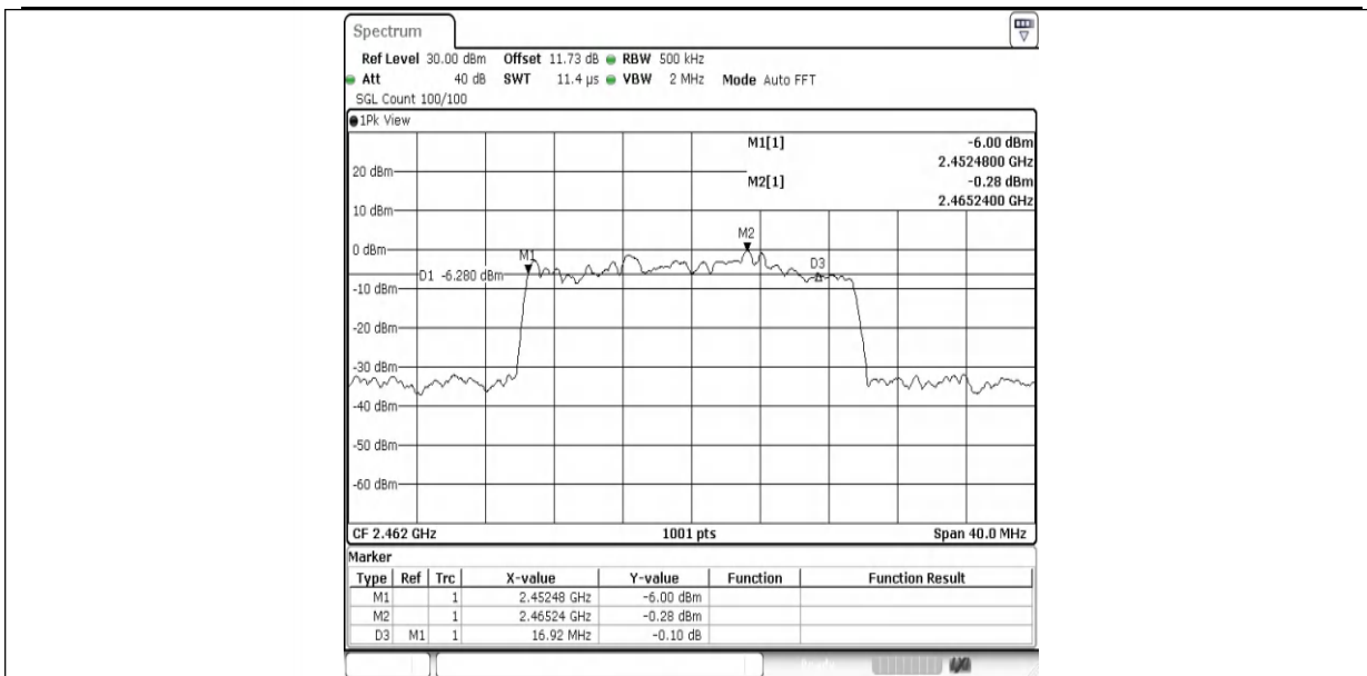
11AX20MIMO-Ant1-2462-PASS
