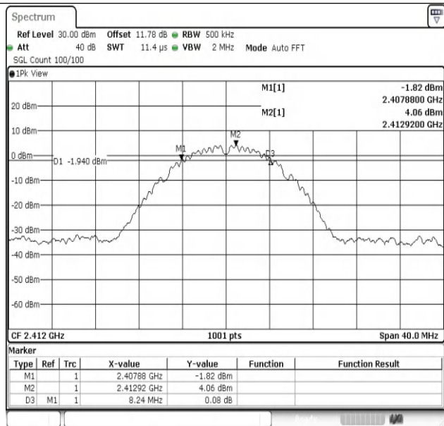
11B-Ant1-2412-PASS
