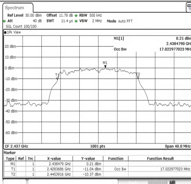
11G-Ant2-2437
