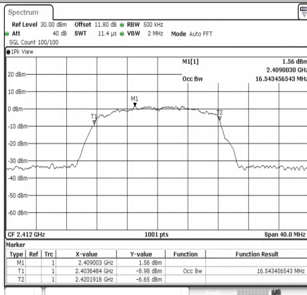
11G-Ant2-2412
