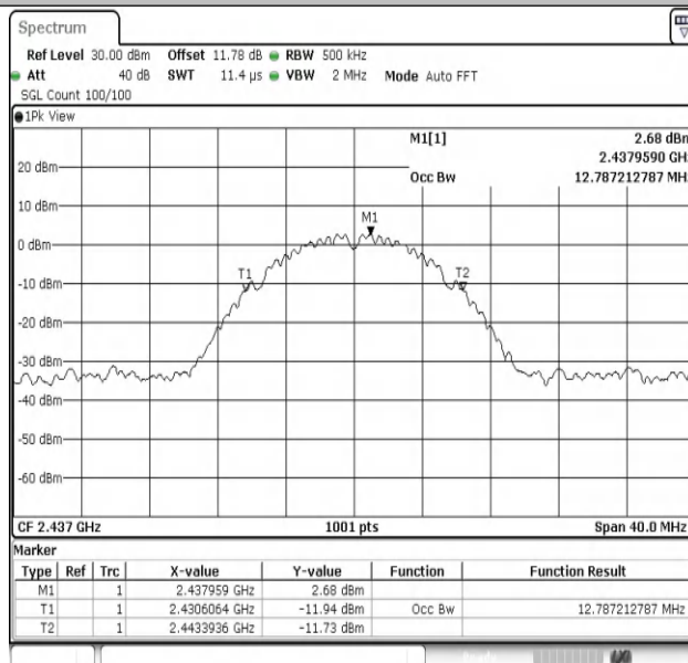
11B-Ant2-2437
