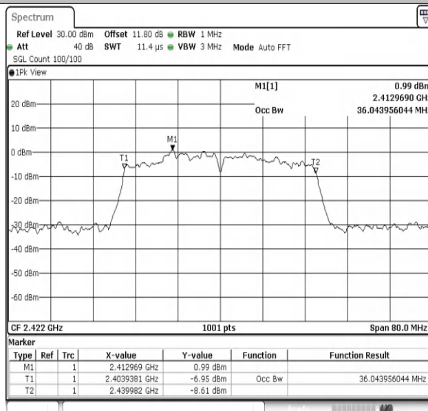
11N40MIMO-Ant2-2422
