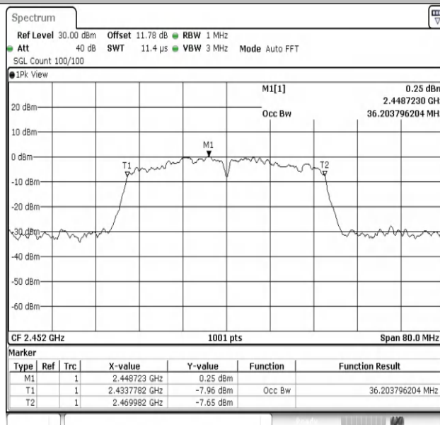
11N40MIMO-Ant2-2452
