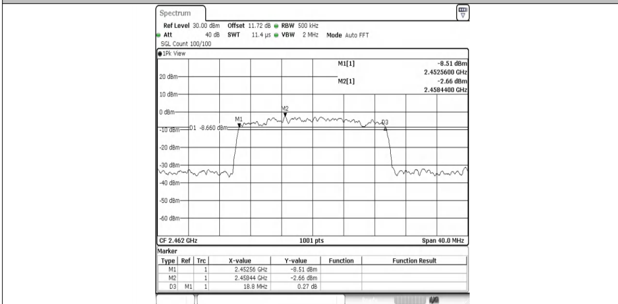
11AX20MIMO-Ant2-2462-PASS
