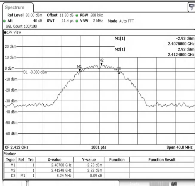
11B-Ant2-2412-PASS
