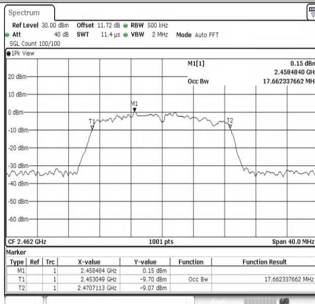
11N20MIMO-Ant2-2462
