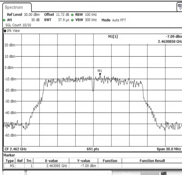
11G-Ant2-2462-0~Reference-PASS
