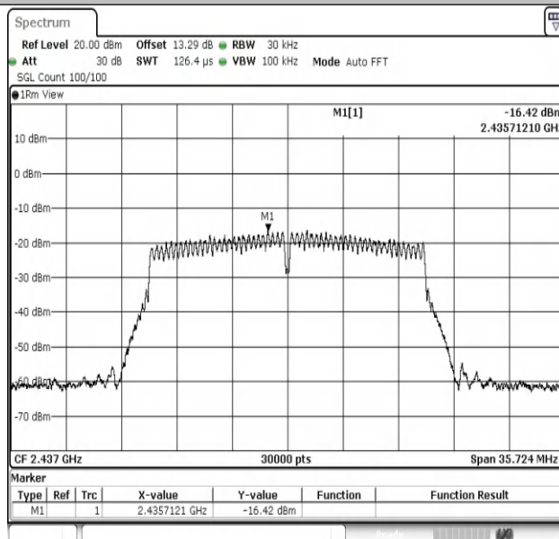
11N20MIMO-Ant2-2437-PASS
