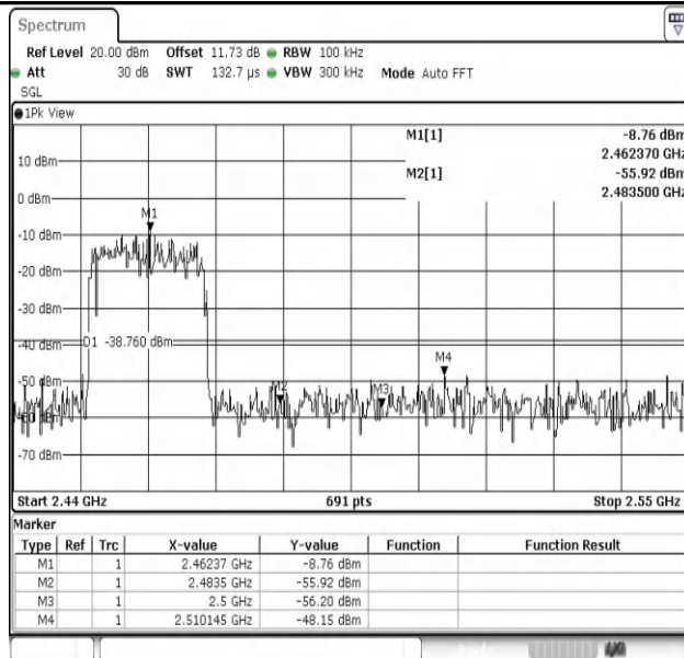
11AX20MIMO-Ant1-2462-PASS
