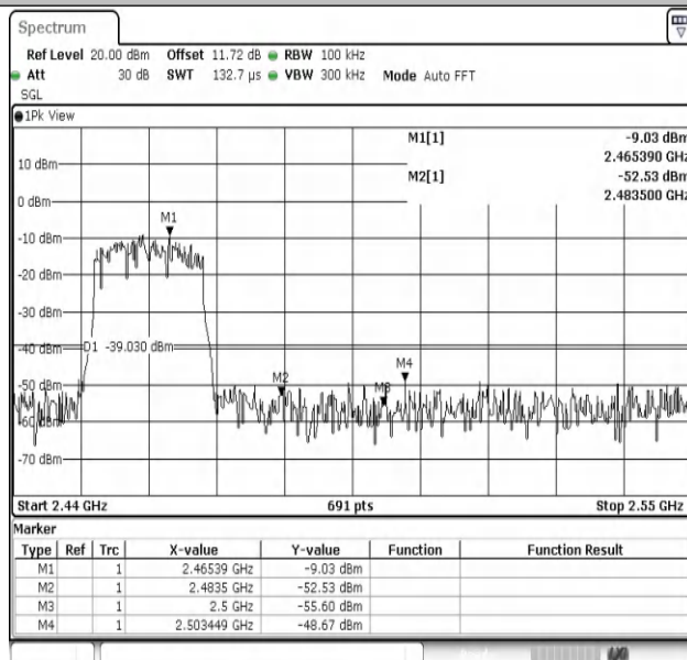
11N20MIMO-Ant2-2462-PASS
