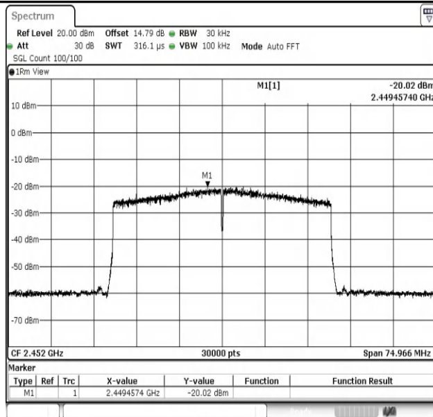
11AX40MIMO-Ant1-2452-PASS
