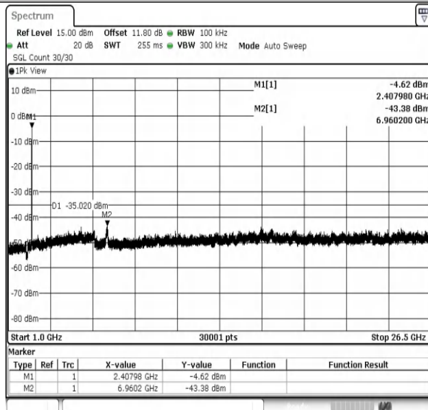
11G-Ant2-2412-1000~26500-PASS
