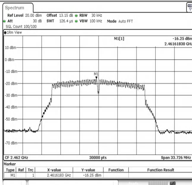
11G-Ant2-2462-PASS
