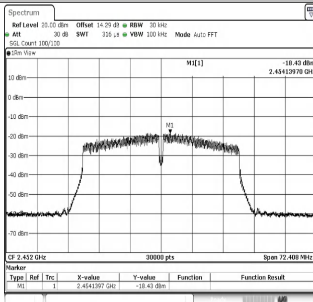
11N40MIMO-Ant2-2452-PASS
