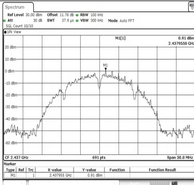
11B-Ant2-2437-0~Reference-PASS
