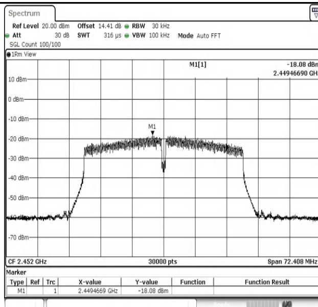
11N40MIMO-Ant1-2452-PASS
