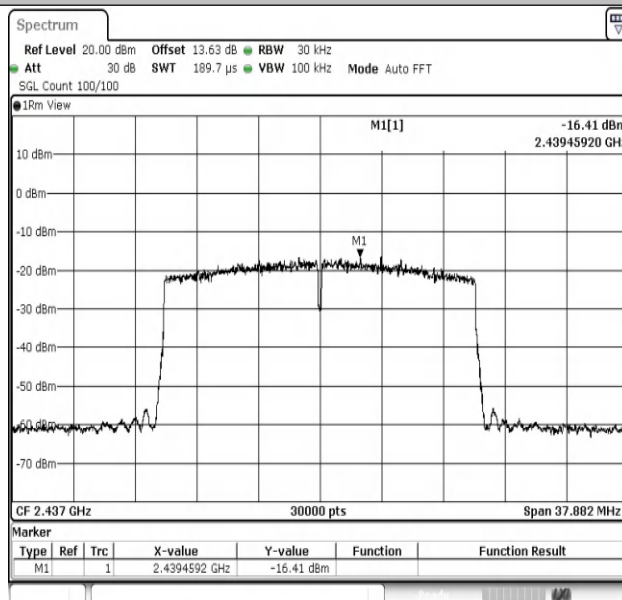
11AX20MIMO-Ant2-2437-PASS
