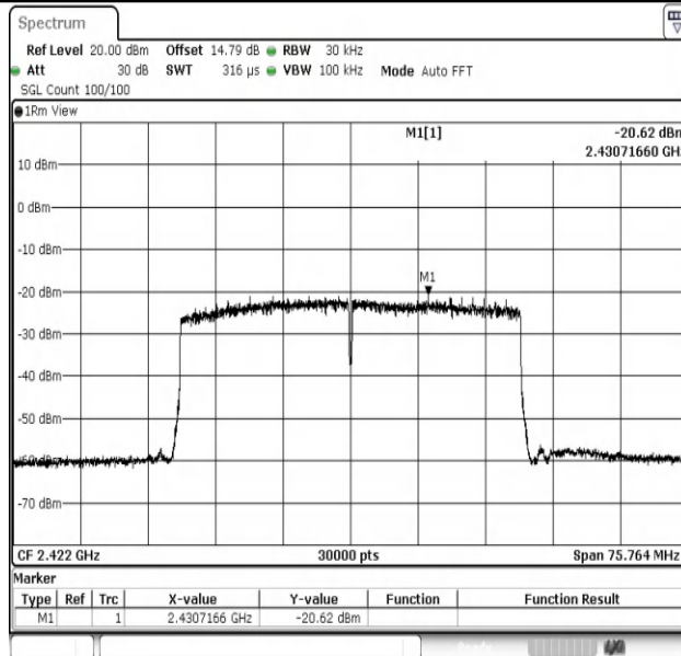
11AX40MIMO-Ant1-2422-PASS
