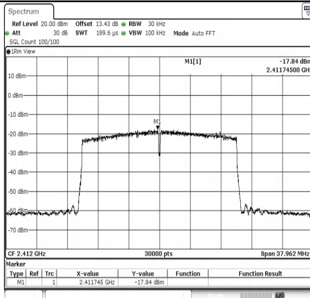
11AX20MIMO-Ant1-2412-PASS
