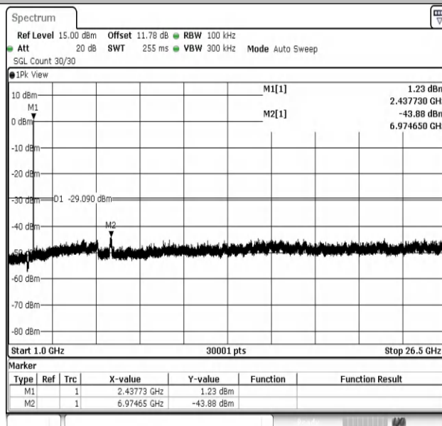
11B-Ant2-2437-1000~26500-PASS
