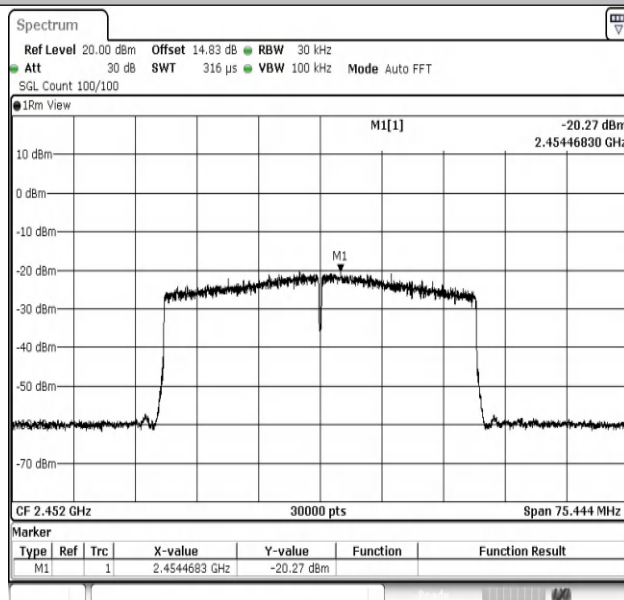
11AX40MIMO-Ant2-2452-PASS
