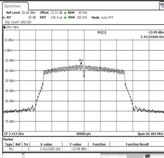
11N20MIMO-Ant1-2412-PASS
