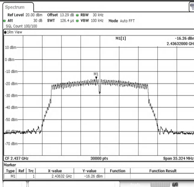
11N20MIMO-Ant1-2437-PASS
