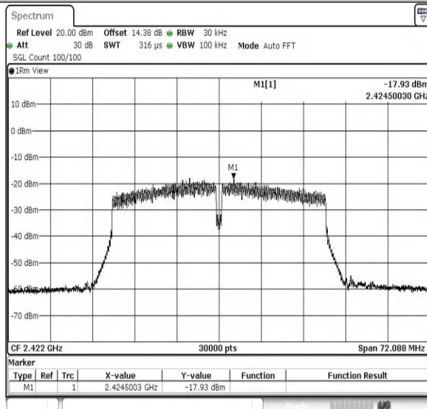
11N40MIMO-Ant2-2422-PASS
