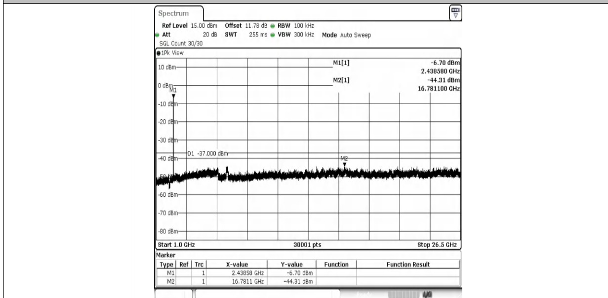
11G-Ant2-2437-1000~26500-PASS
