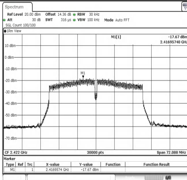
11N40MIMO-Ant1-2422-PASS
