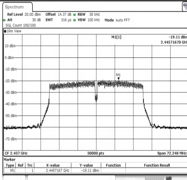
11N40MIMO-Ant1-2437-PASS
