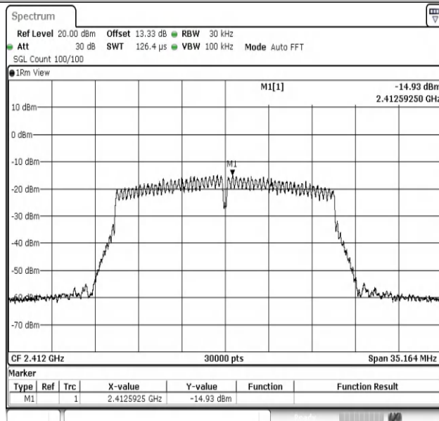
11N20MIMO-Ant2-2412-PASS
