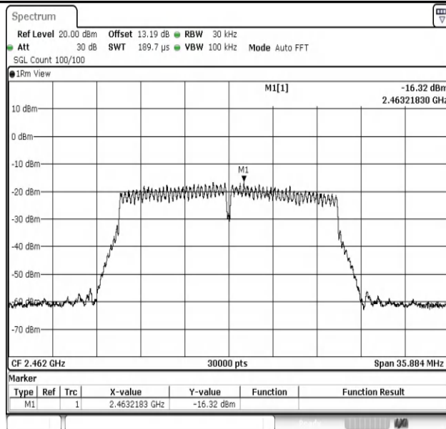
11N20MIMO-Ant1-2462-PASS
