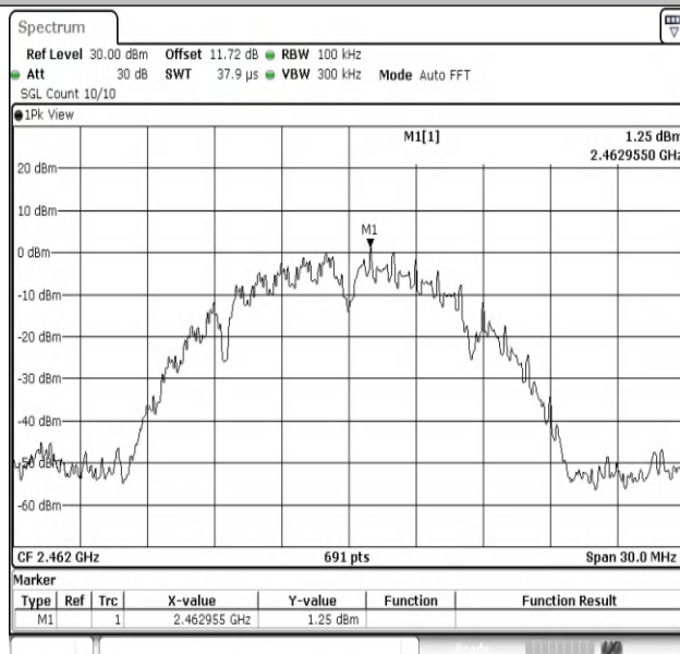
11B-Ant2-2462-0~Reference-PASS
