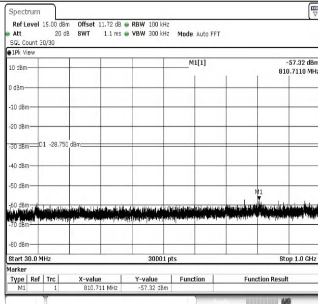
11B-Ant2-2462-30~1000-PASS
