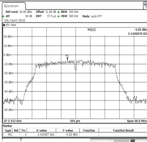
11G-Ant2-2412-0~Reference-PASS
