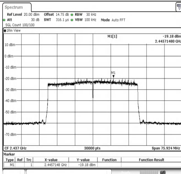
11AX40MIMO-Ant2-2437-PASS
