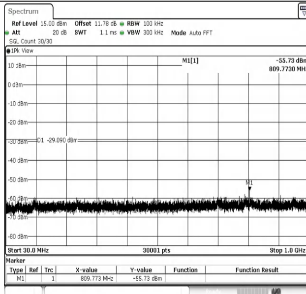
11B-Ant2-2437-30~1000-PASS
