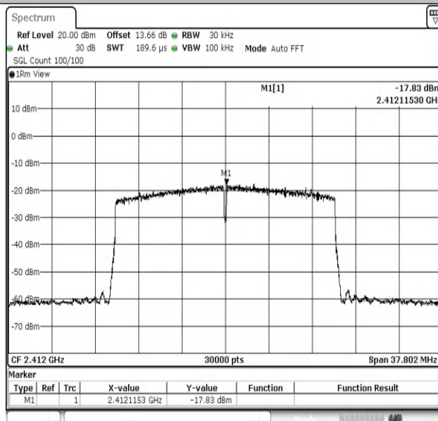
11AX20MIMO-Ant2-2412-PASS
