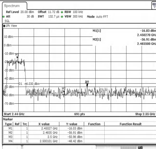
11AX20MIMO-Ant2-2462-PASS
