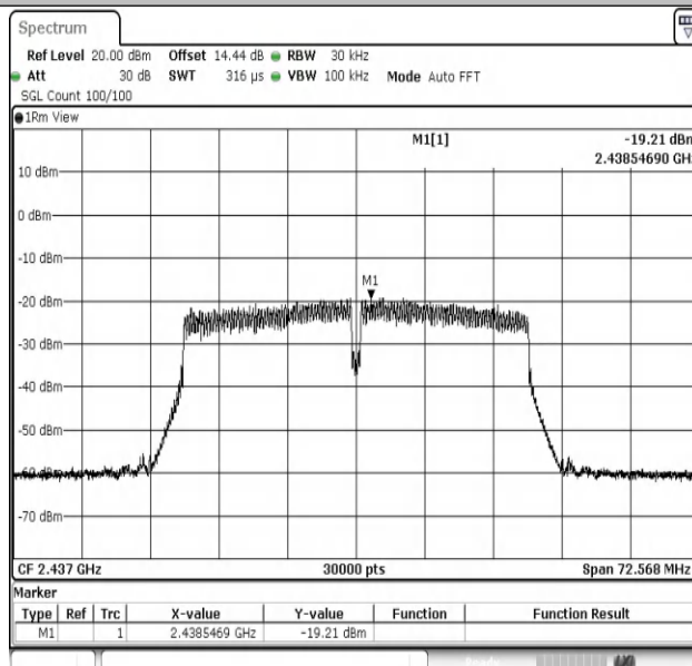
11N40MIMO-Ant2-2437-PASS
