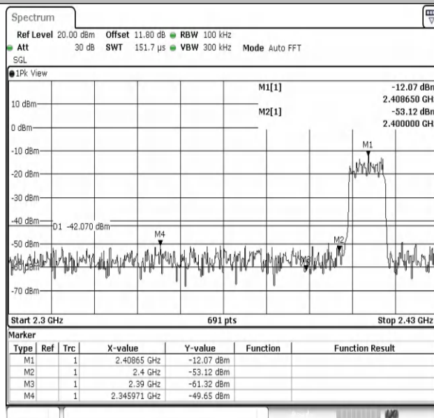
11AX40MIMO-Ant2-2422-PASS
