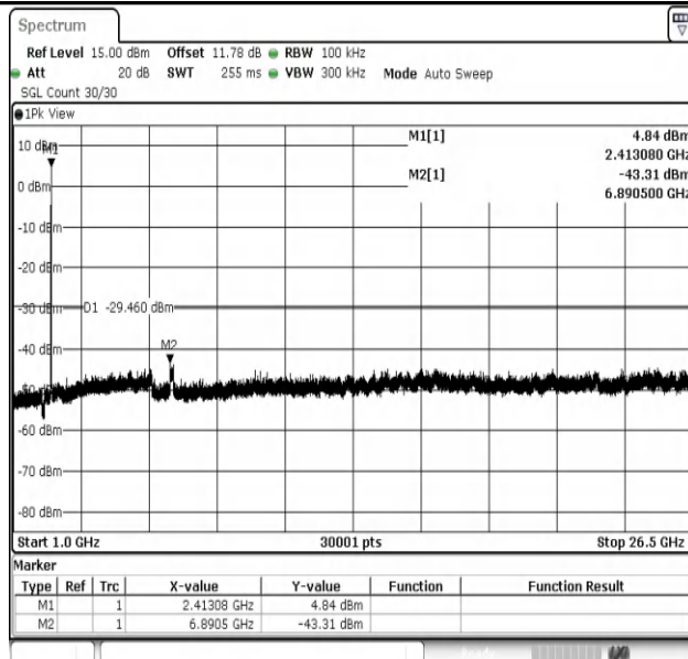
11N20SISO-Ant1-2412-1000~26500-PASS
