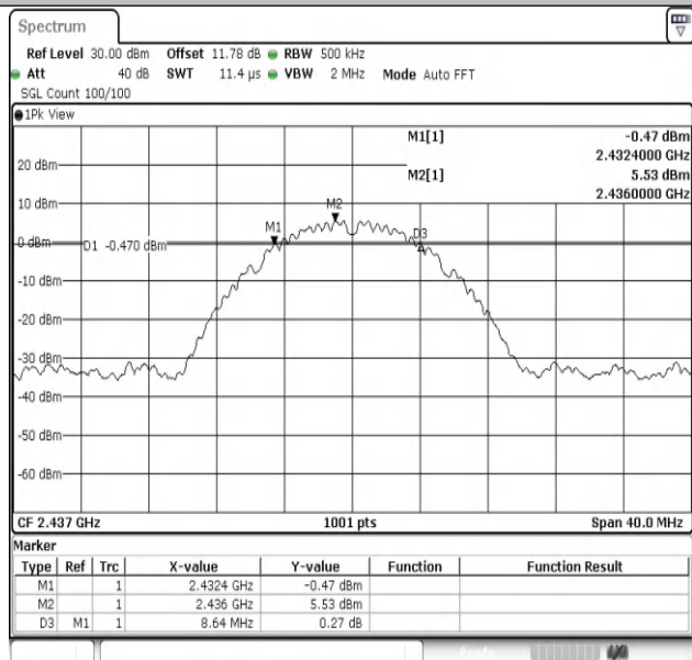
11B-Ant1-2437-PASS
