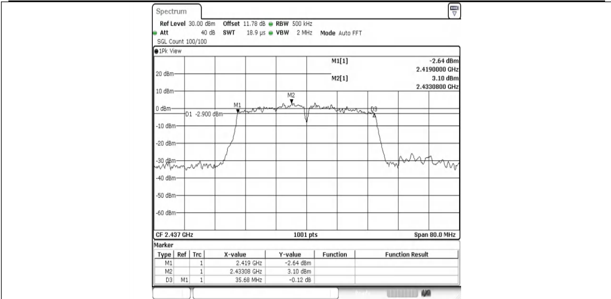
11N40SISO-Ant1-2437-PASS
