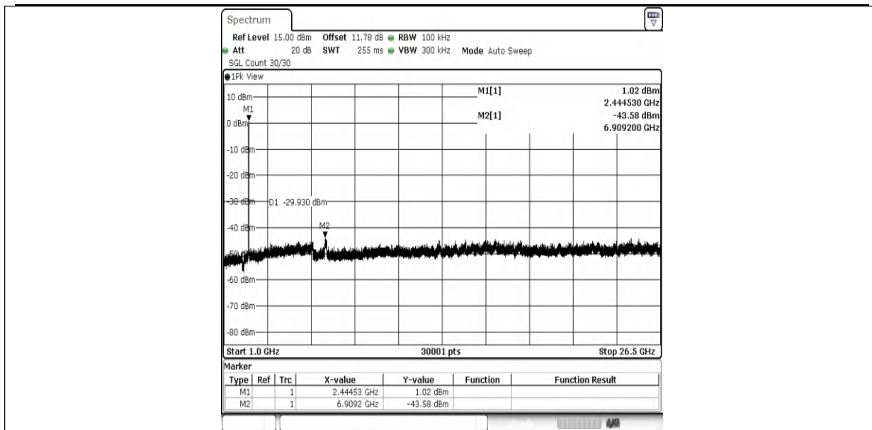
11G-Ant1-2437-1000~26500-PASS
