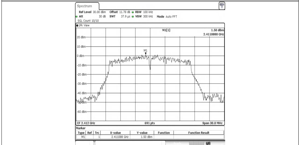
11G-Ant1-2412-0~Reference-PASS
