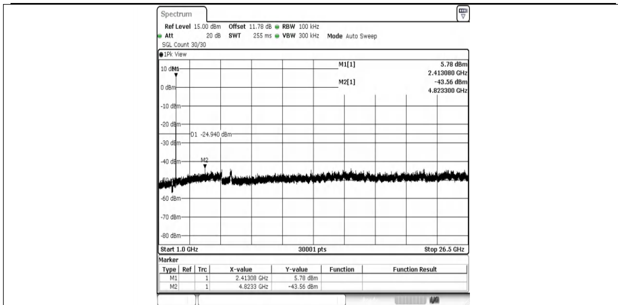
11B-Ant1-2412-1000~26500-PASS
