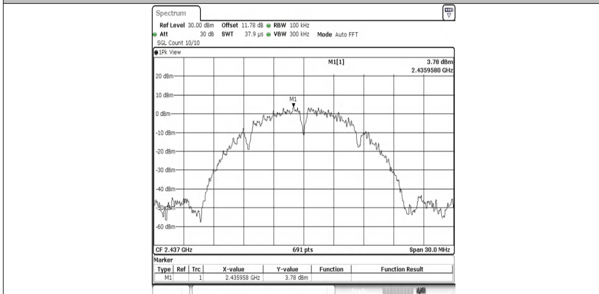
11B-Ant1-2437-0~Reference-PASS
