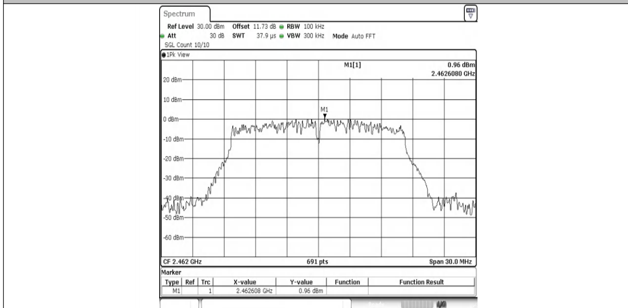
11G-Ant1-2462-0~Reference-PASS
