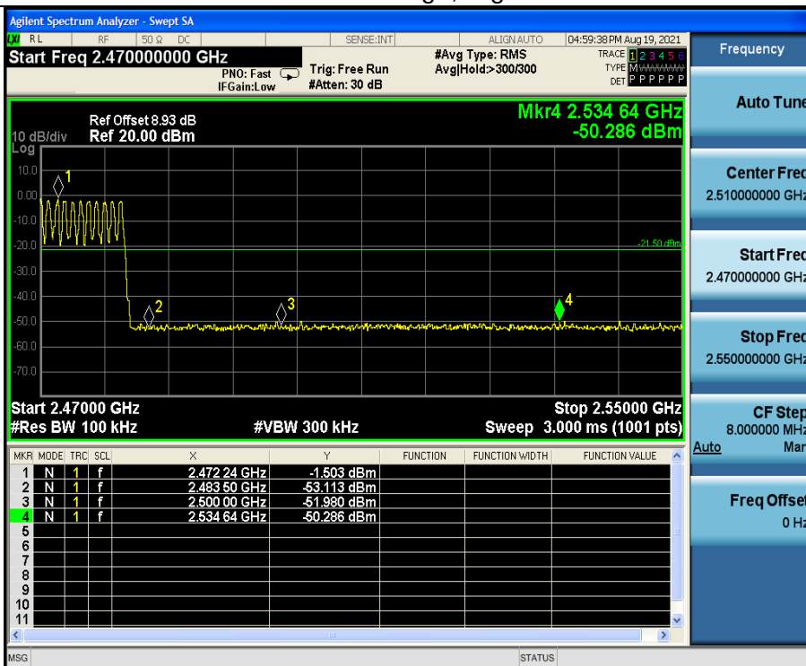
GFSK: Band Edge, Right Side
