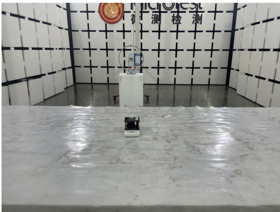
Radiated emissions – Blew 30 MHz
