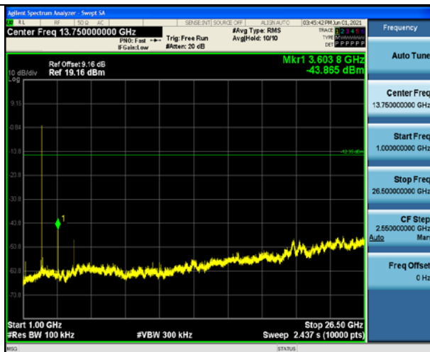
8DPSK on Channel 39
