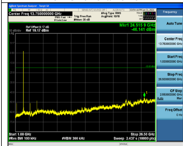
8DPSK on Channel 78
