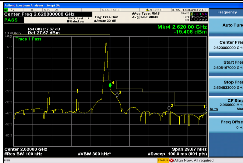
Band38-10MHz-QPSK-38200-1RB#49
