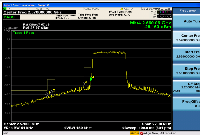
Band38-5MHz-16QAM-37775-25RB#0
