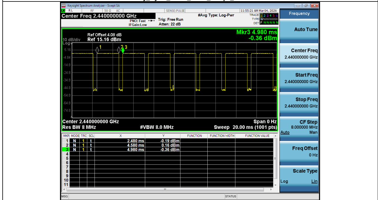
Duty_Cycle_NVNT_ANT1_1Mbps_2440
