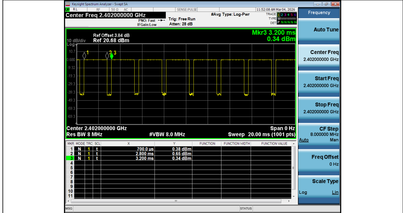
Duty_Cycle_NVNT_ANT1_1Mbps_2402
