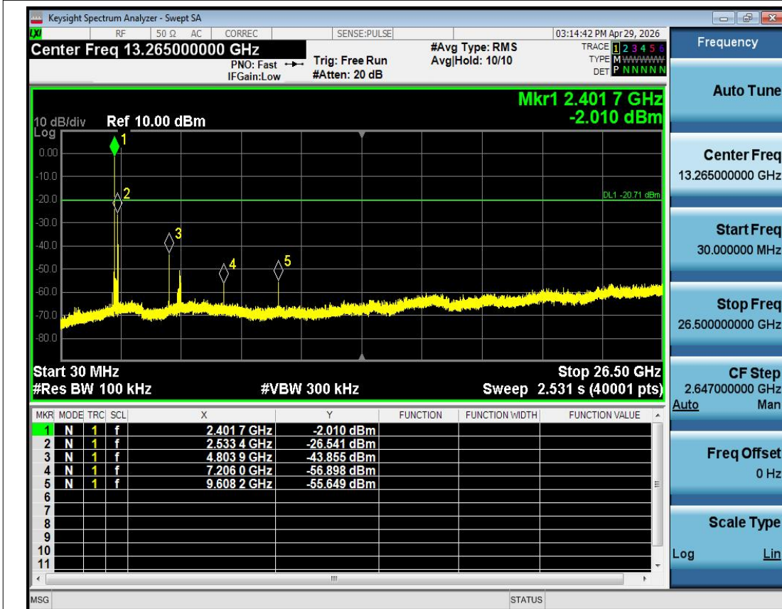
Tx. Spurious NVNT GFSK 2402MHz Ant1 Emission
