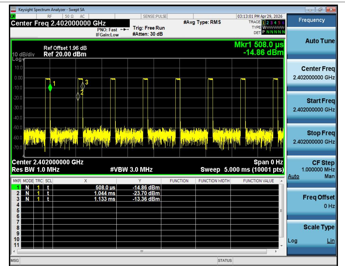
Duty Cycle NVNT GFSK 2402MHz Ant1
