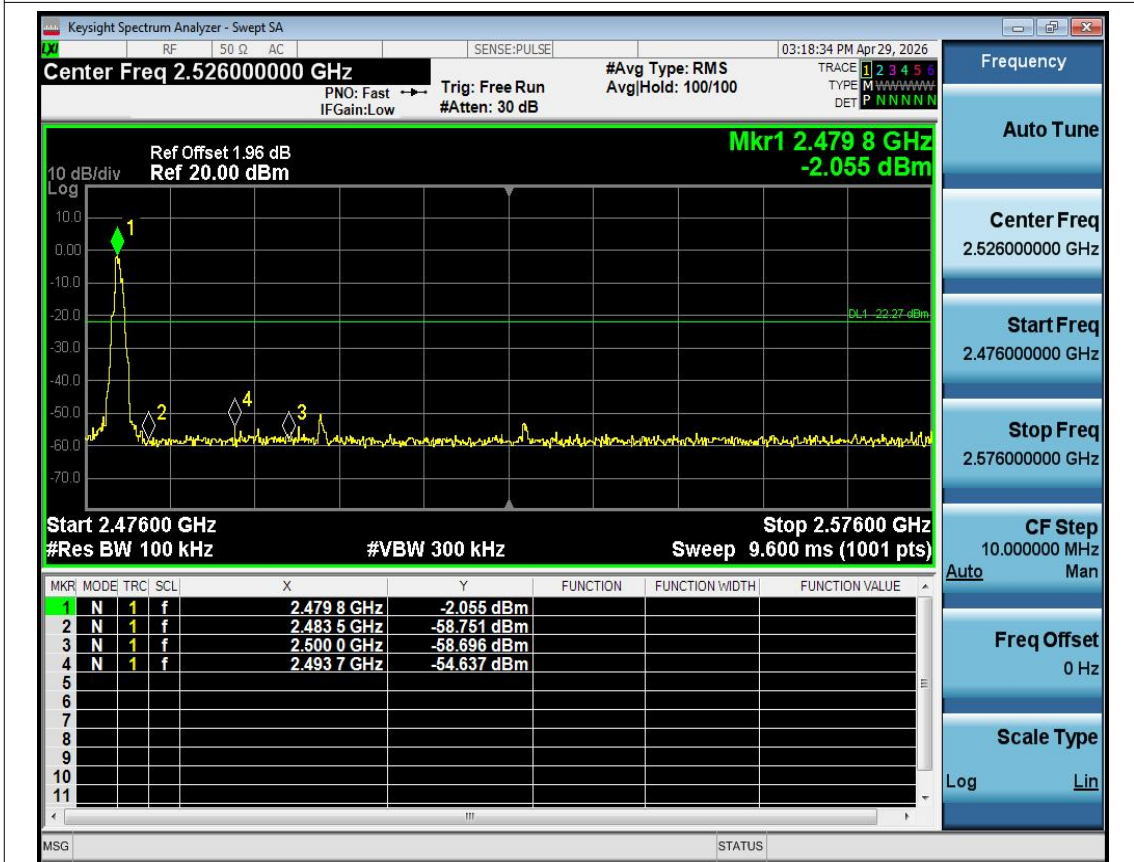
Band Edge NVNT GFSK 2480MHz Ant1 Emission
