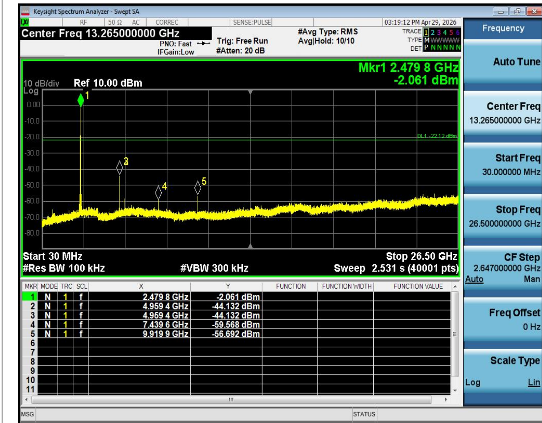
Tx. Spurious NVNT GFSK 2480MHz Ant1 Emission
