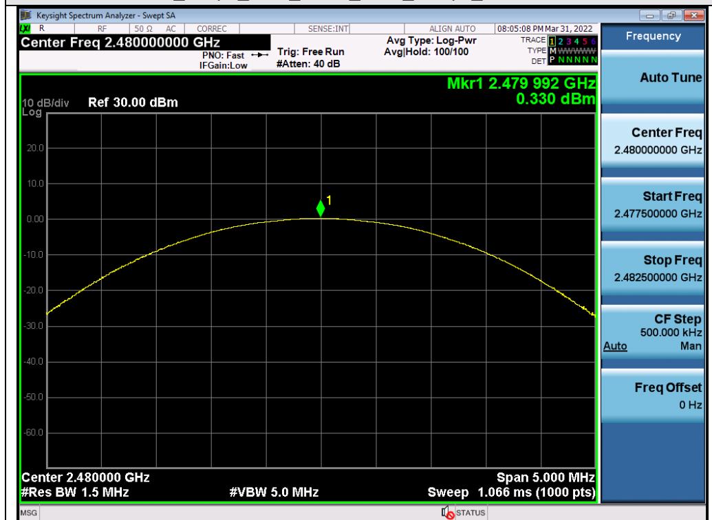
Test_Graph_EDR_ANT1_2480_3Mbps_Peak Power
