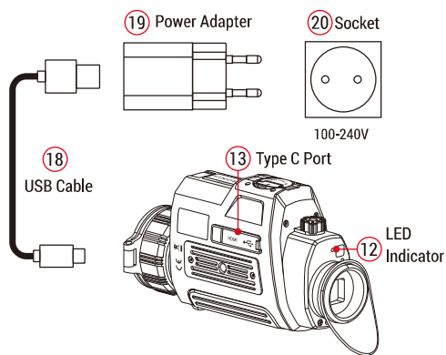
LED indicator displaying the current status of the device
