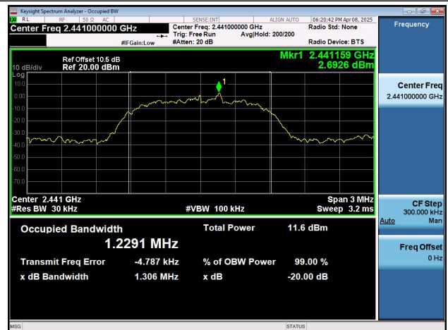
3DH5-Ant1-2441
