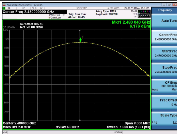
3DH5-Ant1-2480-PASS
