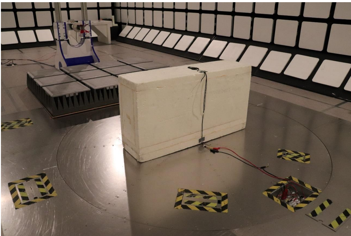
Photograph 2: Test Setup for Radiated Emissions (1 - 18 GHz)
