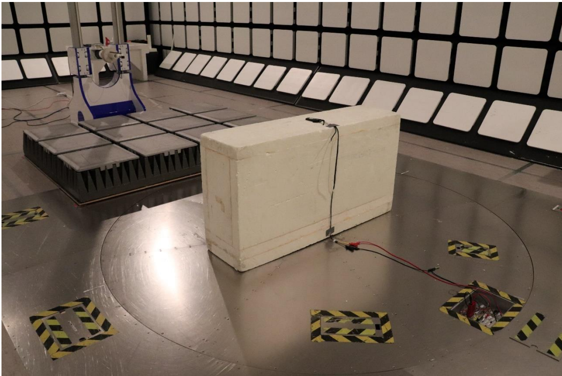
Photograph 3: Test Setup for Radiated Emissions (18 - 22 GHz)
