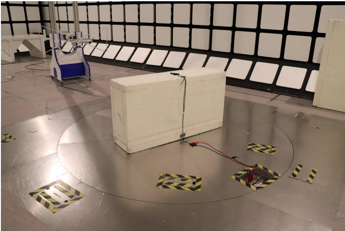
Photograph 1: Test Setup for Radiated Emissions (30 - 1000 MHz)
