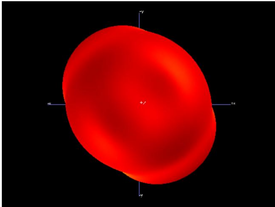
433MHz
