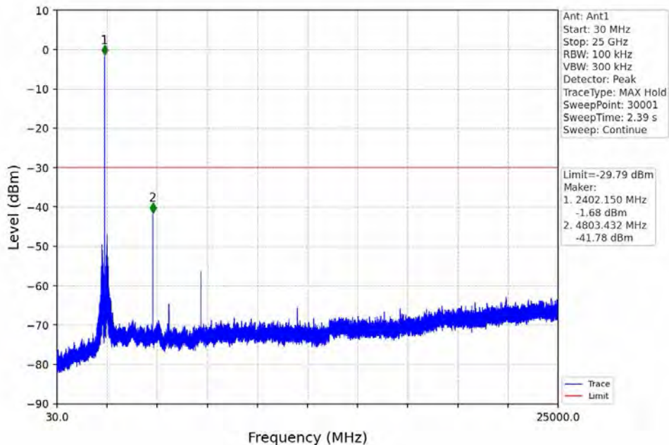
1M_LCH_2402MHz_DataRate=_Ant1_NTNV
