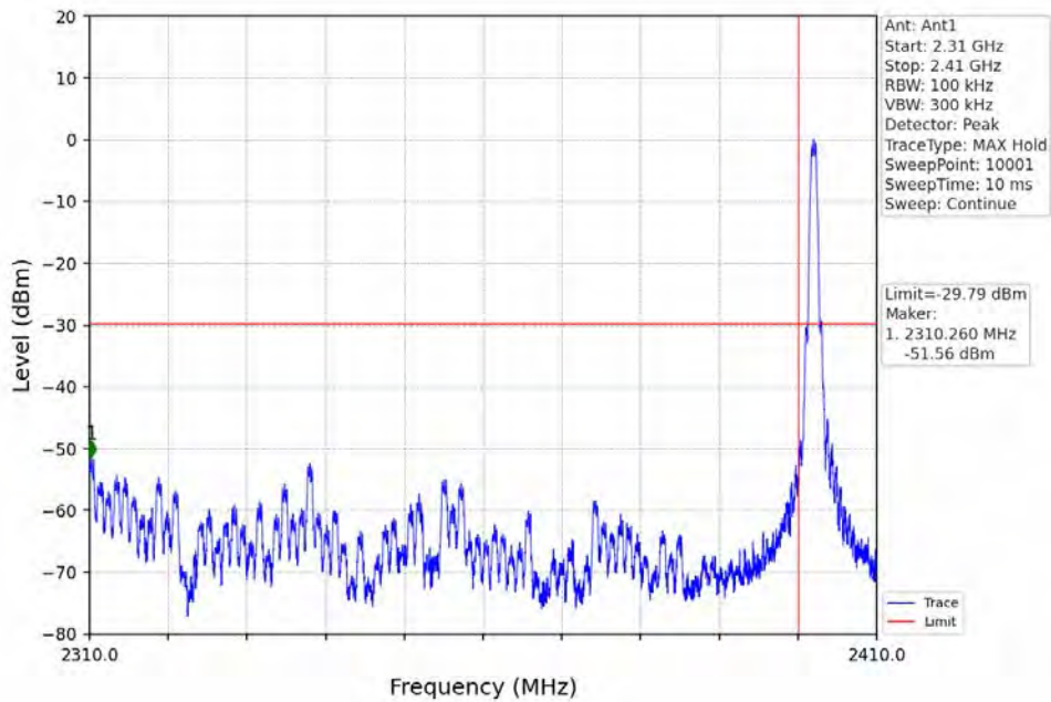
1M_LCH_2402MHz_DataRate=_Ant1_NTNV
