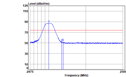
BLE_2M_TX_CH_39_Vertical-Peak
