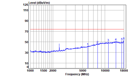
BLE_2M_TX_CH_19_Horizontal-Peak
