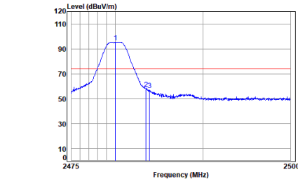
BLE_2M_TX_CH_39_Horizontal-Peak
