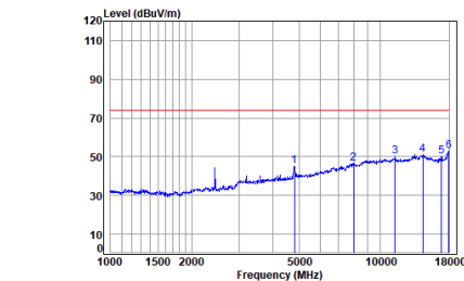
BLE_2M_TX_CH_19_Vertical-Peak
