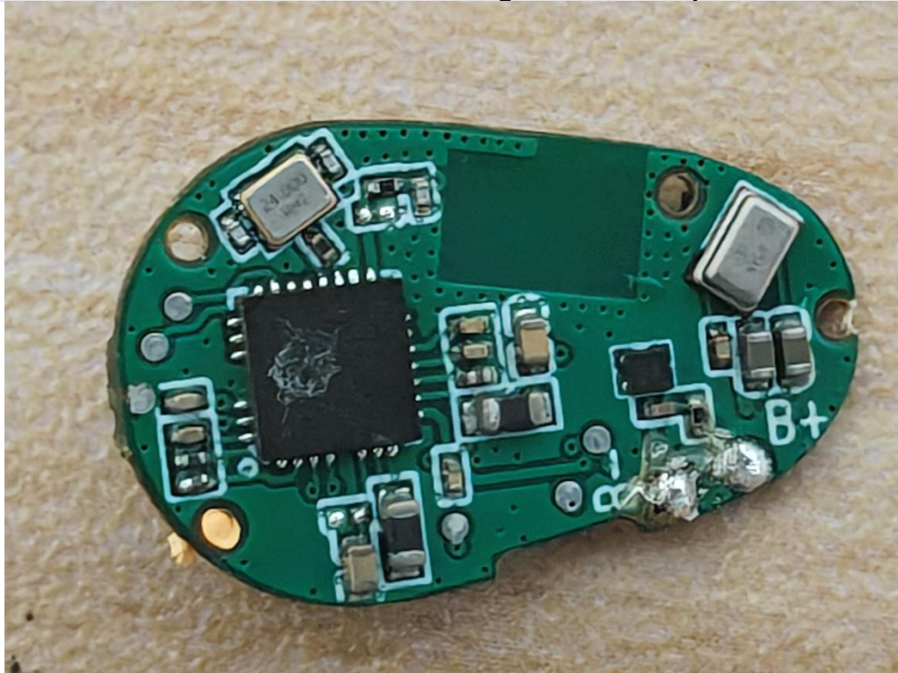
Internal View of MOONDROP Pudding ANC TWS Earphones EUT-8
