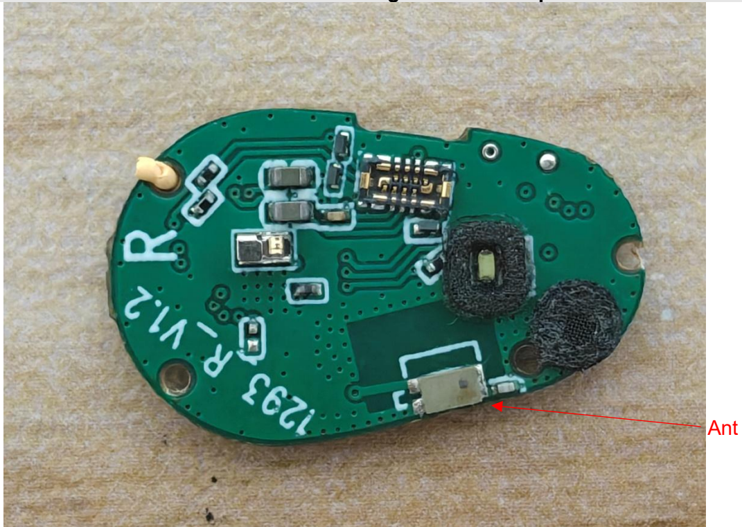
Internal View of MOONDROP Pudding ANC TWS Earphones EUT-8
