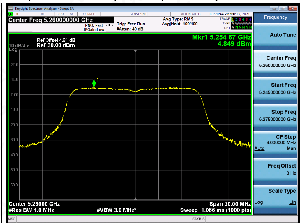
Test_Graph_802.11a_ANT2_5260_6Mbps_PSD
