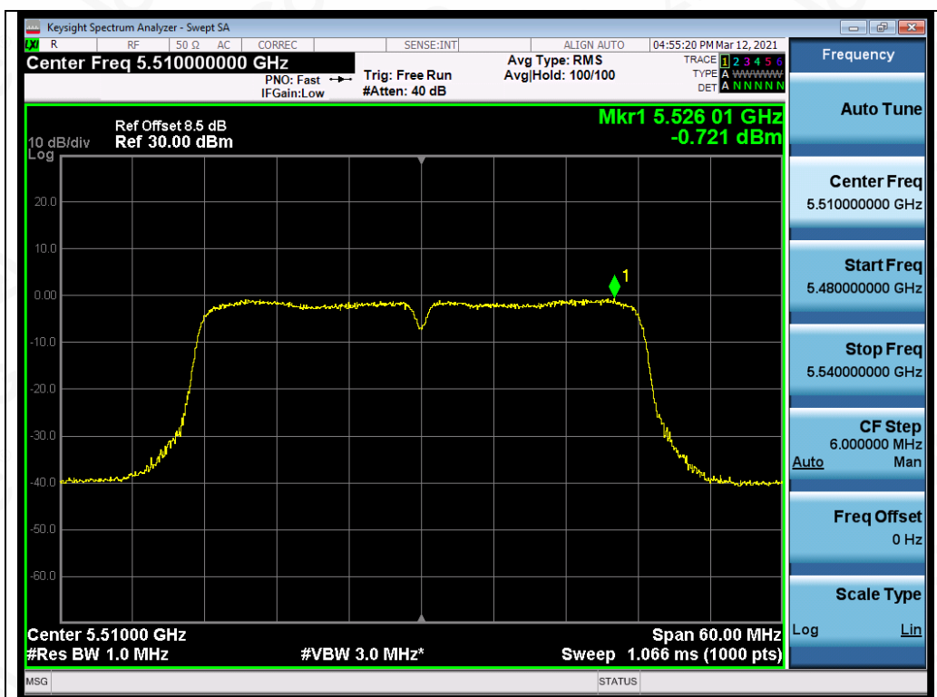
Test_Graph_802.11n40_ANT2_5510_MCS0_PSD
