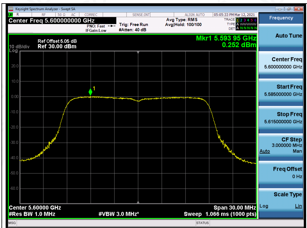
Test_Graph_802.11ac20_ANT2_5600_MCS0_PSD
