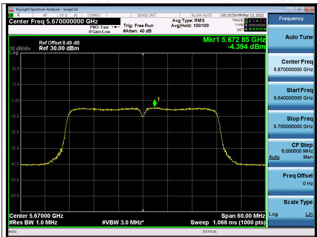
Test_Graph_802.11ac40_ANT2_5670_MCS9_PSD
