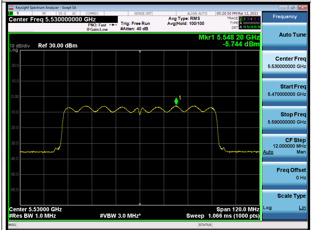
Test_Graph_802.11ac80_ANT2_5530_MCS9_PSD
