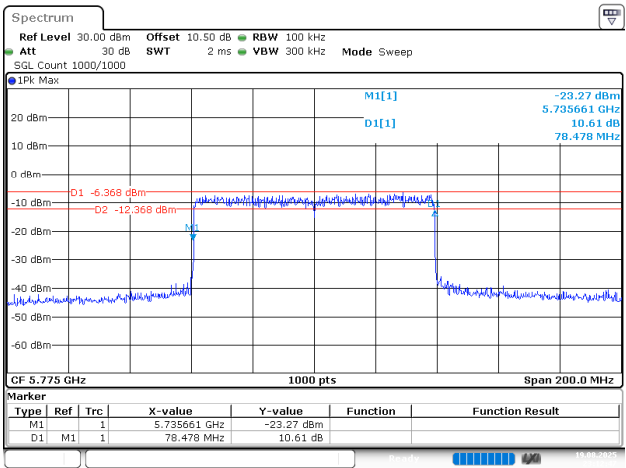
802.11ax80_5775MHz_Chain 0
