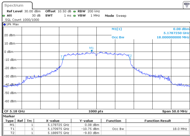
802.11n20_5180MHz_Chain 0
