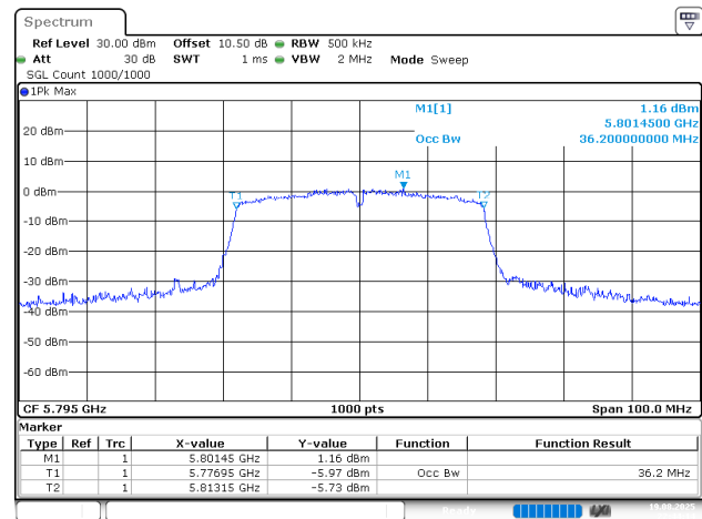
802.11n40_5795MHz_Chain 0
