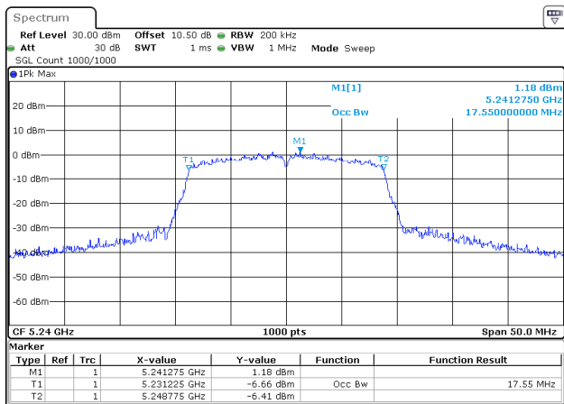
802.11n20_5240MHz_Chain 0
