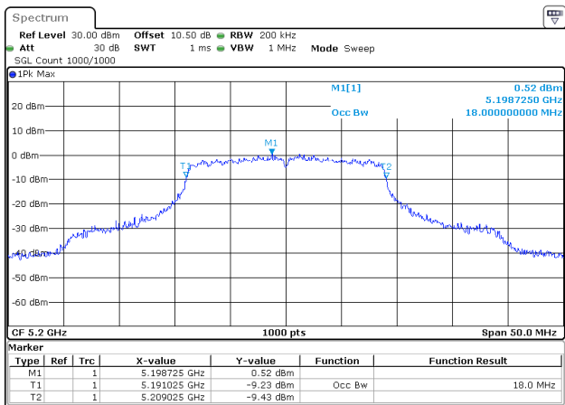
802.11n20_5200MHz_Chain 0
