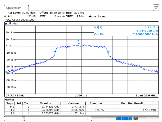
802.11a_5745MHz_Chain 0
