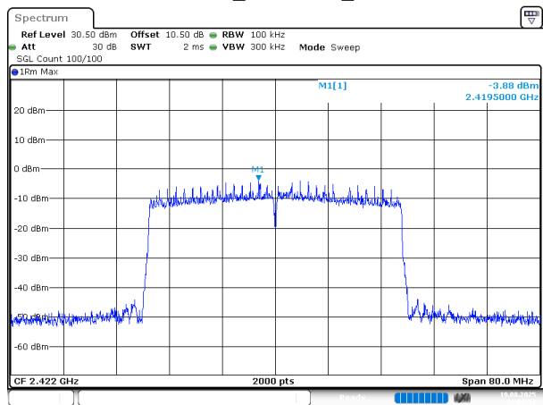
802.11ax40_2422MHz_Chain 0
