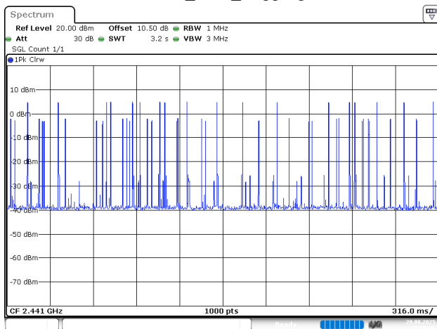
3EDR_DH3_Hopping
