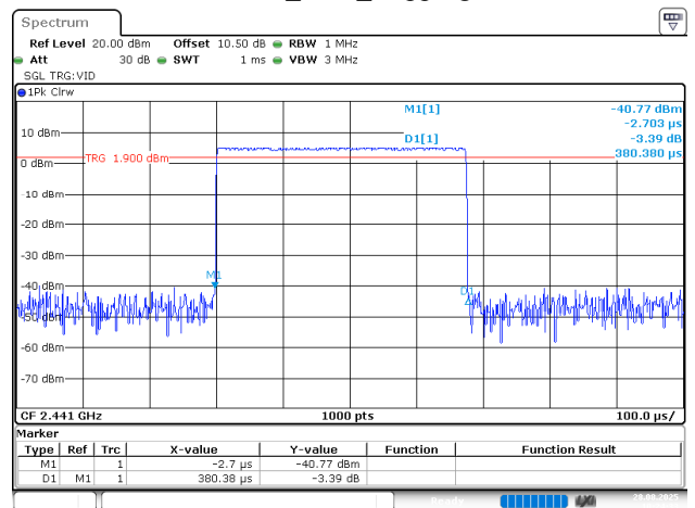
BDR_DH1_Hopping
