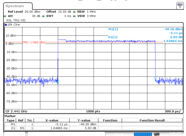
3EDR_DH3_Hopping
