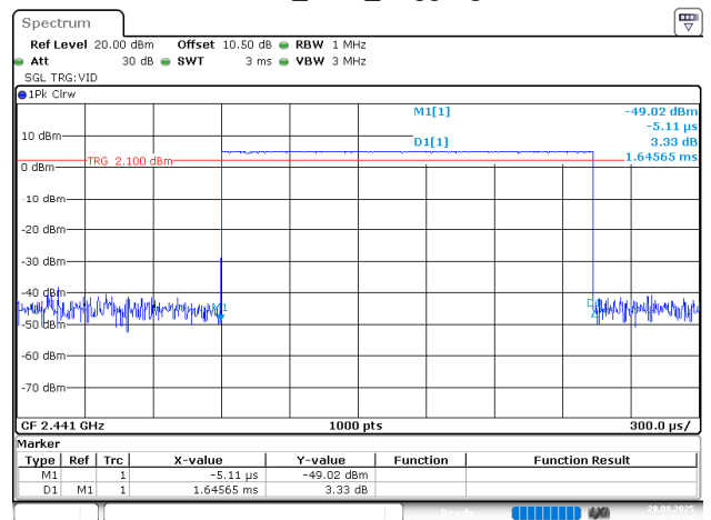
BDR_DH3_Hopping
