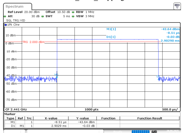
BDR_DH5_Hopping
