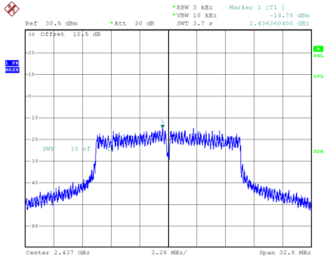
802.11g_2437MHz_Chain 1
