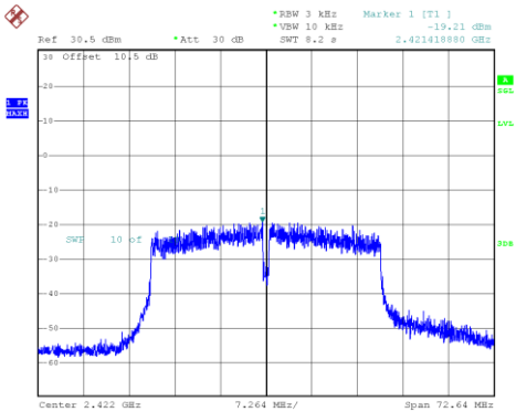
802.11n40_2422MHz_Chain 1
