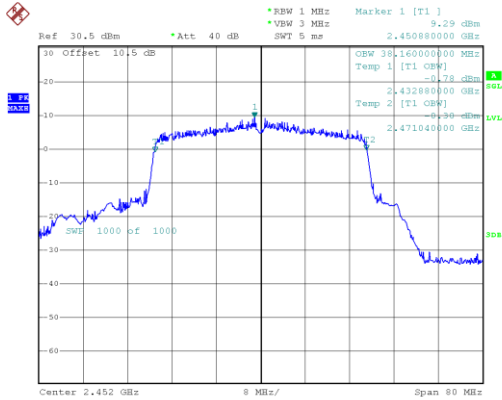
802.11ax40_2452MHz_RU_Full_Chain 0
