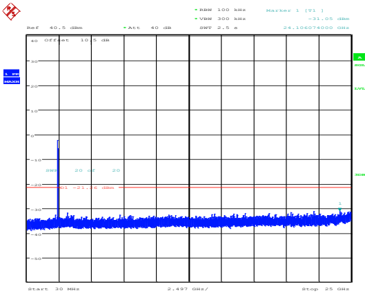
802.11ax40_2422MHz_RU_Full_Chain 1
