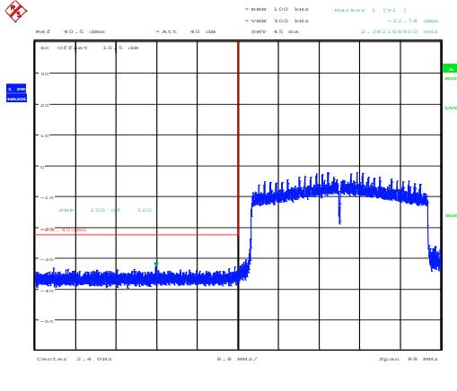
802.11ax40_2422MHz_RU_Full_Chain 0
