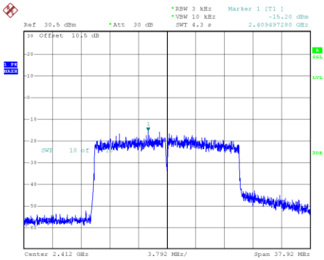
802.11ax20_2412MHz_RU_Full_Chain 0
