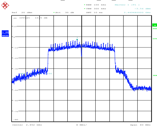
802.11ax40_2452MHz_RU_Full_Chain 1
