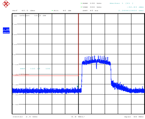
802.11ax20_2412MHz_RU_Full_Chain 0
