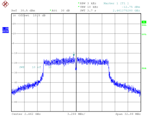
802.11g_2462MHz_Chain 0
