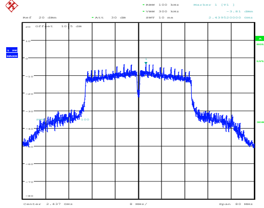
802.11n40_2437MHz_Chain 1
