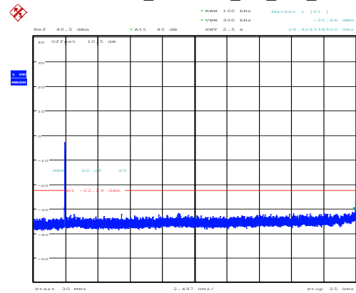
802.11ax40_2452MHz_RU_Full_Chain 0
