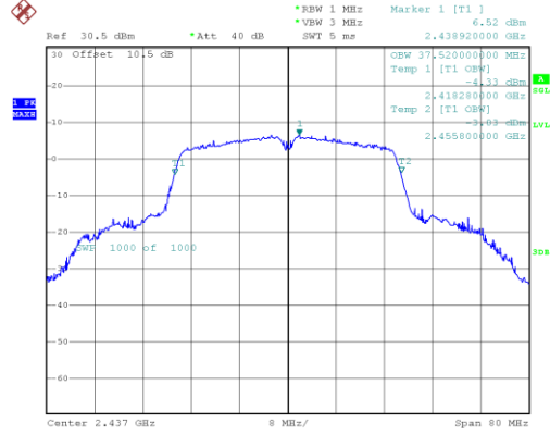
802.11n40_2437MHz_Chain 0
