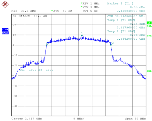
802.11ax40_2437MHz_RU_Full_Chain 0
