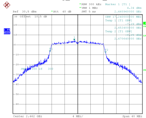
802.11g_2462MHz_Chain 0
