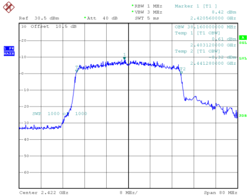
802.11ax40_2422MHz_RU_Full_Chain 0
