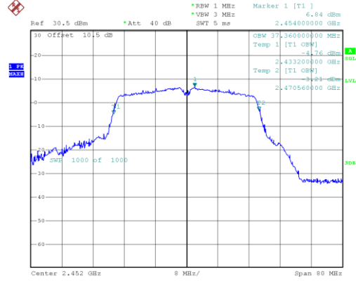
802.11n40_2452MHz_Chain 0
