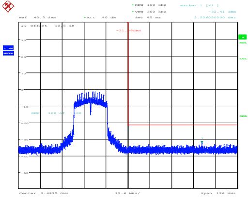
802.11ax20_2462MHz_RU_Full_Chain 1
