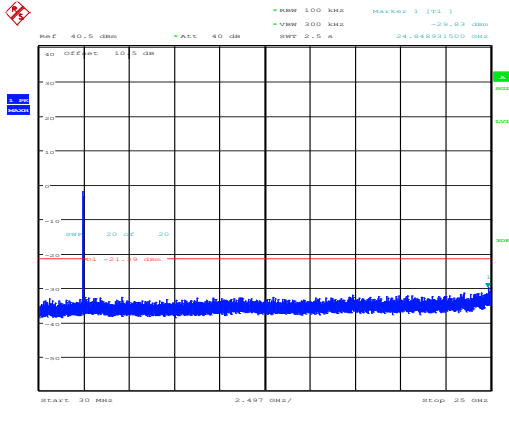
802.11ax20_2462MHz_RU_Full_Chain 1
