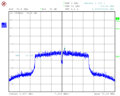
802.11n40_2437MHz_Chain 0
