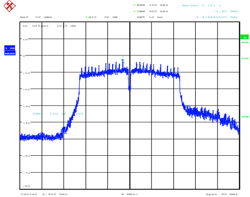
802.11n40_2422MHz_Chain 1
