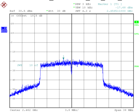
802.11ax20_2462MHz_RU_Full_Chain 1
