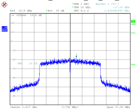
802.11ax20_2437MHz_RU_Full_Chain 1
