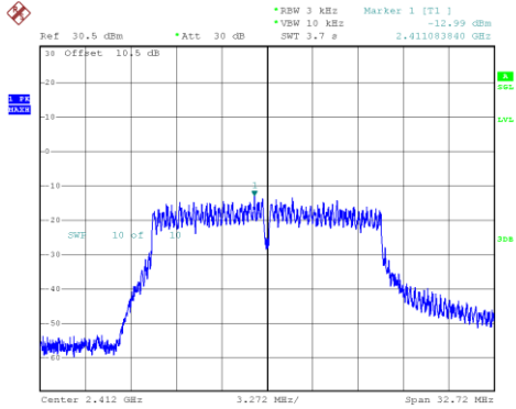
802.11g_2412MHz_Chain 0
