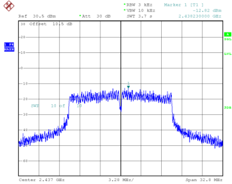
802.11g_2437MHz_Chain 0
