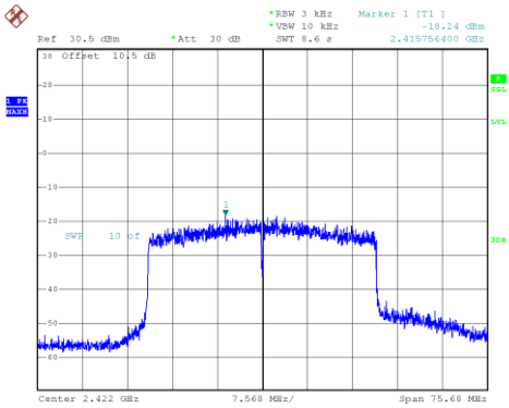
802.11ax40_2422MHz_RU_Full_Chain 0
