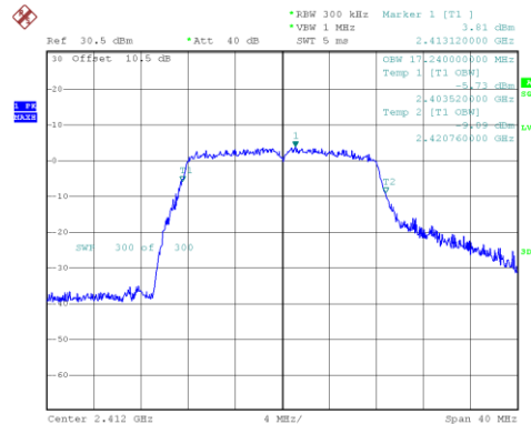
802.11g_2412MHz_Chain 0
