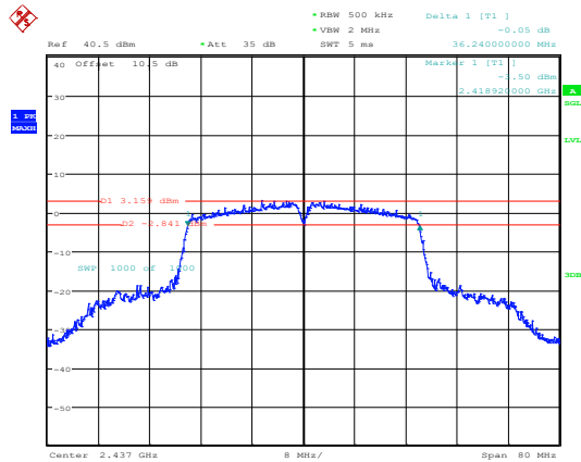
802.11n40_2437MHz_Chain 0
