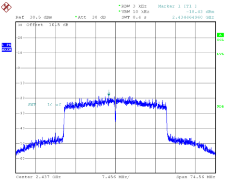
802.11ax40_2437MHz_RU_Full_Chain 0
