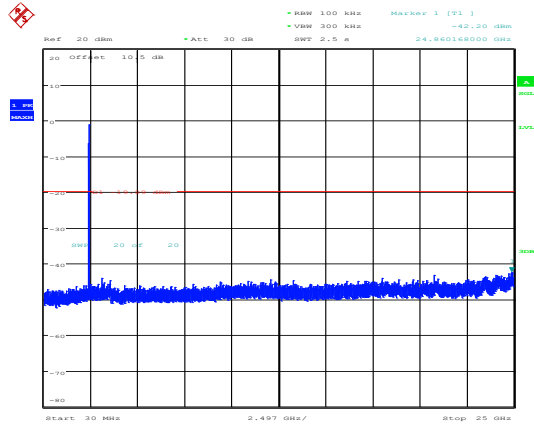
802.11ax20_2437MHz_RU_Full_Chain 0
