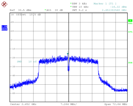
802.11n40_2452MHz_Chain 0
