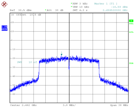
802.11ax20_2462MHz_RU_Full_Chain 0
