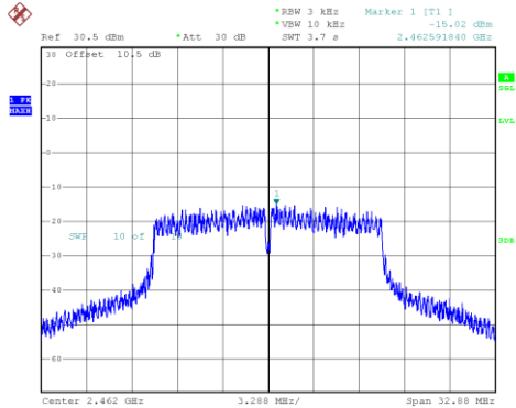
802.11g_2462MHz_Chain 1
