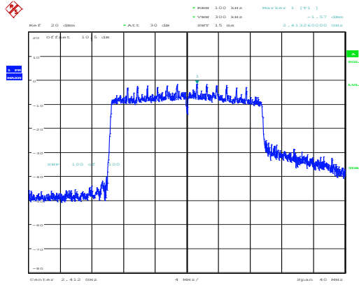
802.11ax20_2412MHz_RU_Full_Chain 0
