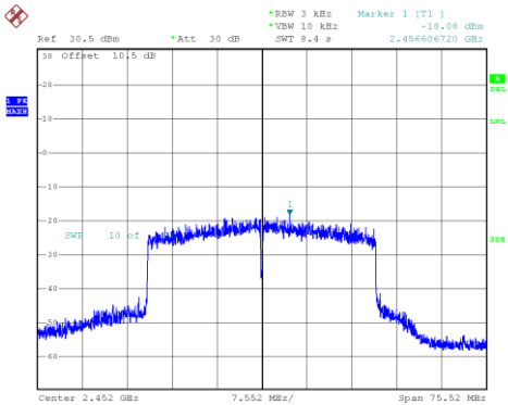
802.11ax40_2452MHz_RU_Full_Chain 0
