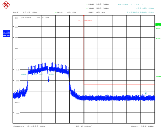
802.11n40_2452MHz_Chain 1
