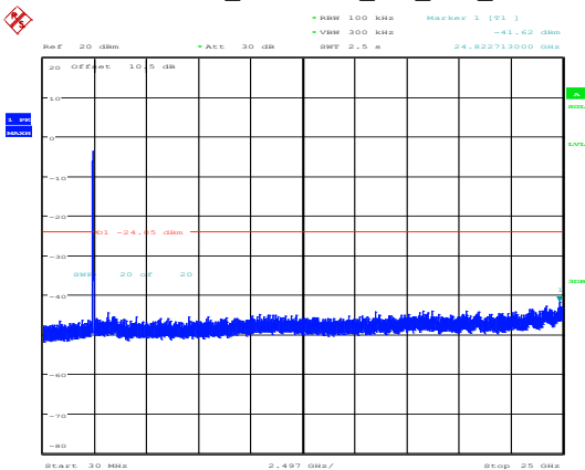
802.11ax40_2437MHz_RU_Full_Chain 1
