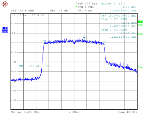
802.11ax20_2412MHz_RU_Full_Chain 0
