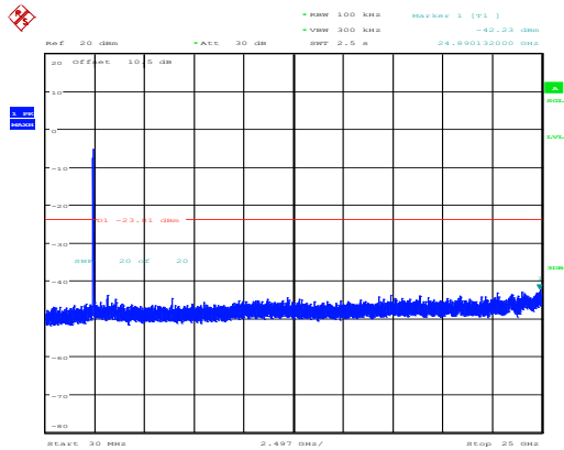
802.11n40_2437MHz_Chain 1
