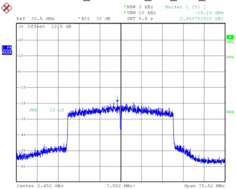
802.11ax40_2452MHz_RU_Full_Chain 1
