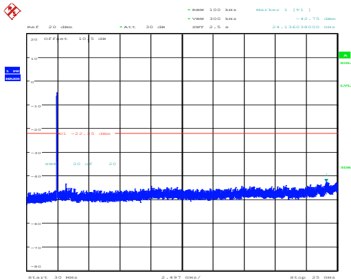
802.11n40_2437MHz_Chain 0
