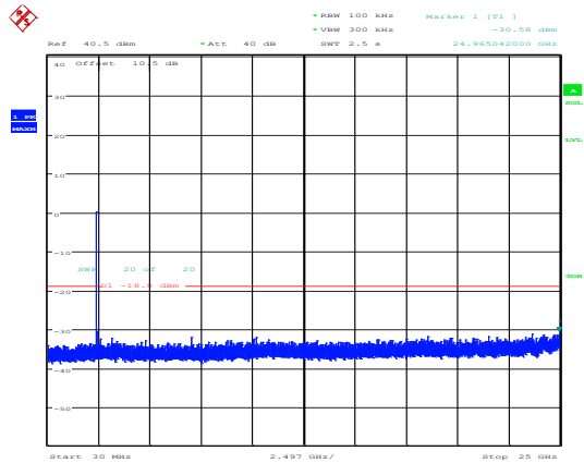
802.11g_2412MHz_Chain 0
