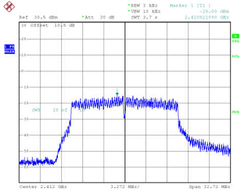
802.11g_2412MHz_Chain 1
