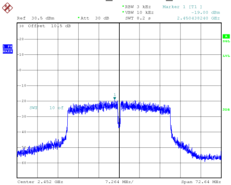
802.11n40_2452MHz_Chain 1
