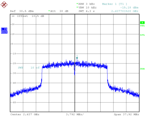
802.11ax20_2437MHz_RU_Full_Chain 0
