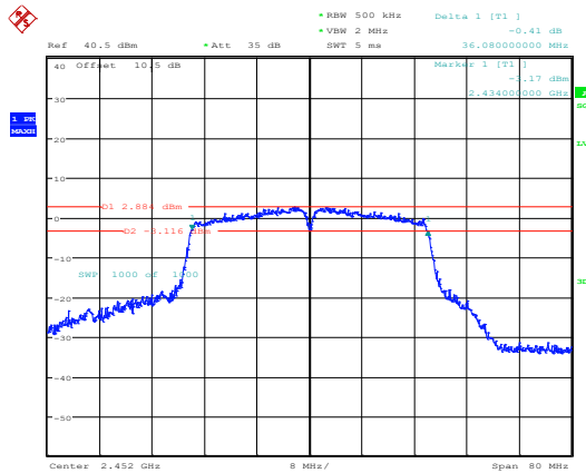
802.11n40_2452MHz_Chain 0
