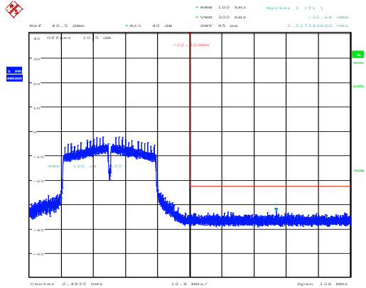
802.11n40_2452MHz_Chain 0
