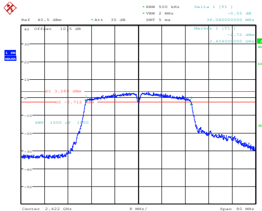
802.11n40_2422MHz_Chain 0
