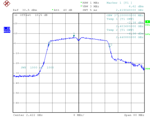
802.11n40_2422MHz_Chain 0
