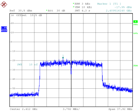
802.11ax20_2412MHz_RU_Full_Chain 1
