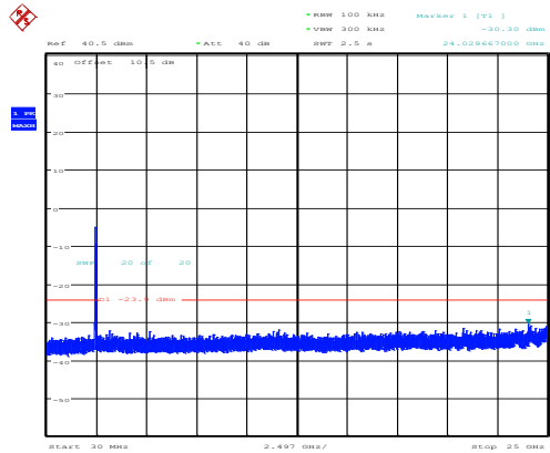
802.11n40_2452MHz_Chain 1
