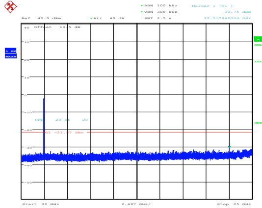
802.11ax20_2412MHz_RU_Full_Chain 0
