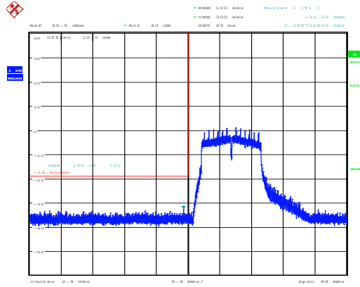
802.11g_2412MHz_Chain 0
