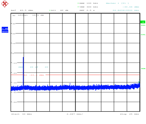
802.11ax40_2422MHz_RU_Full_Chain 0
