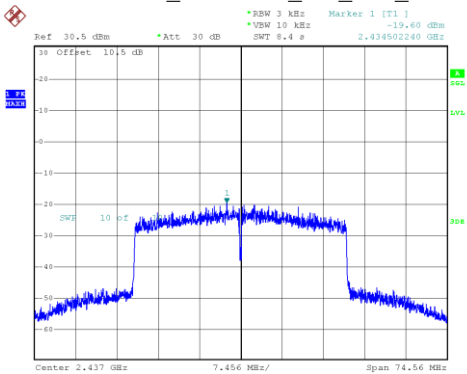
802.11ax40_2437MHz_RU_Full_Chain 1
