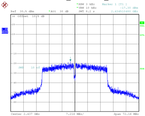
802.11n40_2437MHz_Chain 1
