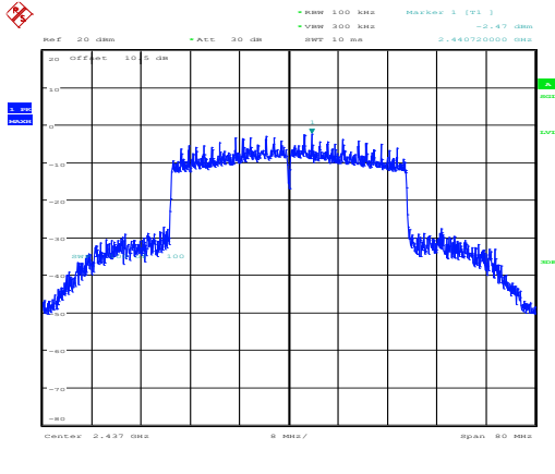
802.11ax40_2437MHz_RU_Full_Chain 0
