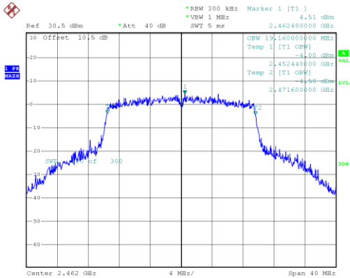
802.11ax20_2462MHz_RU_Full_Chain 0
