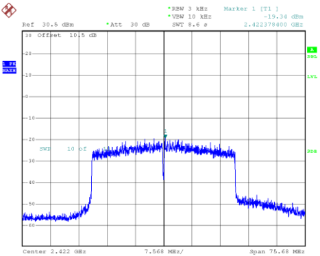
802.11ax40_2422MHz_RU_Full_Chain 1
