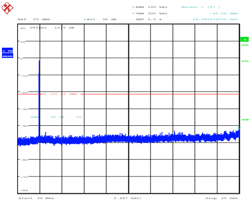
802.11ax20_2437MHz RU_Full_Chain 1
