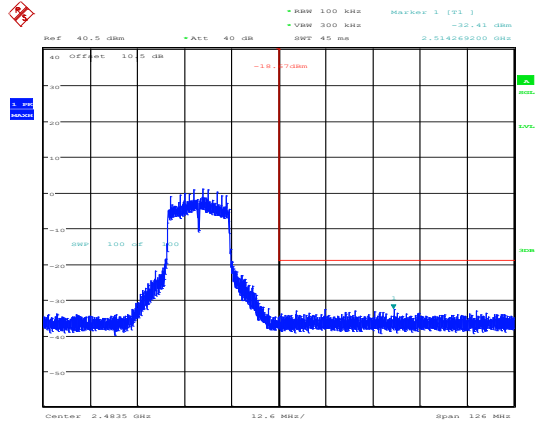
802.11g_2462MHz_Chain 0
