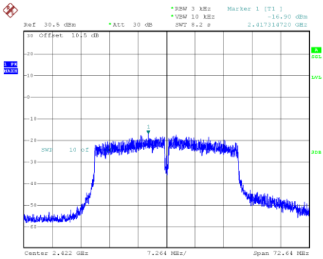
802.11n40_2422MHz_Chain 0
