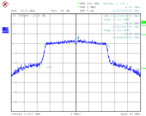
802.11ax20_2437MHz_RU_Full_Chain 0
