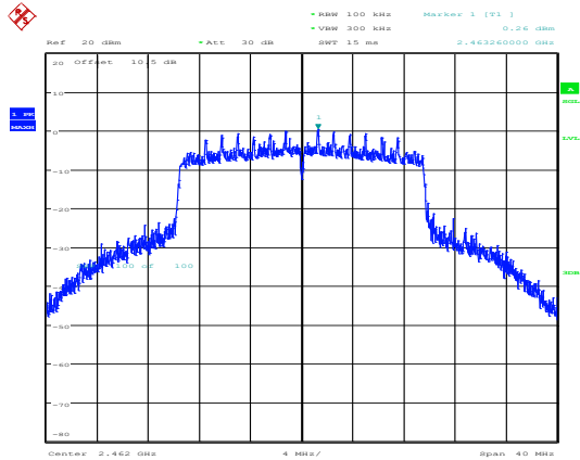
802.11ax20_2462MHz_RU_Full_Chain 0
