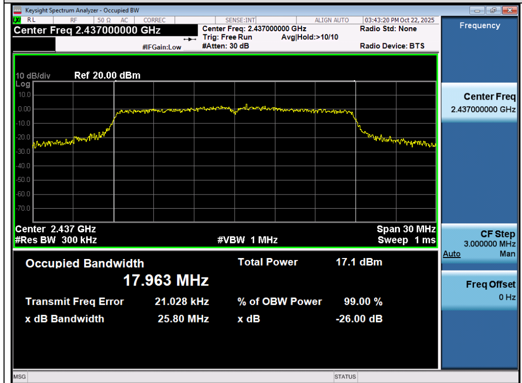
Test_Graph_802.11n20_Chain A_2437_MCS0_OBW
