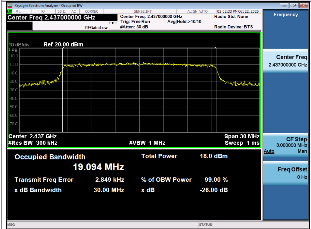
Test_Graph_802.11ax20_Chain B_2437_MCS0_OBW
