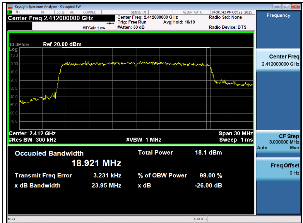
Test_Graph_802.11ax20_Chain A_2412_MCS0_OBW
