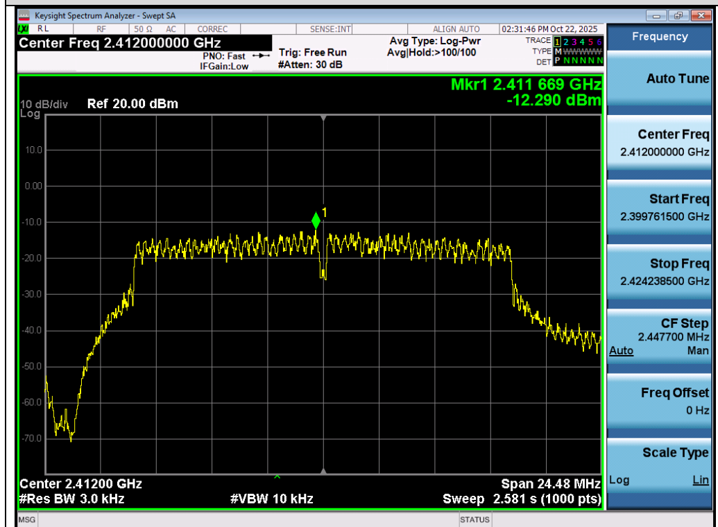
Test_Graph_802.11g_Chain B_2412_6Mbps_PSD
