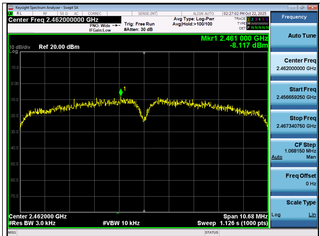
Test_Graph_802.11b_Chain B_2462_1Mbps_PSD
