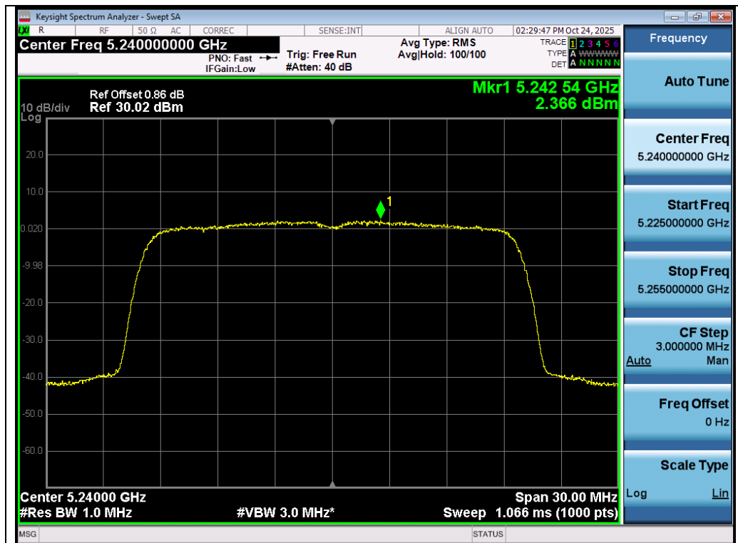
Test_Graph_802.11ax20_Chain B_5240_MCS0_PSD
