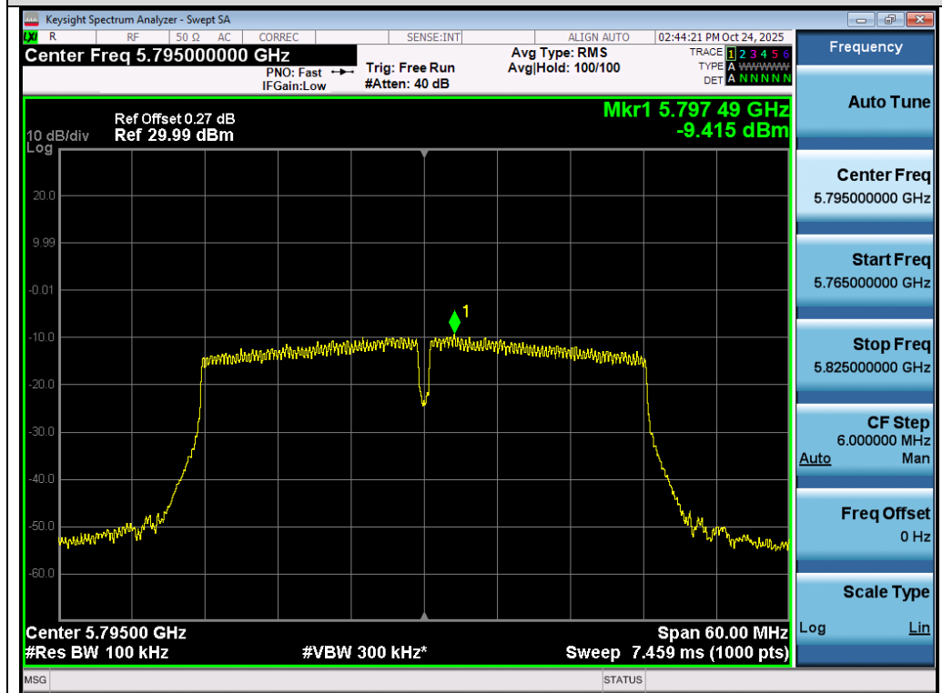
Test_Graph_802.11n40_Chain B_5795_MCS0_PSD
