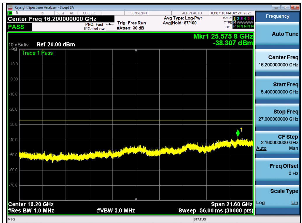
Test_Graph_802.11a_Chain A_5240_6Mbps_Frequency Band 4
