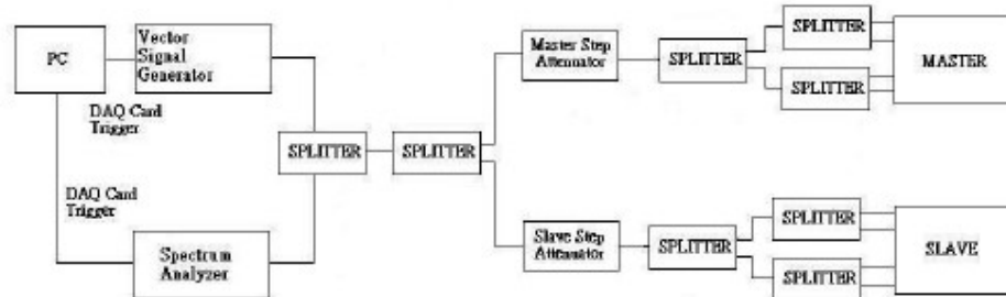
Conducted Method System Block Diagram
