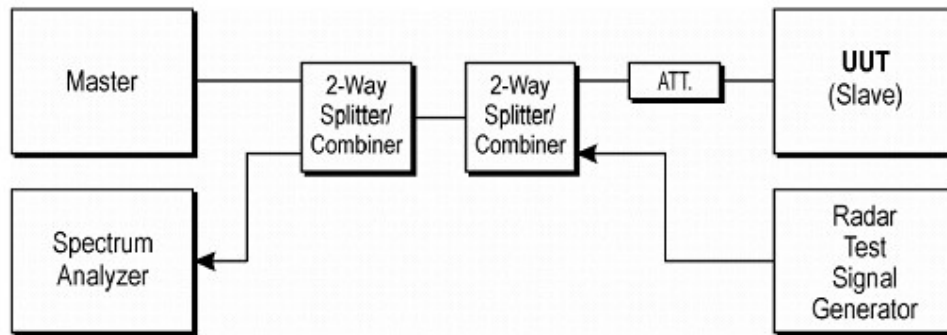
Figure 7-1. Test Setup
