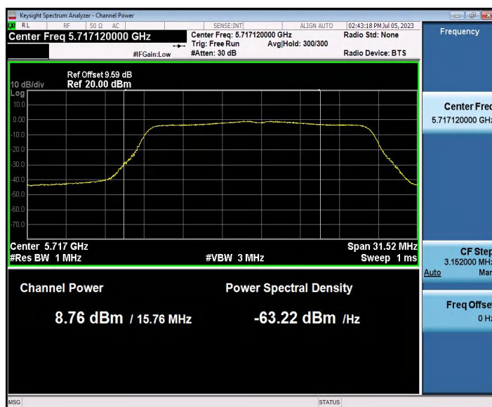
11AC20SISO_Ant1_5720_UNII-2C
