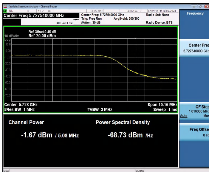
11AC40SISO_Ant1_5710_UNII-3
