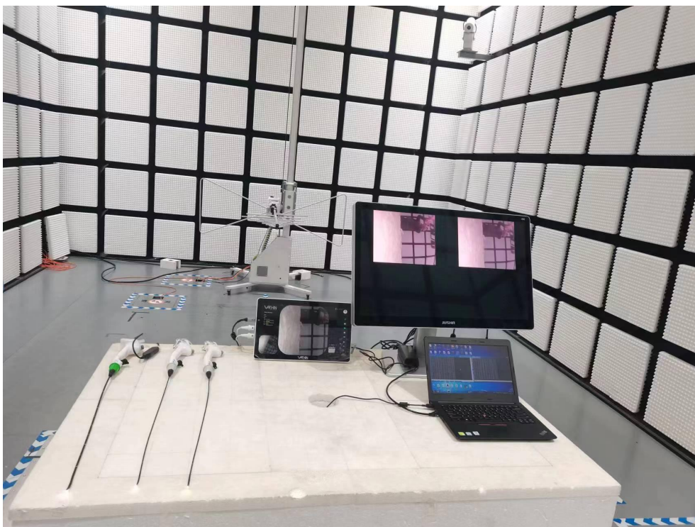
Fig. 1 Radiated emission setup photo(30MHz-1GHz)
