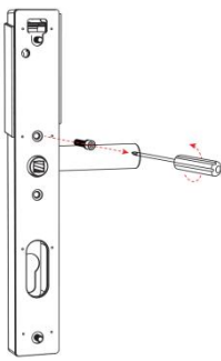
1.Loosen the screw.
