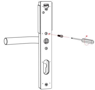
3.Tighten reverse screw.
