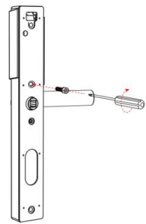
3.Tighten reverse screw.
